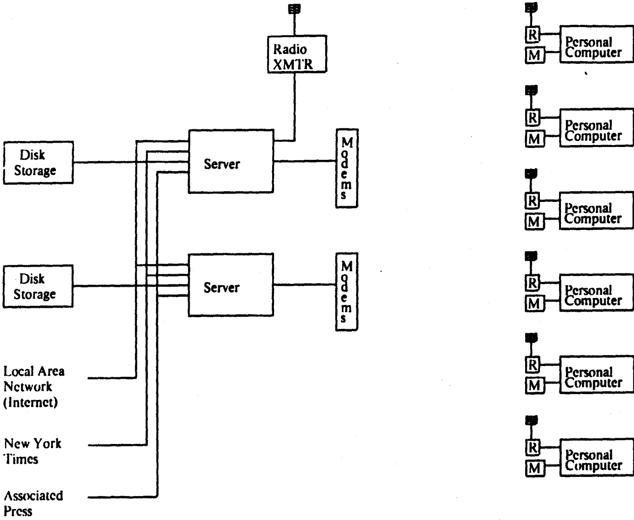
Figure 2-1: Boston CommInS System Block Diagram
