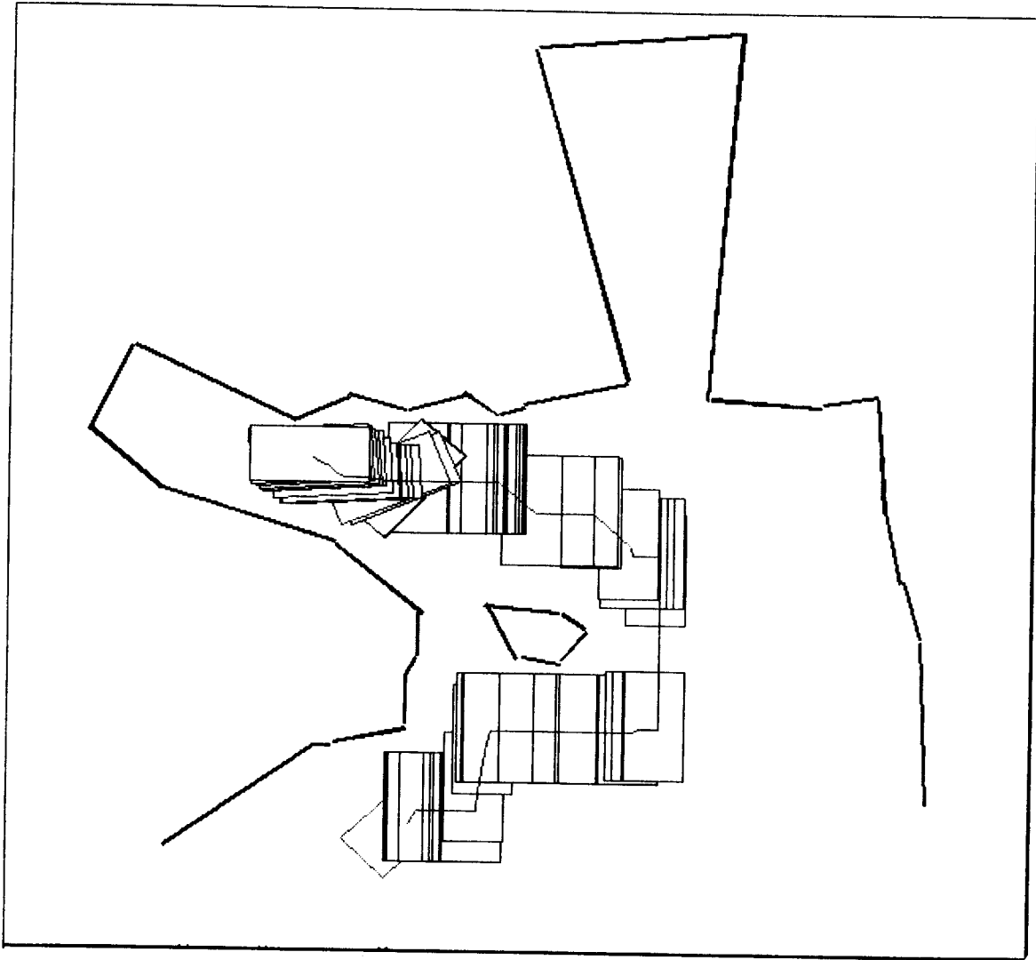
Figure 5-9: Configuration Space Planner
