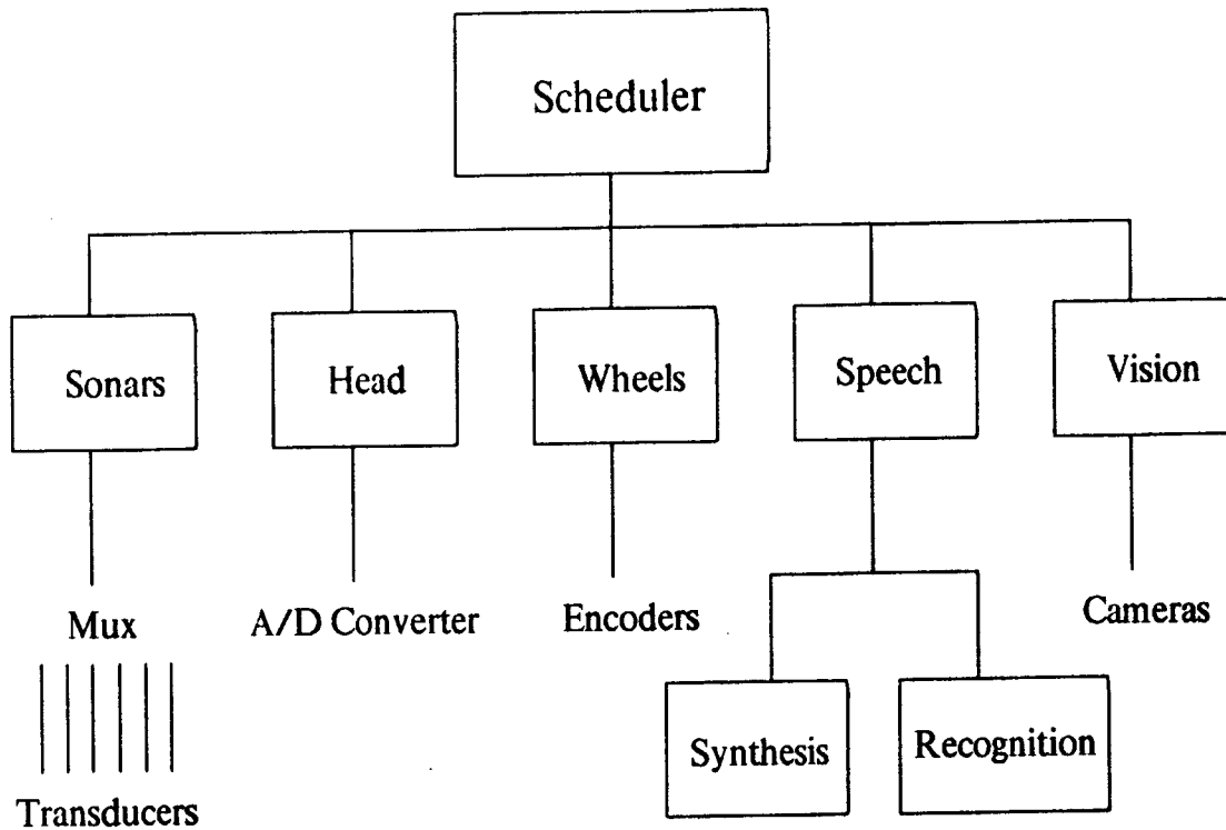
Figure 2-15: Architecture of the Controllers
