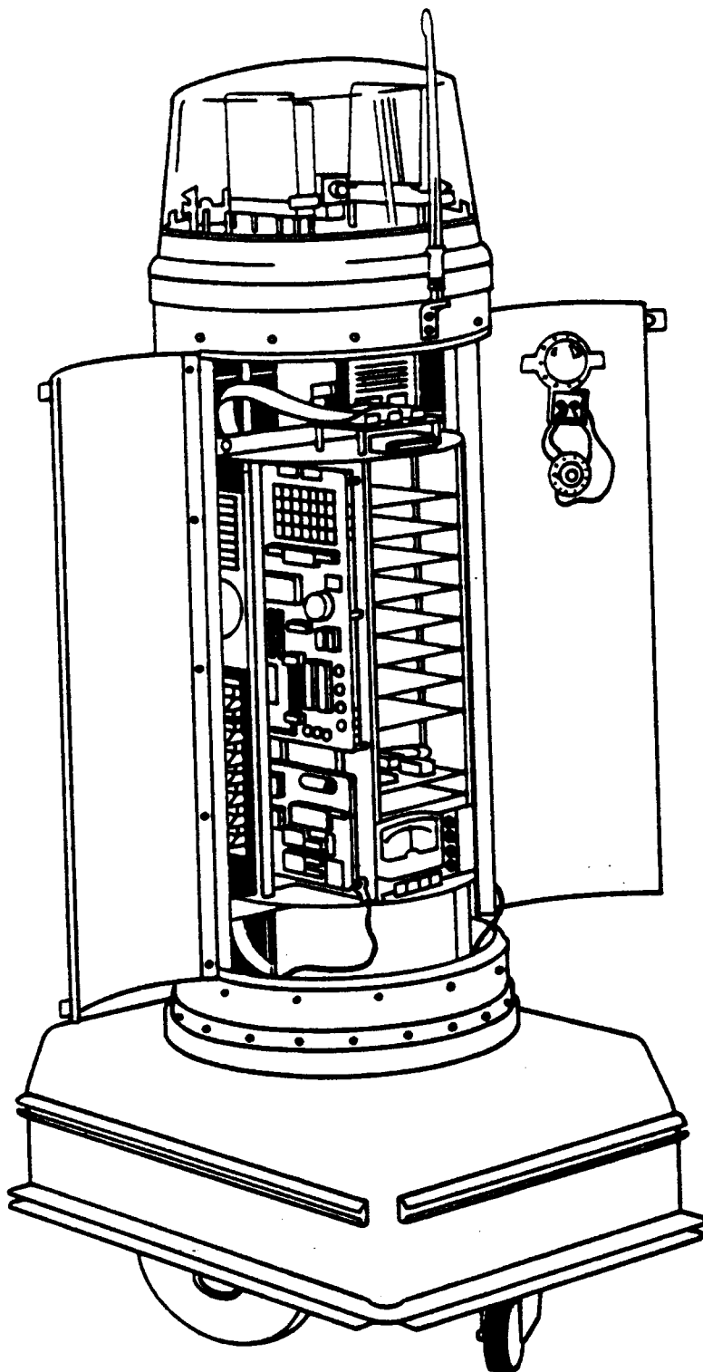
Figure 1-1:Robart II - An Autonomous Sentry Robot
