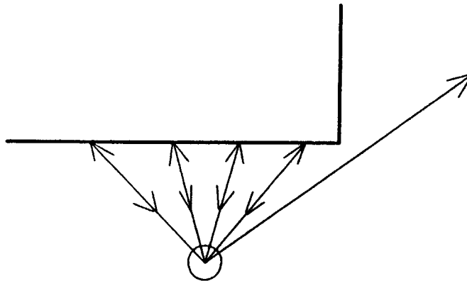
Figure 3-5: Infrared Sensor Finds a Corner
