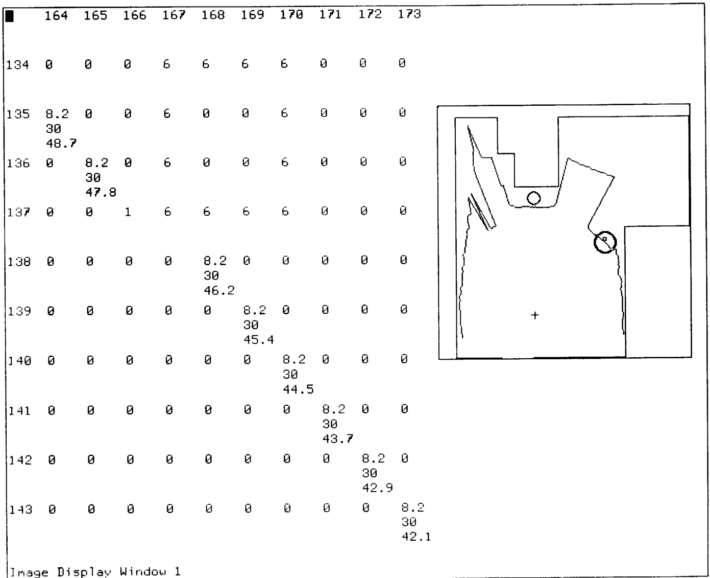
Figure 4-11: The Infrared Misses the Pole at 8.2 Feet
