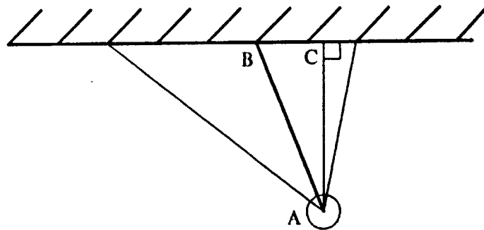
Figure 3-2: Sensor Measures Shortest Distance to a Wall
