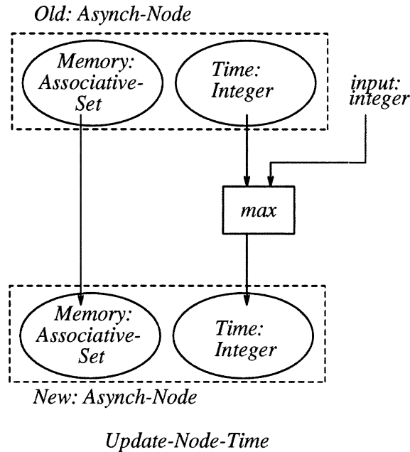
Figure 4-25: Plan definition for the Update-Node-Time cliché.
