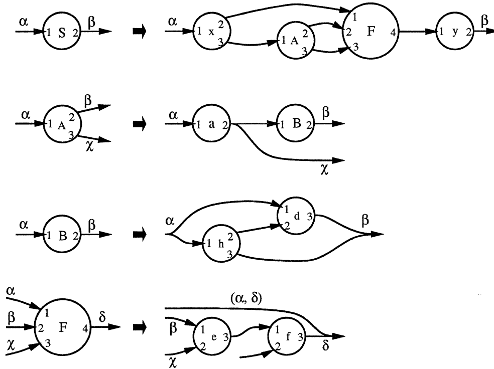
Figure 3-2: An example flow graph grammar.
