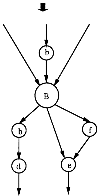
A legal reduction.
