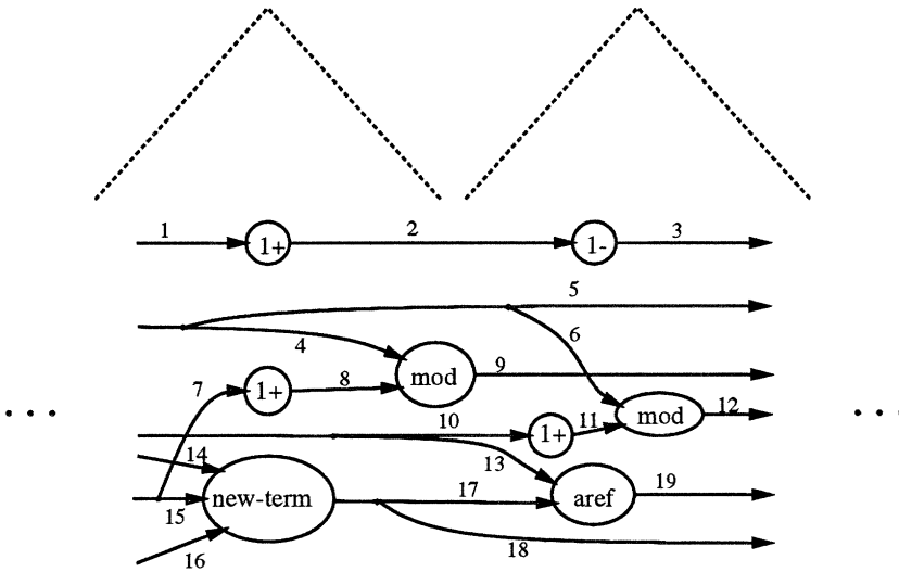
Input Graph
