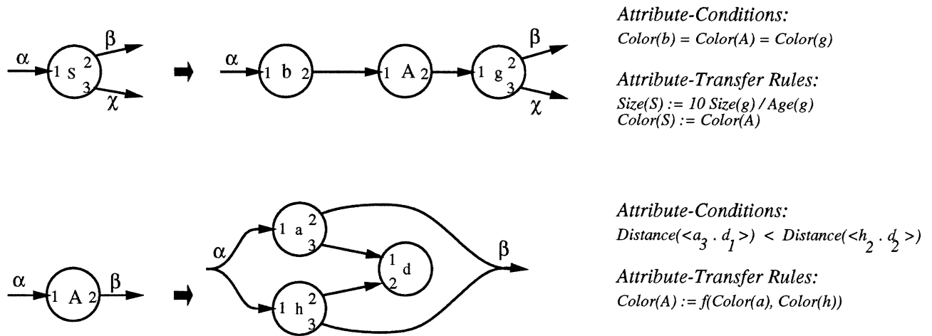
Figure 3-5: An example attributed flow graph grammar.
