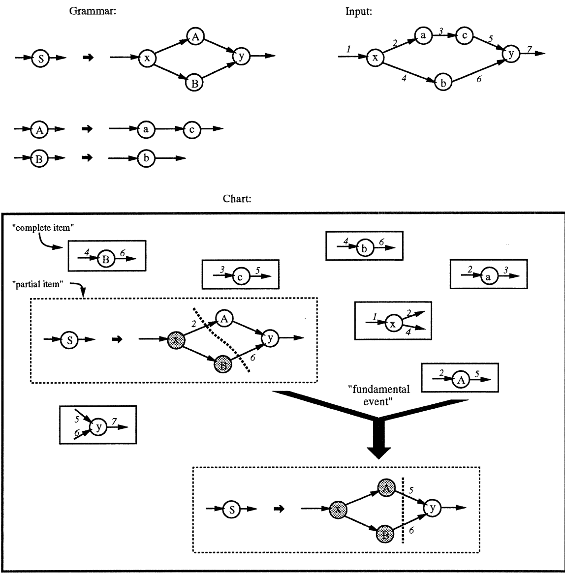
Figure 3-30: Graph chart parsing.
