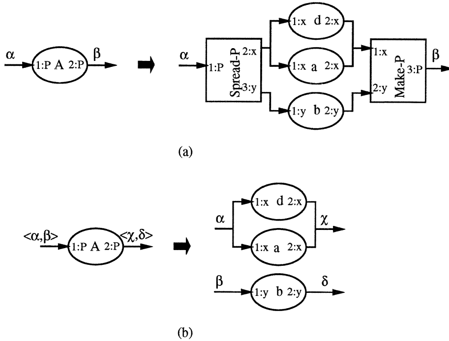
Figure 3-21: (a) A rule which aggregates port types. (b) The same rule with aggregation information moved to the embedding relation.
