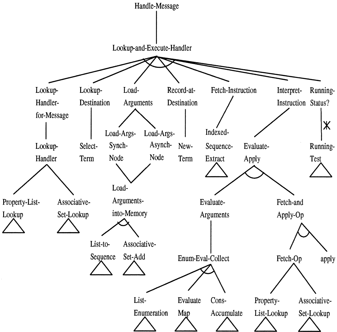
Figure 2-4: Node action simulation clichés.
