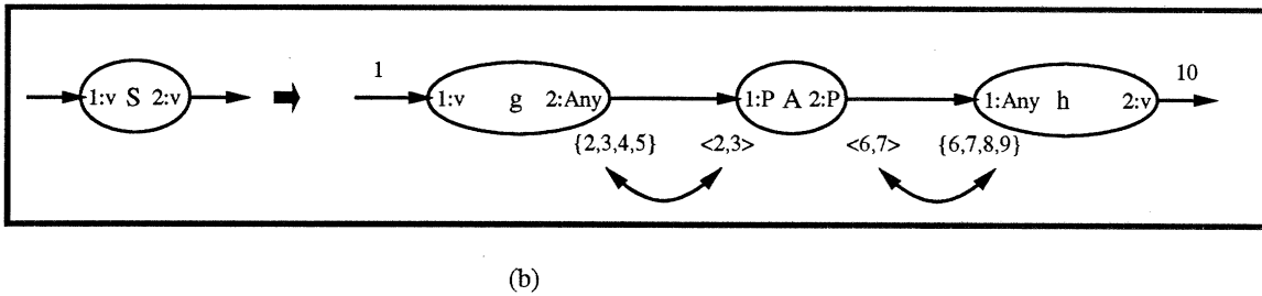
Figure 3-38: Simulating the break up of residual Spreads and Makes.
