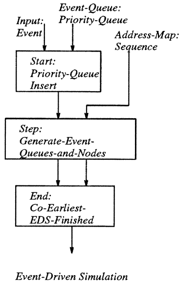
Figure 4-18: Plan definition for Event-Driven Simulation cliché.
