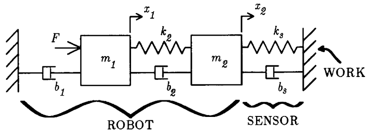
Figure 8: Robot Model Including Arm Dynamics Only
