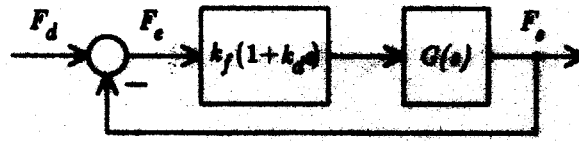
Figure 18: PD Force Control Law
