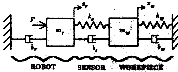
Figure 2: Robot Model Including Workpiece Dynamics
