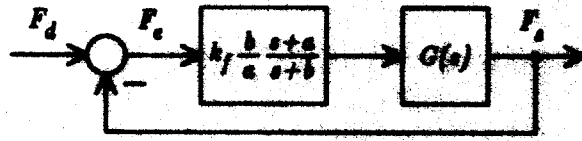
Figure 20: Load Compensator Force Control Law
