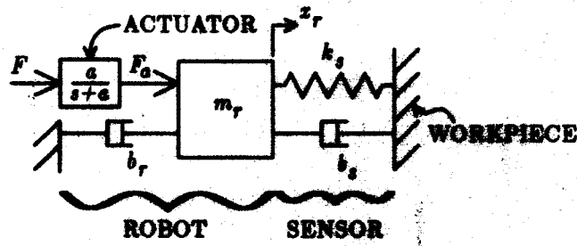
Figure 10: Rigid-Body Robot Model With Actuator Bandwidth Limitation
