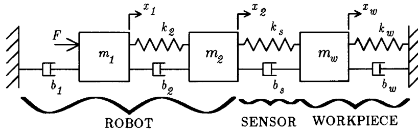
Figure 4: Robot Model Including Higher-Order Arm Dynamics
