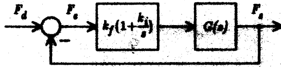
Figure 16: PI Force Control Law
