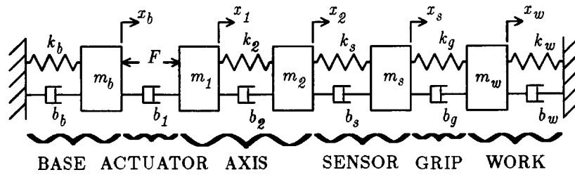
Figure 6: Robot Model Including Base, Sensor, and Grip
