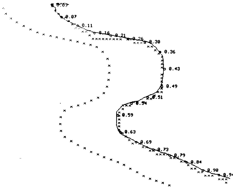
Figure 9. Dimensionality-reduction under sparsely sampled training data. During training, data was sampled from locations shown by X's at left. Each data sample was used repeatedly during training. Constraint curve found is shown displaced from the training data for clarity.
