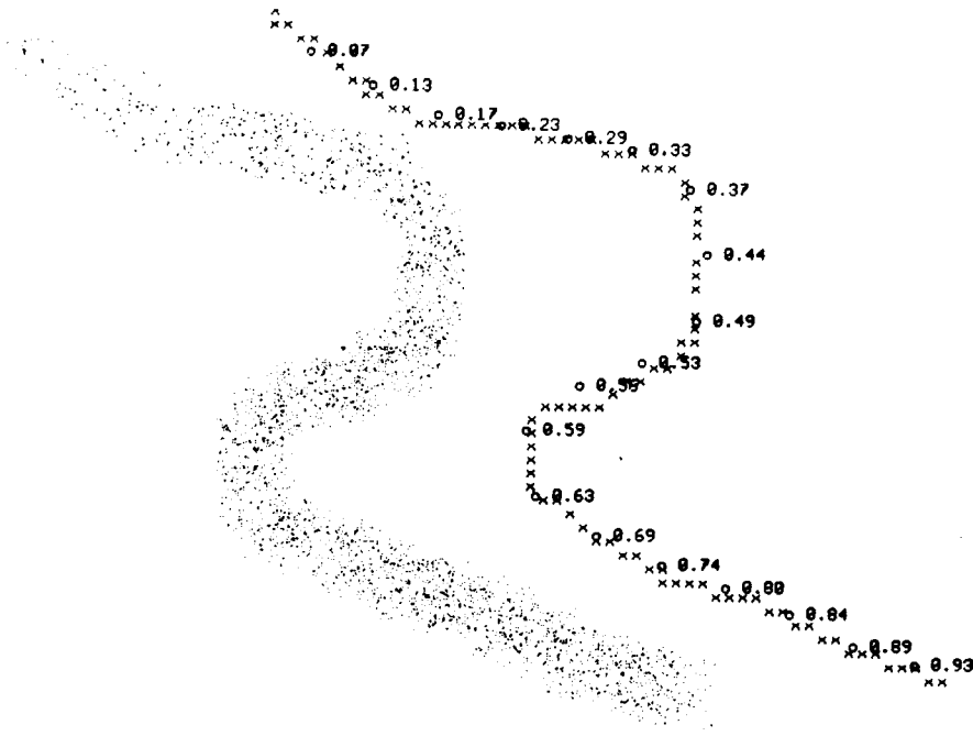
Figure 8. Dimensionality-reduction under noisy training data. For clarity, constraint curve found (denoted by x's) is shown displaced from the band of data samples used in training.
