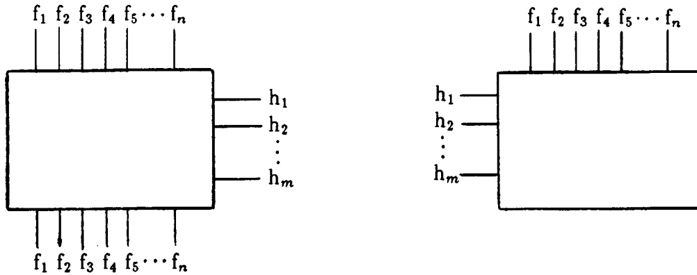
Figure 2. Black-box dimensionality-reducer.
