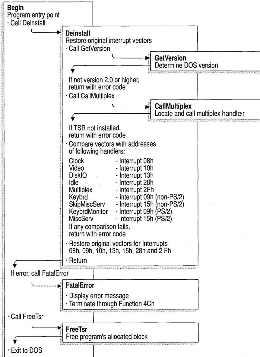
Figure 11.4 Flowchart for SNAP.EXE: Deinstallation Phase
