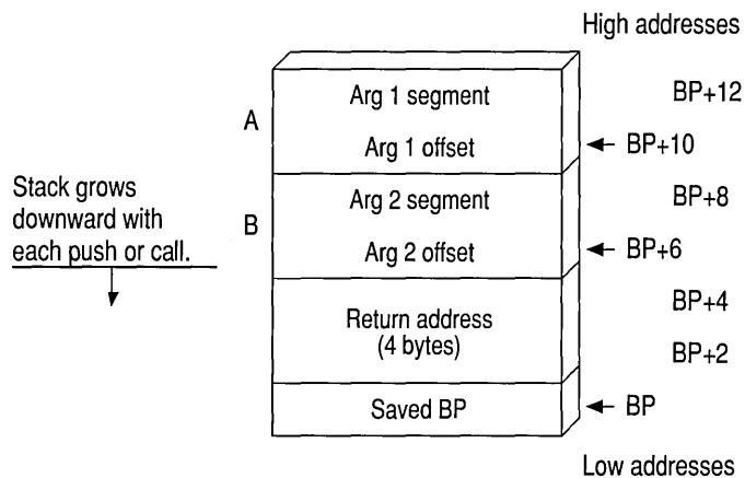
Figure 12.4 FORTRAN Stack Frame
