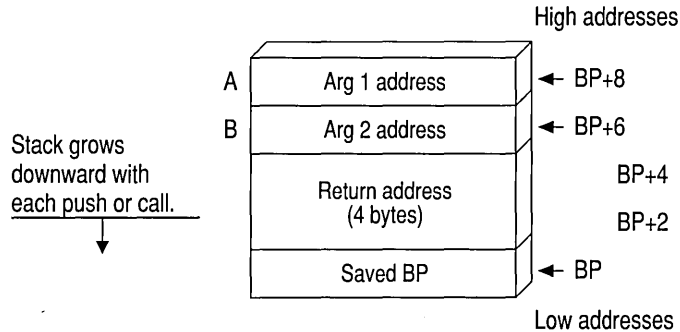
Figure 12.6 Basic Stack Frame
