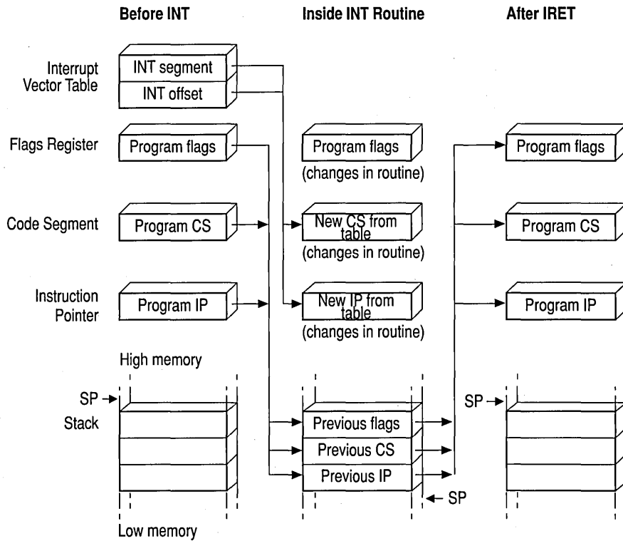
Figure 7.3 Operation of Interrupts
