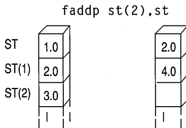
Figure 6.6 Status of the Already Initialized Register Stack
