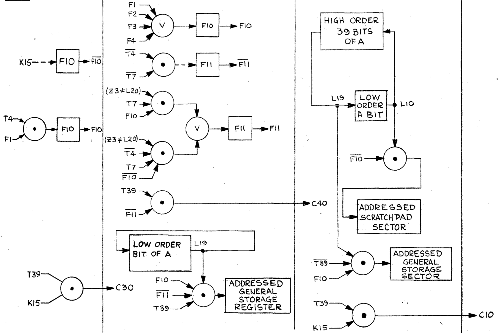
Figure 3.48.9 Store Command, Flow Chart.
