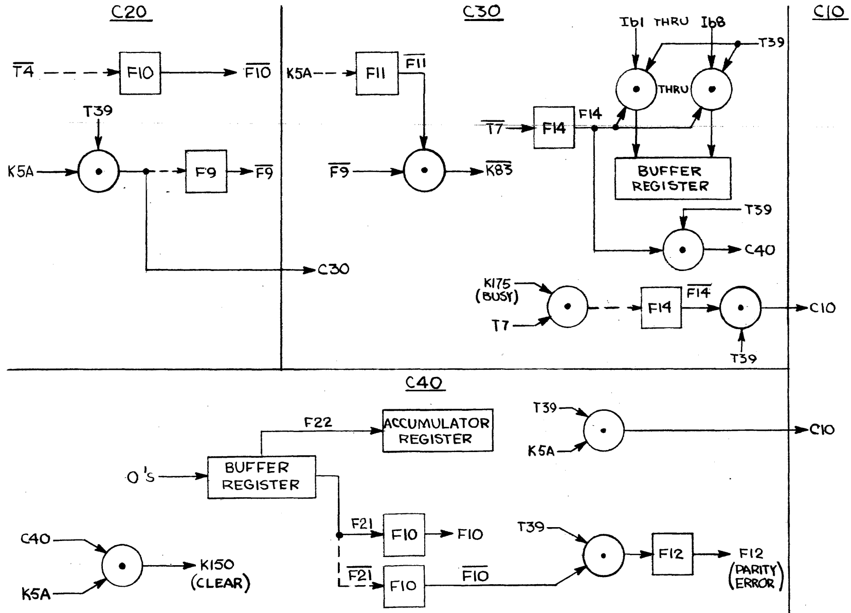
Figure 3.32 Clear, Input, Check Odd Parity Command, Flow Chart.
