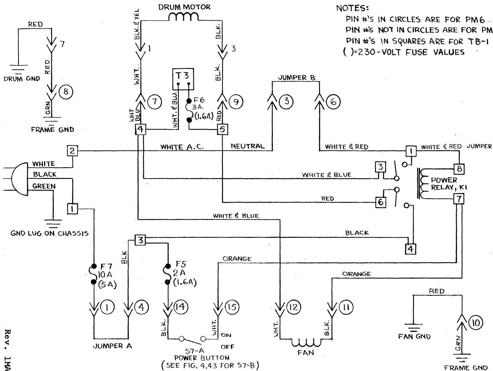
Figure 4.44 AC Wiring.
