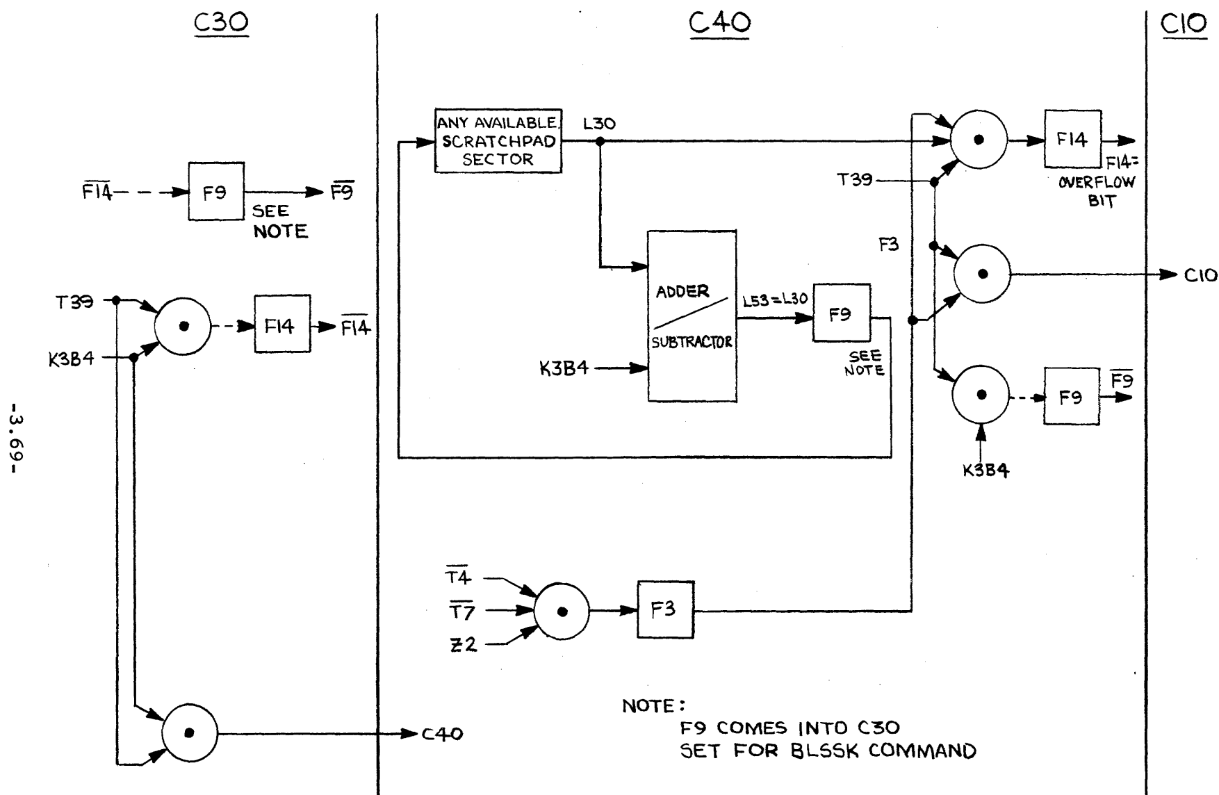
Figure 3.23 Binary Left Single Shift on Scratchpad Command and Binary Left Single Shift on Scratchpad Including K Command, Flow Chart.
