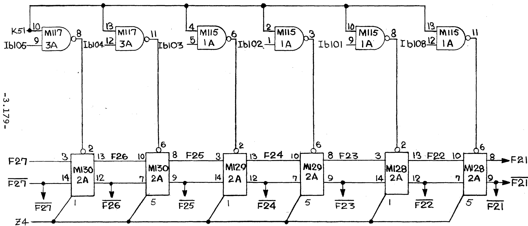
PART OF I/O BUFFER
