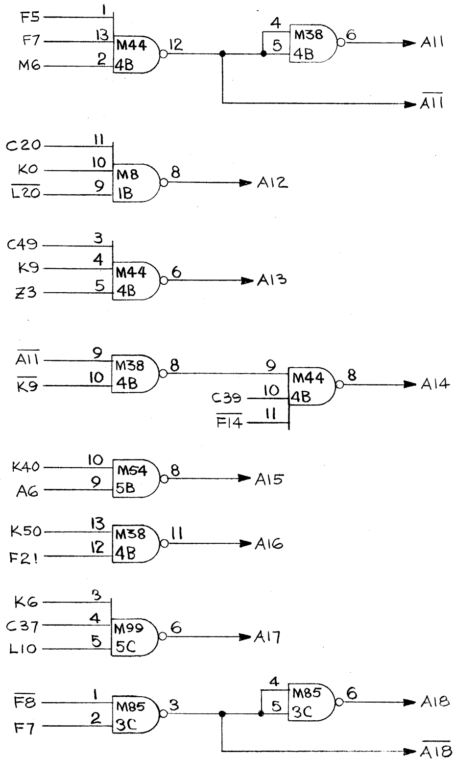
Figure 3.51 Logic Diagram.
