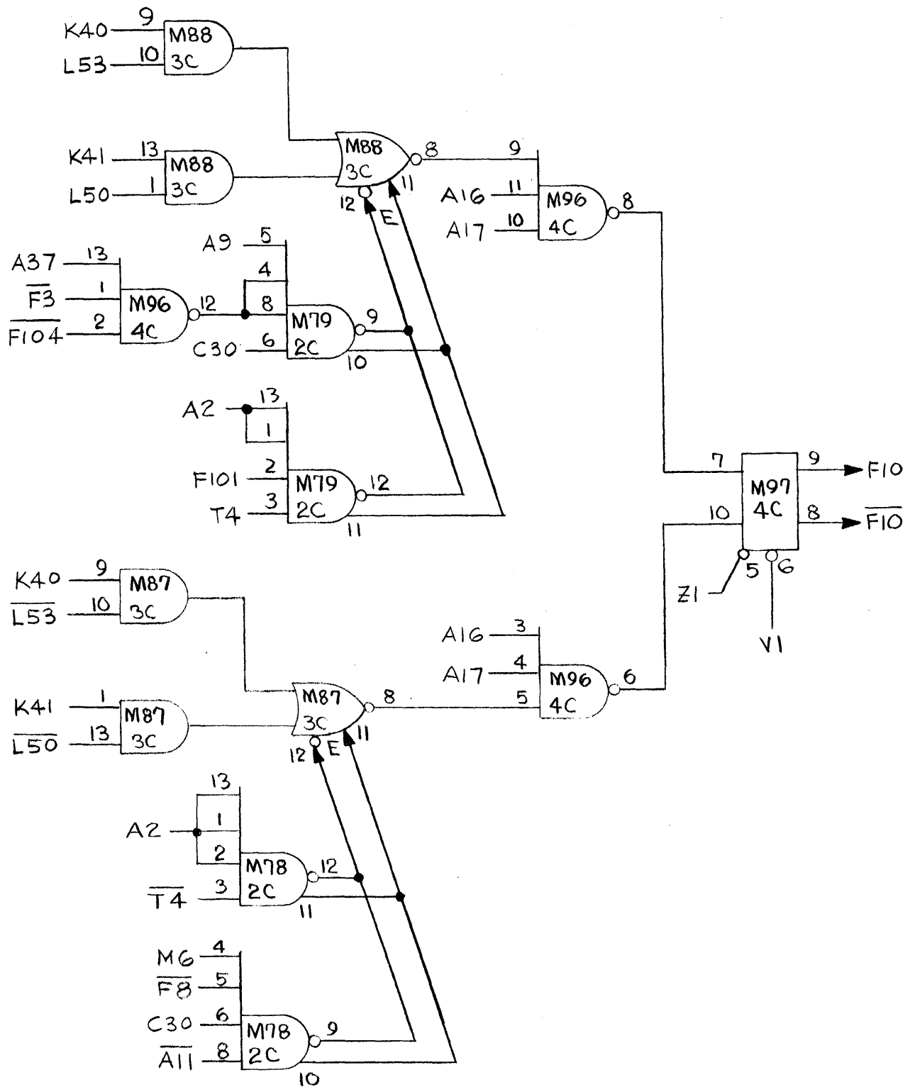
Figure 3.63 Logic Diagram.
