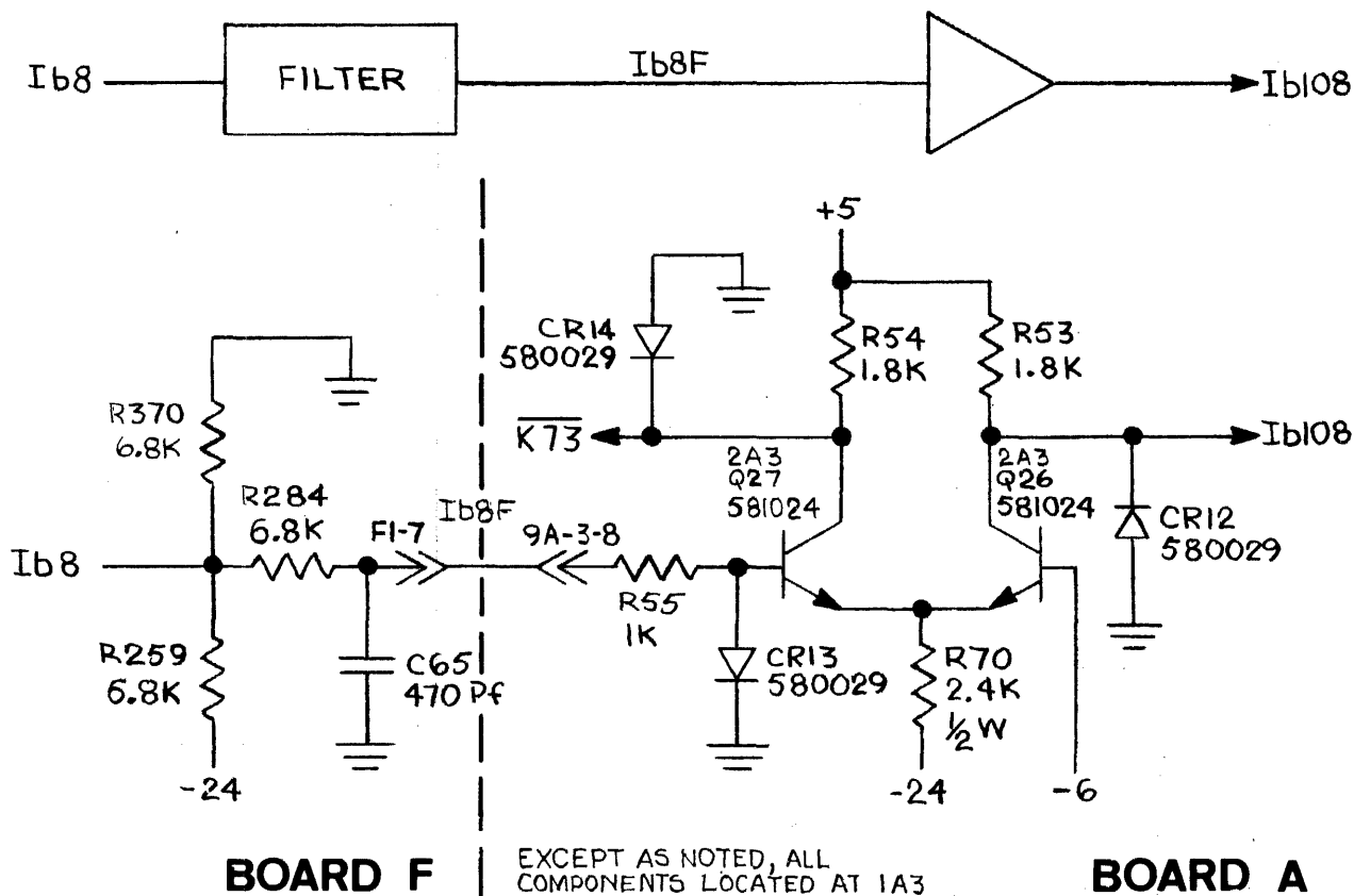
Figure 4.23 Input Circuits Ib108 and \overline{K73} .
