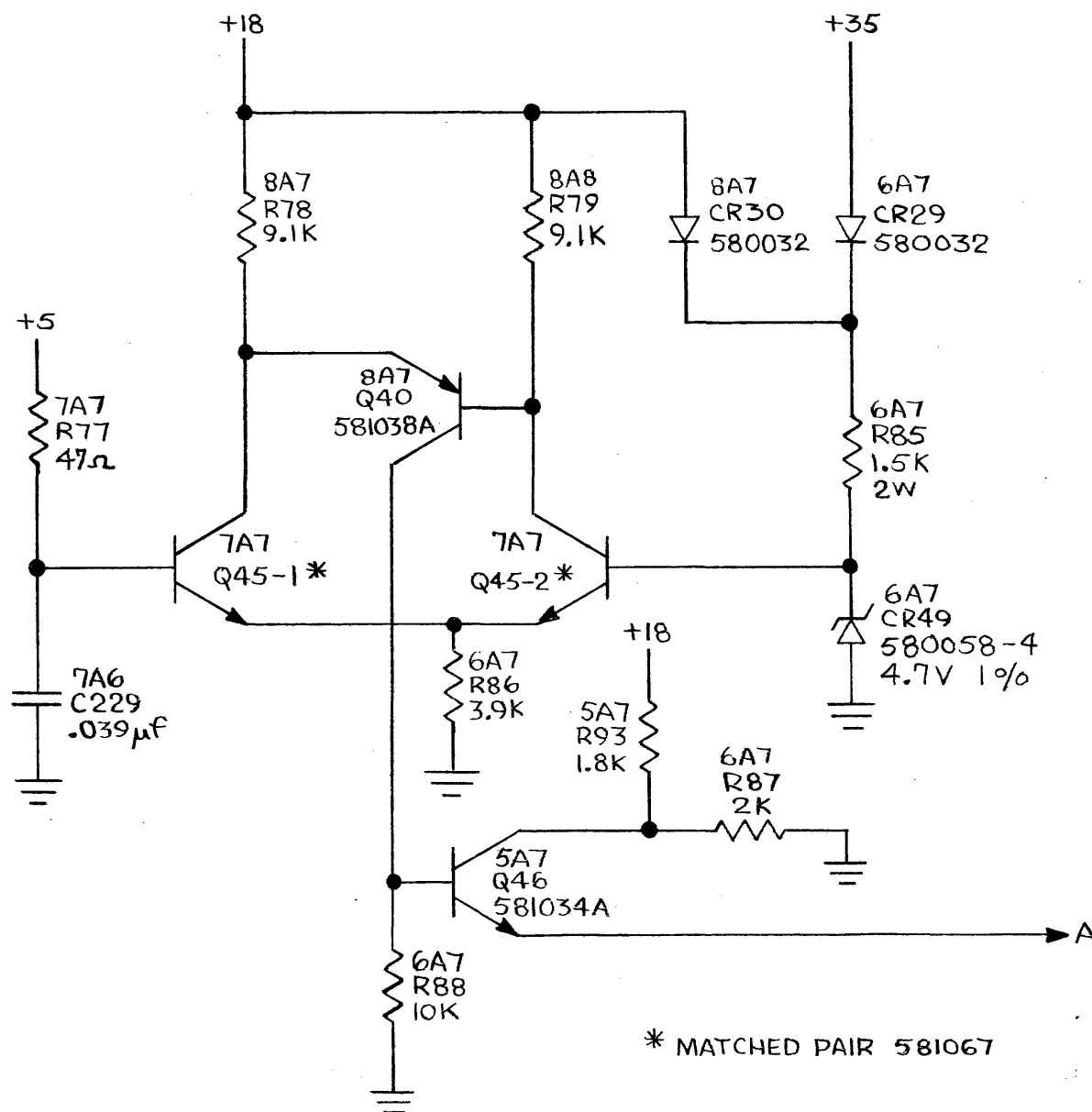
Figure 4.40 +5 Volt Check Circuit.
