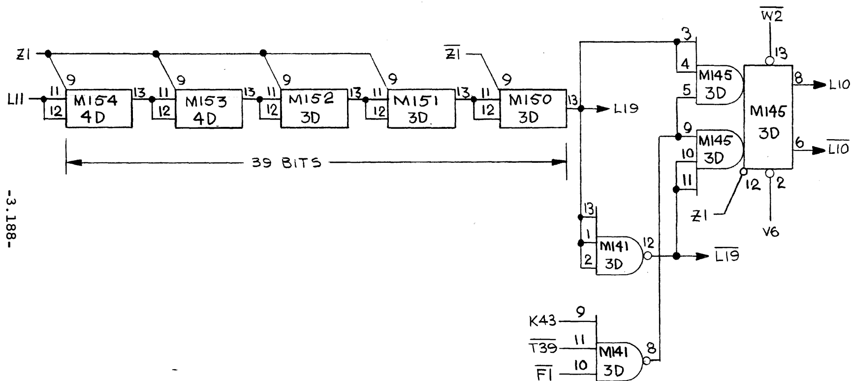
ACCUMULATOR 40 BITS Figure 3.80 Logic Diagram.
