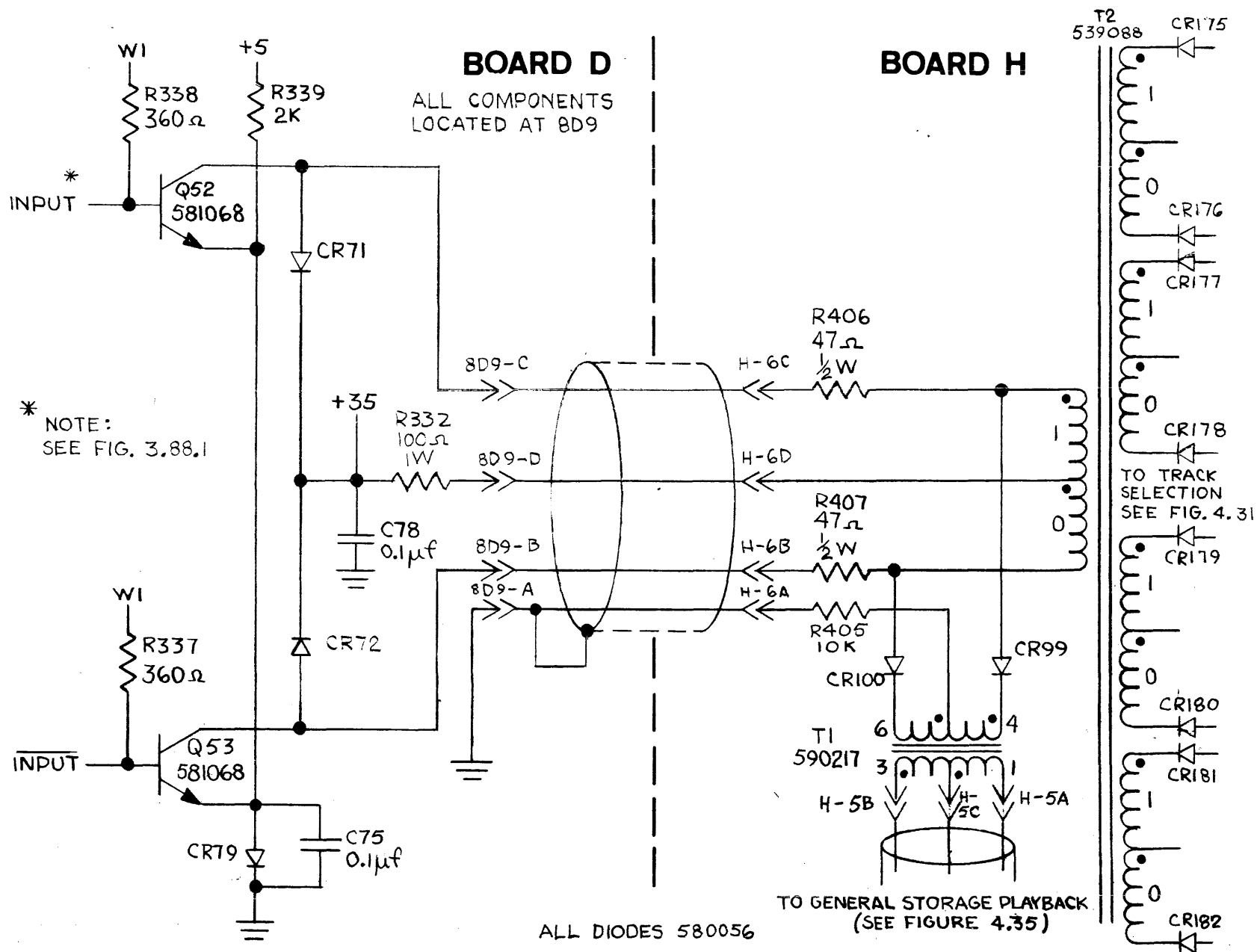
Figure 4.33 Record Circuit, General Storage.
