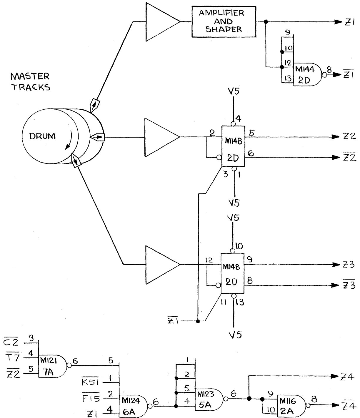
Figure 3.98 Logic Diagram.
