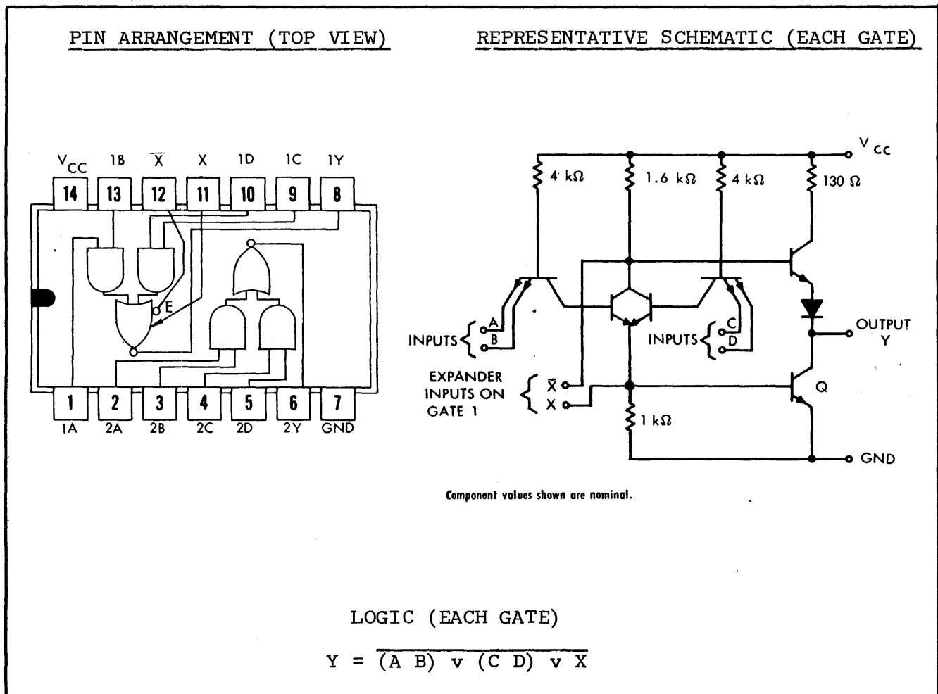
Figure 4.6 585012, Dual 2-Wide 2-Input AND-OR-Invert Gate Package.
