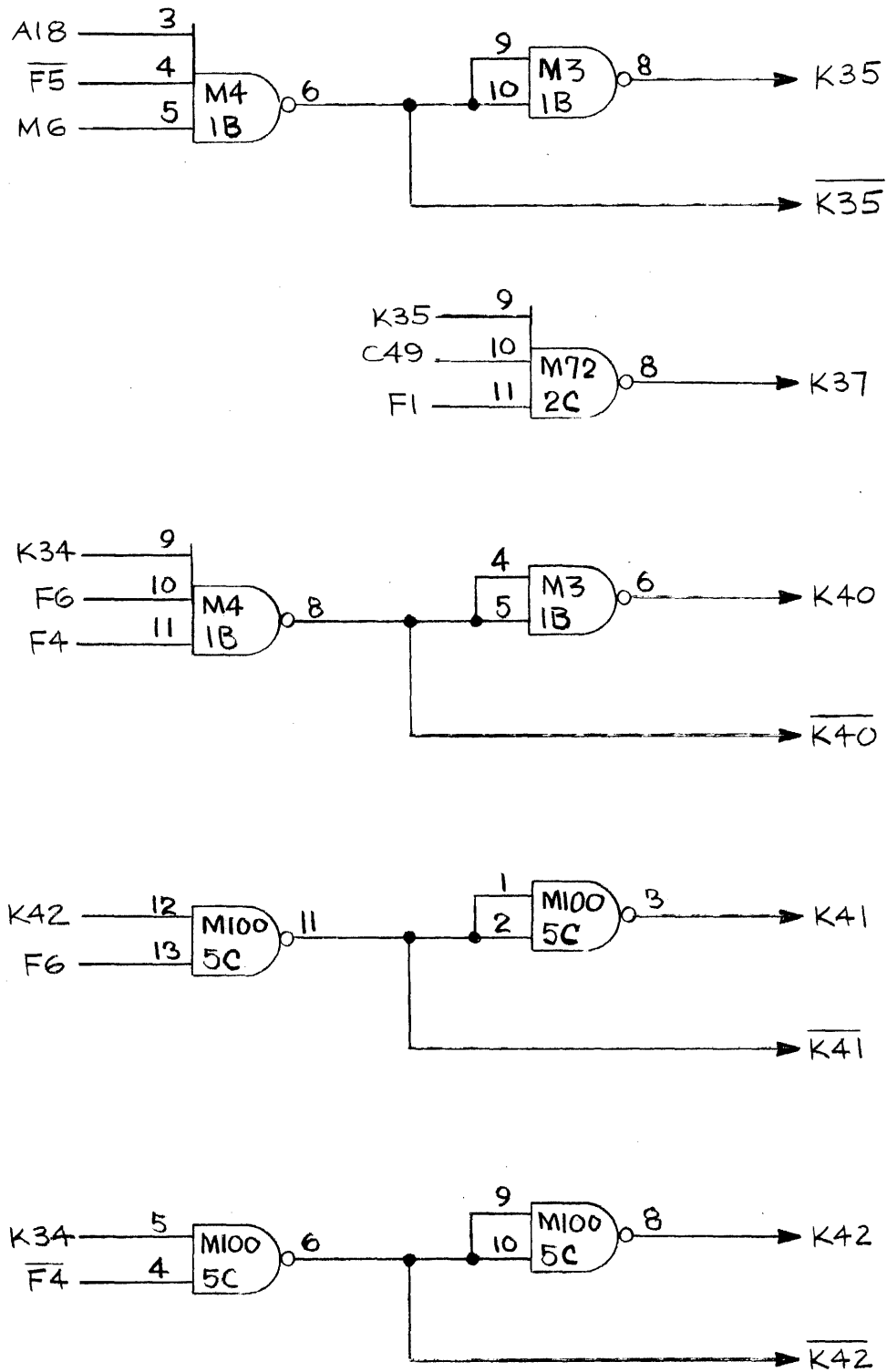
Figure 3.76 Logic Diagram.
