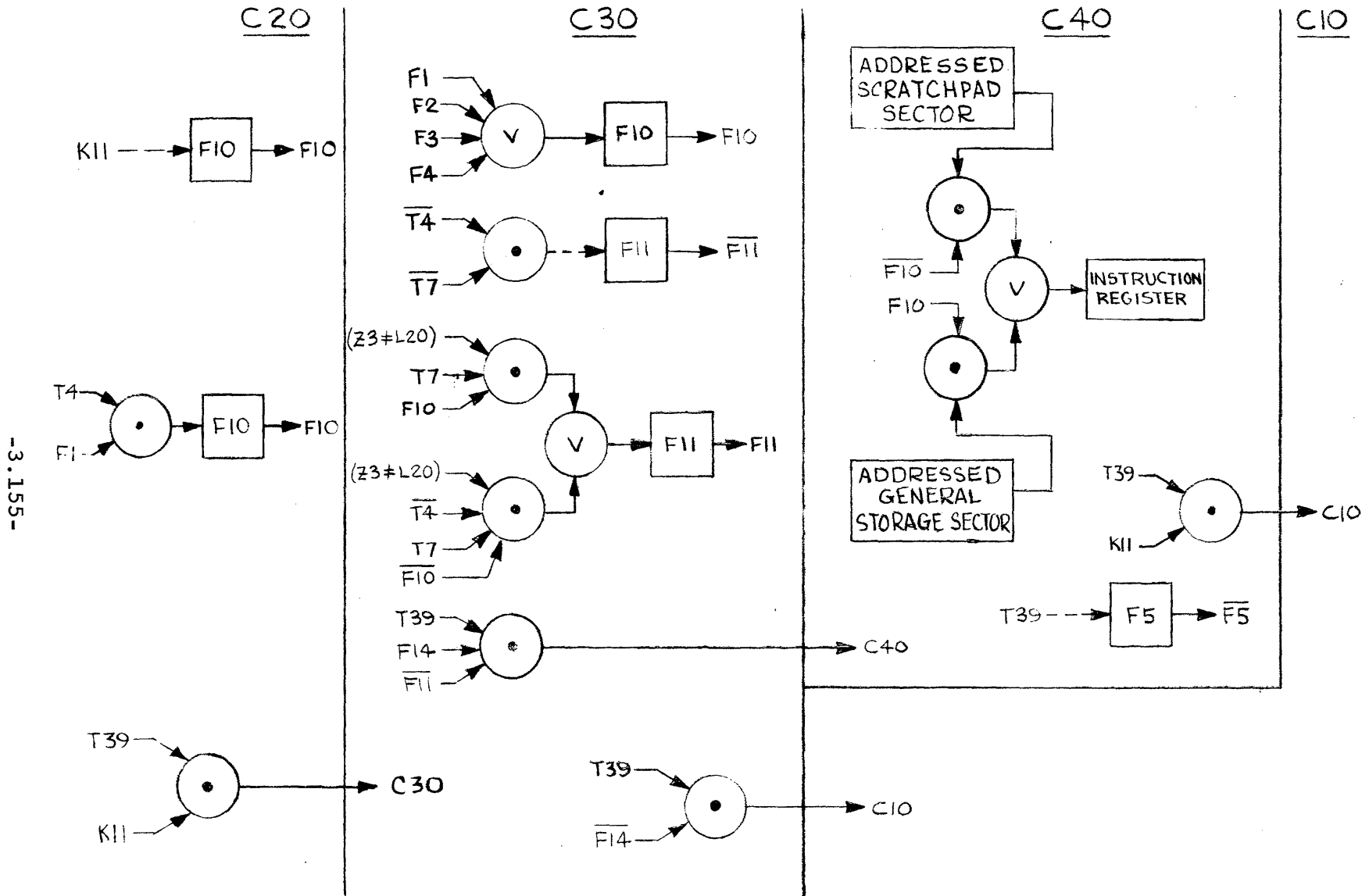
Figure 3.48.13 Jump Conditional Command, Flow Chart.
