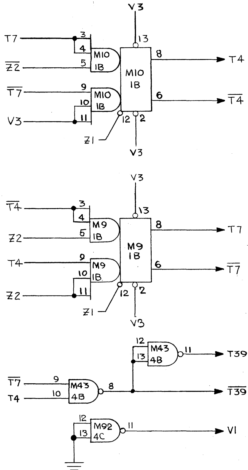
Figure 3.96 Logic Diagram.
