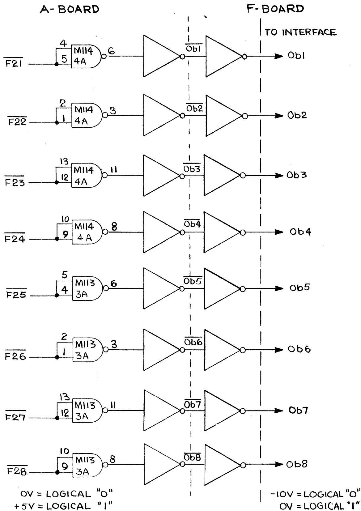
Figure 3.93 Logic Diagram.
