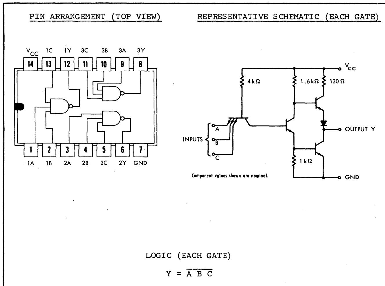
Figure 4.2 585008, Triple 3-Input NAND Gate Package.
