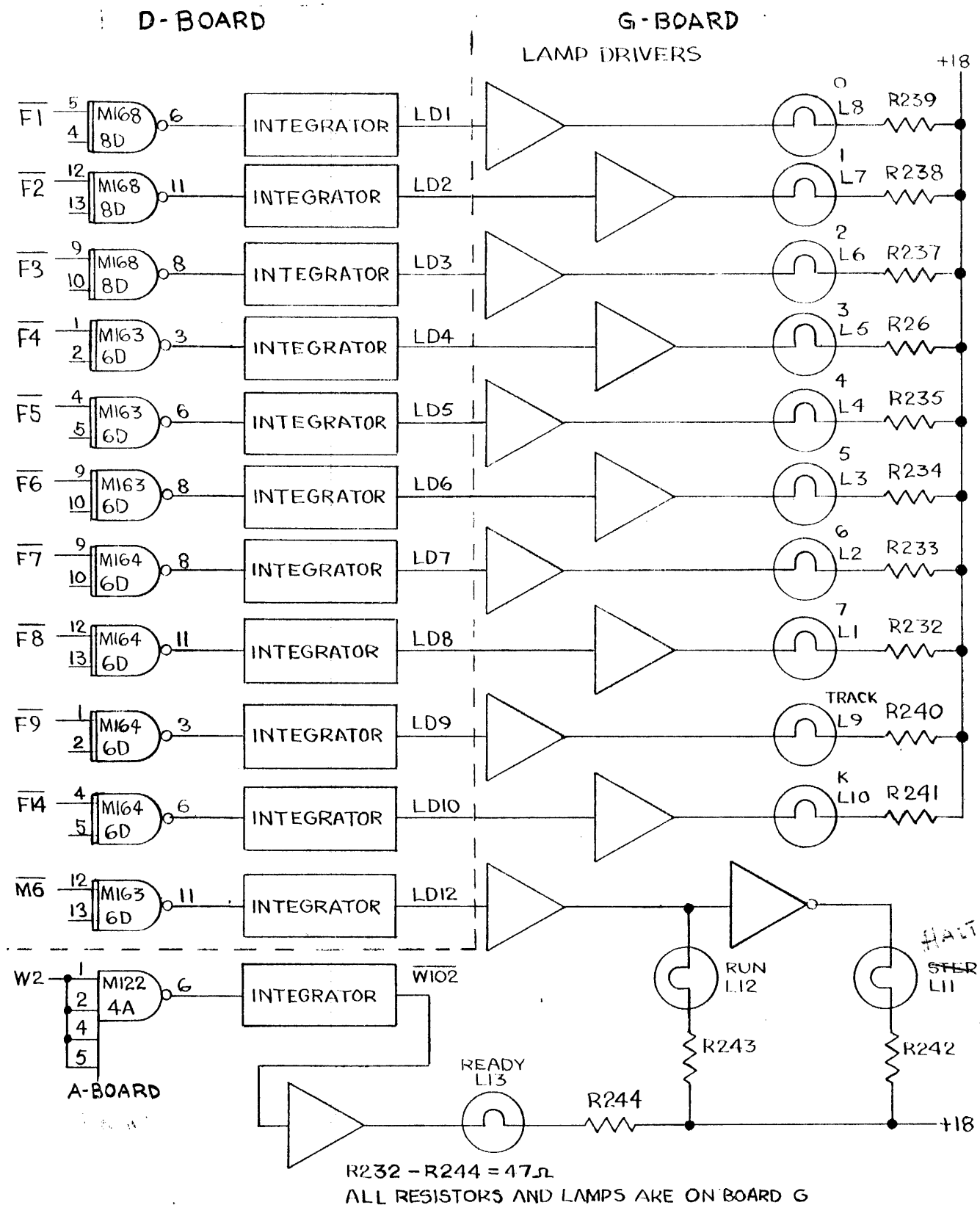
Figure 3.99 Logic Diagram.
