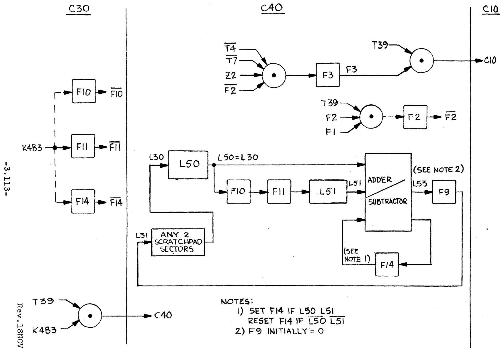
Figure 3.42 Decimal Left Double Shift on Scratchpad Command, Flow Chart.
