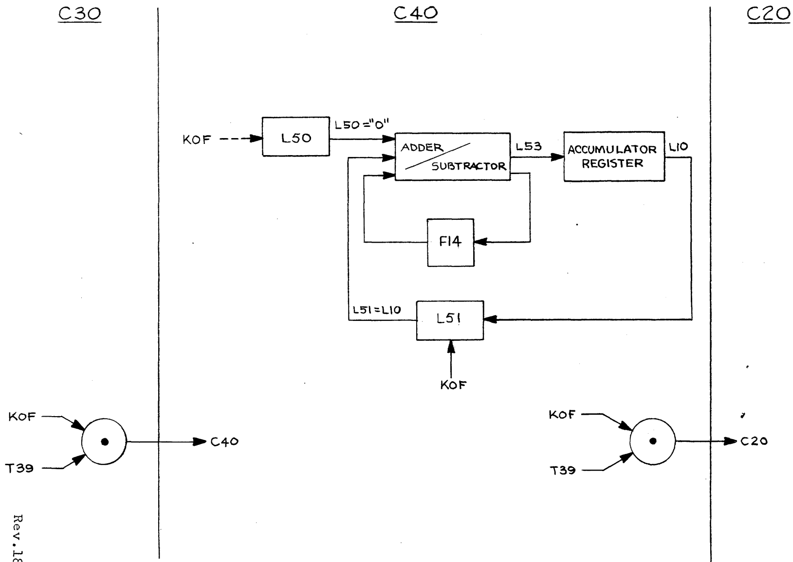
Figure 3.6 Add K Command, Flow Chart.
