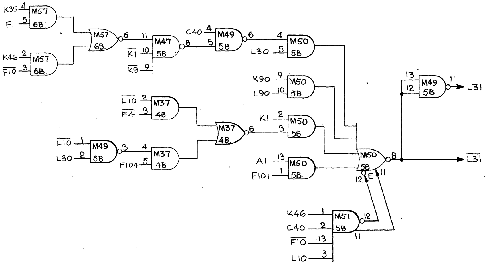
FAST ACCESS RECORD NET
