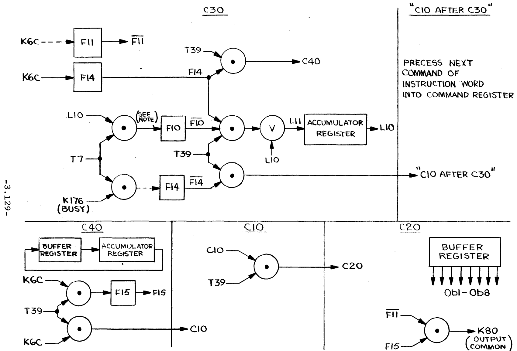
Figure 3.47 Output Accumulator with Even Parity Command, Flow Chart.
