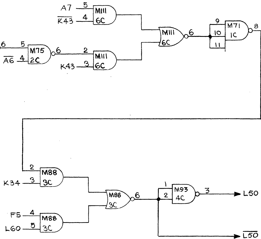
PART OF ADDER / SUBTRACTOR INPUT NET
