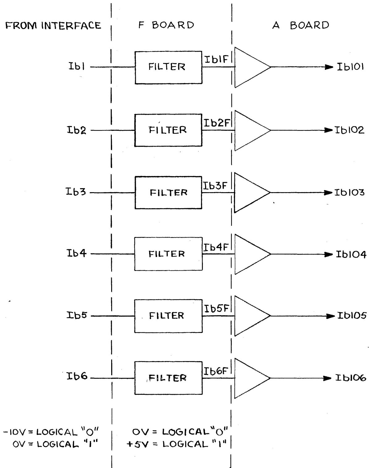
Figure 3.72 Logic Diagram.
