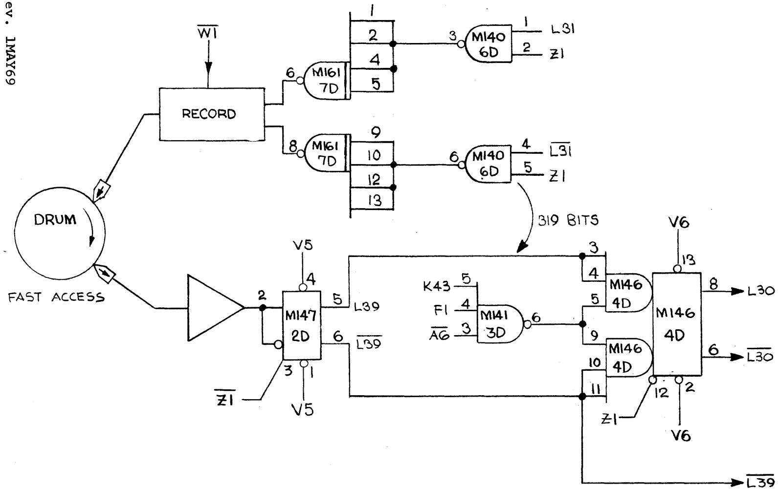
FAST ACCESS LOOP, 8 WORDS (320 BITS)
