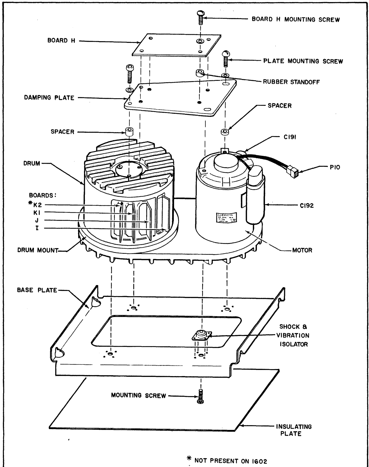
Figure 5.5 Drum Assembly.
