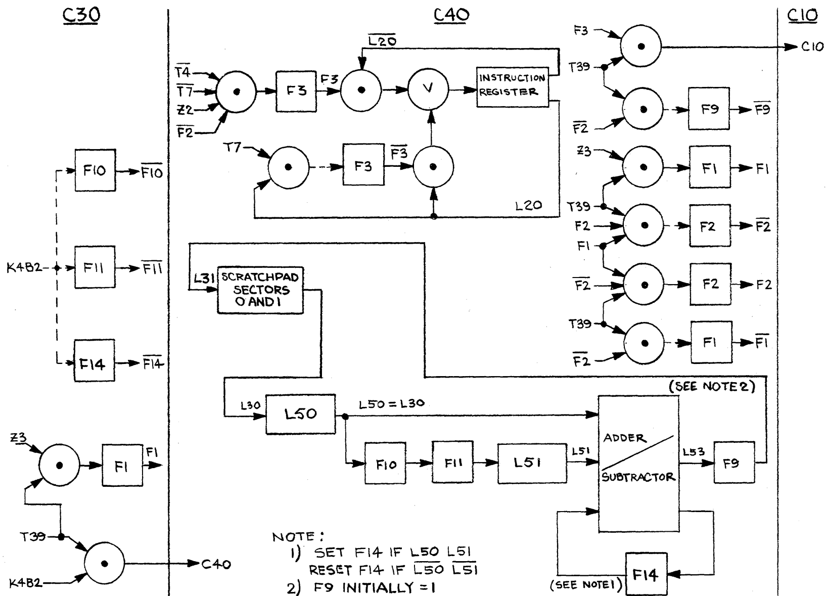
Figure 3.41 Decimal Left Double Shift, Plus Constant Command, Flow Chart.
