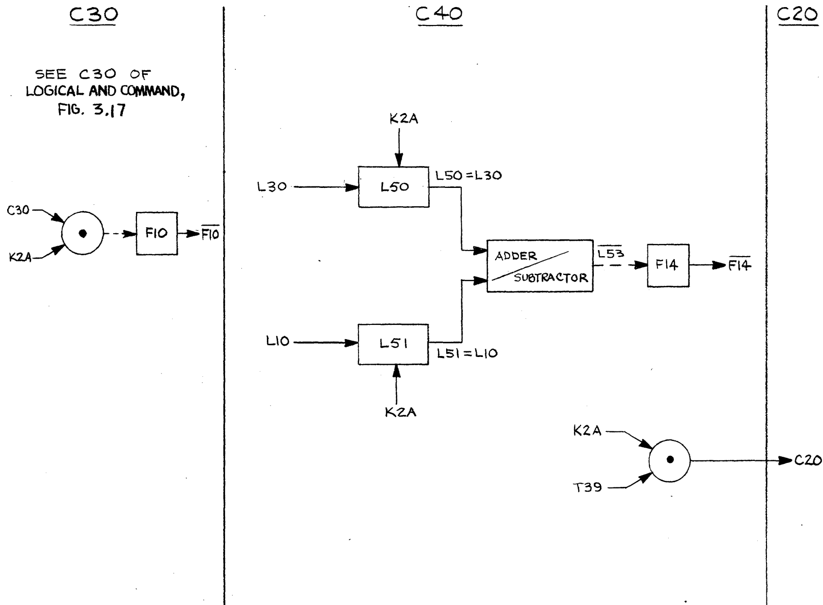
Figure 3.20 Test Equal Command, Flow Chart.
