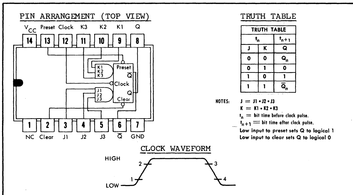
Figure 4.11 585017, JK Master-Slave Flipflop Package.
