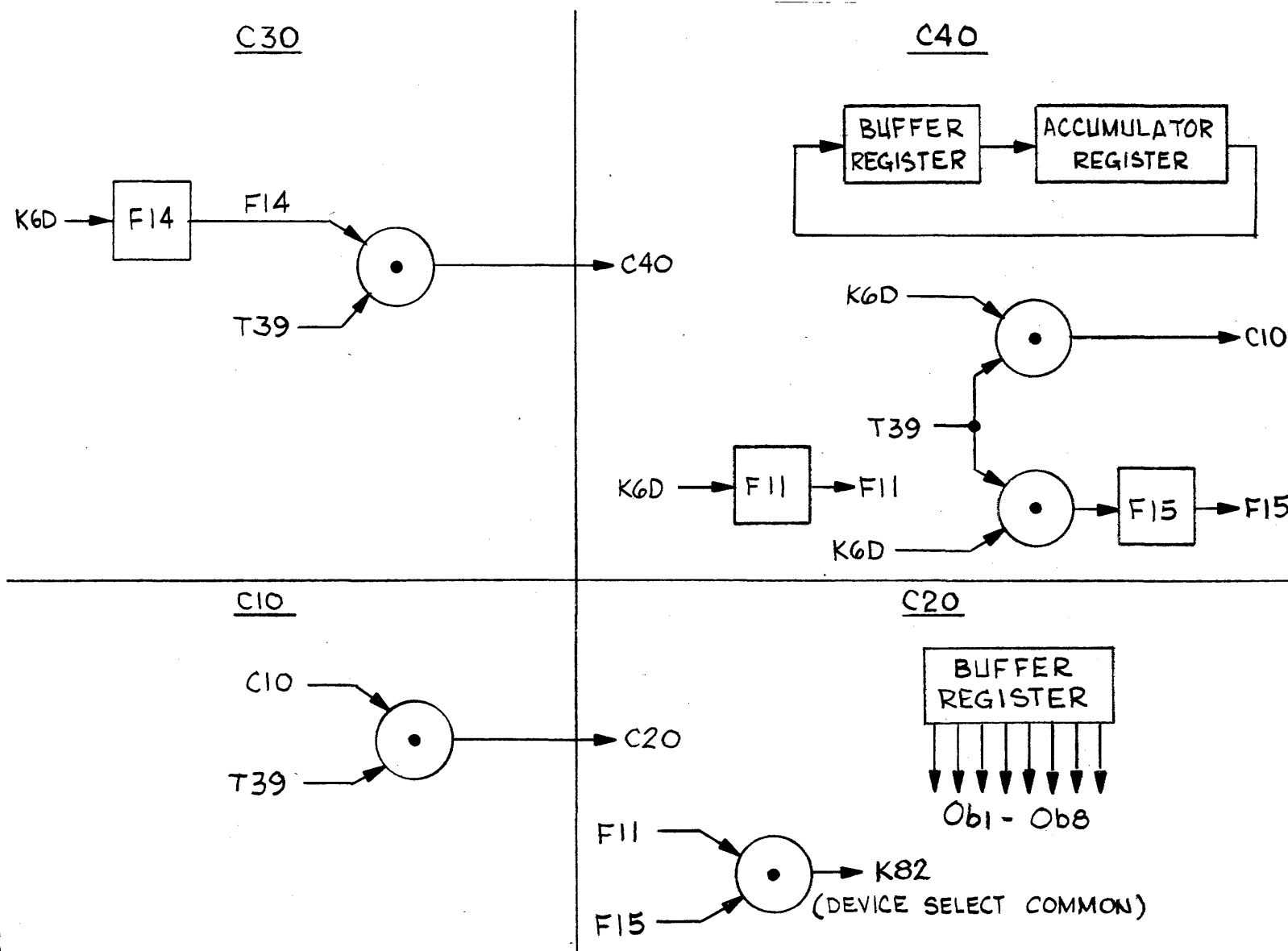
Figure 3.48.3 Accumulator Select Command, Flow Chart.
