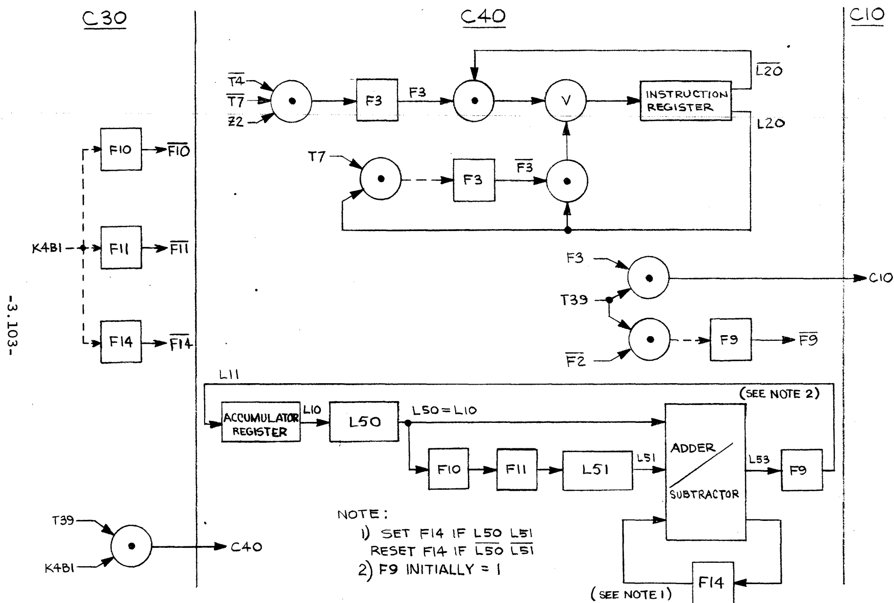
Figure 3.37 Decimal Left Single Shift, Plus Constant Command, Flow Chart.
