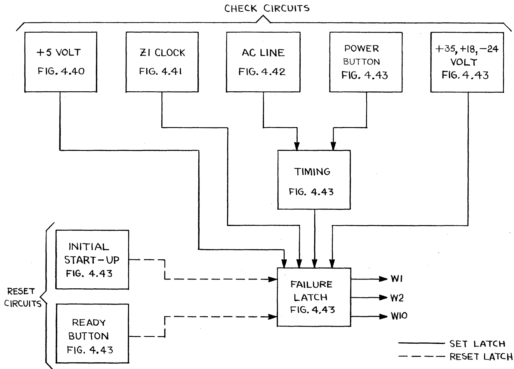
Figure 4.39 Block Diagram, Warm-Up Circuit.
