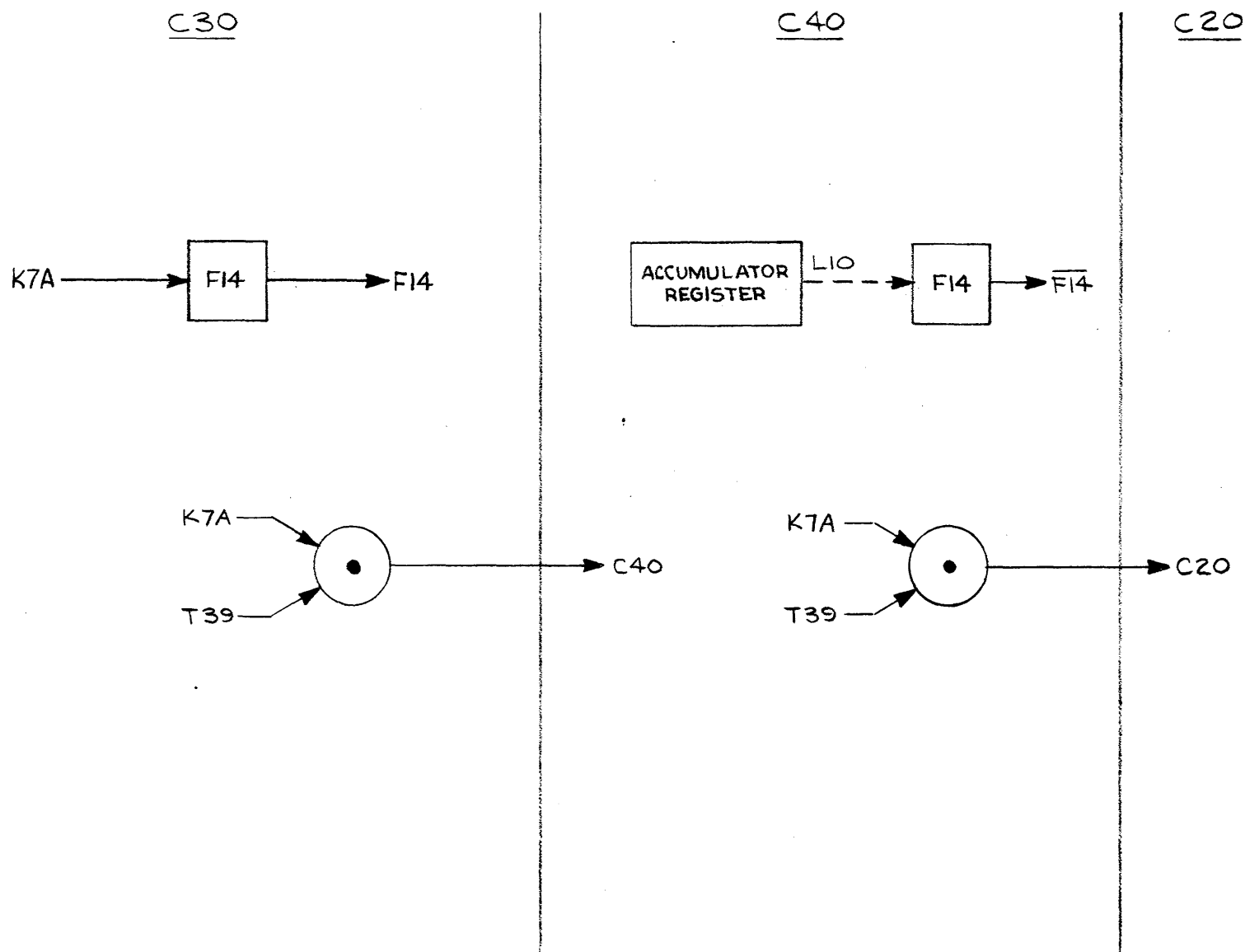
Figure 3.13 Test for Zero Command, Flow Chart.
