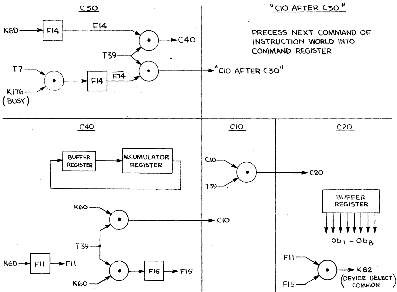
Figure 3.48.2 Accumulator Select on Test Command, Flow Chart.
