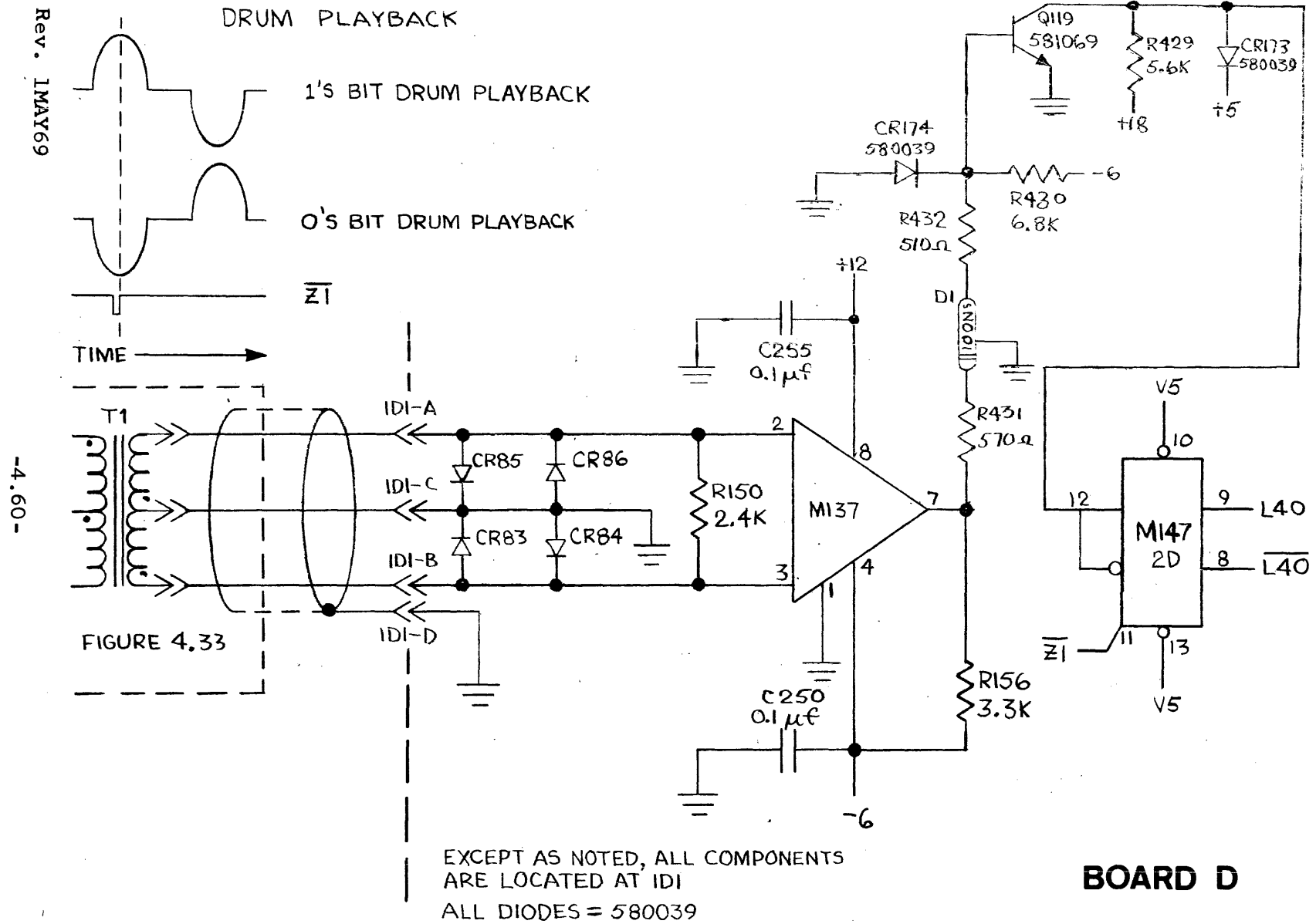
Figure 4.35 Playback Circuit, General Storage.
