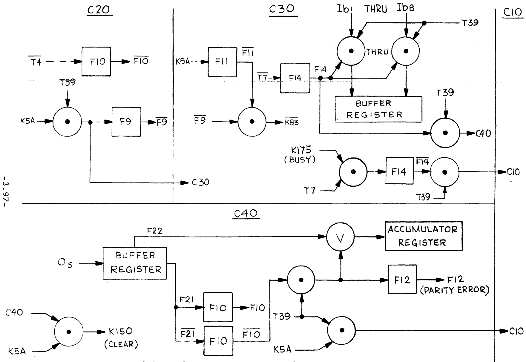
Figure 3.34 Clear, Input, Check Odd Parity Into A Command, Flow Chart.
