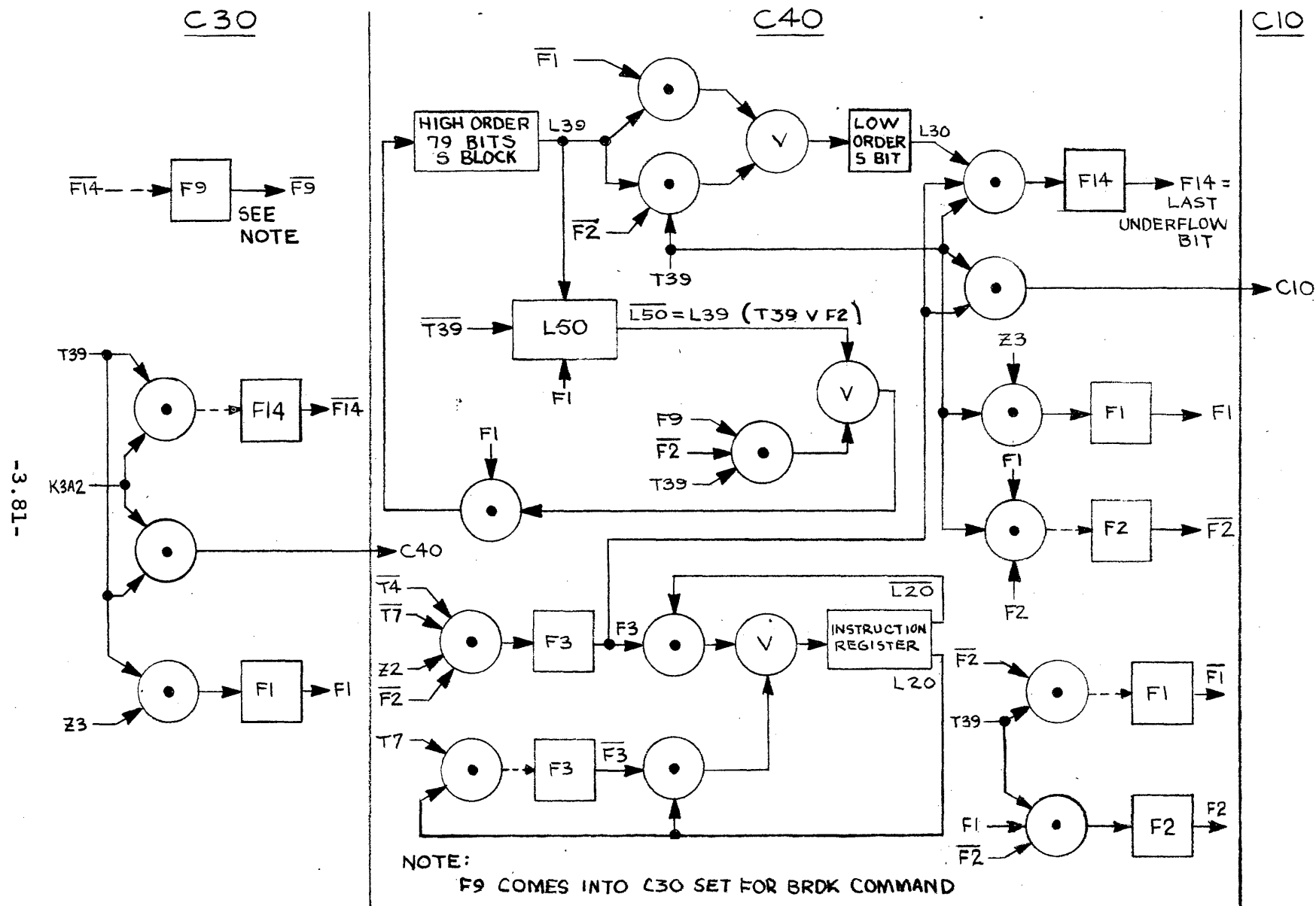
Figure 3.28 Binary Right Double Shift Command and Binary Right Double Shift Including K Command, Flow Chart.
