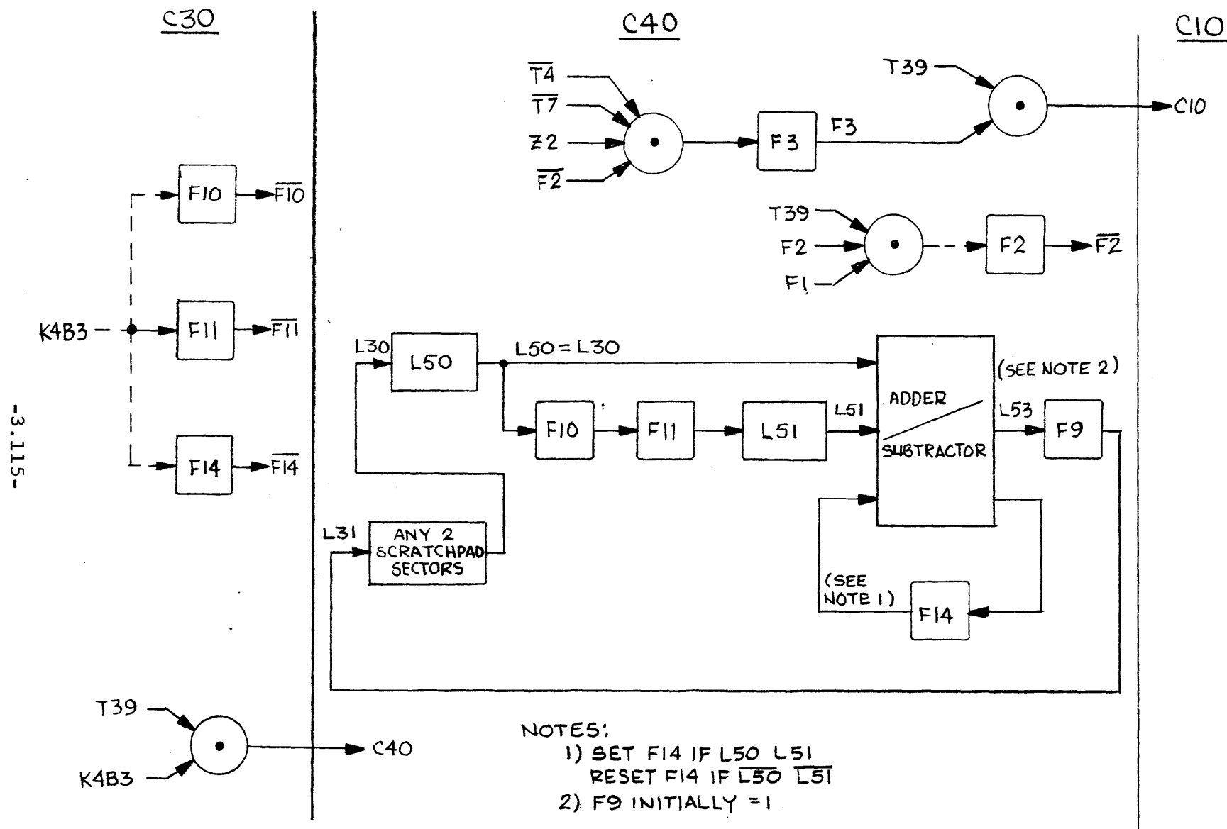
Figure 3.43 Decimal Left Double Shift on Scratchpad, Plus Constant Command, Flow Chart.
