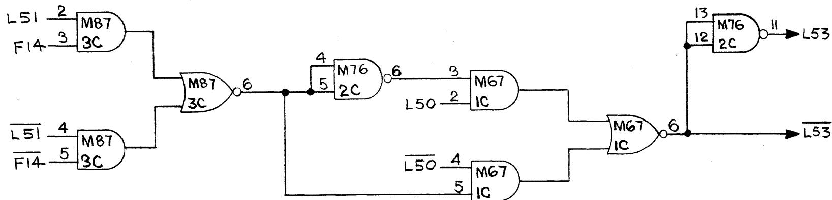
ADDER/SUBTRACTOR
