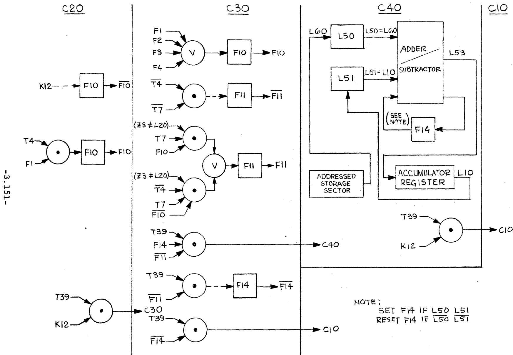
Figure 3.48.11 Add Conditional Command, Flow Chart.
