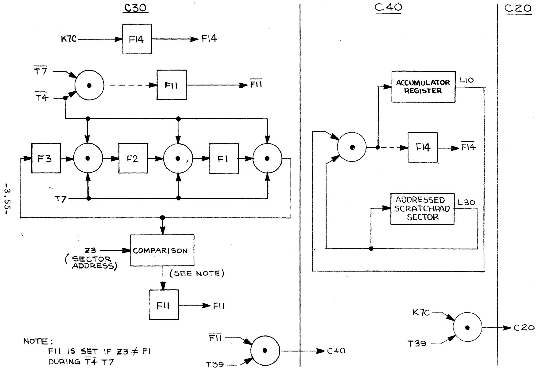
Figure 3.17 Logical And Command, Flow Chart.
