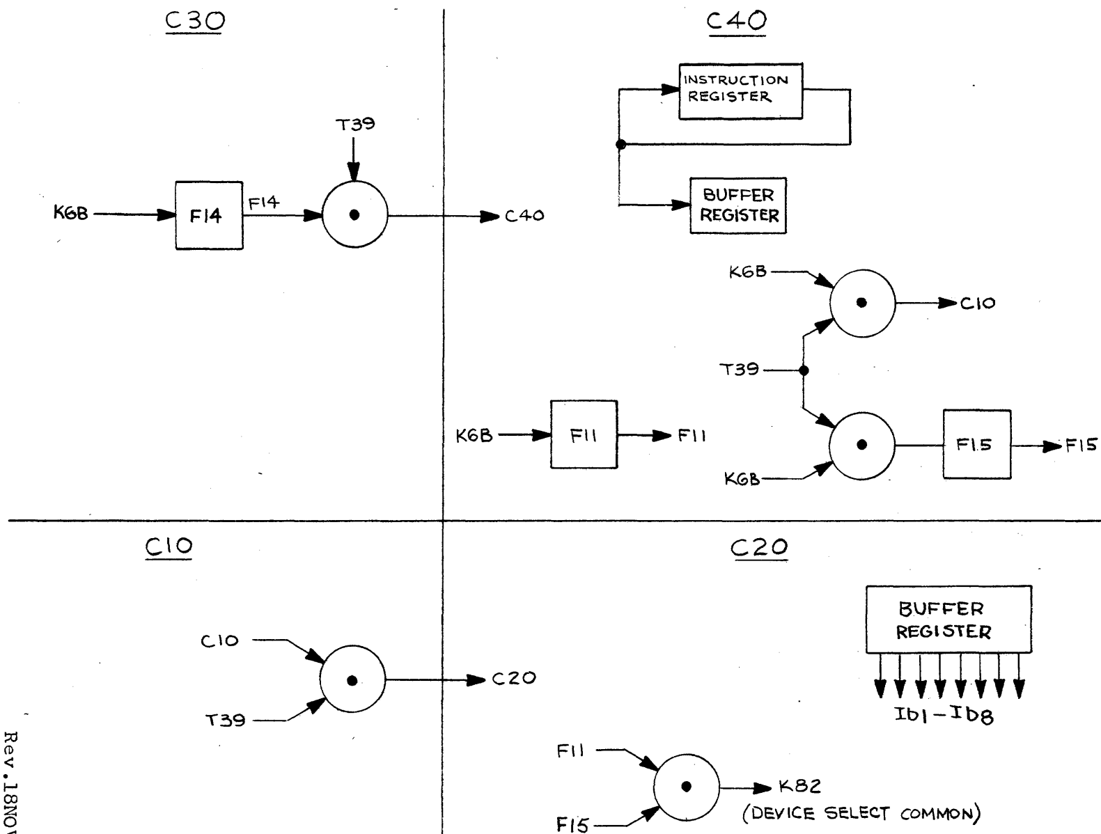
Figure 3.48.6 Immediate Select Command, Flow Chart.
