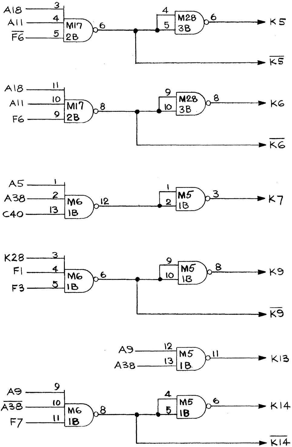
Figure 3.74 Logic Diagram.
