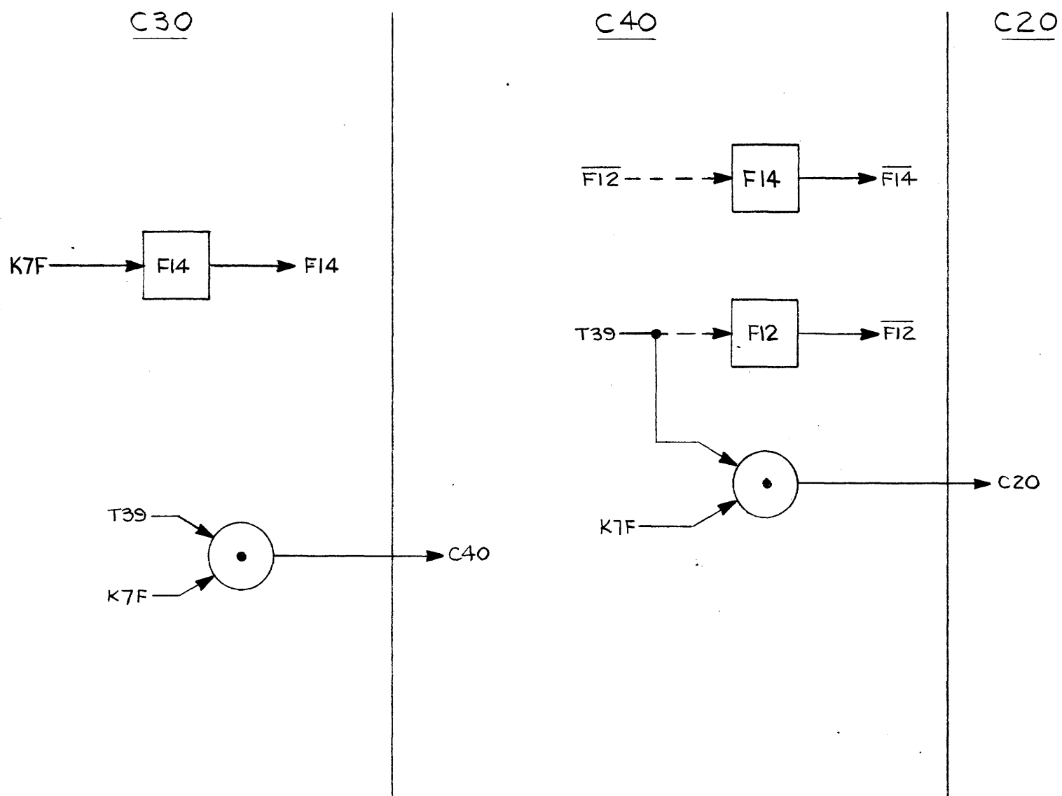
Figure 3.16 Test Parity Failure Command, Flow Chart.
