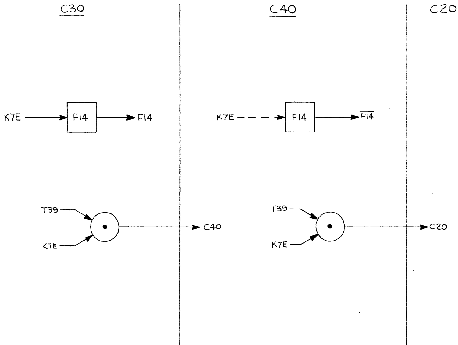
Figure 3.15 Reset K to 0 Command, Flow Chart.
