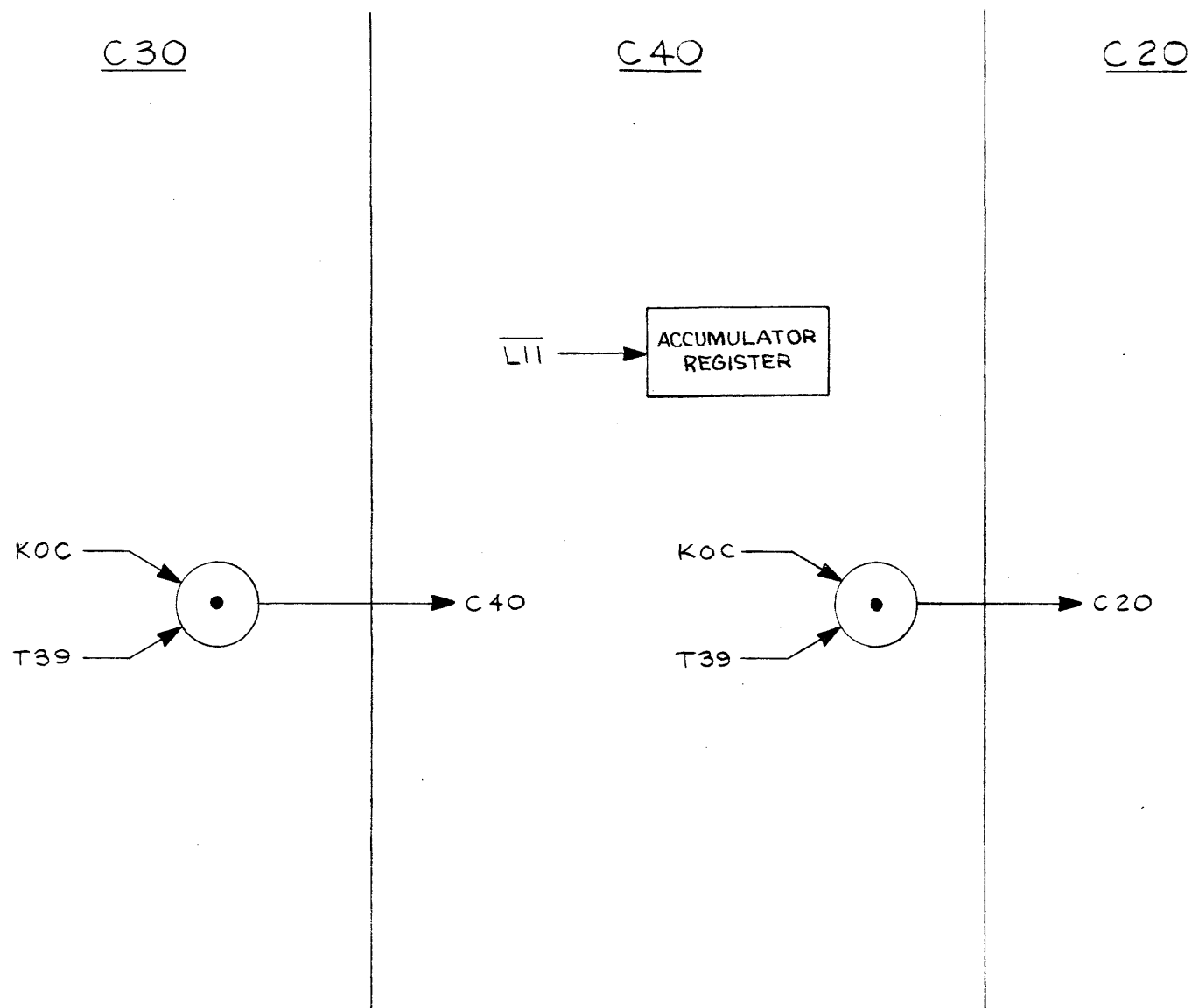
Figure 3.7 Clear A Command, Flow Chart.
