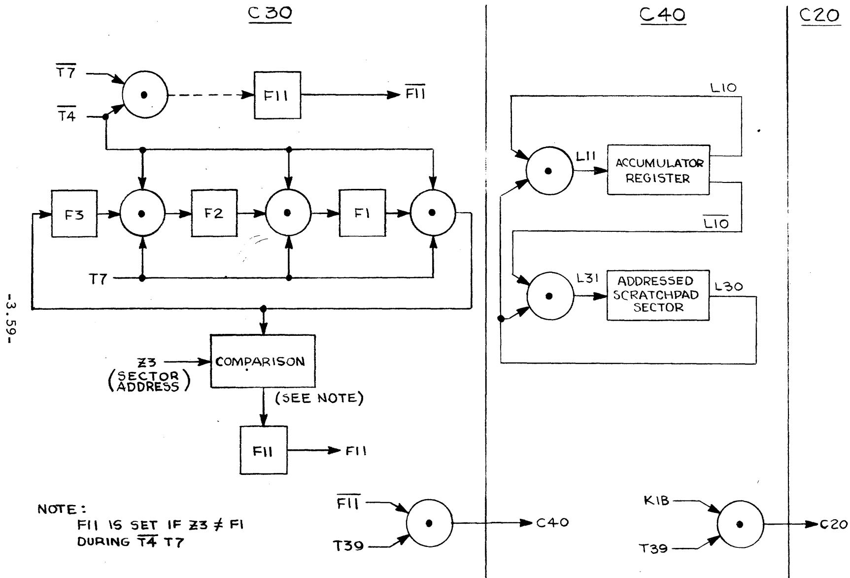
Figure 3.19 Extract Command, Flow Chart.
