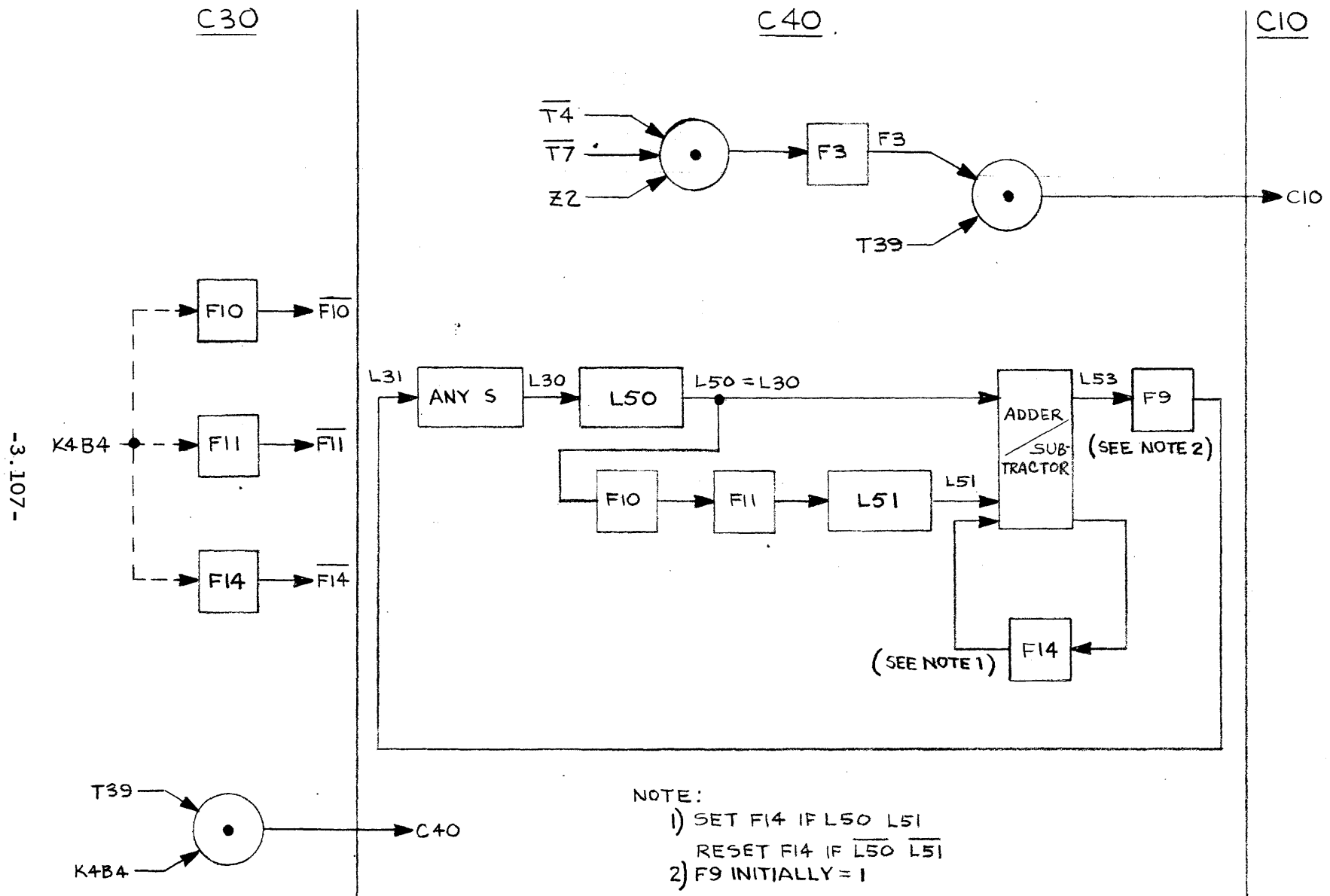
Figure 3.39 Decimal Left Single Shift on Scratchpad, Plus Constant Command, Flow Chart.
