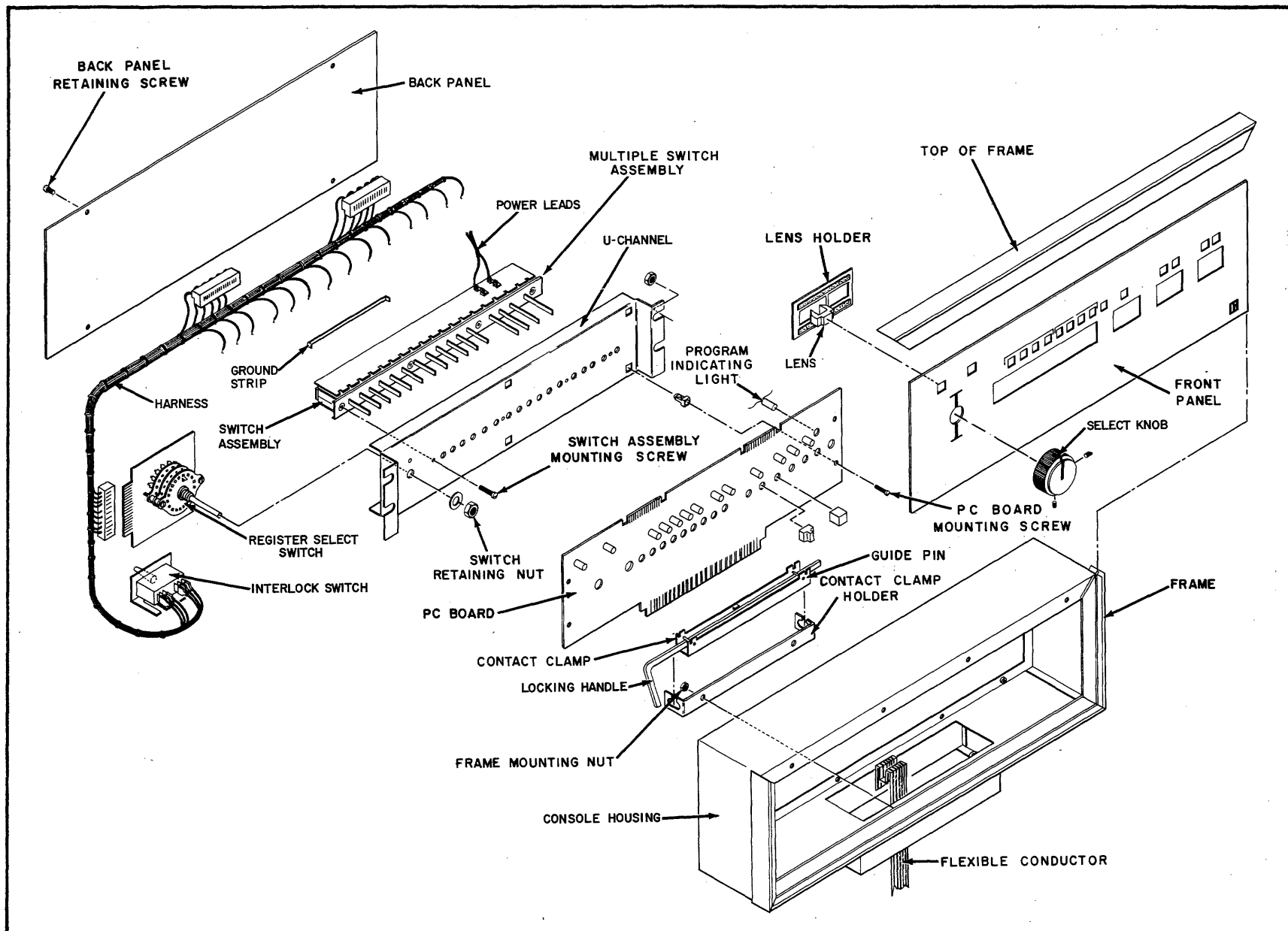
Figure 5.4 Operator Console.
