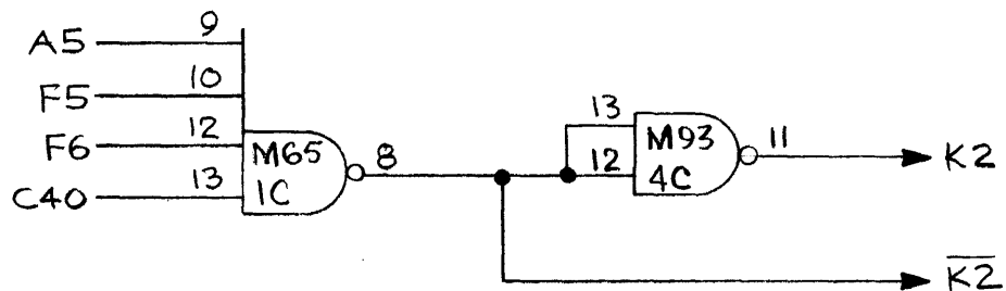
Figure 3.73 Logic Diagram.
