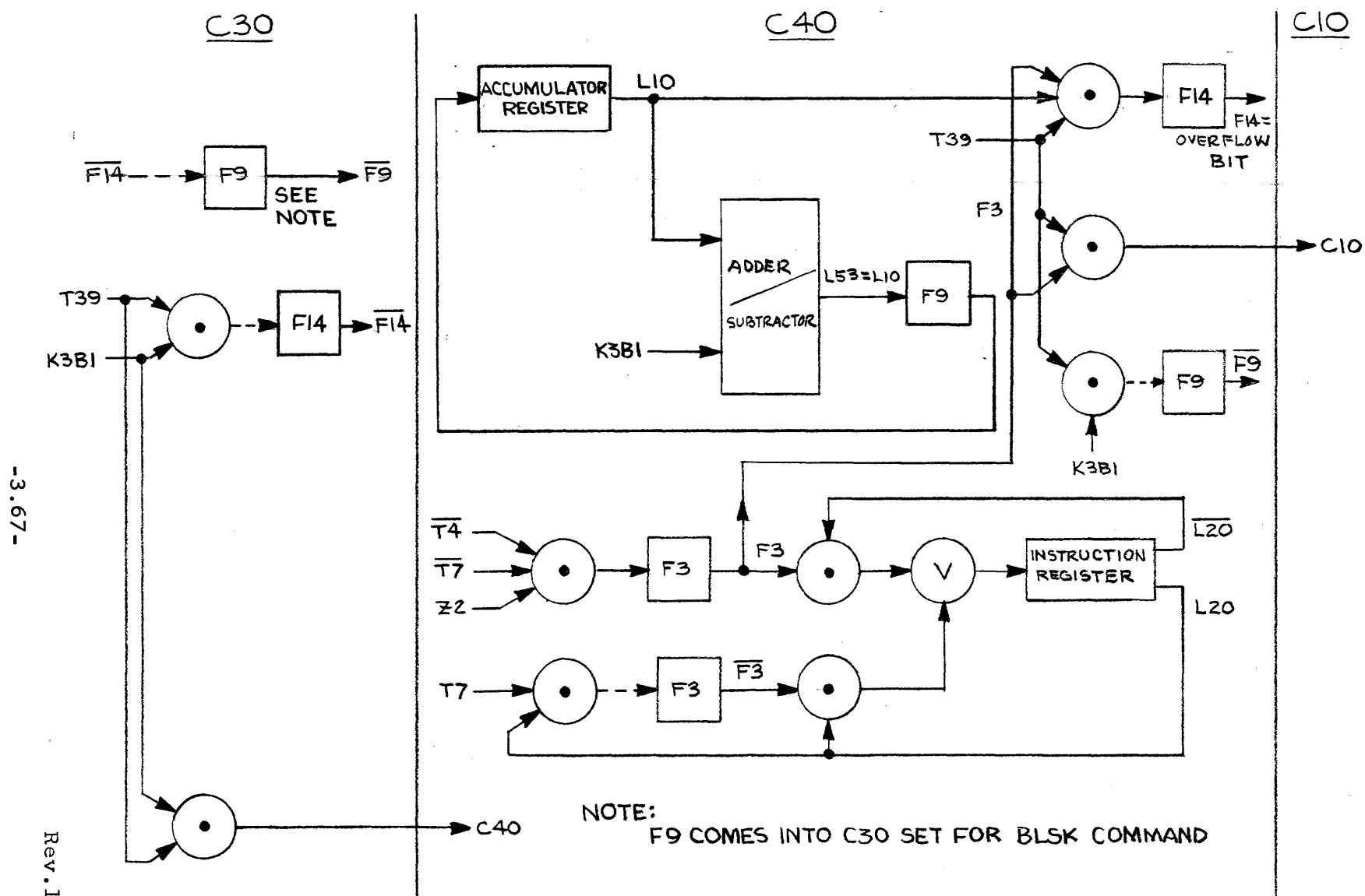
Figure 3.22 Binary Left Single Shift Command and Binary Left Single Shift Including K Command, Flow Chart.
