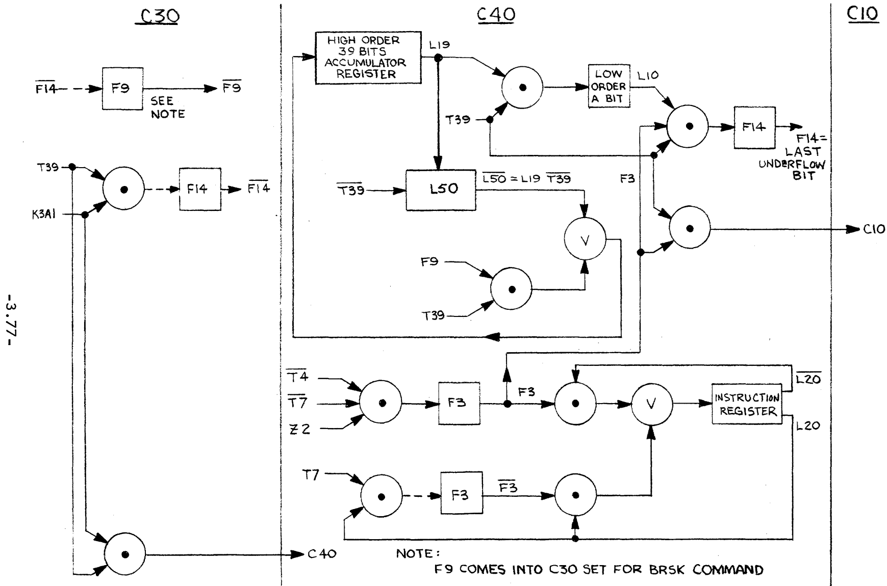
Figure 3.26 Binary Right Single Shift Command and Binary Right Single Shift Including K Command, Flow Chart.
