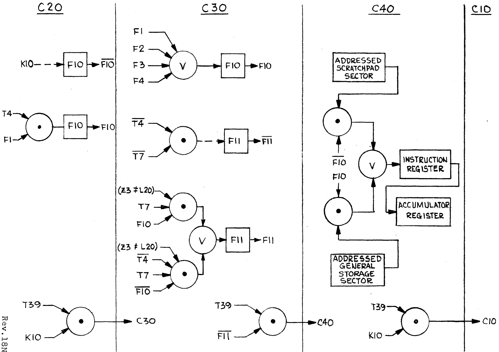
Figure 3.48.10 Jump Mark Command, Flow Chart.
