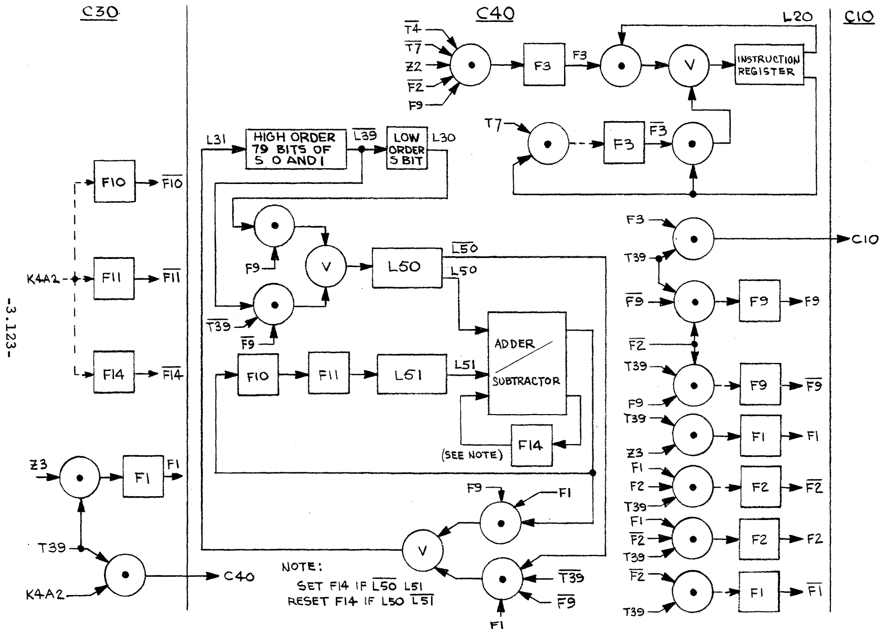
Figure 3.45 Decimal Right Double Shift Command, Flow Chart
