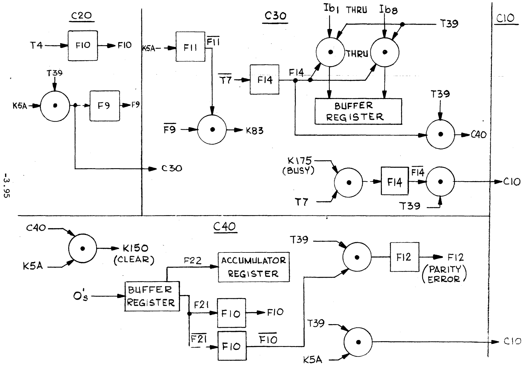
Figure 3.33 Clear, Input, Check Even Parity Command, Flow Chart.
