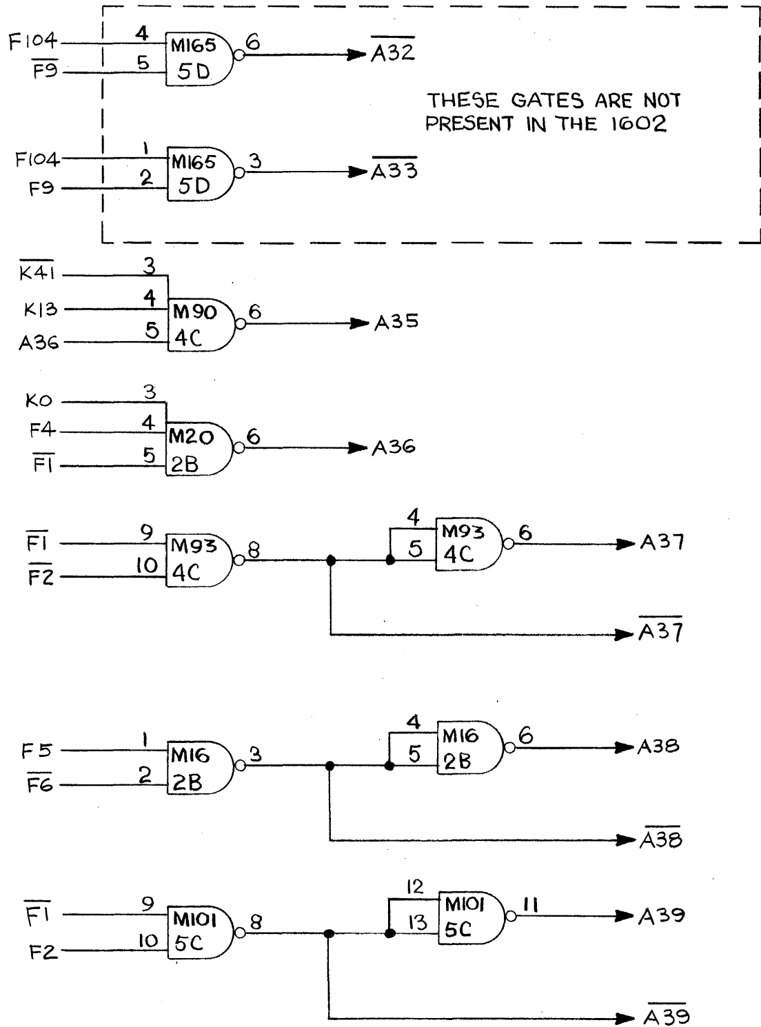
Figure 3.53 Logic Diagram.
