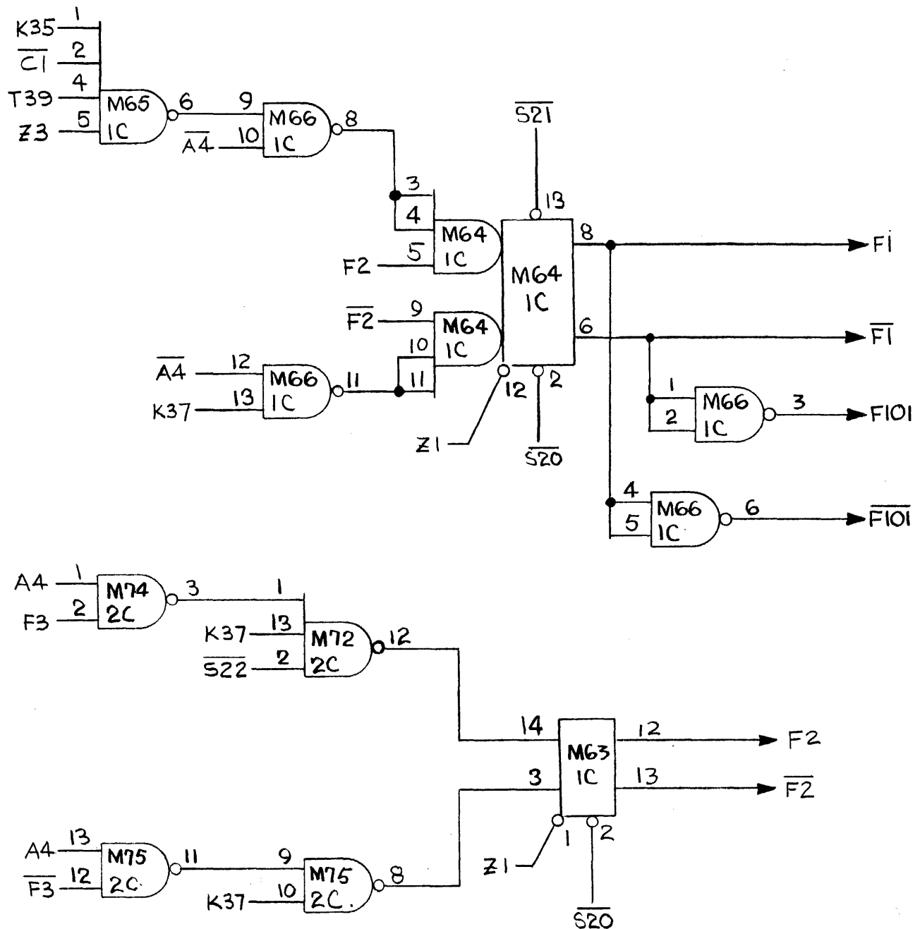
PART OF COMMAND REGISTER
