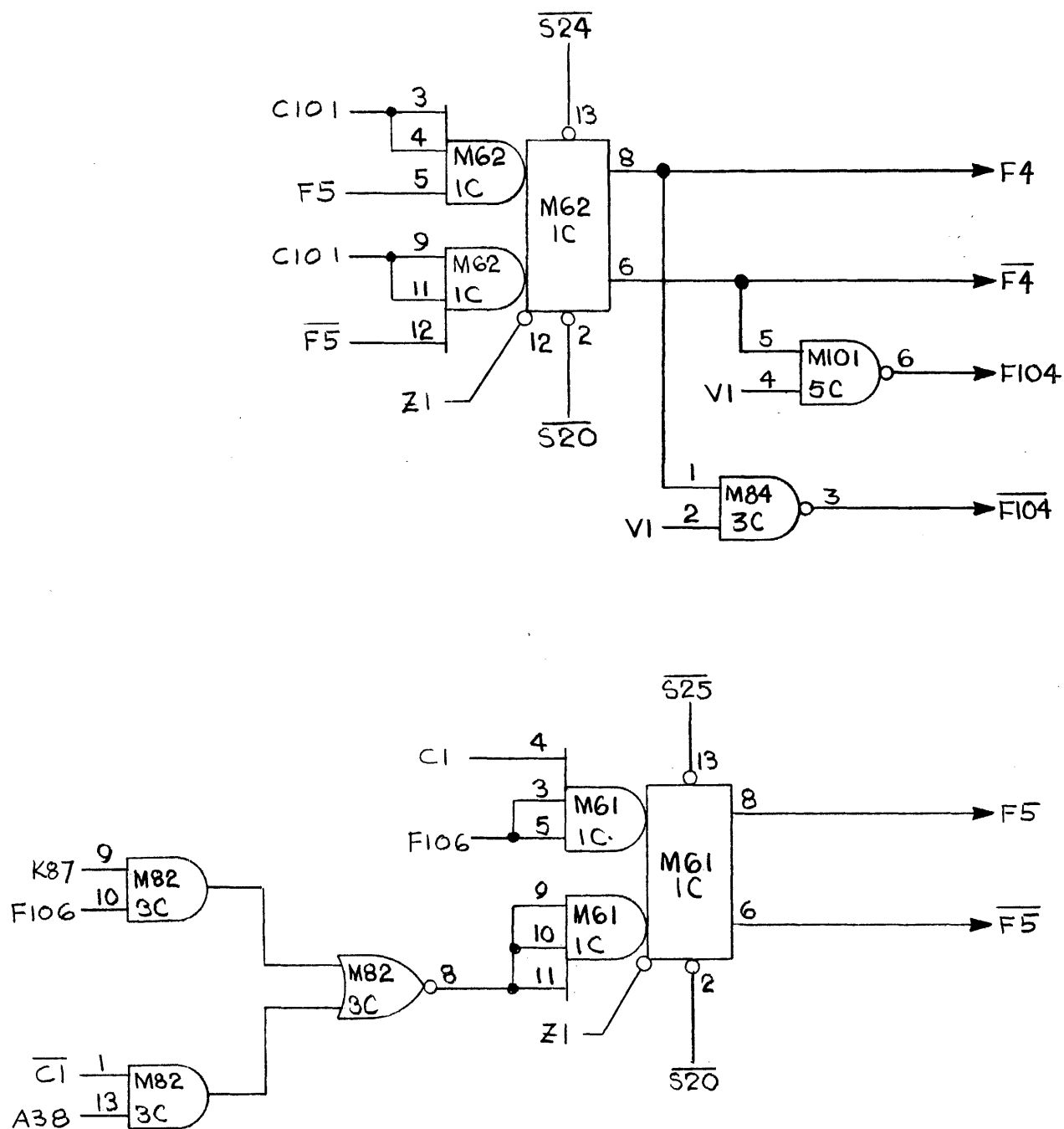
PART OF COMMAND REGISTER
