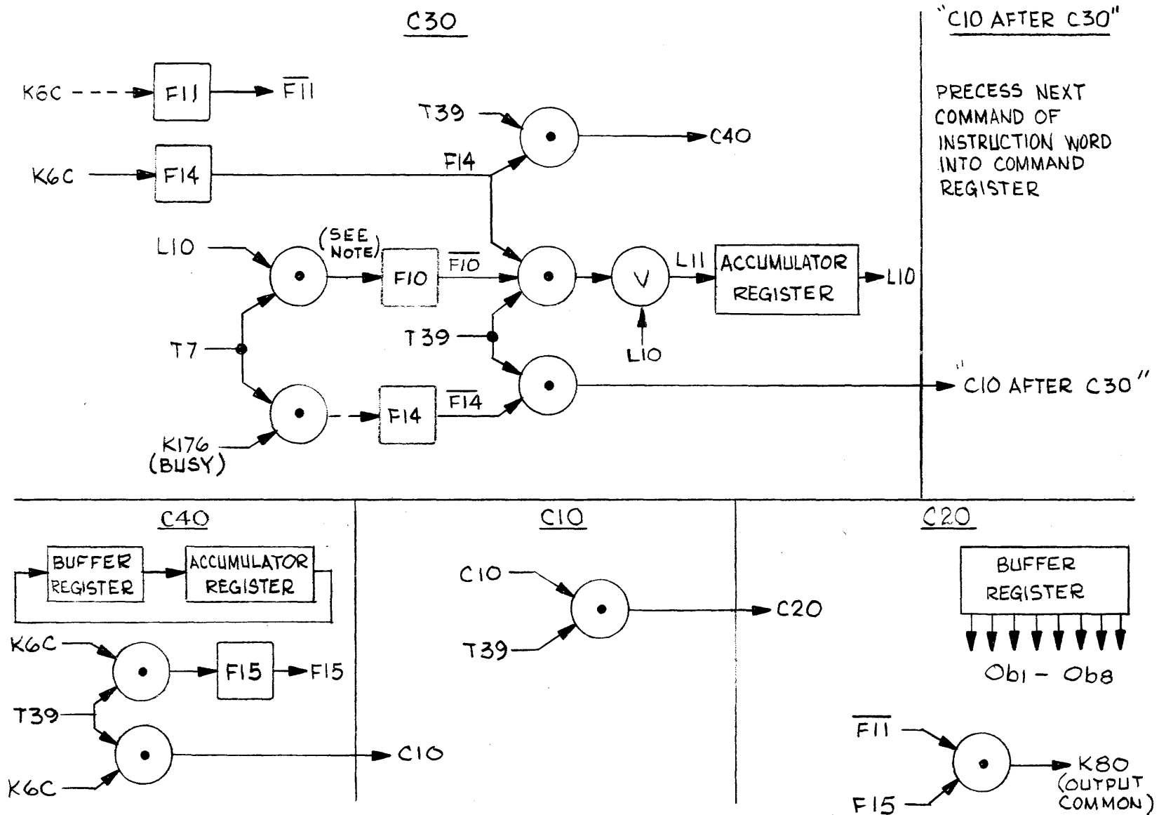
Figure 3.46 Output Accumulator with Odd Parity Command, Flow Chart.
