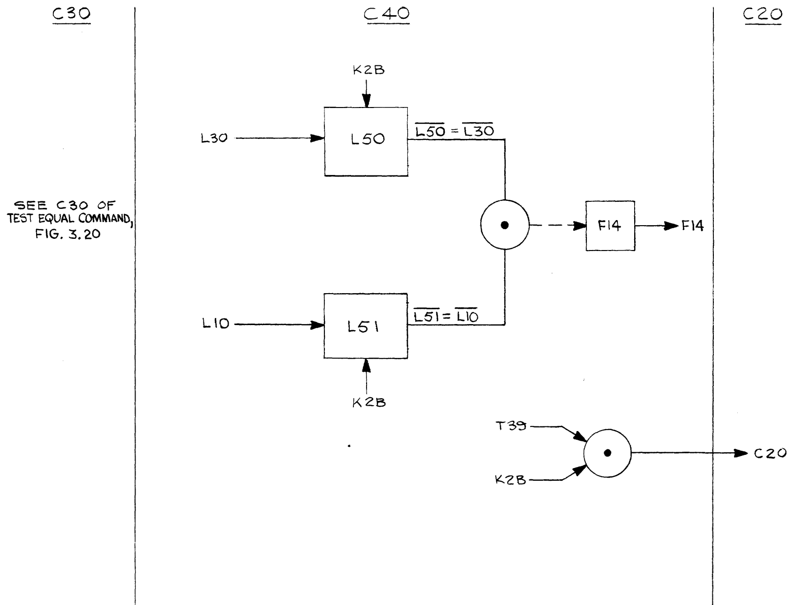
Figure 3.21 Test Equal or Greater Command, Flow Chart.
