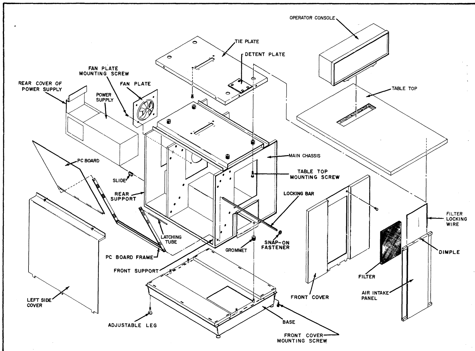
Figure 5.1 Housing.
