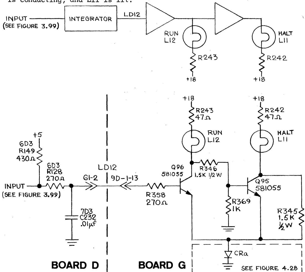
Figure 4.29 Lamp Driver Circuit, HALT and RUN.
