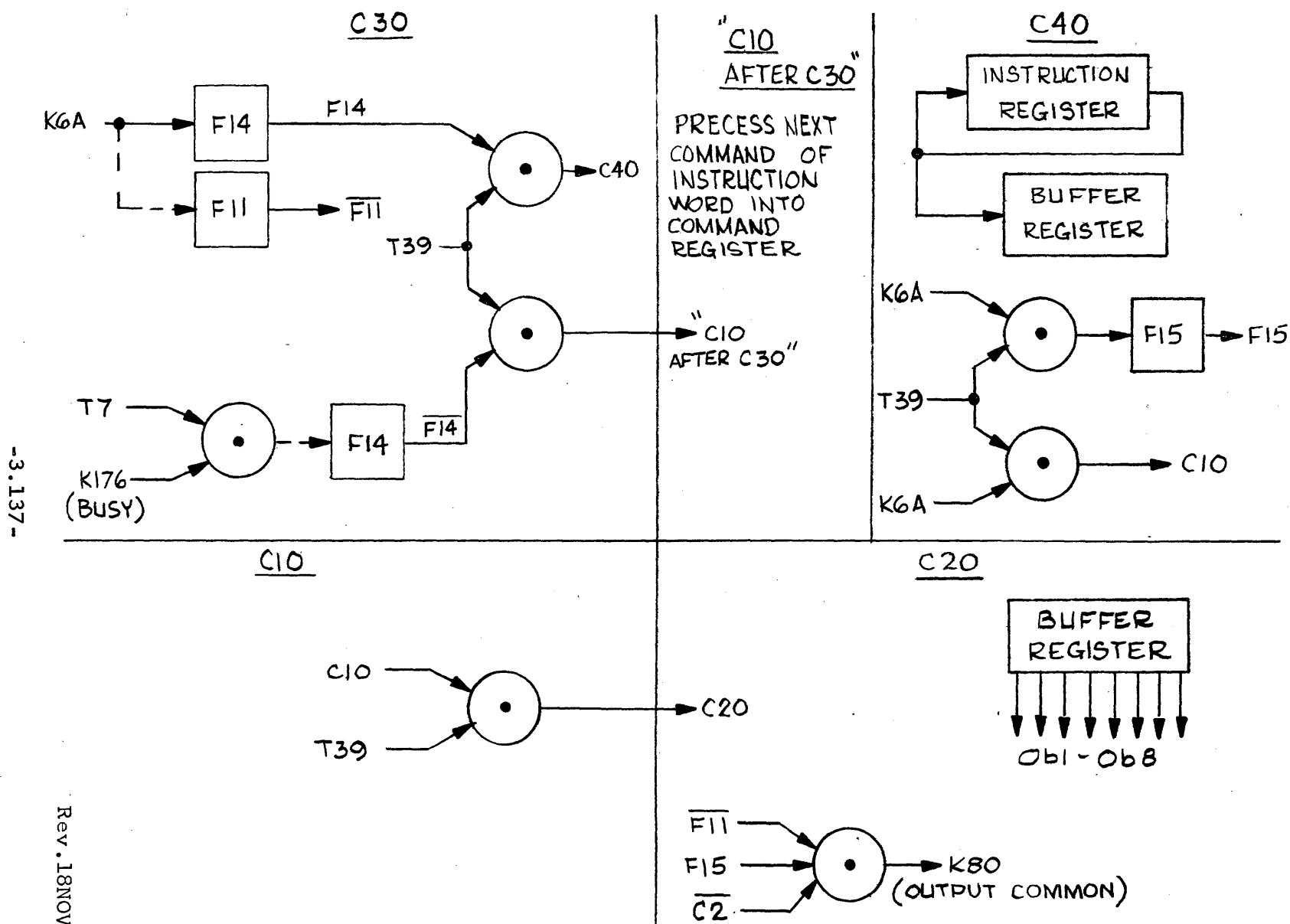
Figure 3.48.4 Output Immediate Command, Flow Chart.
