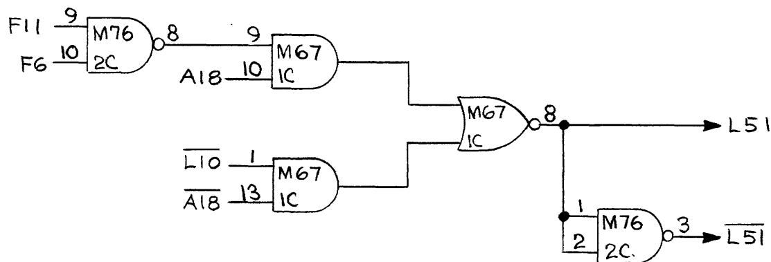
PART OF ADDER/SUBTRACTOR INPUT NET
