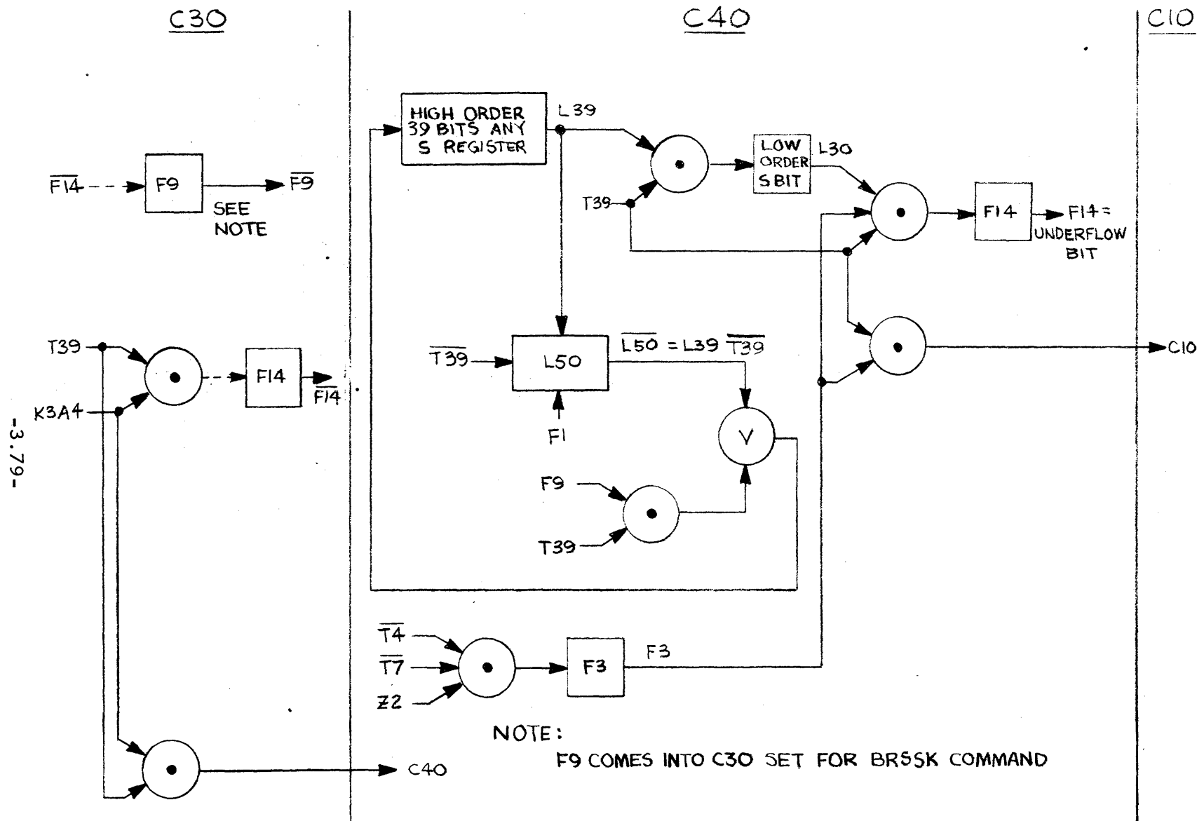
Figure 3.27 Binary Right Shift on Scratchpad Command and Binary Right Shift on Scratchpad Including K Command, Flow Chart.
