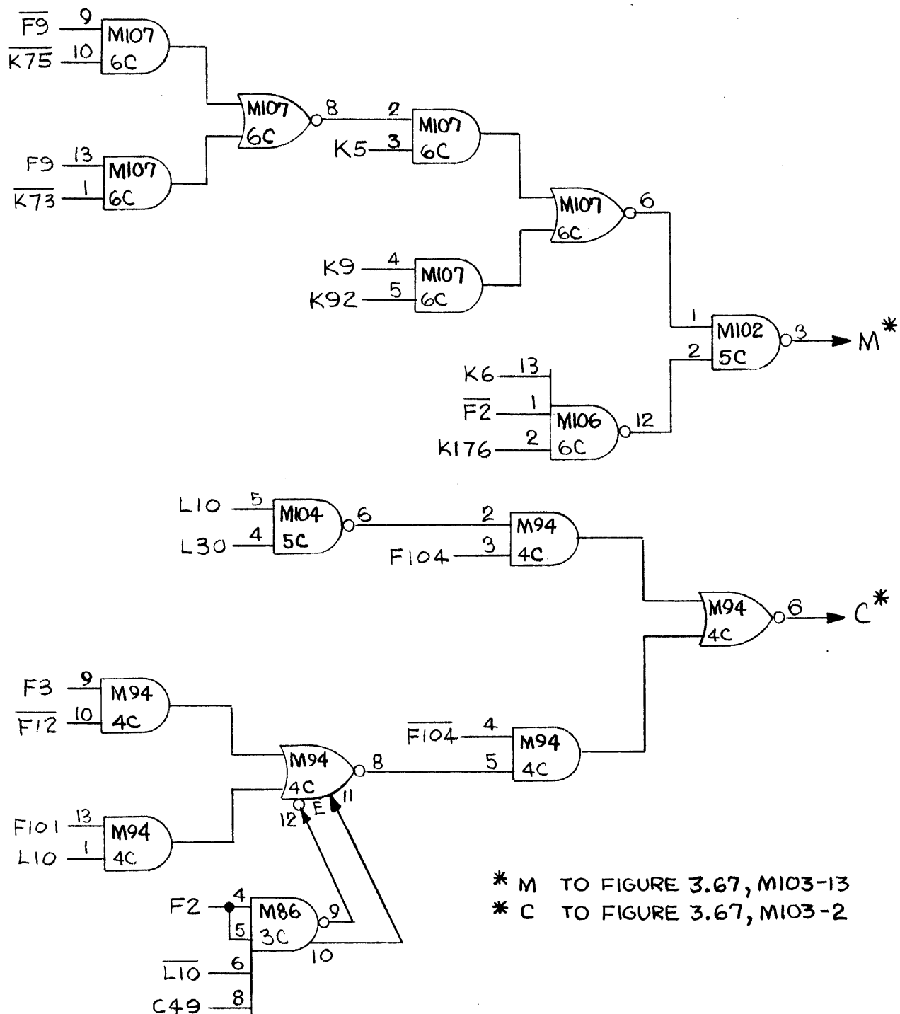
PART OF F14 RESET NET
