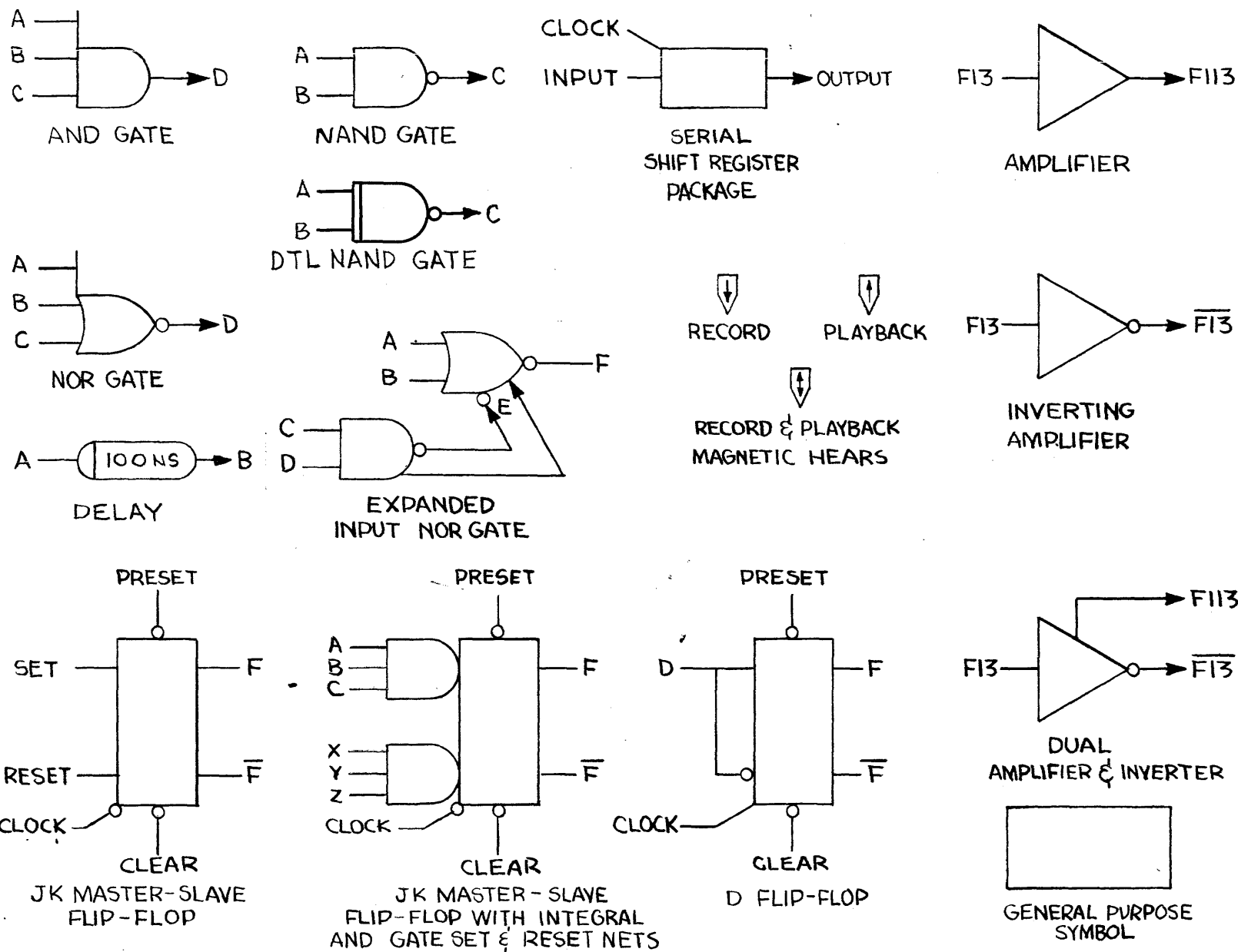
Figure 1.4 Logic Diagram Symbols.
