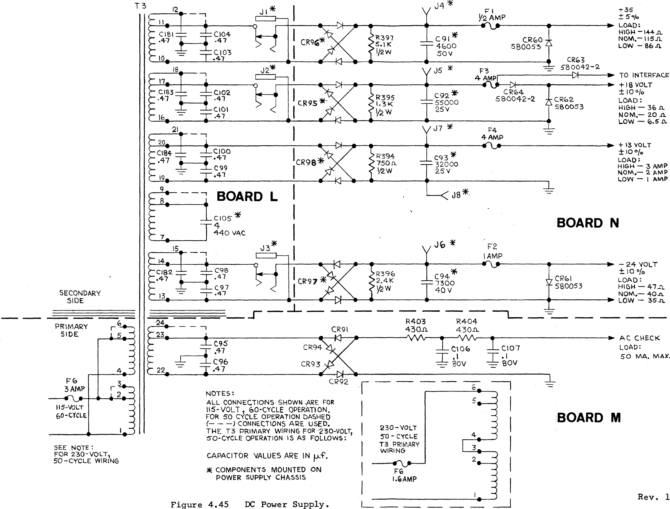
Figure 4.45 DC Power Supply.
