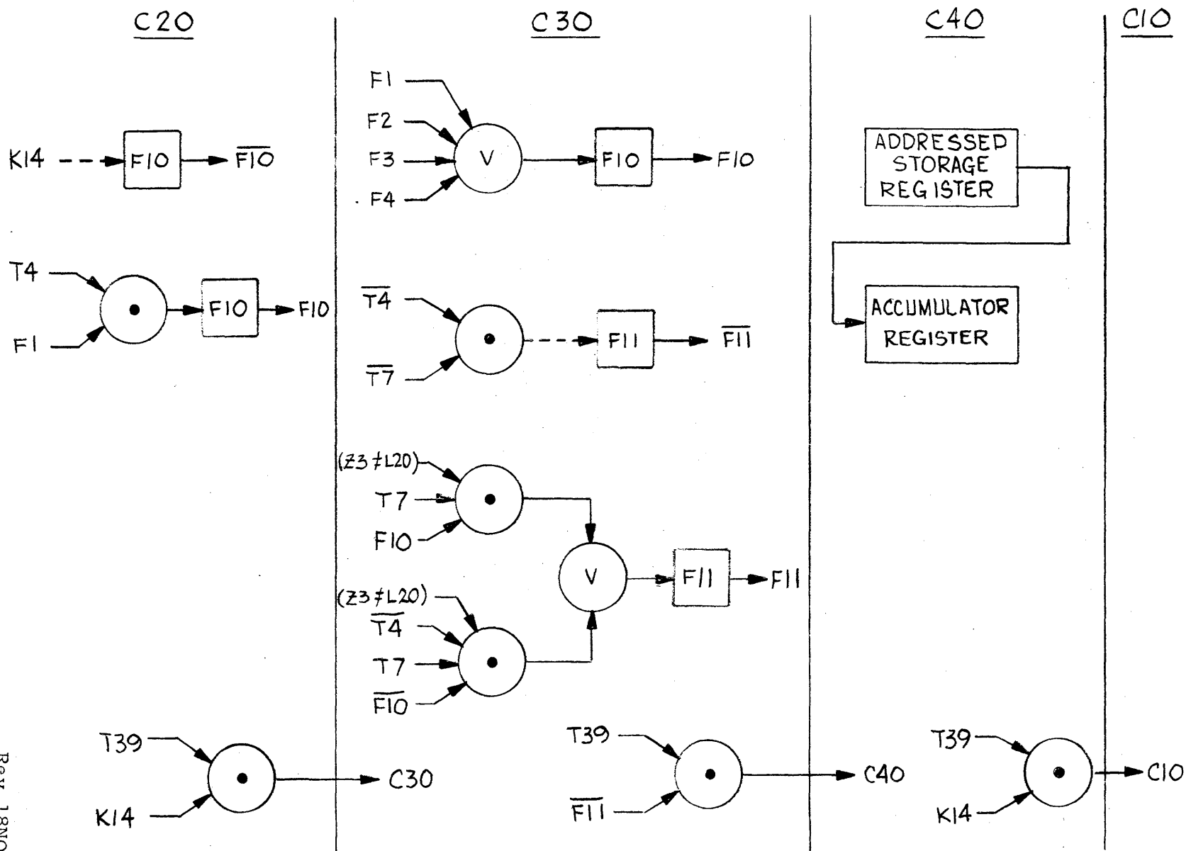
Figure 3.48.7 Clear and Add Command, Flow Chart.
