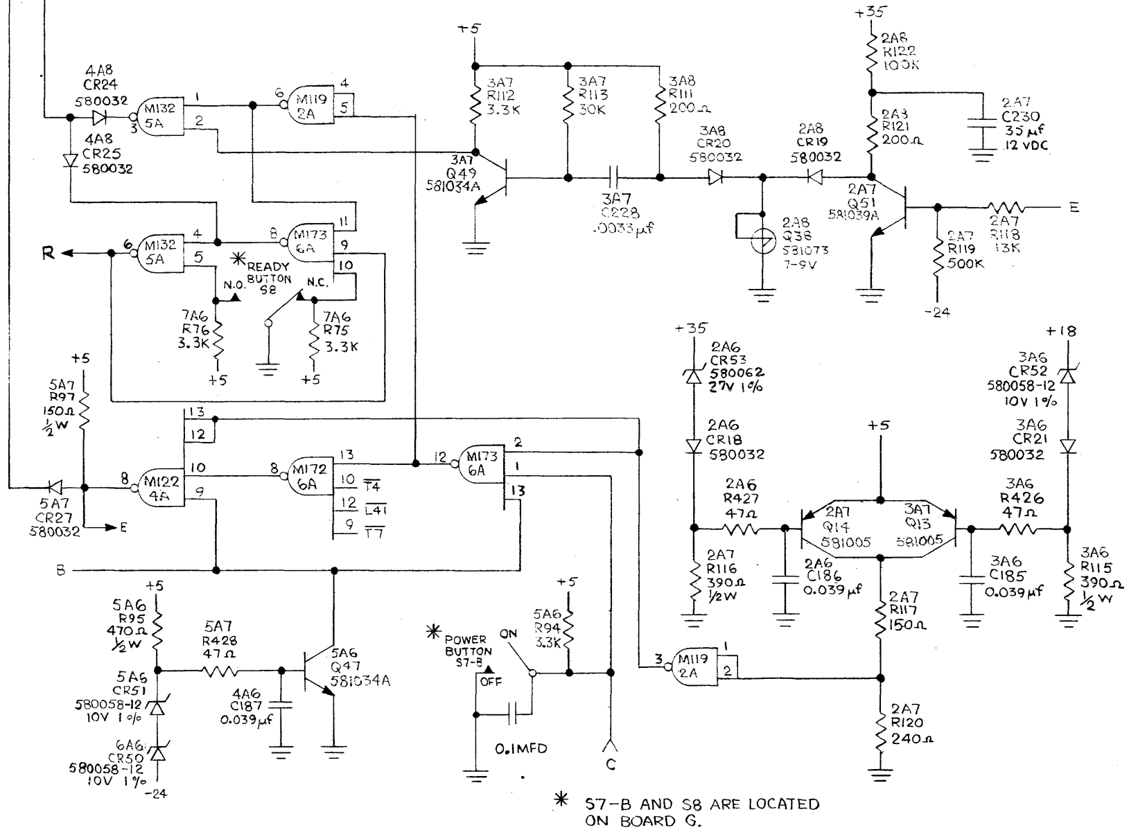
Figure 4.43 Warm-Up Circuits.
