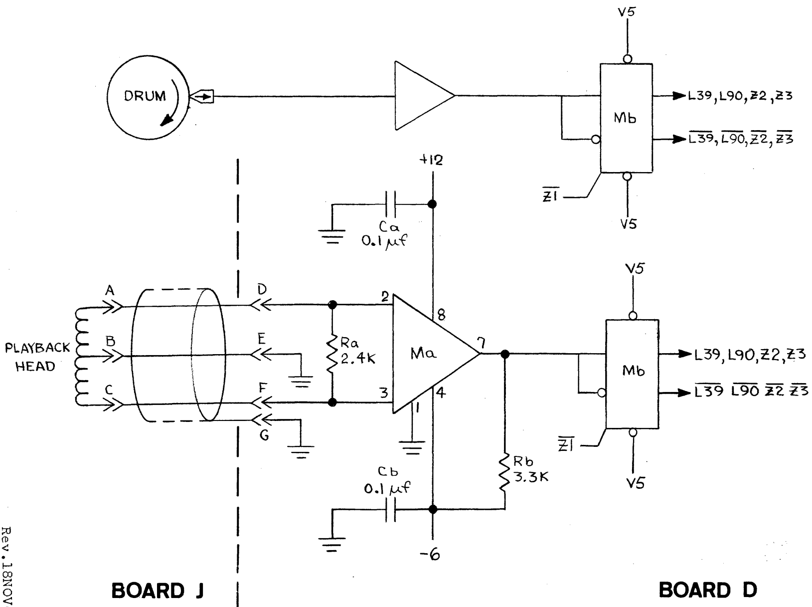
Figure 4.36 Playback Circuits L39, L90, Z2, Z3.
