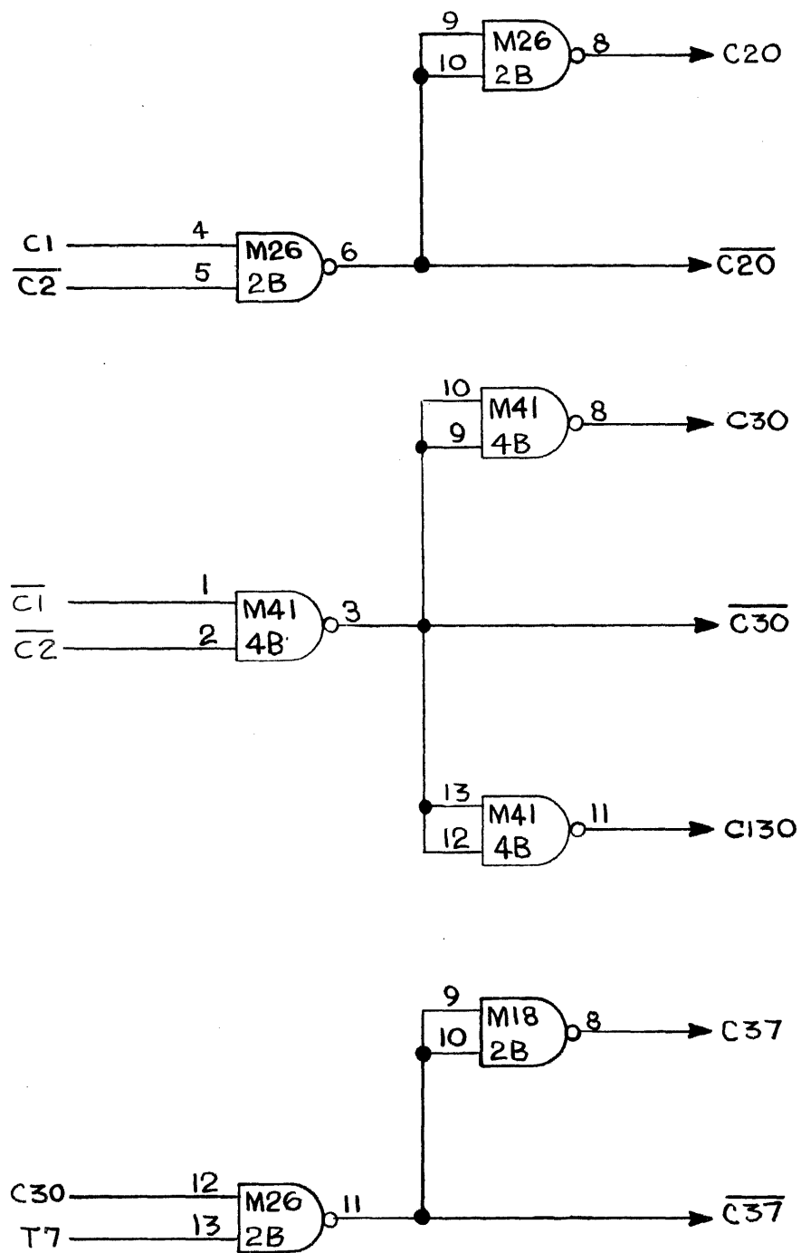
Figure 3.56 Logic Diagram.
