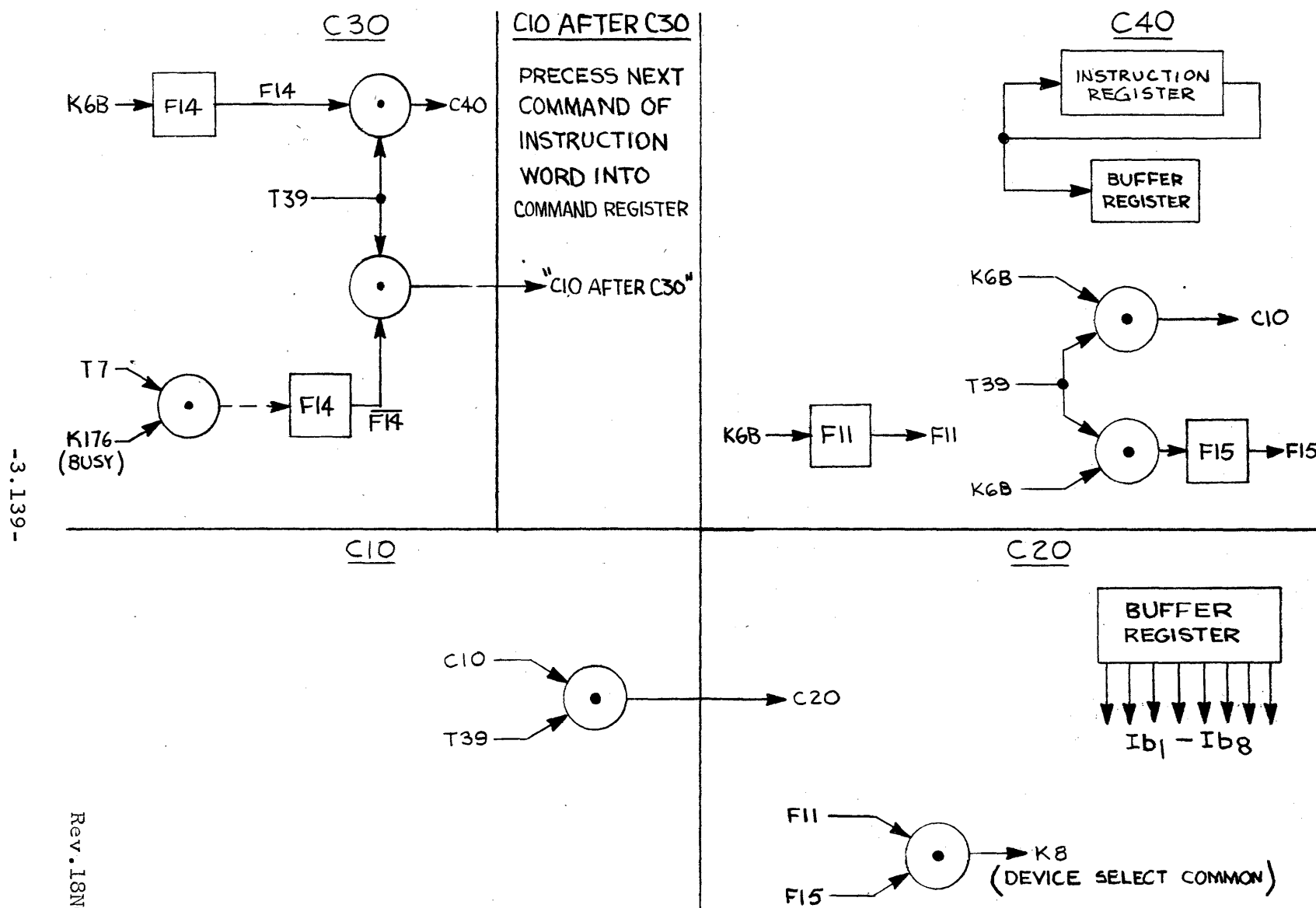
Figure 3.48.5 Immediate Select on Test Command, Flow Chart.
