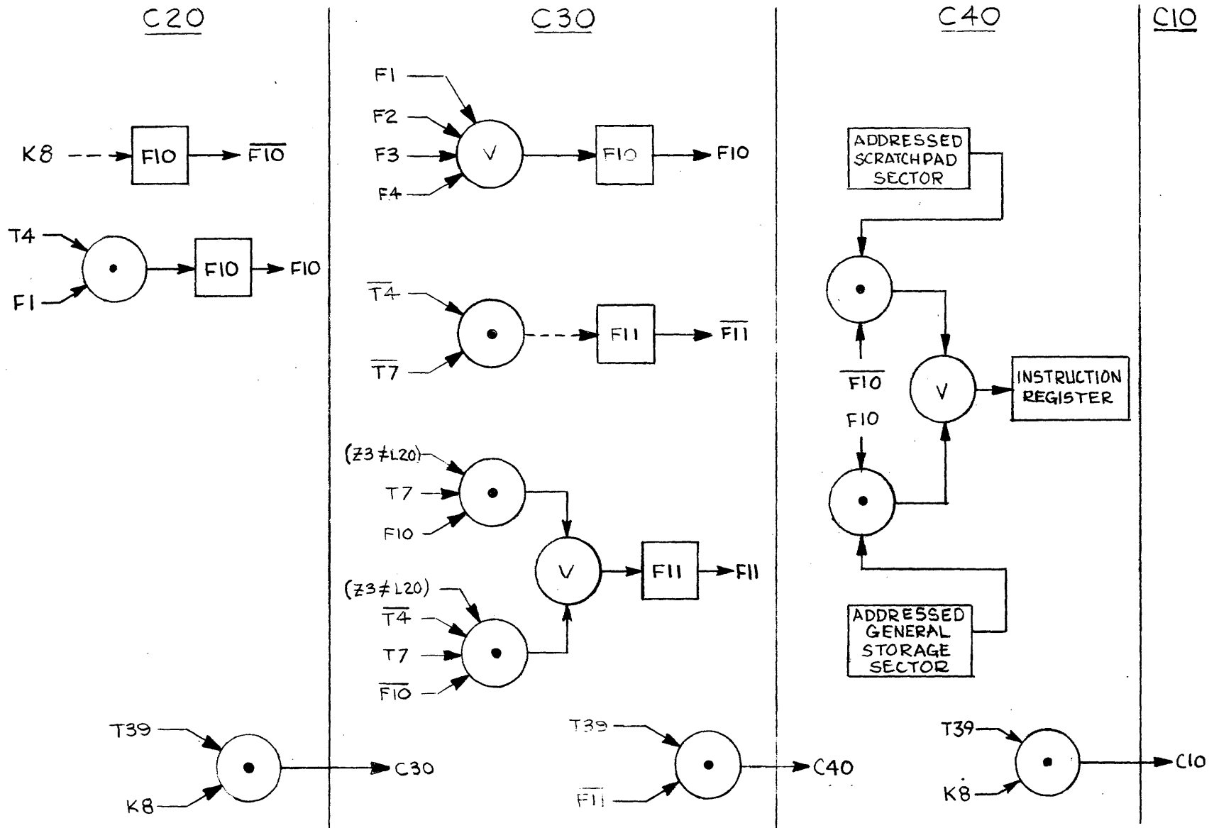
Figure 3.48.12 Jump Unconditional Command, Flow Chart.
