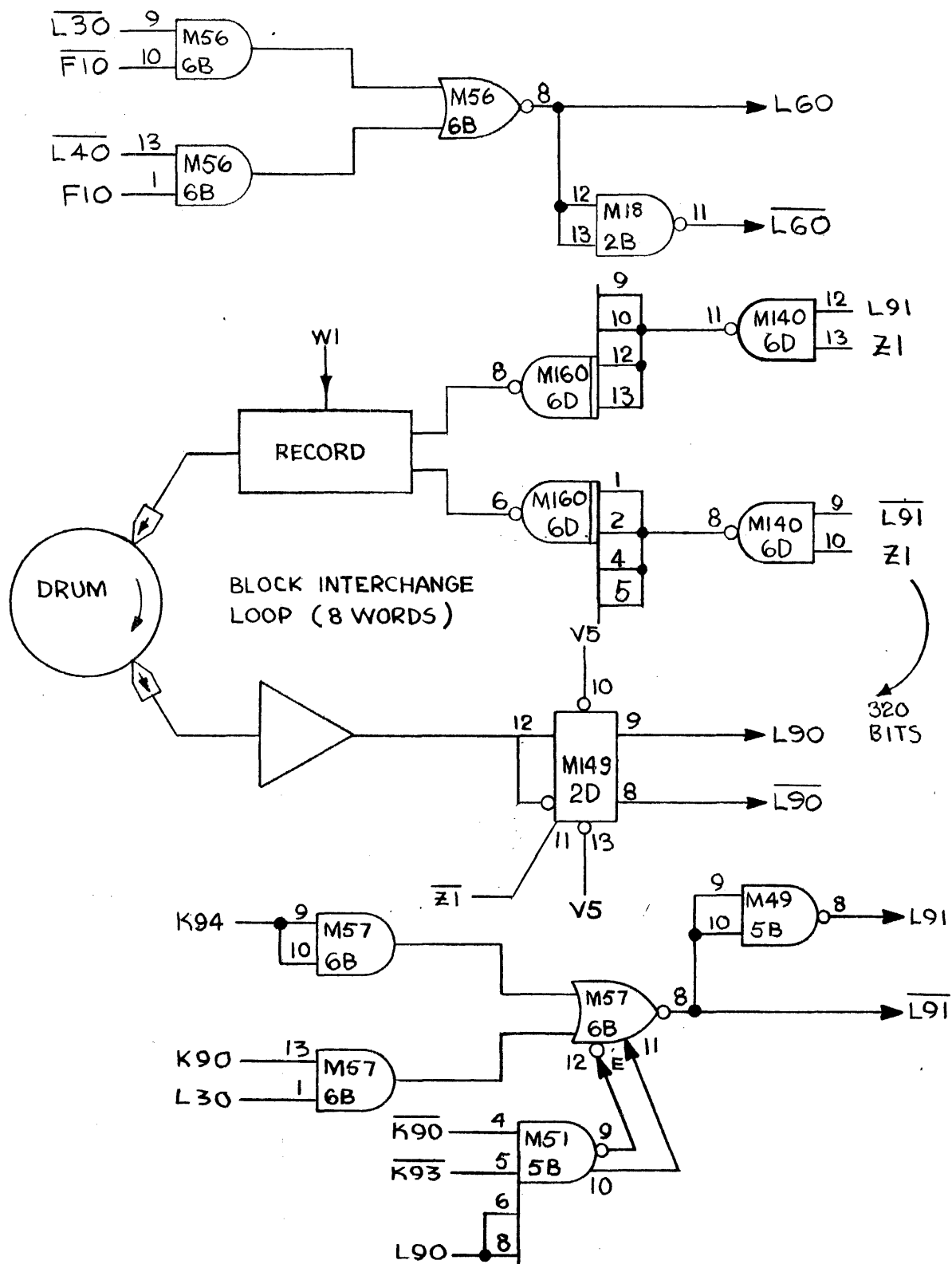
Figure 3.91 Logic Diagram.
