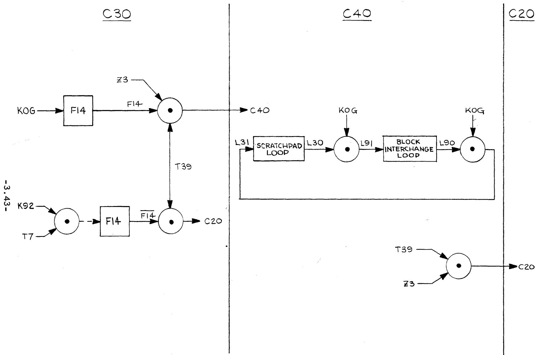
Figure 3.11 Block Interchange Command, Flow Chart.
