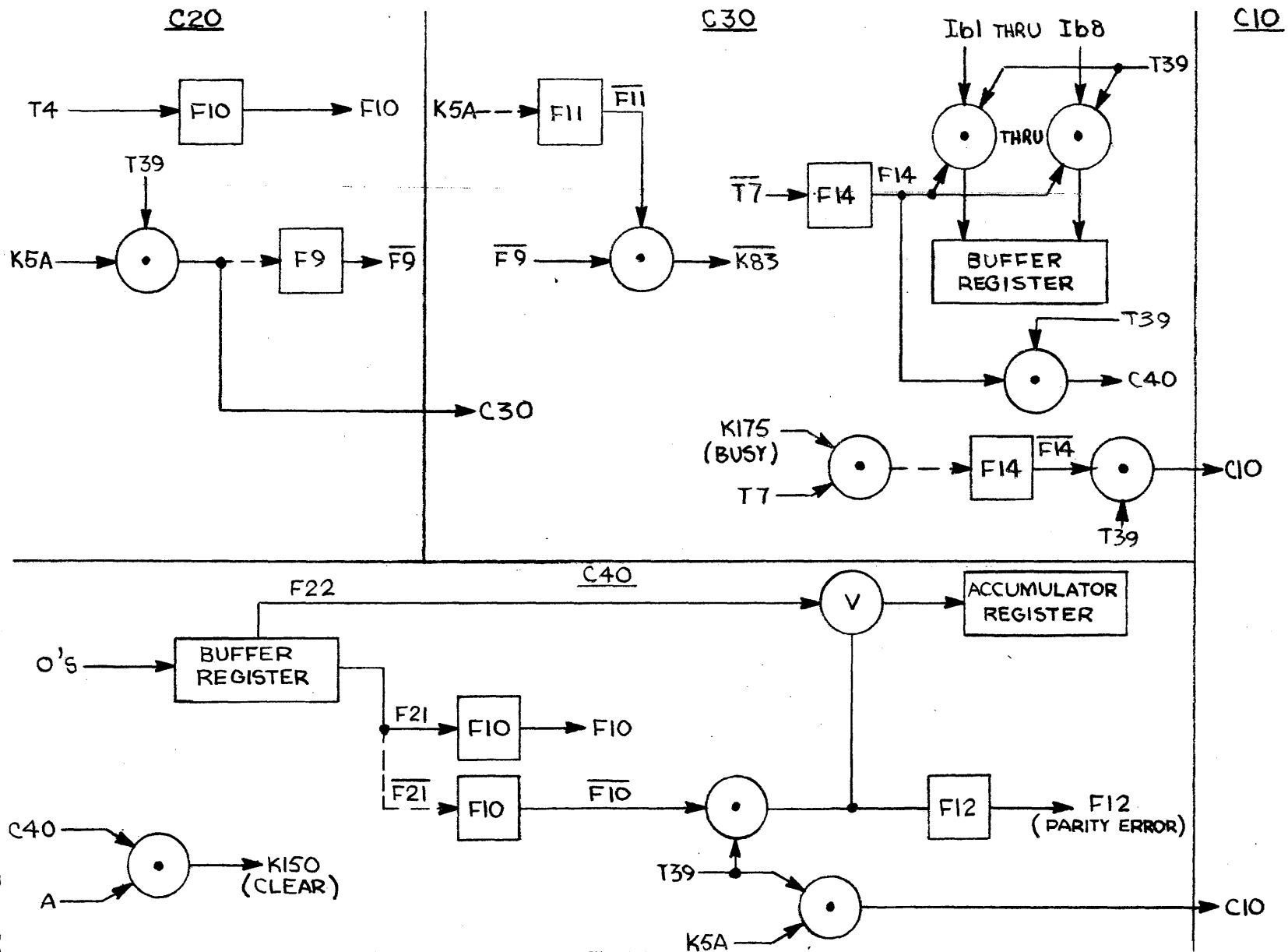
Figure 3.35 Clear, Input, Check Even Parity Into A Command, Flow Chart.
