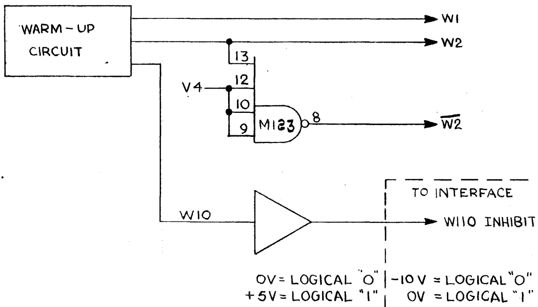
Figure 3.97 Logic Diagram.
