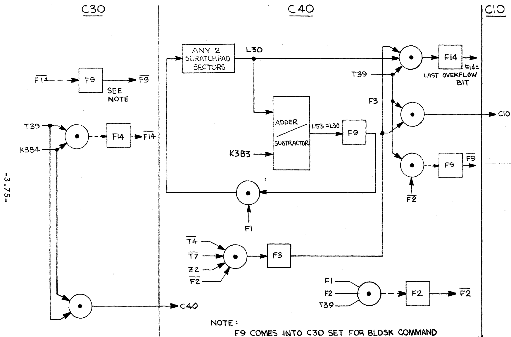
Figure 3.25 Binary Left Double Shift on Scratchpad Command and Binary Left Double Shift on Scratchpad Including K Command, Flow Chart.
