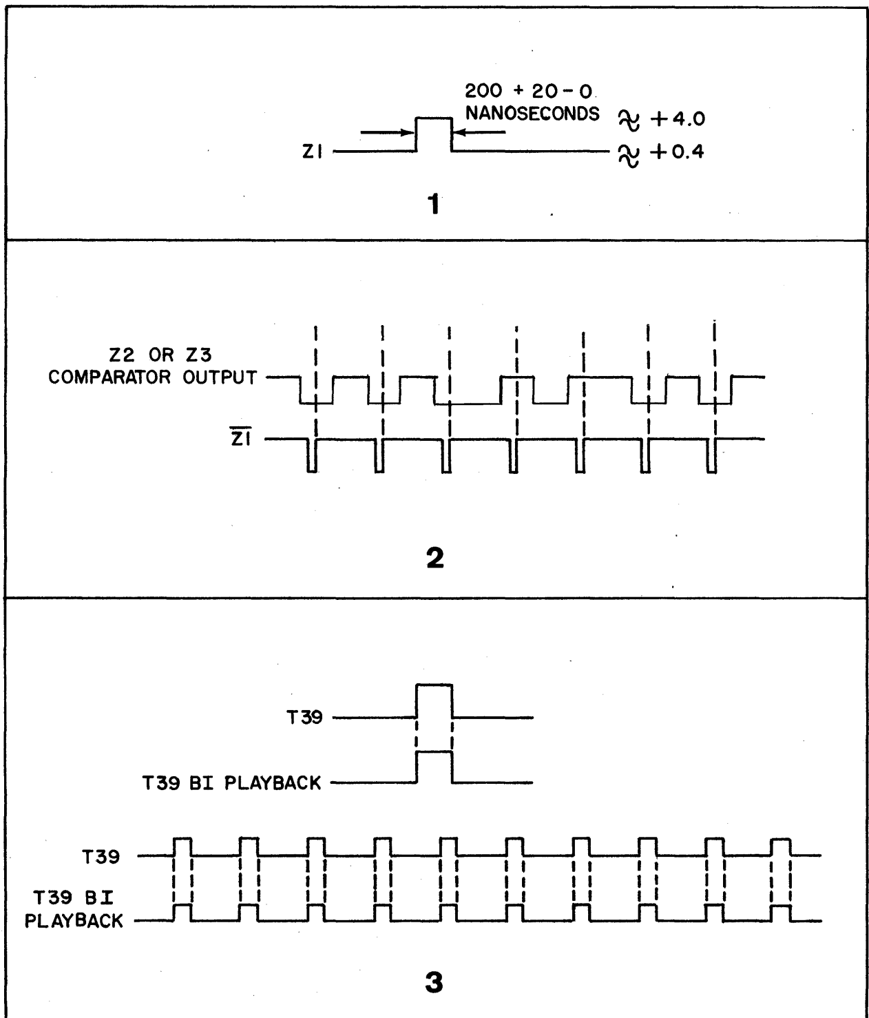
Figure 5.12 Playback Sensing.
