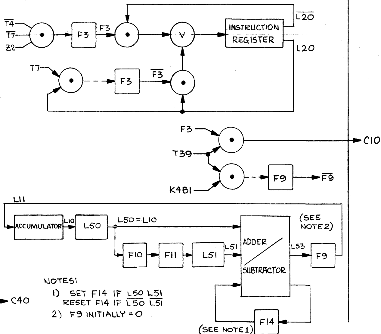
Figure 3.36 Decimal Left Single Shift Command, Flow Chart.
