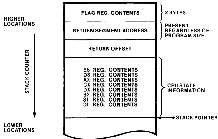
Figure I-7. 8086 Stack Layout After Interrupt Procedure Preface and Before Procedure Prologue
