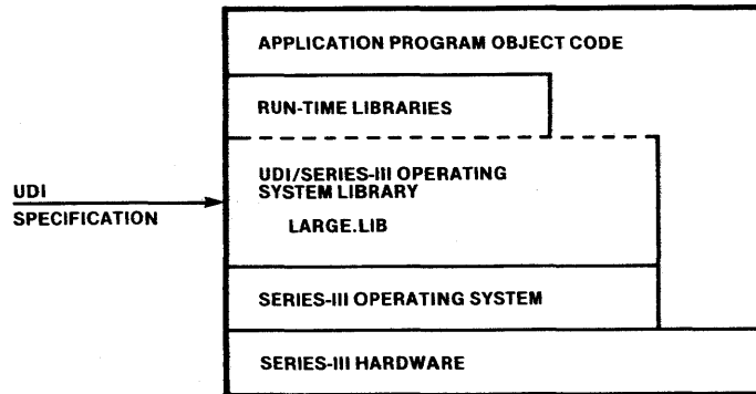
Figure I-3. UDI Libraries in Series III Development
