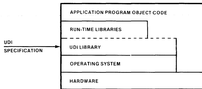
Figure I-2. Use of UDI Library
