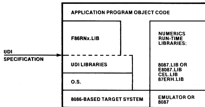
Figure I-5. I/O and Numerics Run-Time Libraries in System 121570-12
