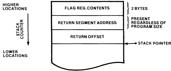
Figure I-6. 8086 Stack Layout When Interrupt Procedure Gains Control
