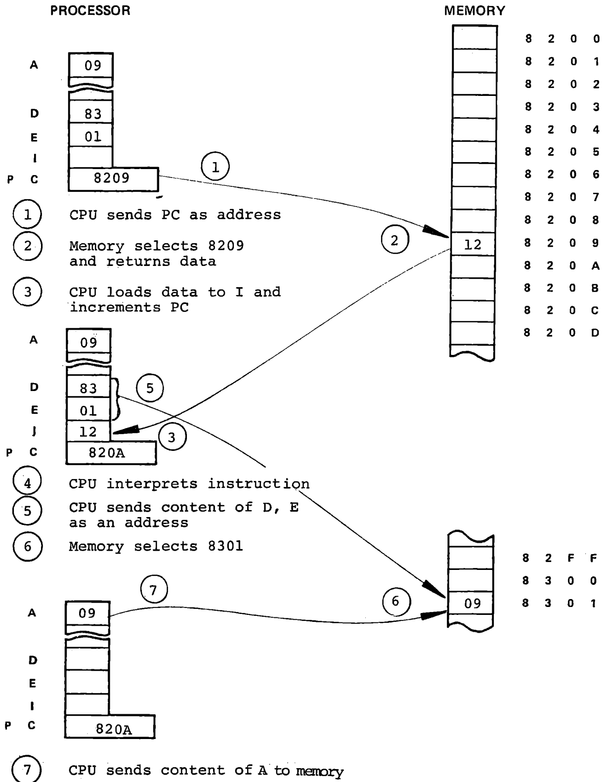
Instruction Cycle for STAX D Instruction Figure 4-6
