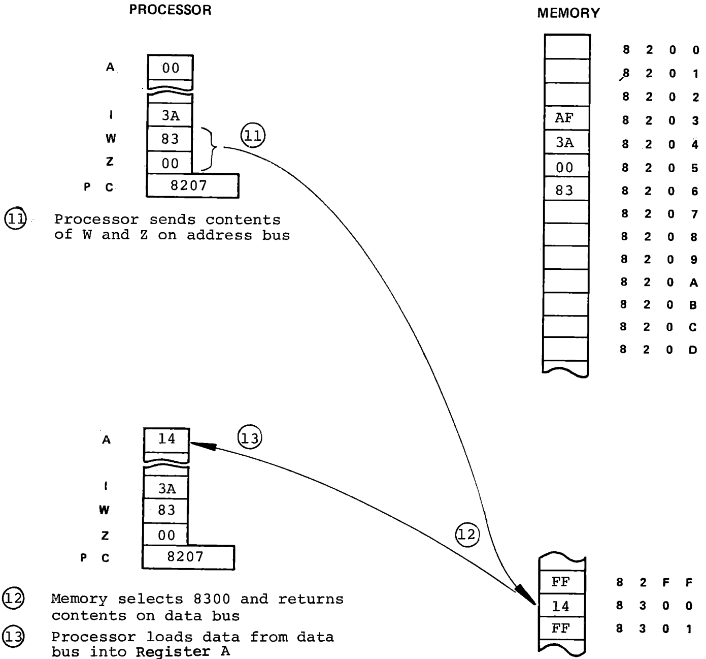
LDA Instruction Cycle (continued)
