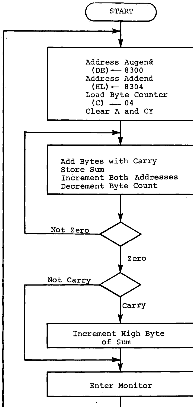
Four Byte Addition in Memory
