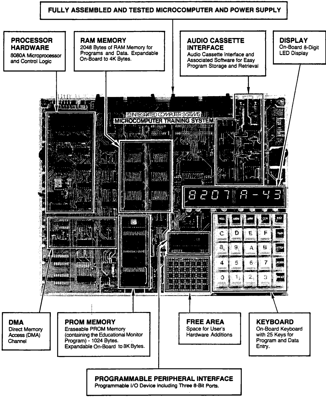
MTS Board Layout Figure 1-1
