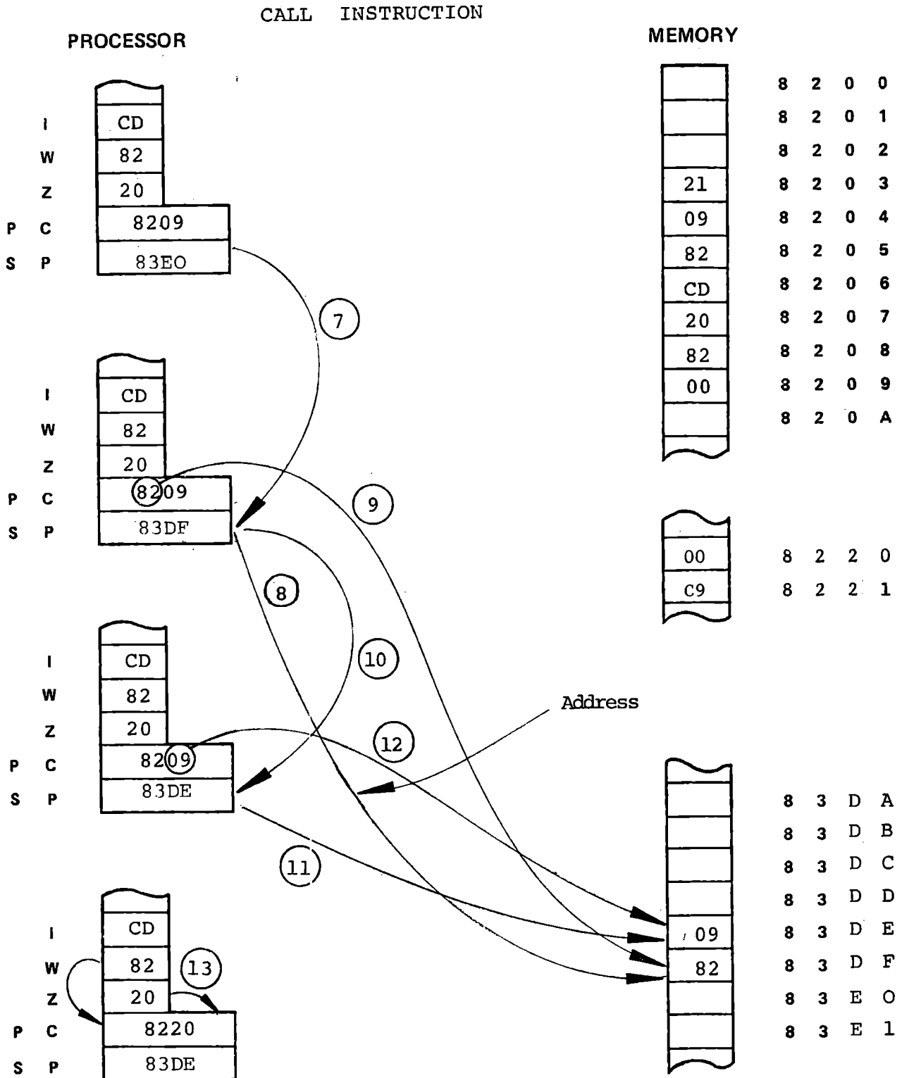
The stack pointer is decremented (7) and sent out as an address (8). The high byte of the program counter is sent on the data bus (9) and written to the addressed memory location. This is repeated for the low byte of the program counter (10,11,12). Then the content of W,Z, is moved to PC.
