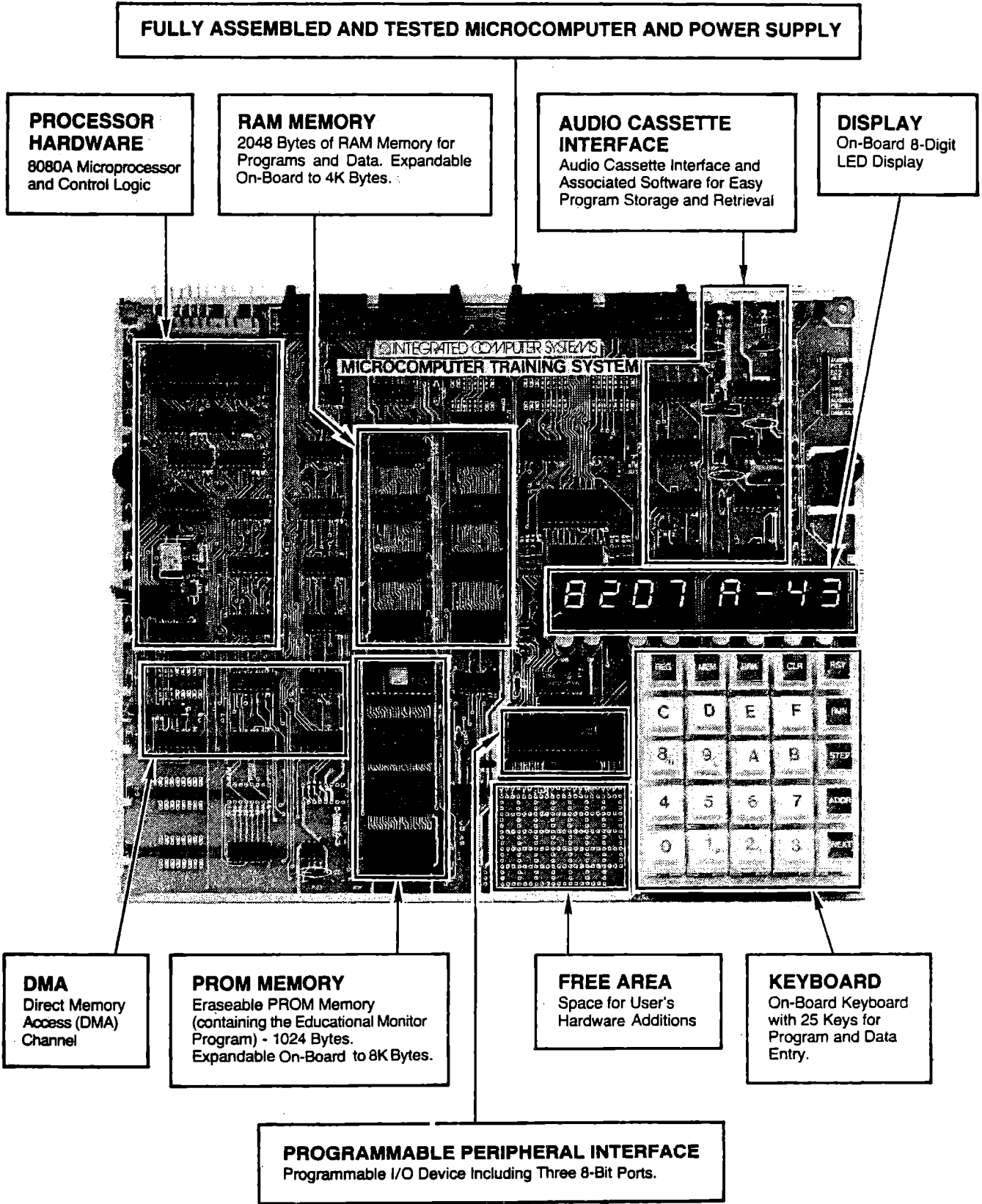
MTS Board Layout Figure 1-2
