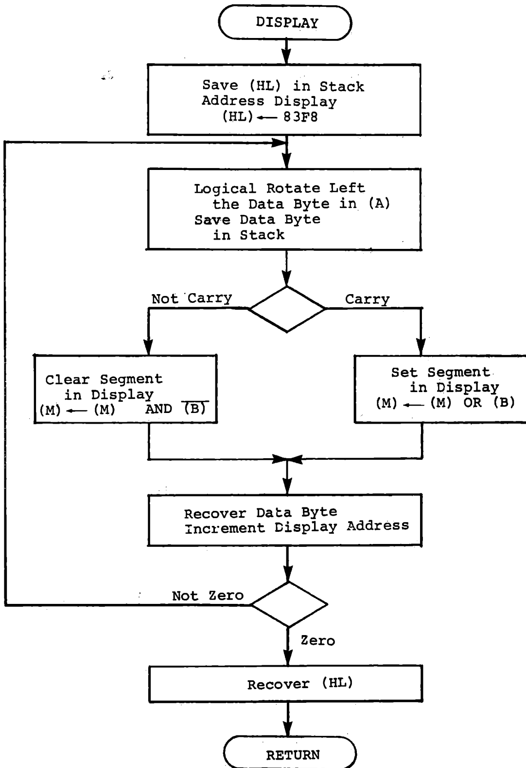
Logic Functions Display Subroutine
