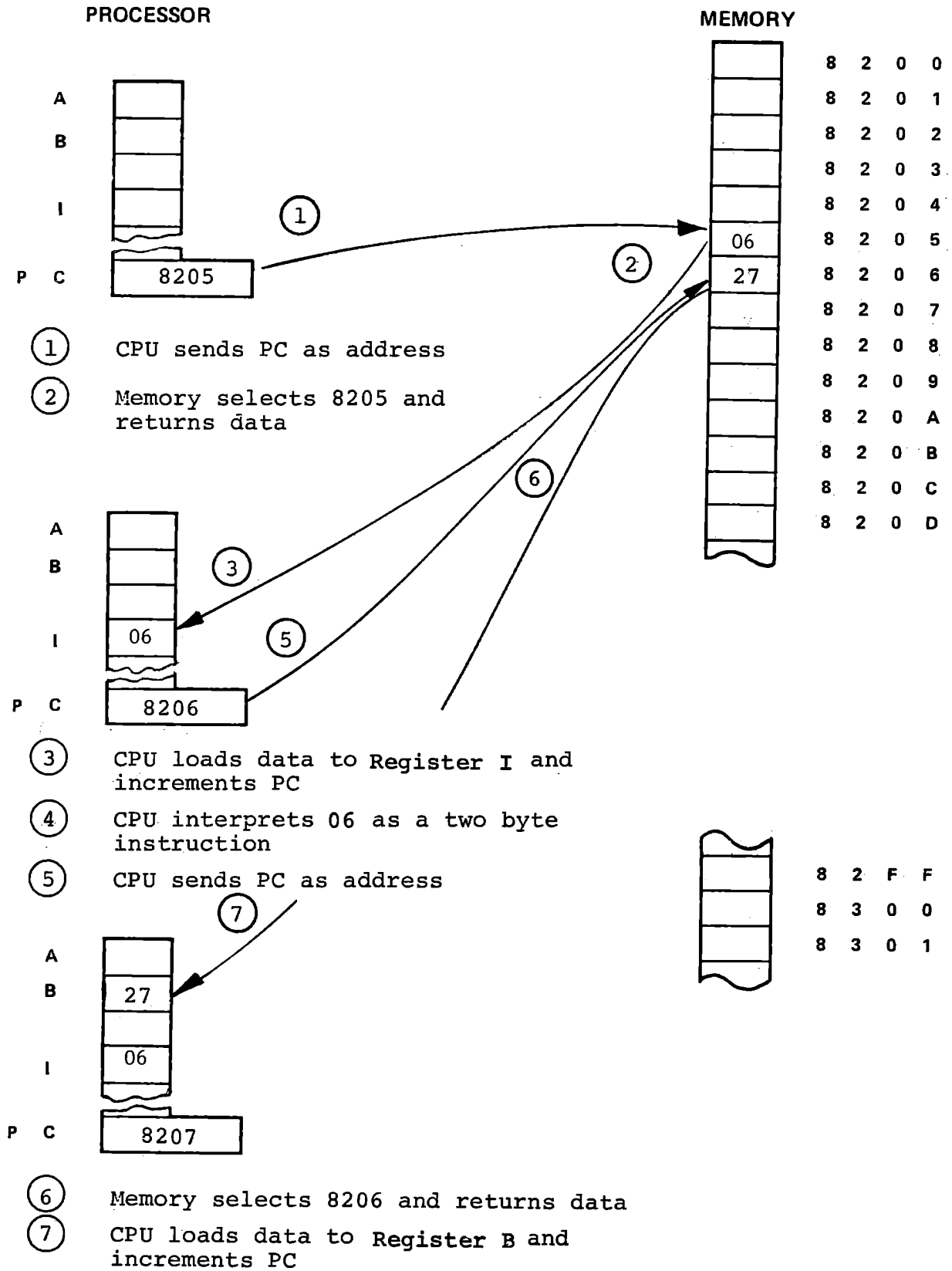
MVI Instruction Cycle
