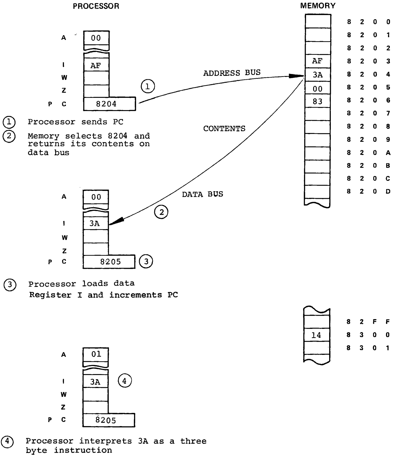
LDA Instruction Cycle
