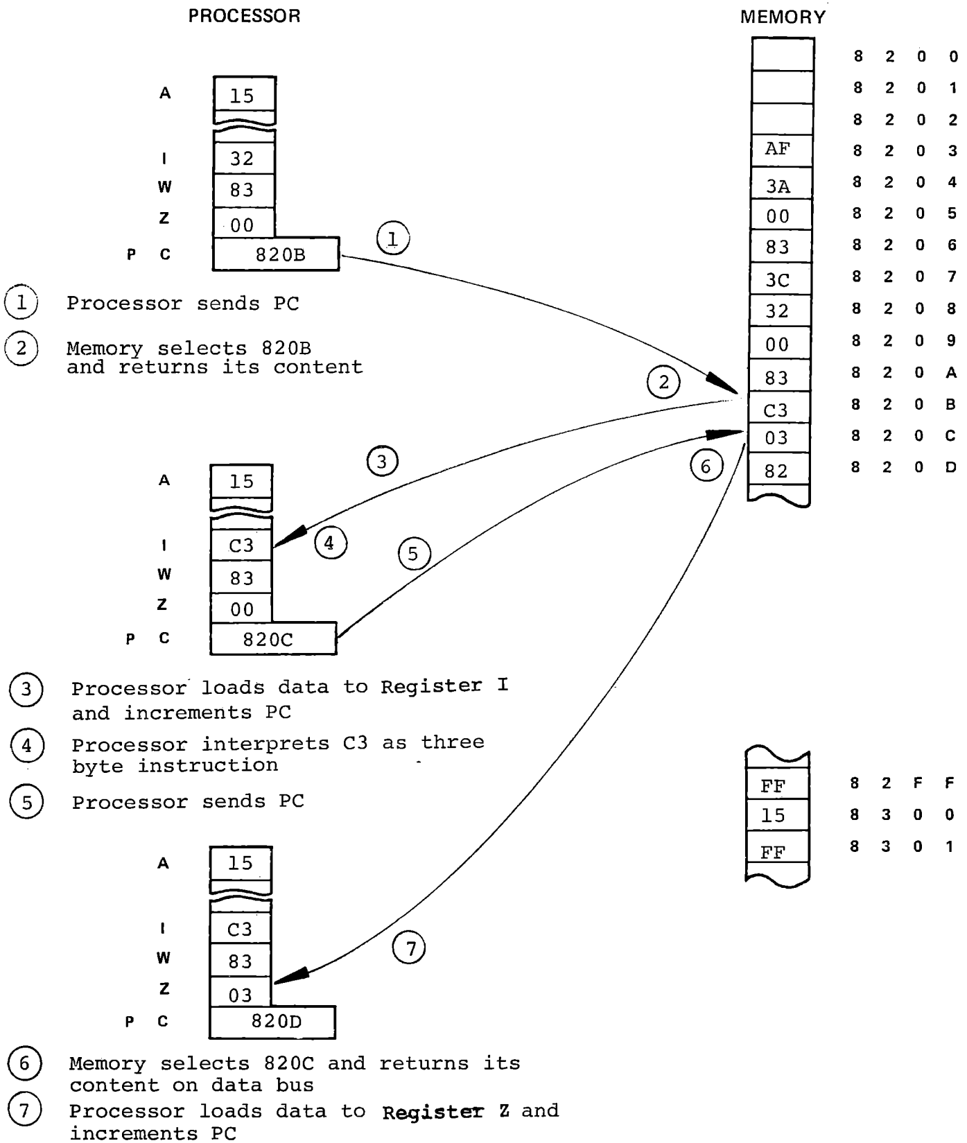
JMP Instruction Cycle
