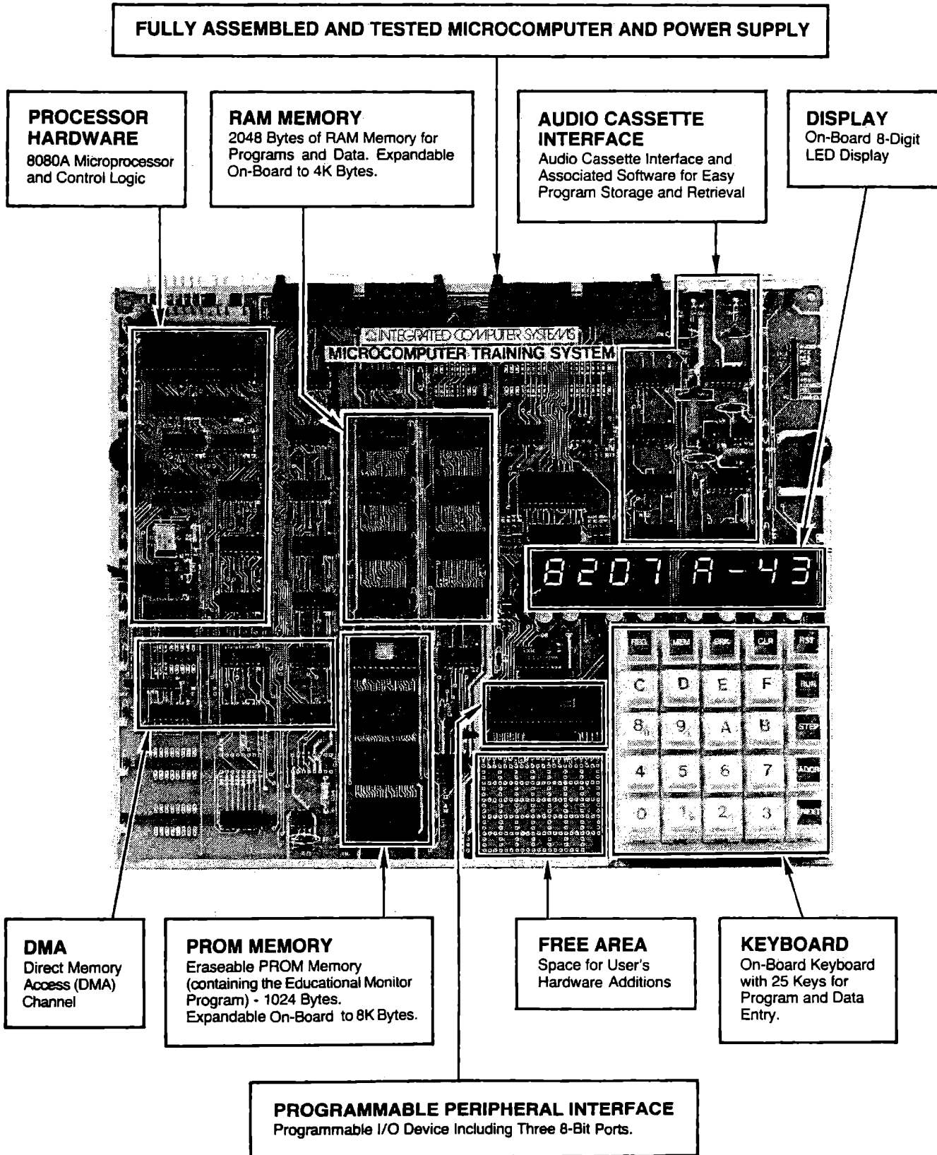
MTS Board Layout Figure 1-3
