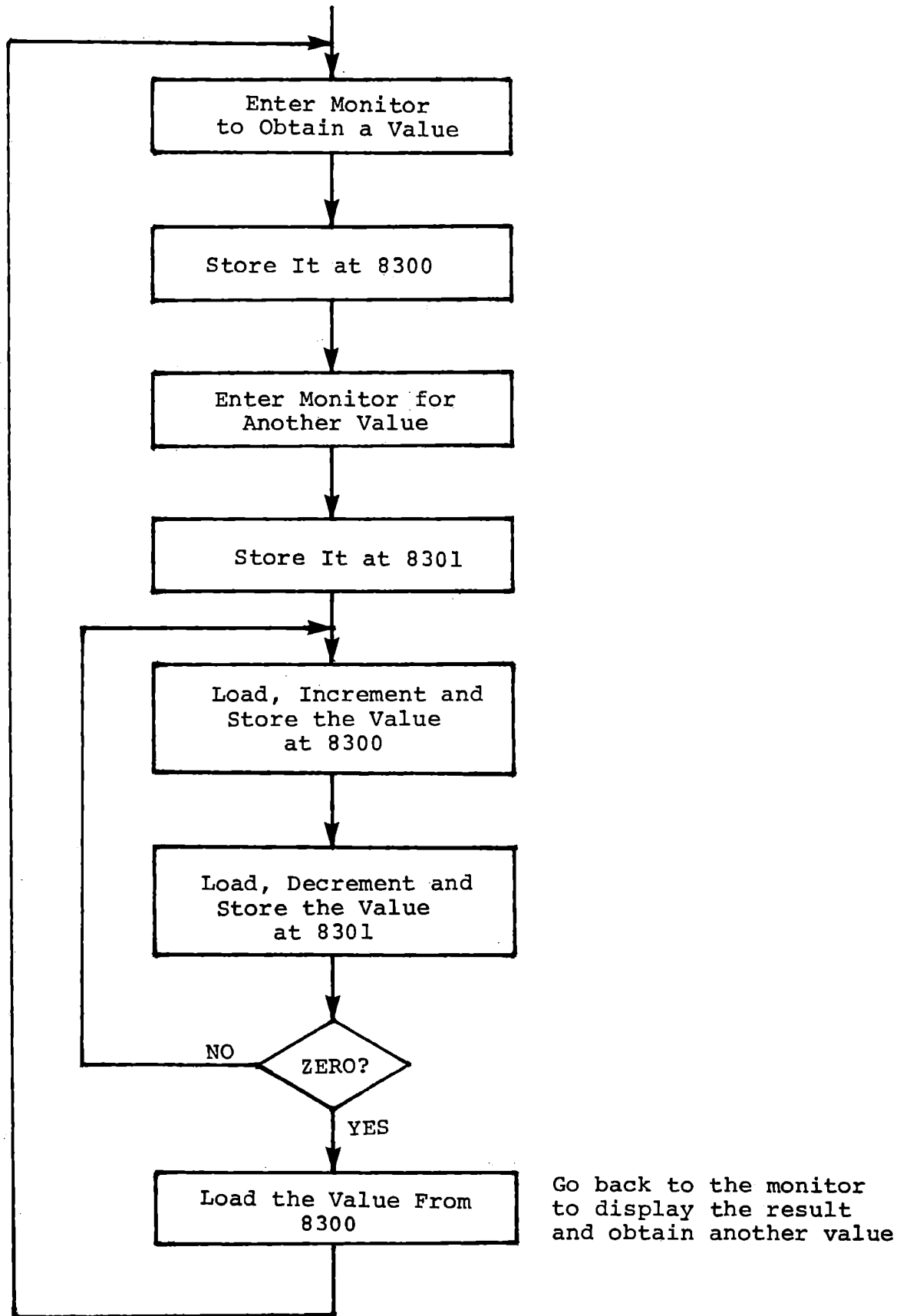
Addition by Counting
