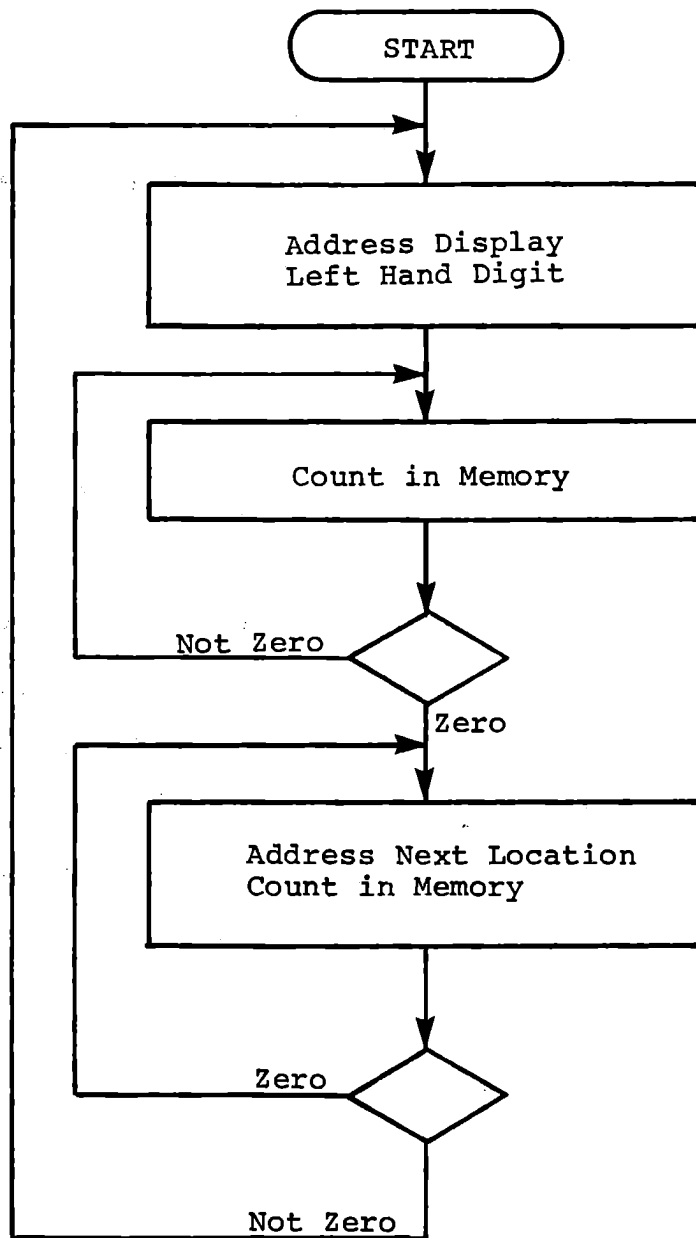
Counting in the Display
