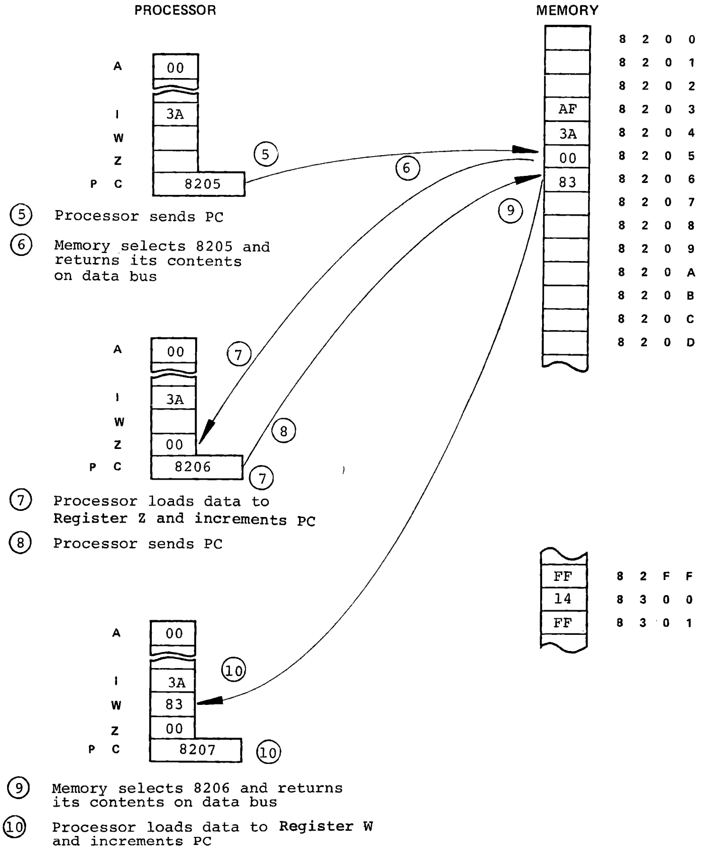
LDA Instruction Cycle (continued)
