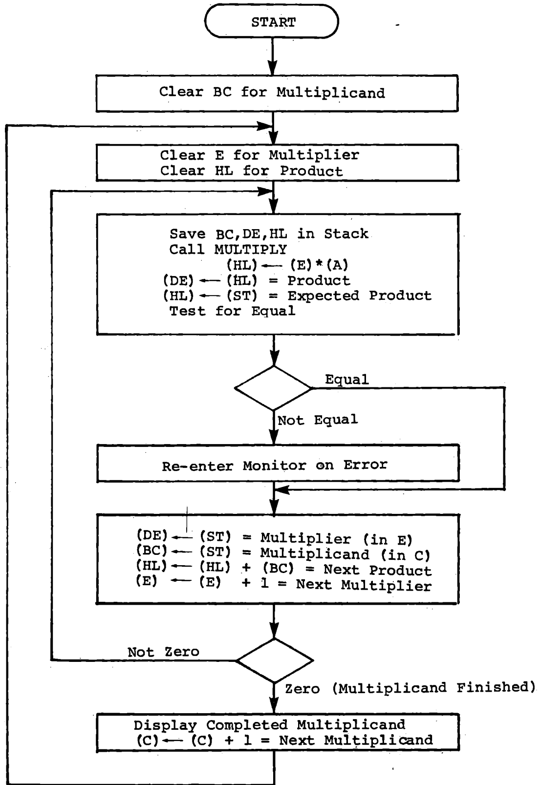
Test Driver for MULTIPLY
