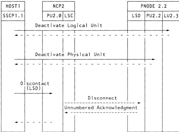
Deactivating a Peripheral Node Attached via a Nonswitched SDLC Link
