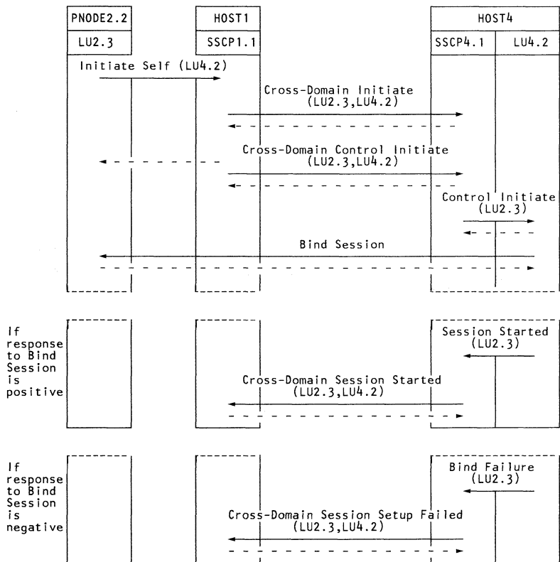
Establishing a Cross-Domain LU-LU Session
