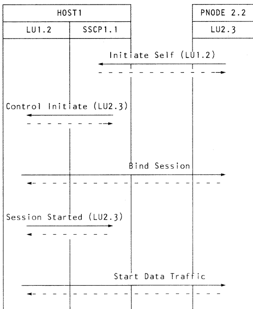
Establishing a Same-Domain LU-LU Session Figure 14-9.
