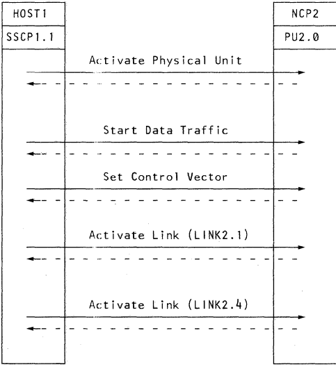
Activating a Channel-Attached Subarea Node and Attached Links
