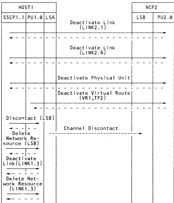
Deactivating a Channel-Attached Subarea Node and Associated Resources
