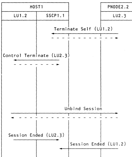
Terminating a Same-Domain LU-LU Session Figure 14-12.
