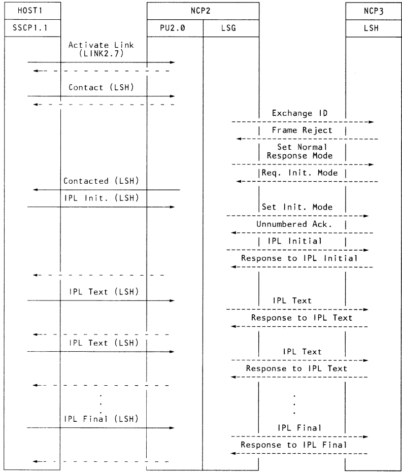
Loading a 3705 Communications Controller with an NCP Figure 14-6.
