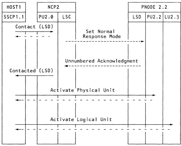
Activating a Peripheral Node Attached via a Nonswitched SDLC Link
