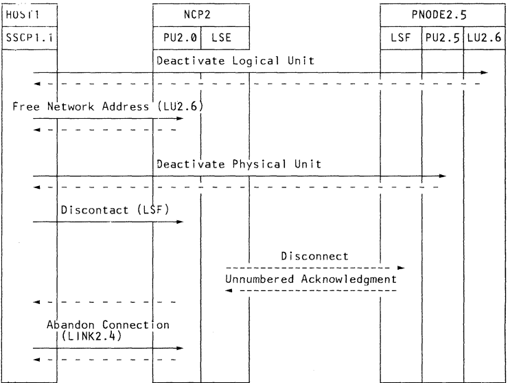
Deactivating a Peripheral Node Attached to a Switched SDLC Link Figure 14-17.
