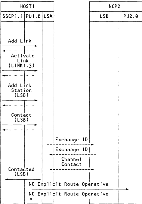
Activating a Host Node, a Channel-Attached Subarea Node, and the Channel Between Them Figure 14-1.
