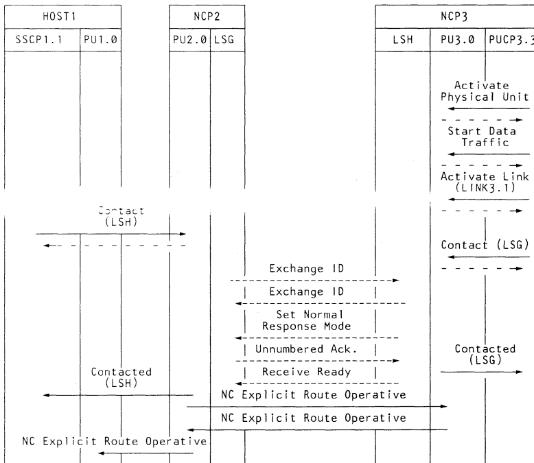
Activating and SDLC Link Between Subarea Nodes
