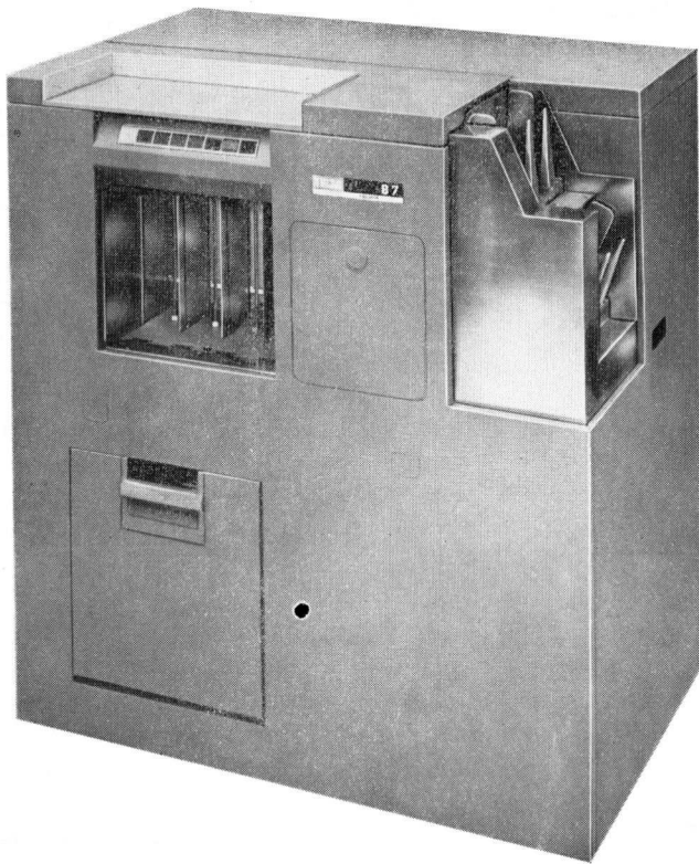
FIGURE 28. IBM 87 COLLATOR
