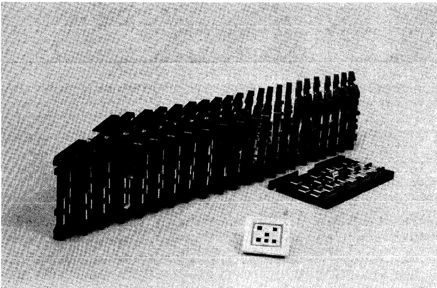
Figure 05.05.6. One MLC 50 logic module with six chips and 23 MST logic cards with the same number of circuits
