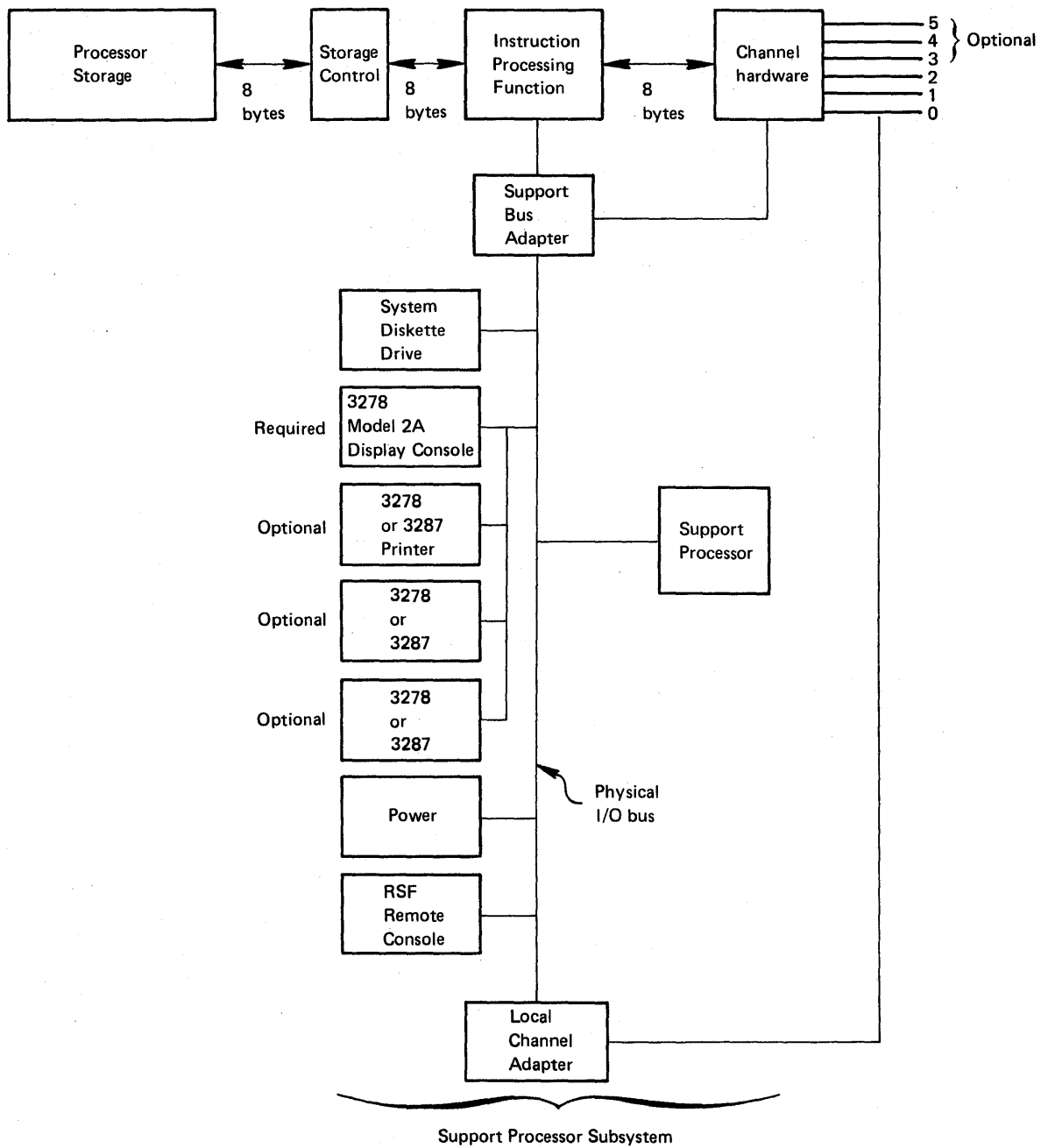
Figure 05.15.2. Logical components in the 4341 Processor
