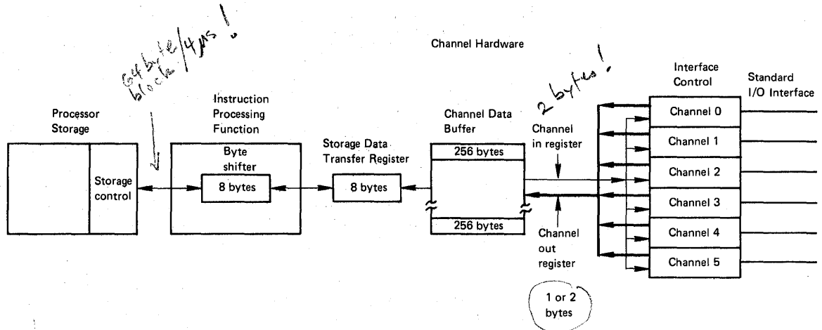
Figure 10.20.1. General flow of data between the channels and processor storage
