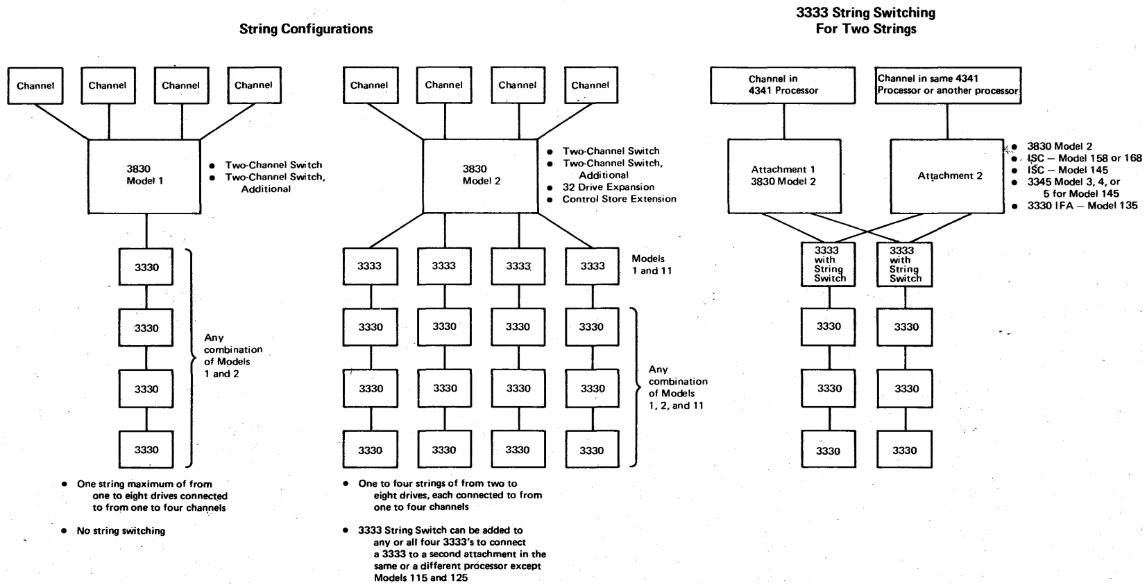
Figure 20.10.1. Summary of 3330-series string configurations for the 4341 Processor
