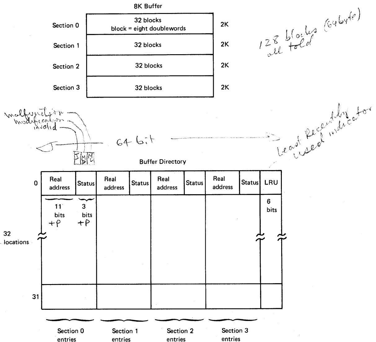
Figure 10.10.3. Buffer organization in the 4341 Processor
