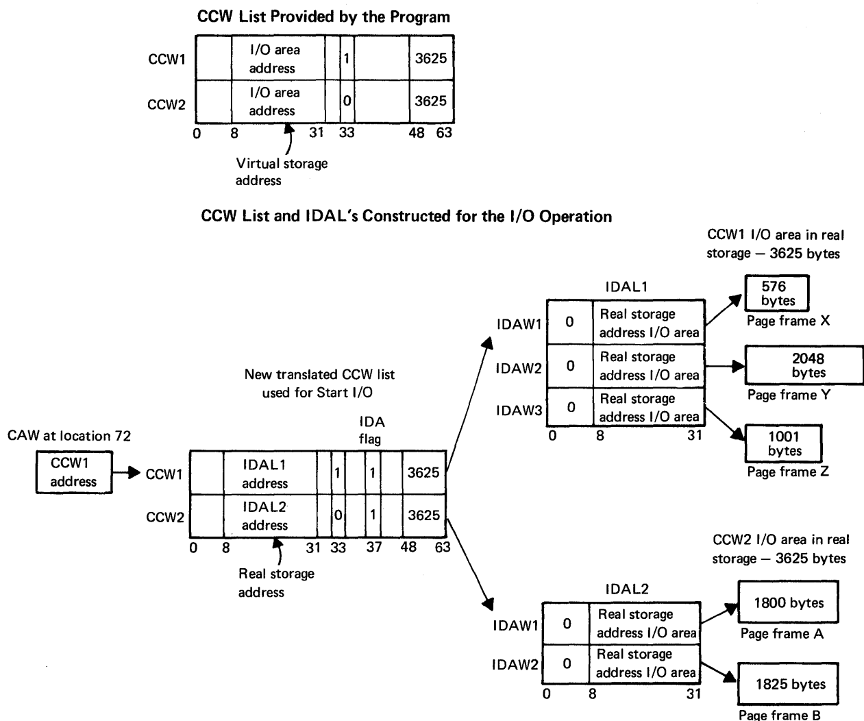
Figure 15.10.5. Example of IDALs required for a CCW list when page size is 2K
