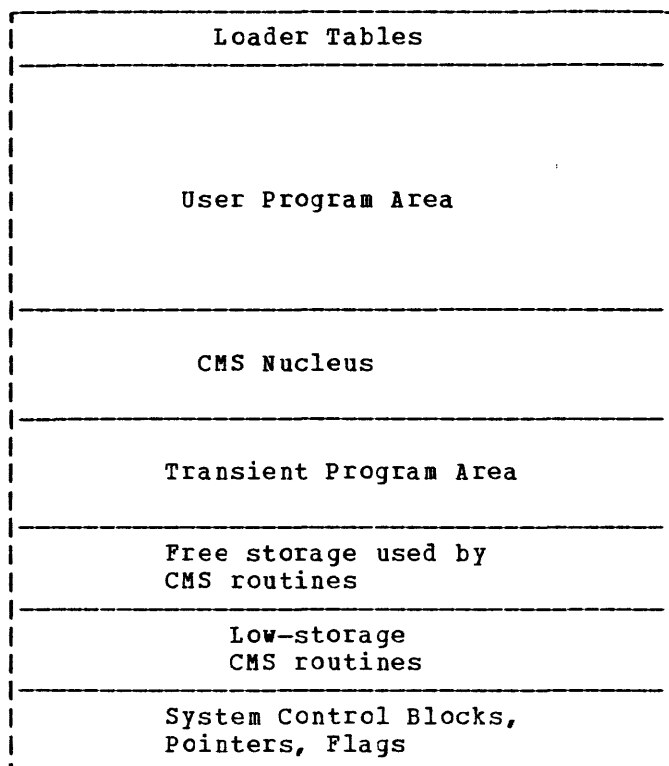
Figure 19. Simplified CMS Storage Map
