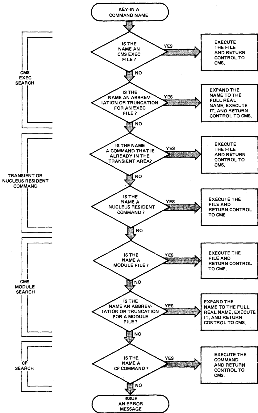
Figure 4. How CMS Searches for the Command to Execute
