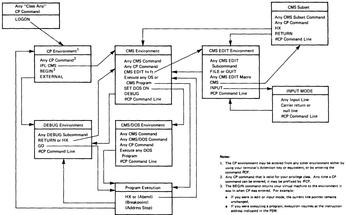
Figure 1. VM/370 Environments and Mode Switching
