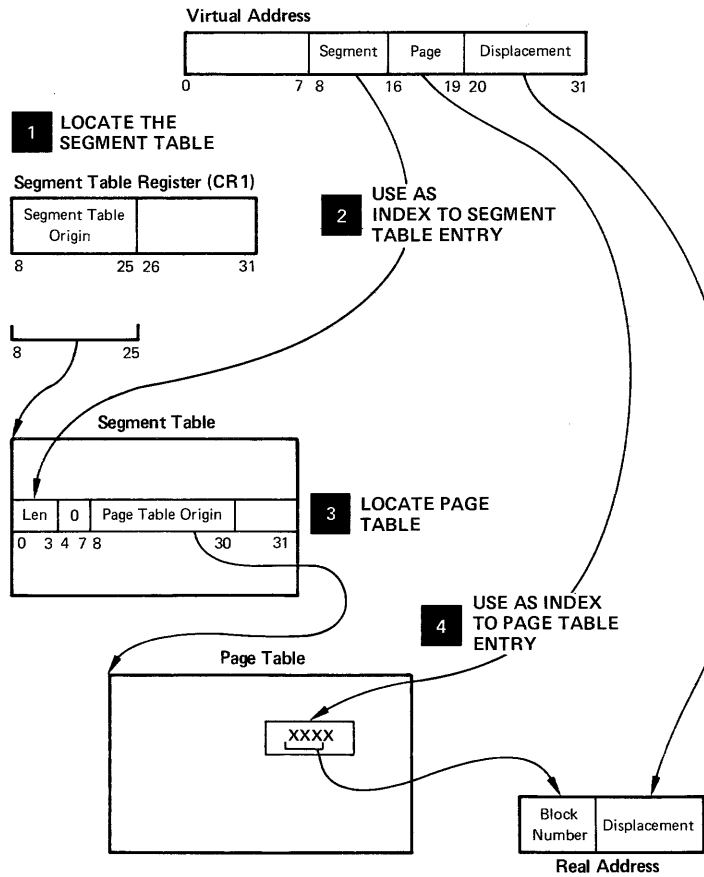
Figure 27. Virtual-to-Real Address Translation
