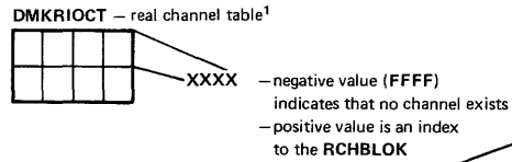
Figure 18. Real I/O Control Blocks
