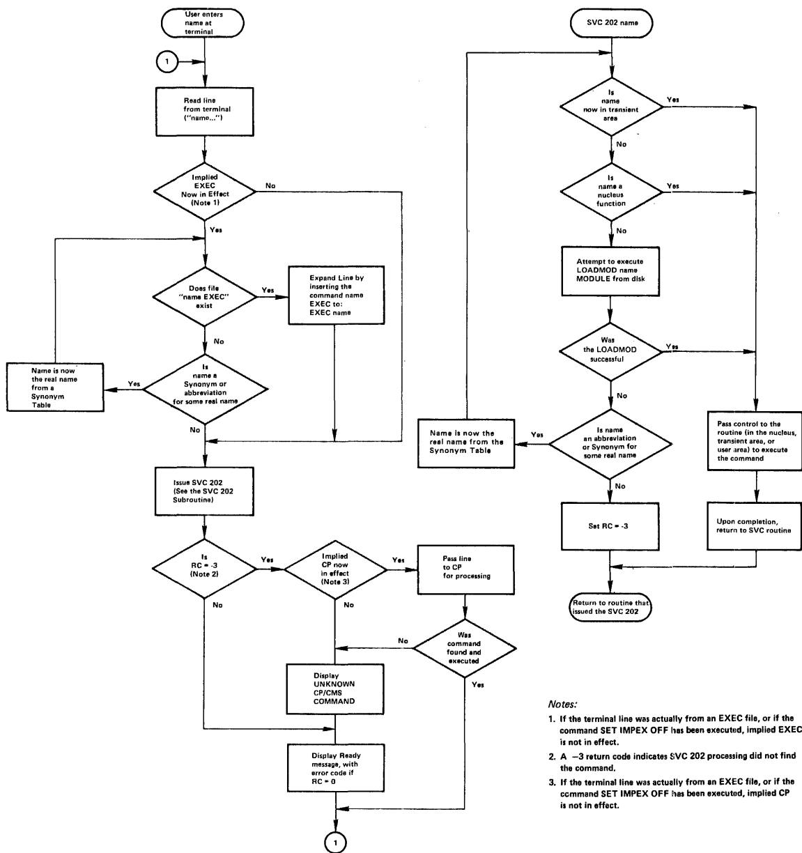
Figure 35. CMS Command (and Request) Processing
