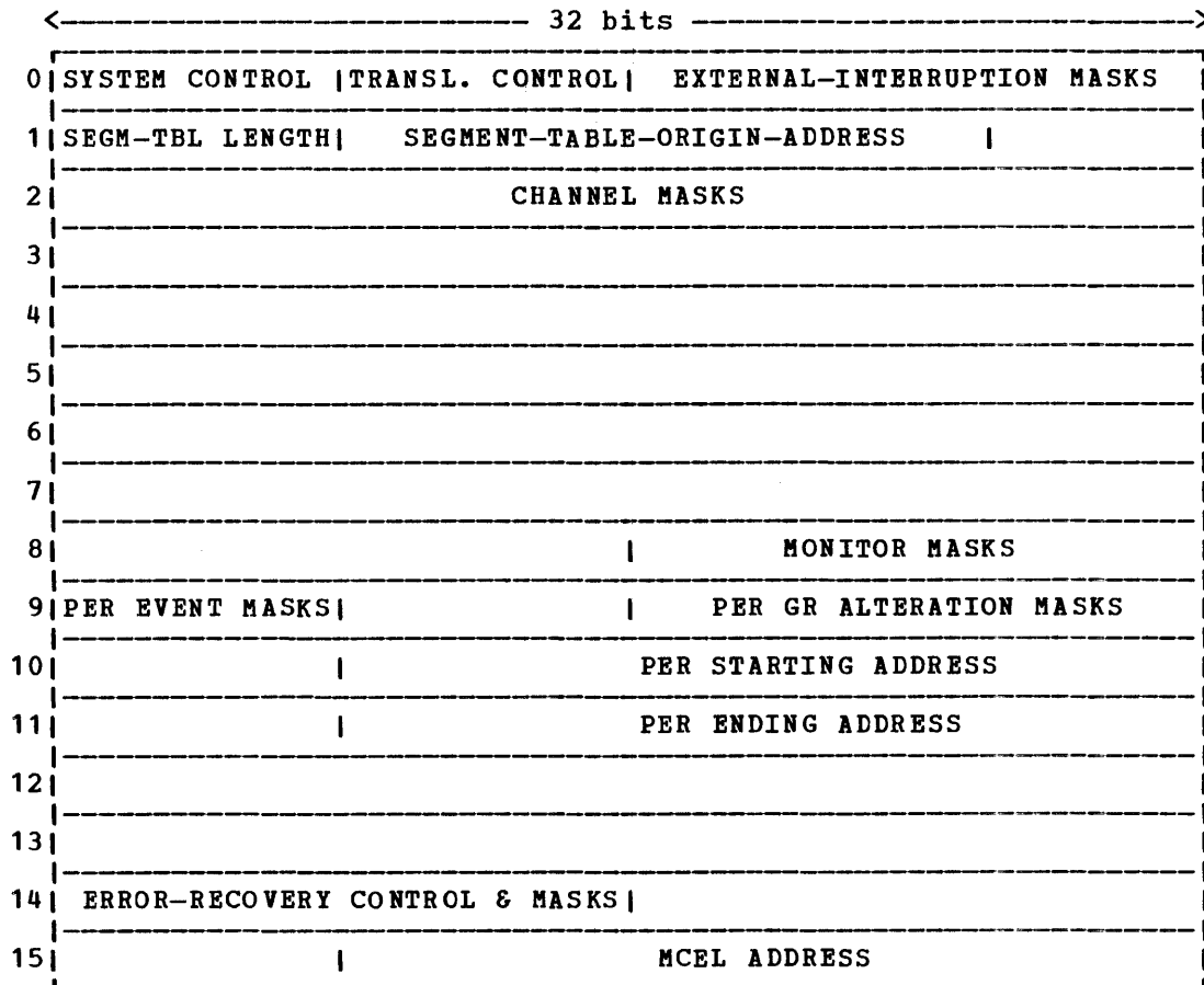
Figure 52. Control Register Allocation
