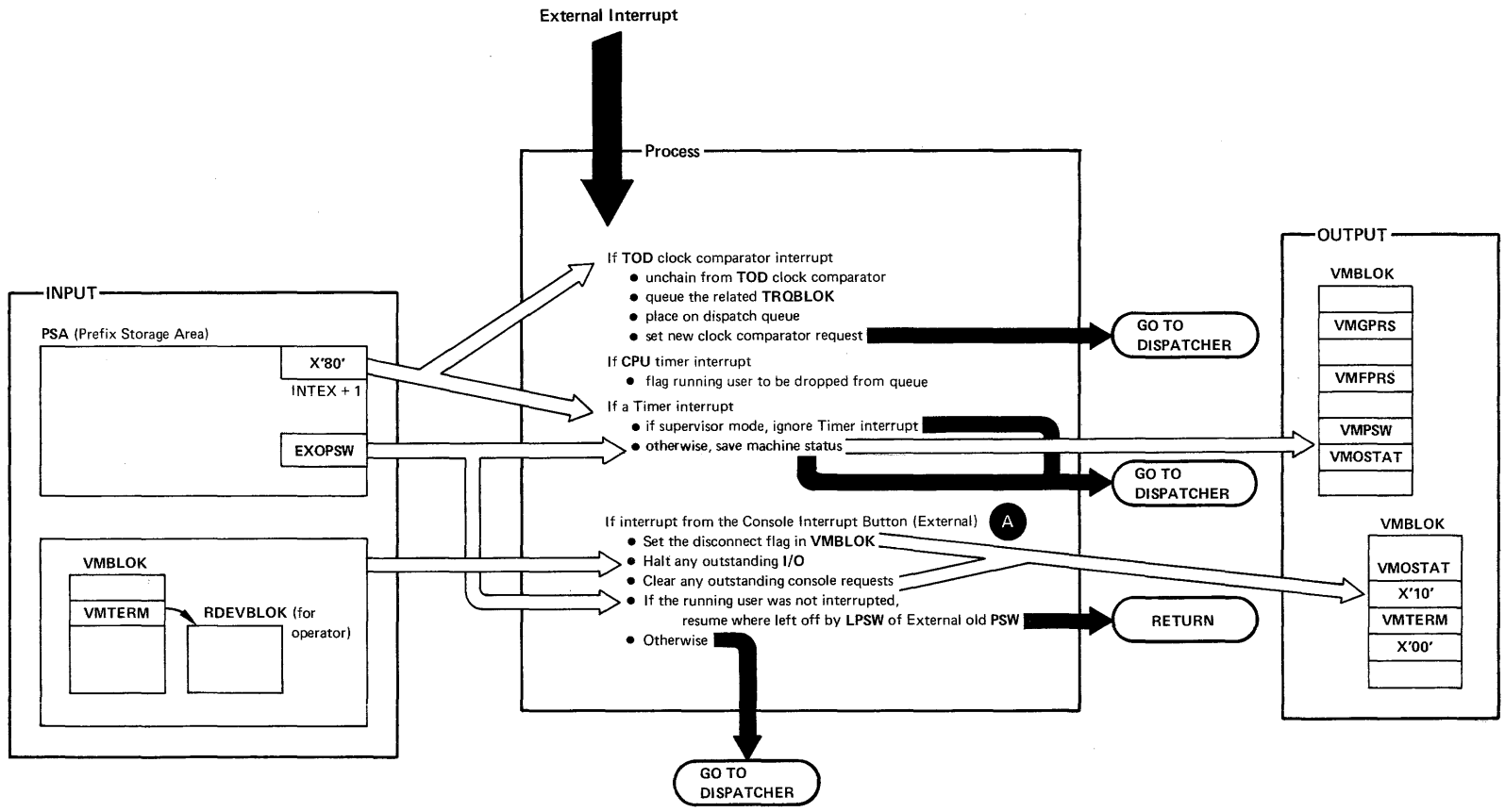
Figure 21. External Interrupt Handling
