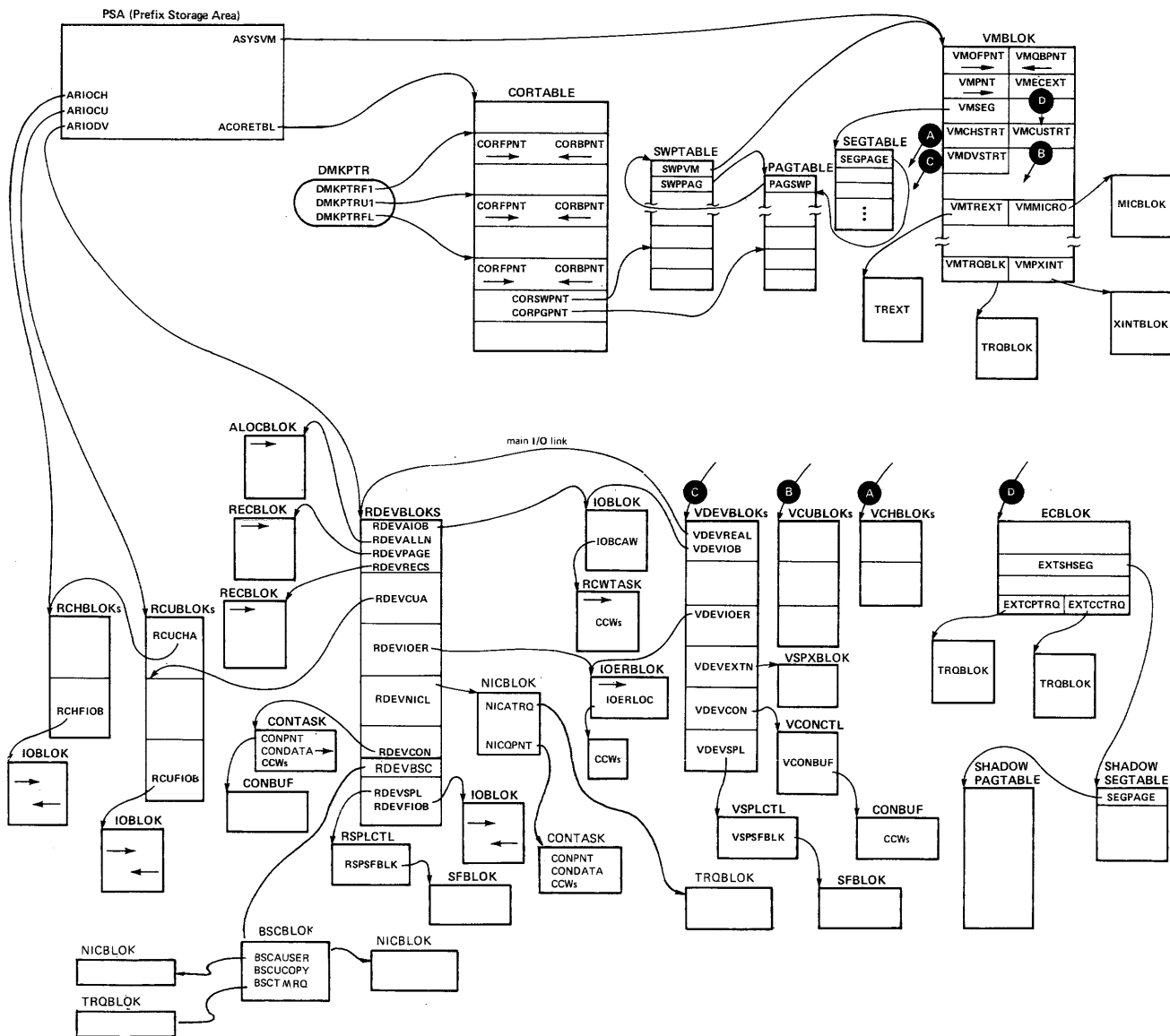
Figure 11. CP Control Block Relationships
