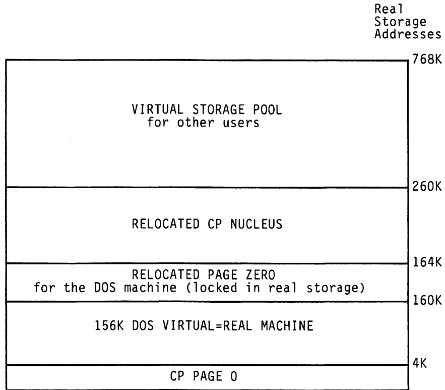
Figure 1. DOS 160K Virtual=Real Storage Assignments
