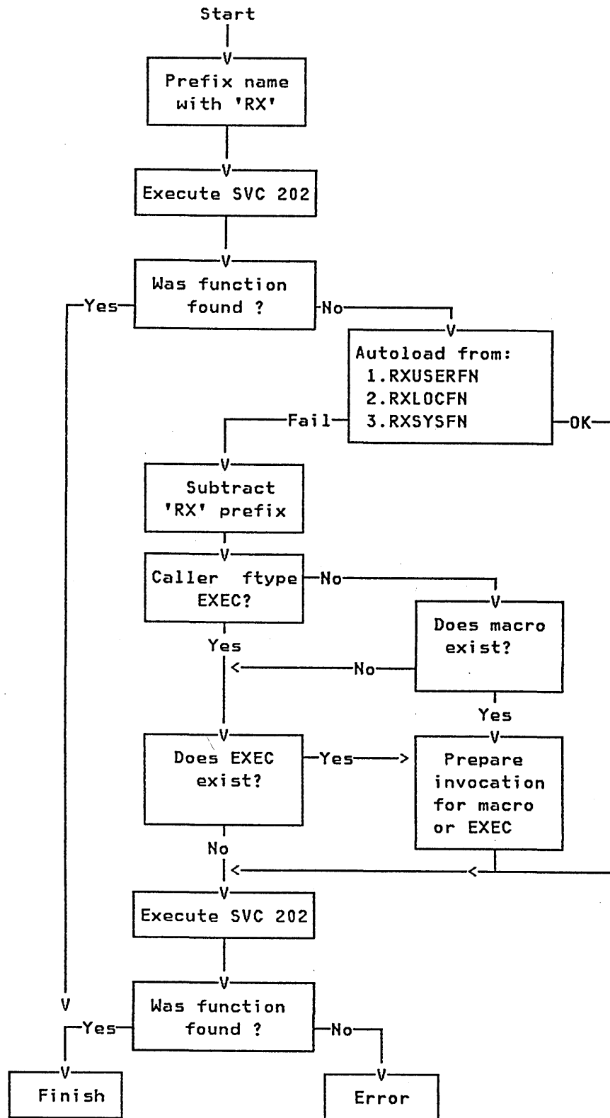
Figure 2. External Routine Resolution and Execution
