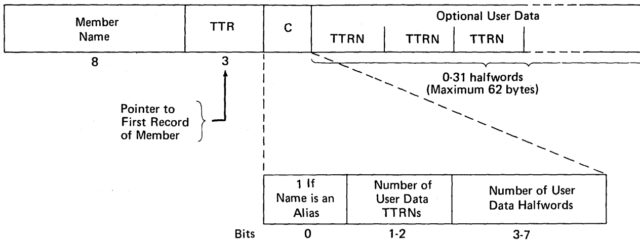
Figure 44. A Partitioned Data Set Directory Entry
