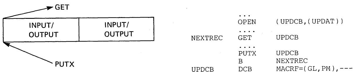
Figure 36. Simple Buffering with MACRF=GL and MACRF=PM-UPDAT Mode
