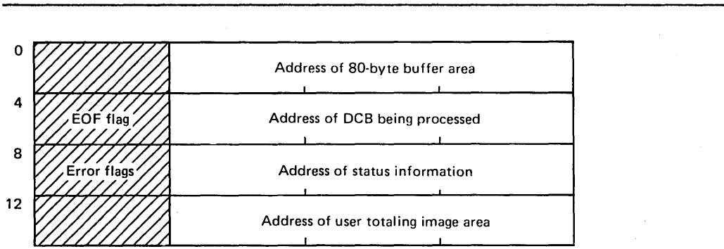
Figure 16. Parameter List Passed to User Label Exit Routine
