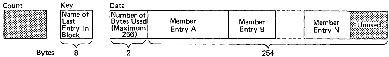
Figure 43. A Partitioned Data Set Directory Block
