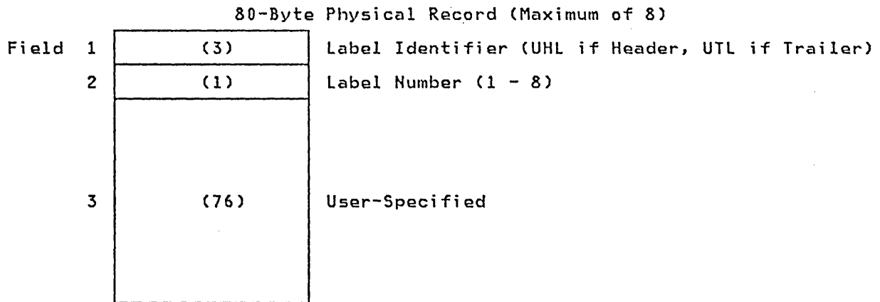
Figure 69. User Header and Trailer Labels
