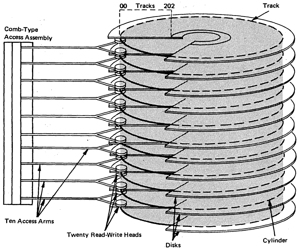
Figure 10. 2316 Disk Pack
