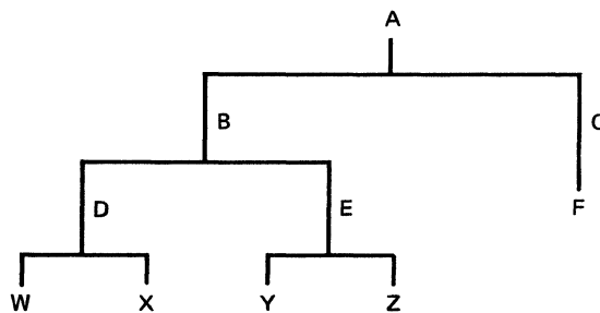
Figure 108. Index Structure—Listed by IEHLIST
