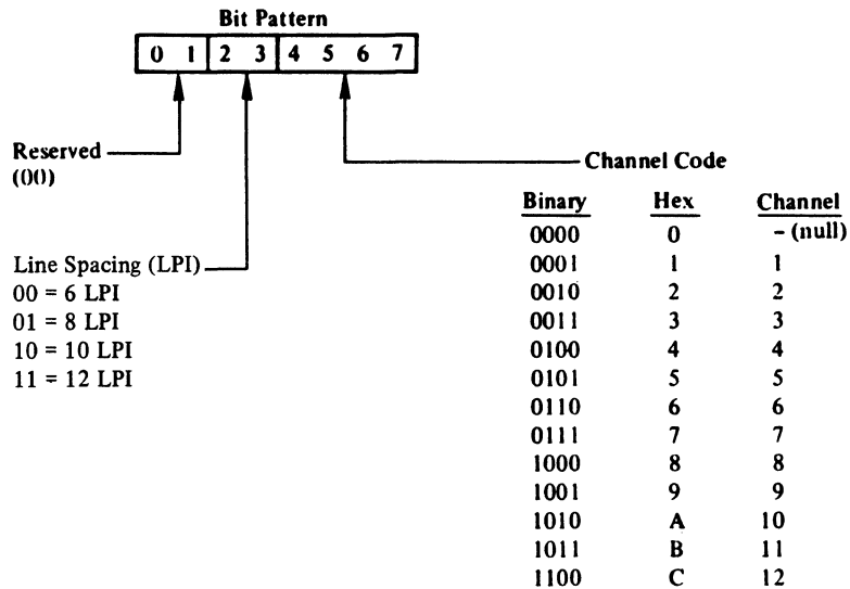
Figure 63. 3800 FCB Module Structure
