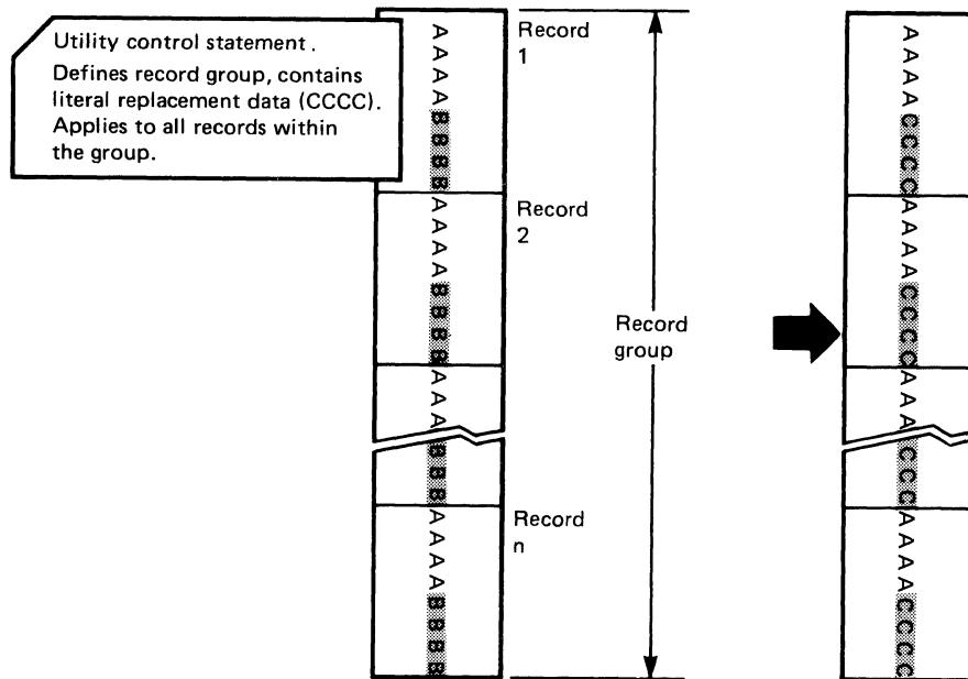
Figure 57. Editing a Sequential Data Set Using IEBGENER
