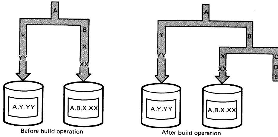
Figure 131. Index Structure Before and After an IEHPROGM Build Operation
