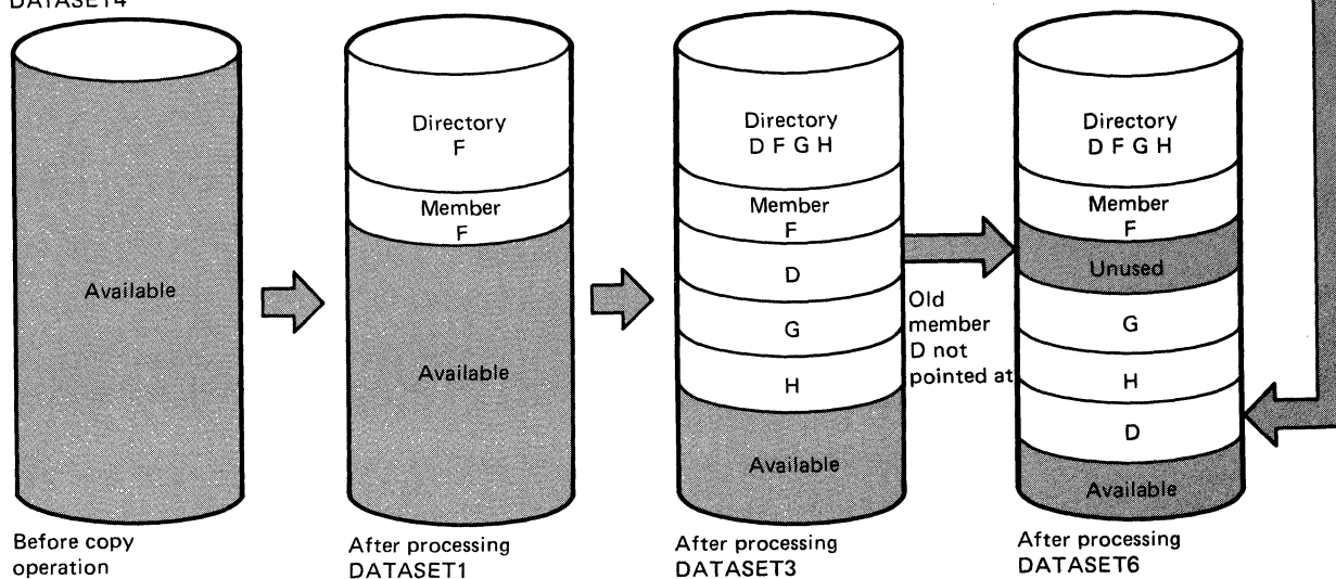
Figure 31. Exclusive Copy with "Replace" Specified for One Input Partitioned Data Set
