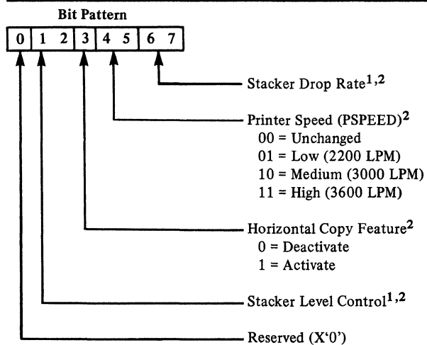
Figure 65. 4248 FCB Module Control Byte
