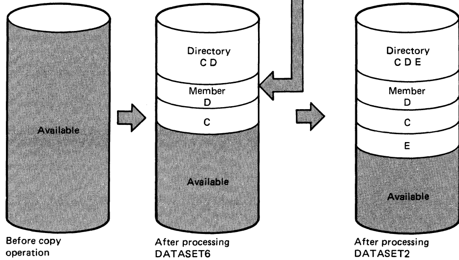
Figure 27. Copying Selected Members with Reblocking and Deblocking
