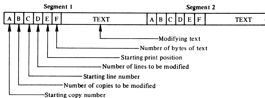
Figure 68. Copy Modification Module Structure
