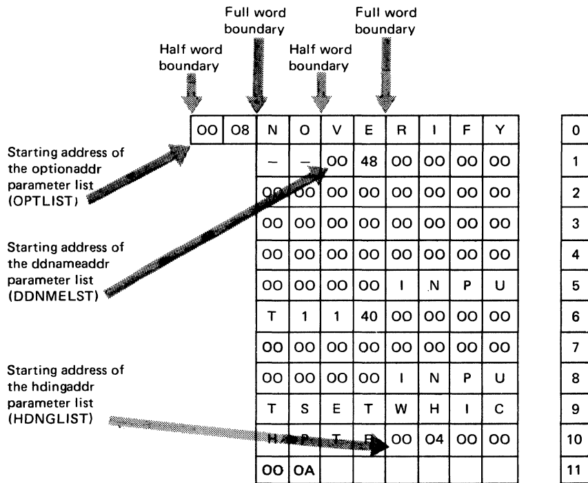
Figure 7. Typical Parameter Lists
