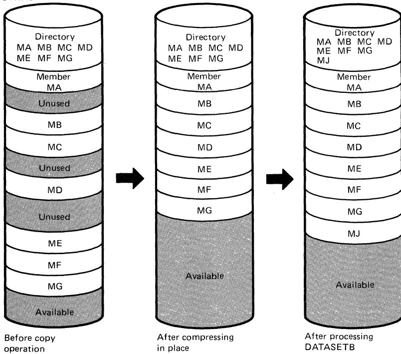
Figure 33 (Part 1 of 2). Multiple Copy Operations/Copy Steps
