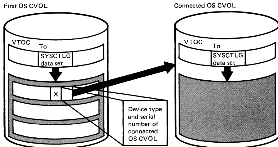
Figure 133. Connecting an OS CVOL to a Second OS CVOL Using IEHPROGM
