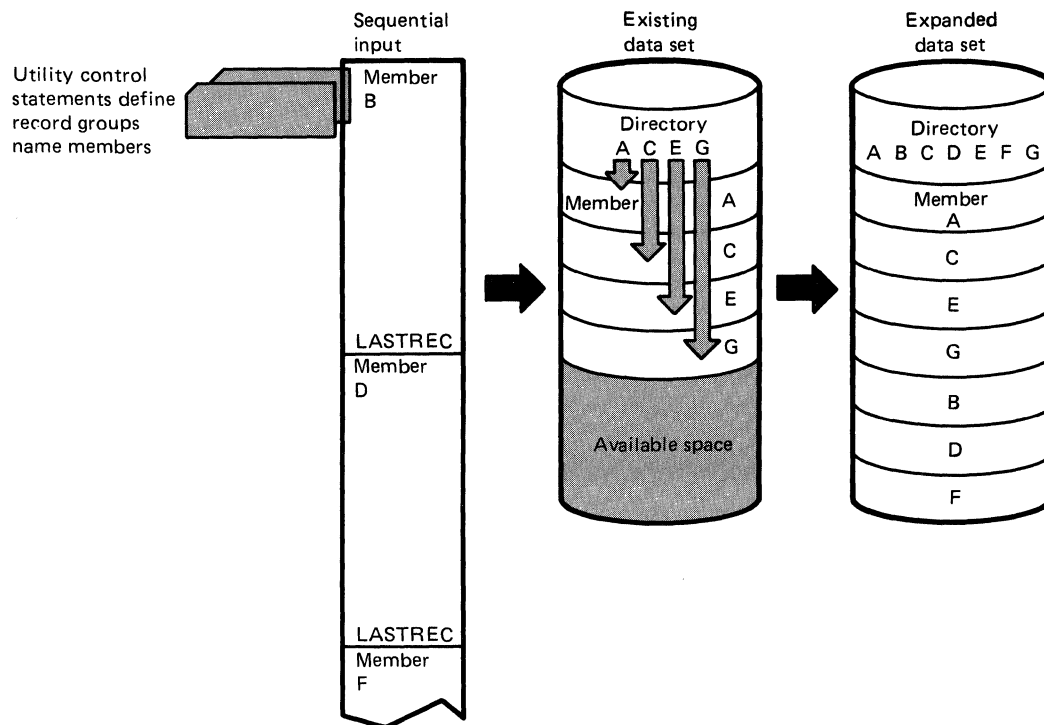
Figure 56. Expanding a Partitioned Data Set Using IEBGENER
