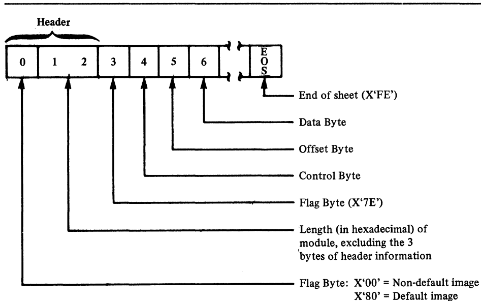
Figure 64. 4248 FCB Module Structure
