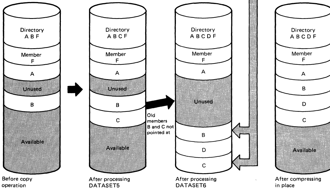
Figure 32. Compress-in-Place Following Full Copy with "Replace" Specified
