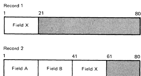
Figure 44. Default Placement of Fields within an Output Record Using IEBDG
