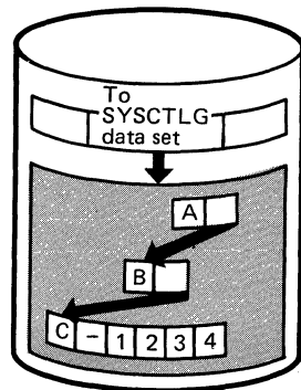
Figure 135. Building a Generation Data Group Index Using IEHPROGM
