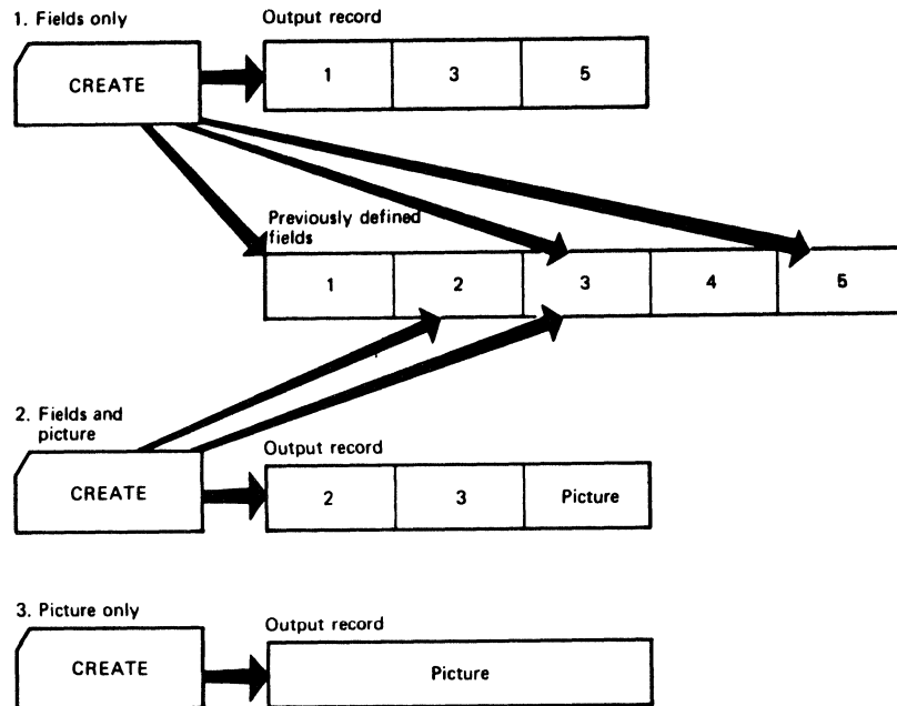
Figure 45. Creating Output Records with Utility Control Statements
