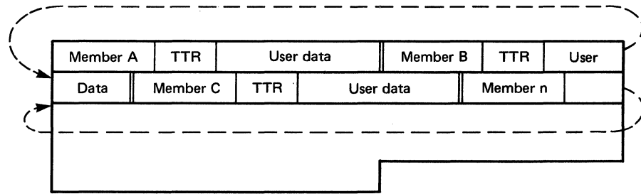
Figure 109. Sample Directory Block
