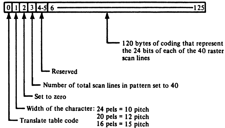
Figure 72. Graphic Character Modification Module Structure
