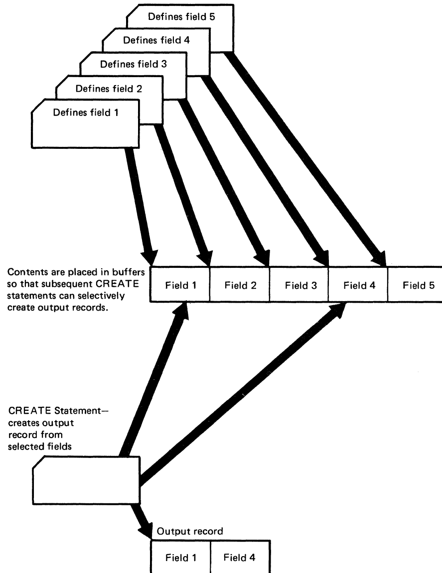
Figure 40. Defining and Selecting Fields for Output Records Using IEBDG
