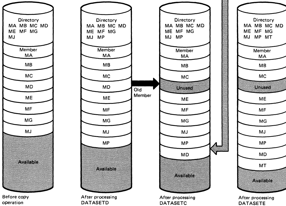
Figure 33 (Part 2 of 2). Multiple Copy Operations/Copy Steps
