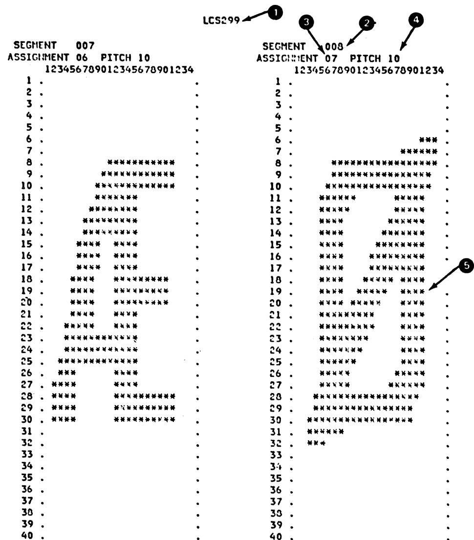
Figure 75. IEBIMAGE Listing of Two Segments of a Library Character Set
