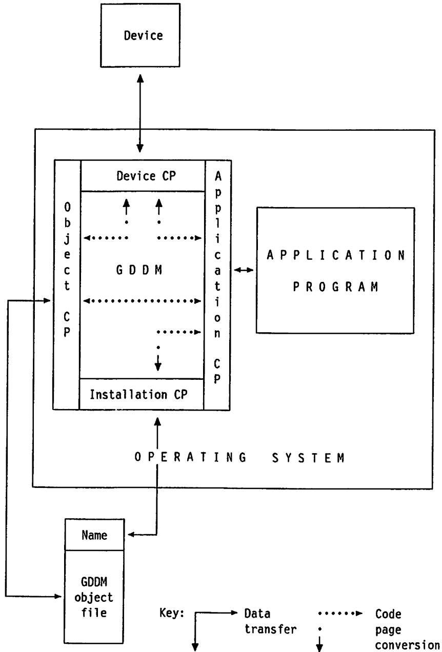
Figure 49. Code page conversion
