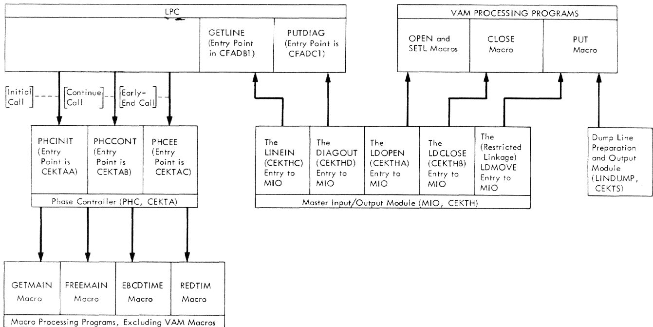
Figure 4. Compiler Interfaces
