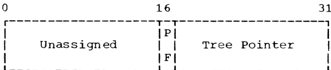
Figure 33. Stack Table Entry
