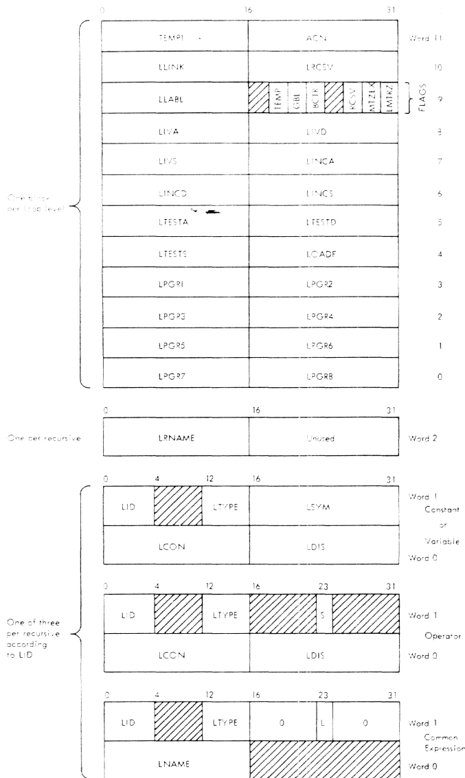
Figure 28. Loop Table
