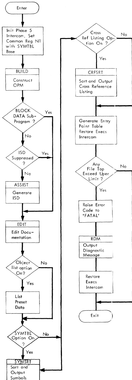
Figure 38. Phase 5 General Flow
