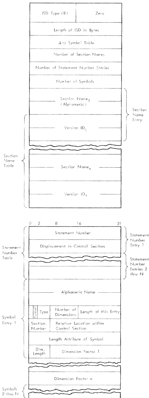
Figure 36. FORTRAN Internal Symbol Dictionary
