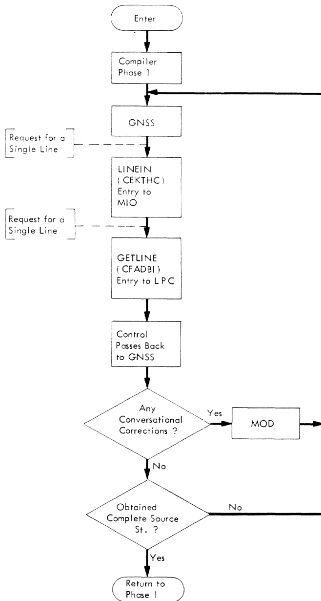
Figure 5. Source-Statement-Preparation Modules
