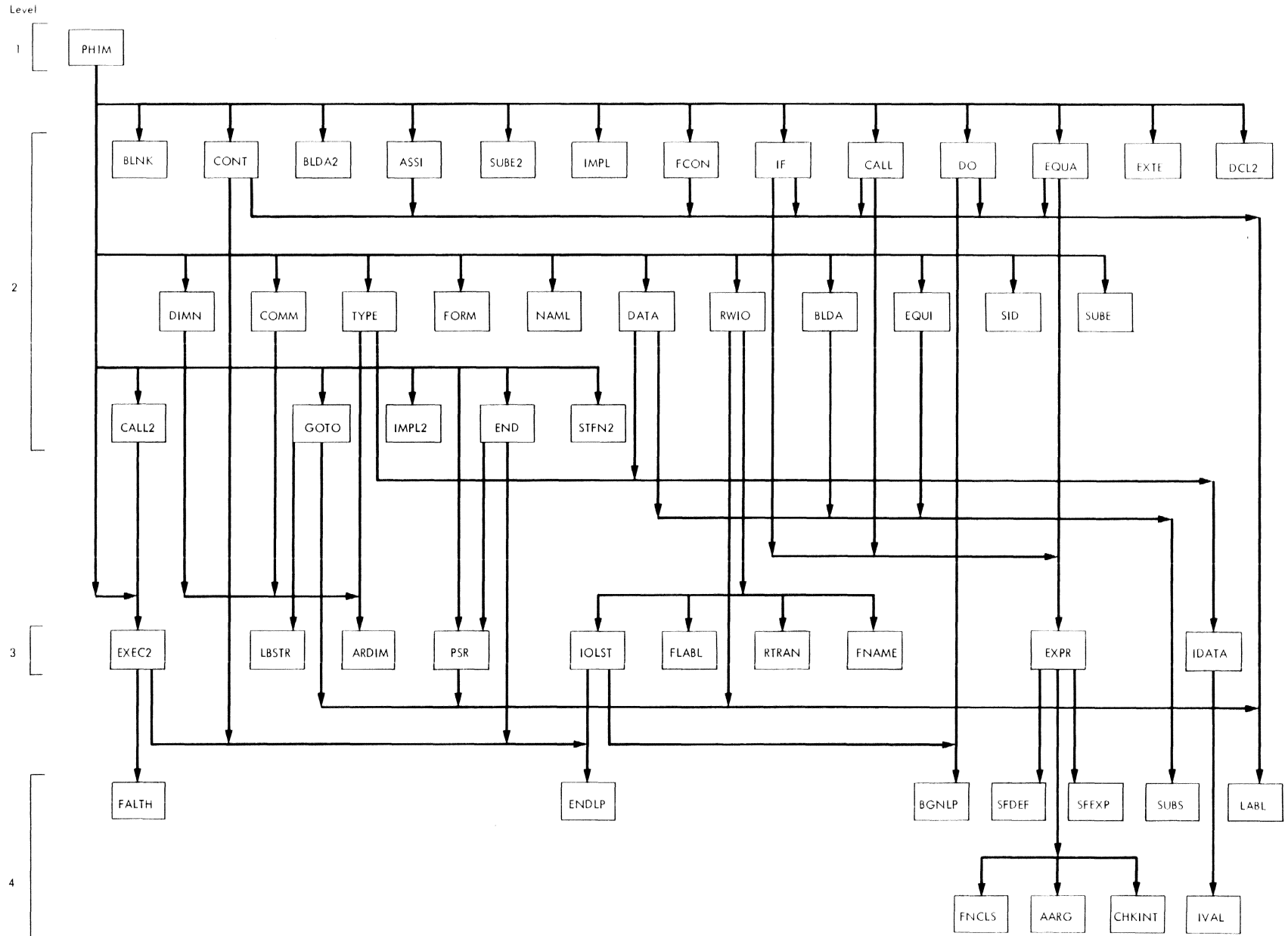
Figure 15. Phase 1 Nesting Chart
