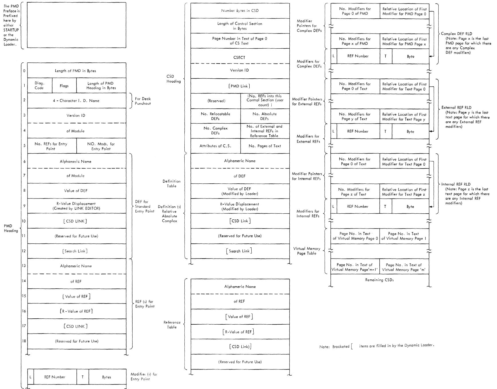
Figure 35. Format of PMD Entry
