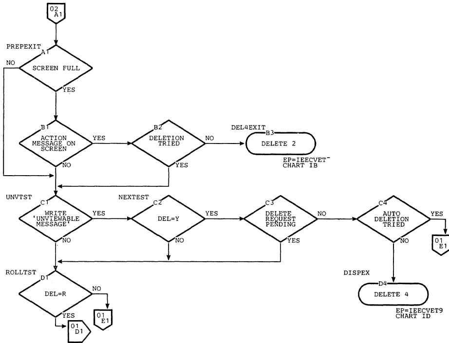
Chart HP. DIOCS Display 2 Routine (Page 2 of 2)
