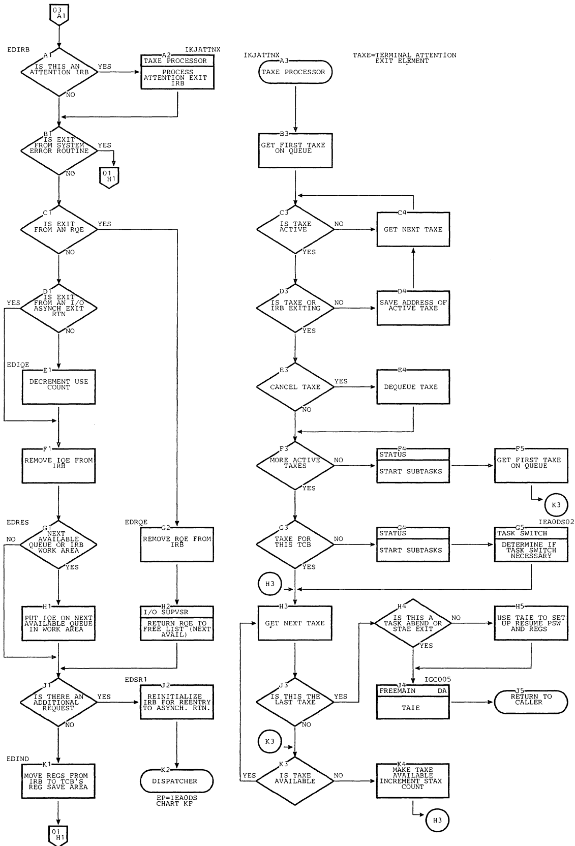
Chart KB. Exit Routine (Page 3 of 3)
