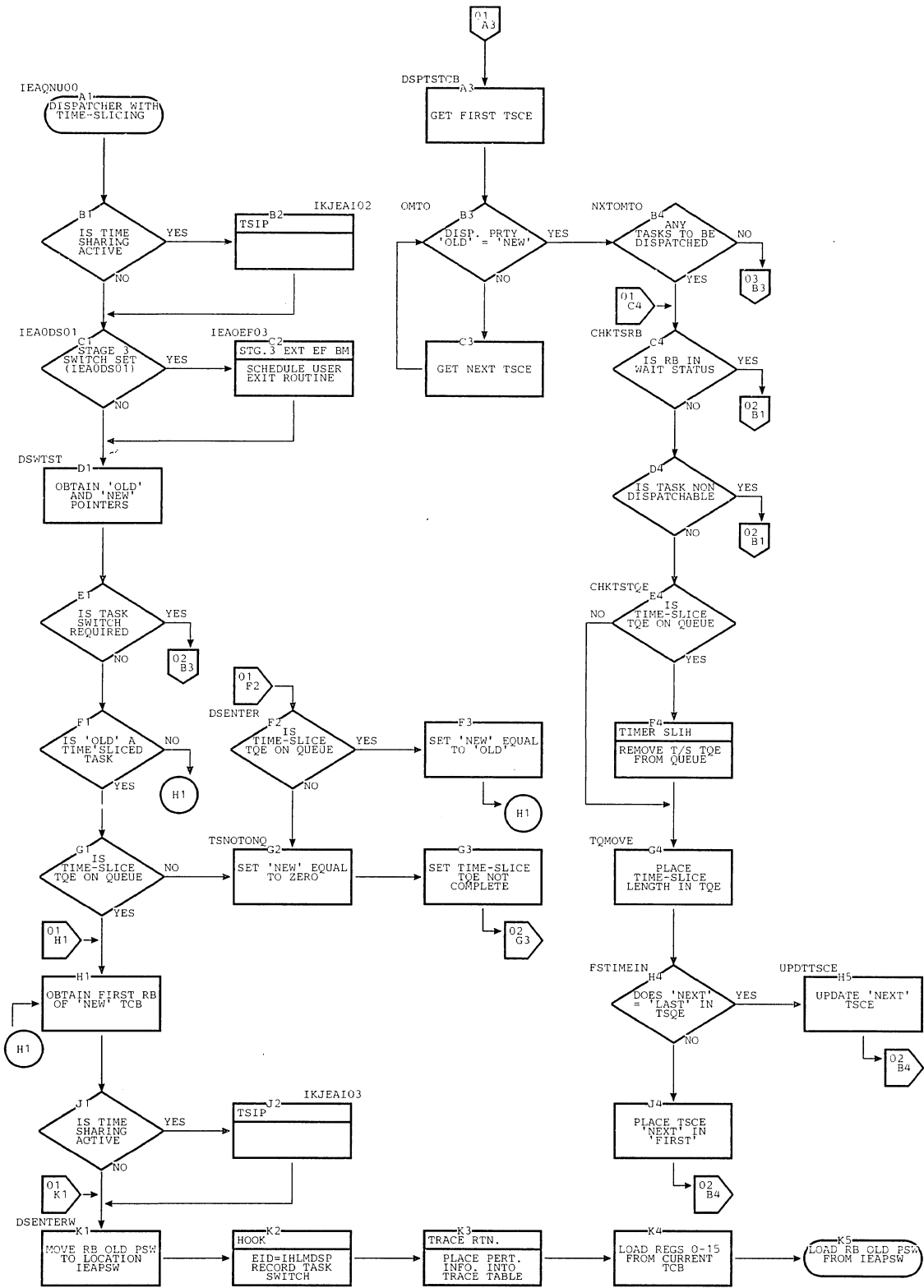
Chart KI. Dispatcher with Time Slicing (Page 1 of 3)
