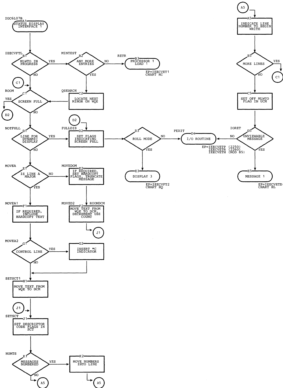
Chart IJ. Status Display Interface 1 Routine
