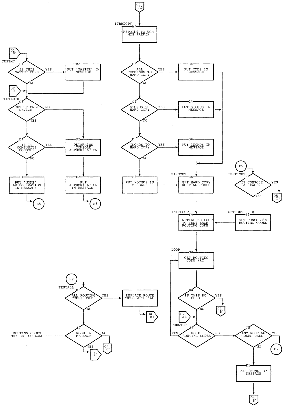
Chart FD. Communications Task Initialization Routine (Page 2 of 5)
