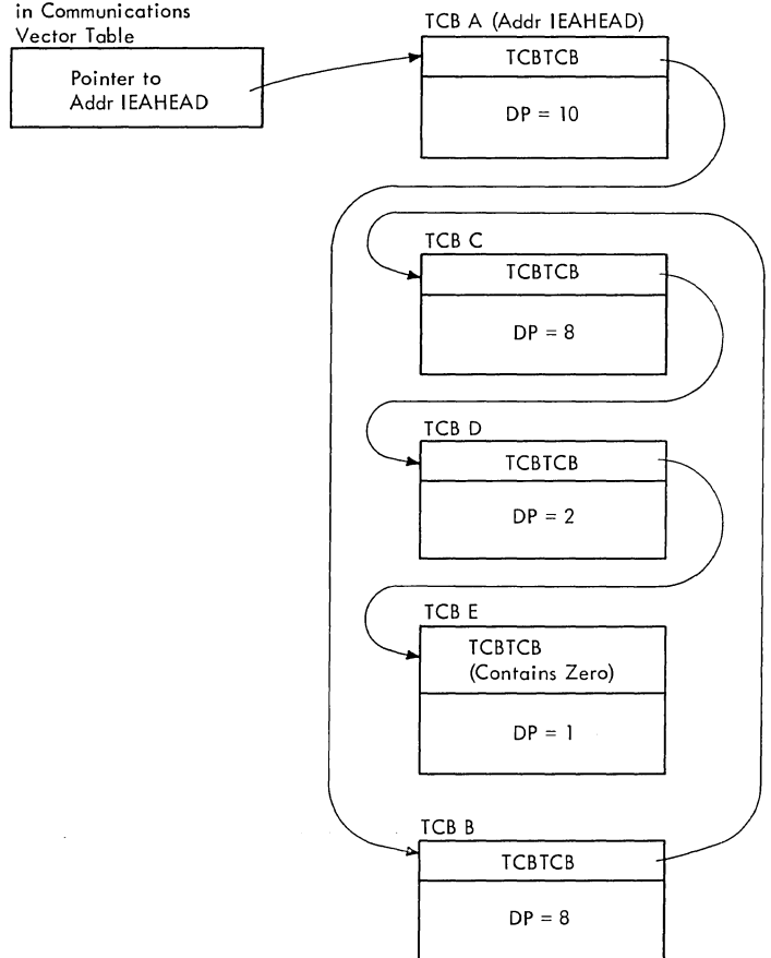
Figure 3-4. The Task Control Block Queue
