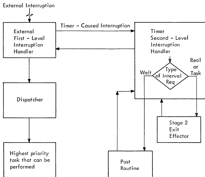
Figure 6-3. Timer Interruption Handling
