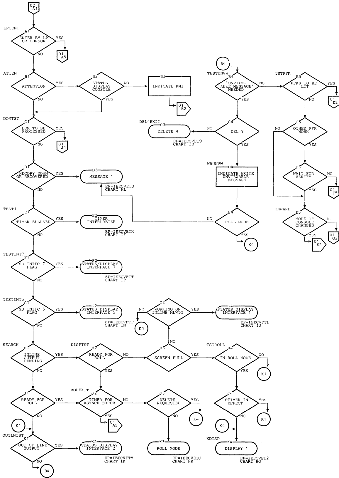
Chart HC. DIDOCS Processor 1, Load 1 (Page 2 of 2)
