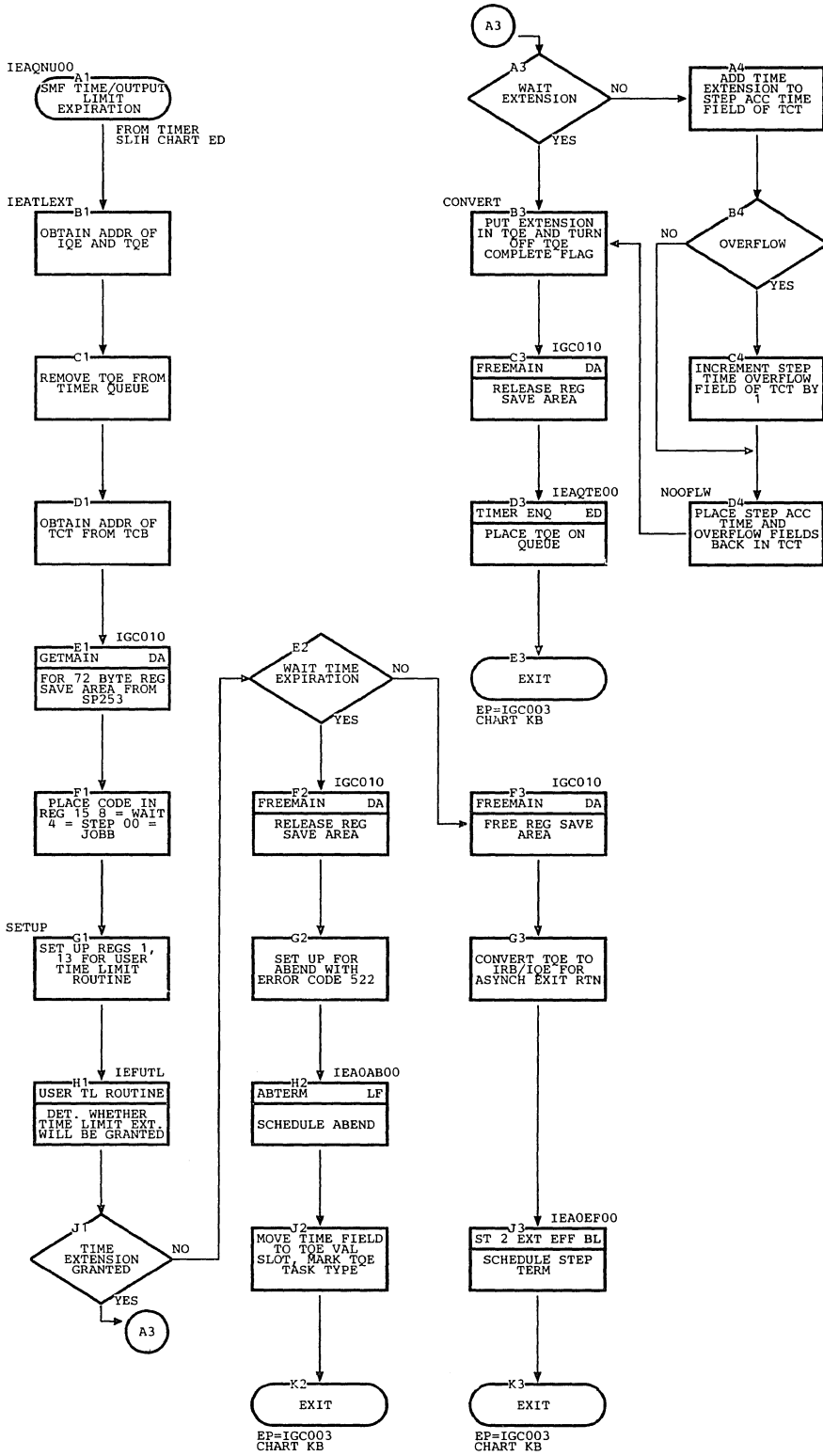
Chart MN. System Management Facility Time/Output Limit Expiration Routine
