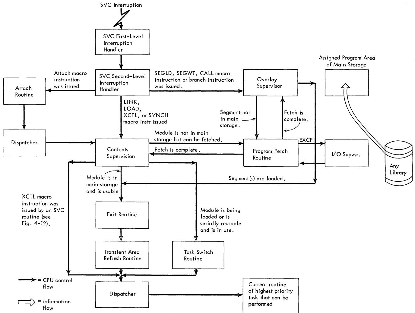
Figure 4-14. Relationship of Program Fetch Routine to Other Routines for the Fetch of a Module or Overlay Segment
