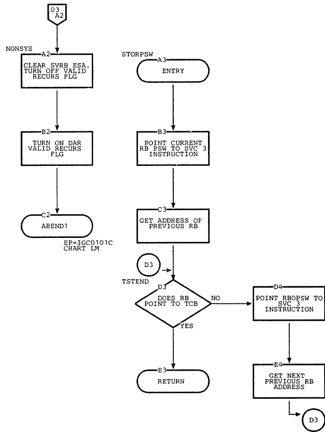
Chart MC. DAR3 (Page 3 of 3)
