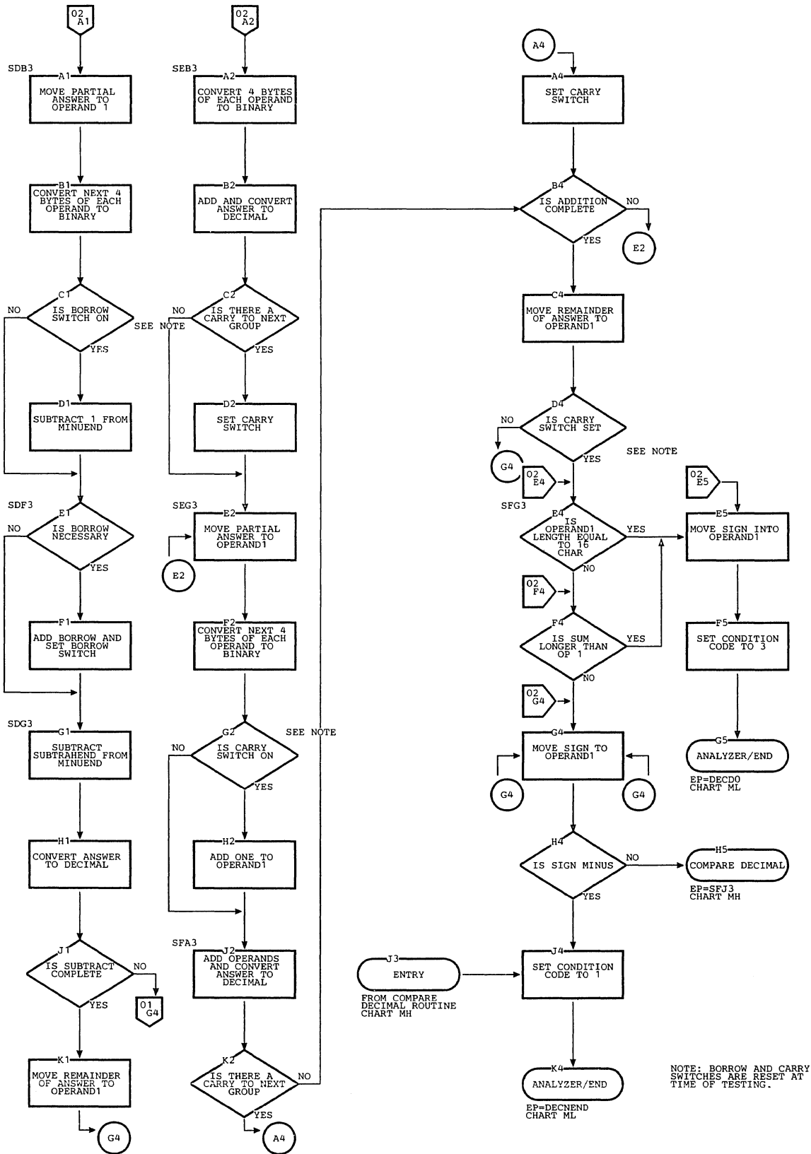
Chart MI. Model 91 Add/Subtract/Zero-and-Add Decimal Routine (Page 2 of 2)
