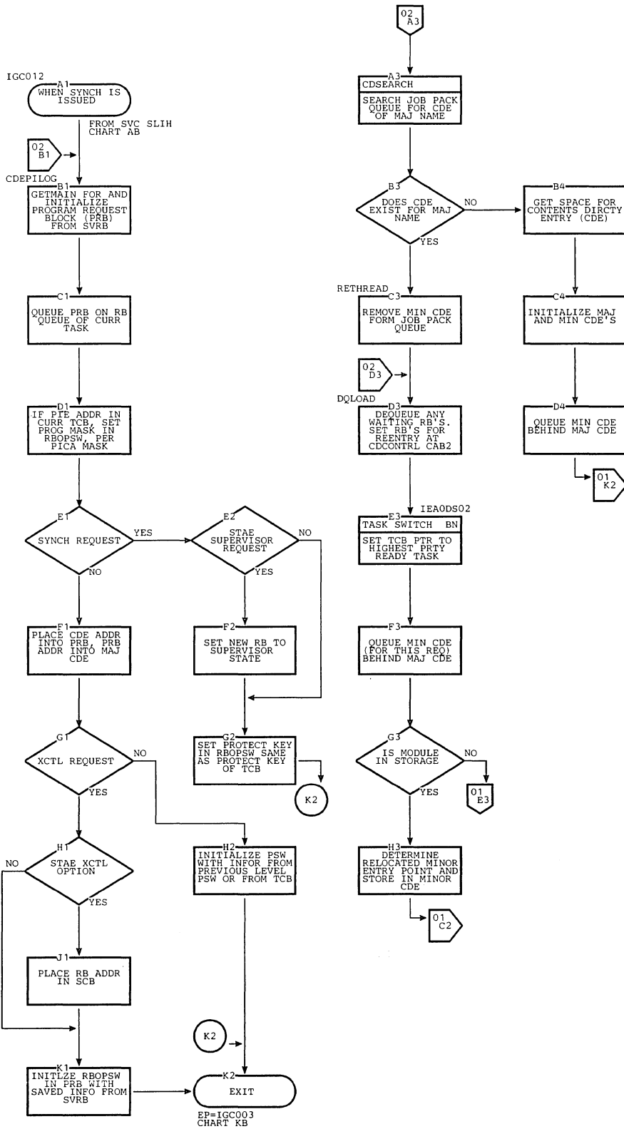
Chart CA. Link, Load, XCTI, and SYNCH Processing (Page 2 of 3)
