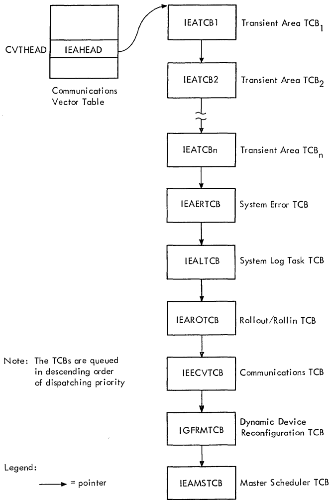
Figure 5-8. Position of Rollout/Rollin TCB on TCB Queue
