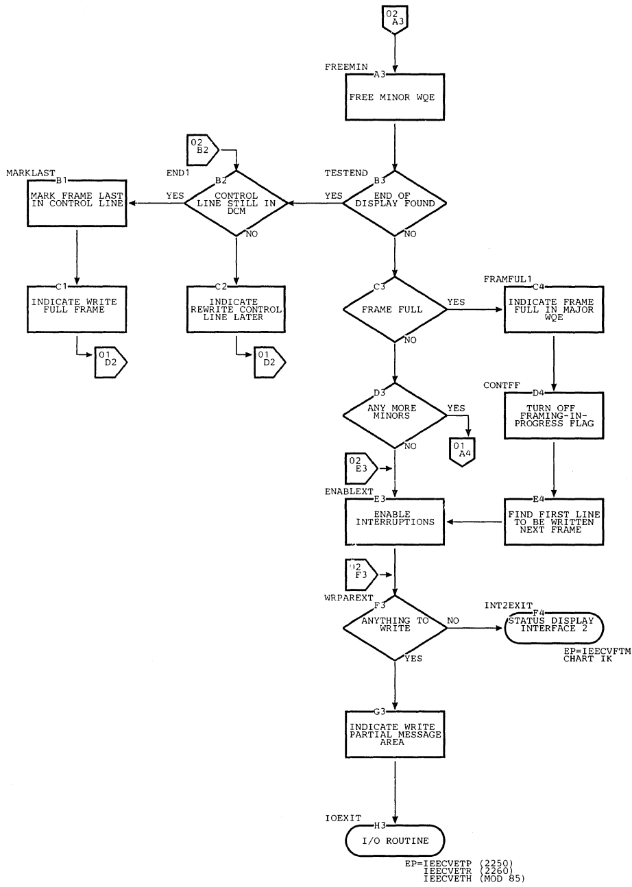
Chart IO. Status Display Interface 6 Routine (Page 2 of 2)
