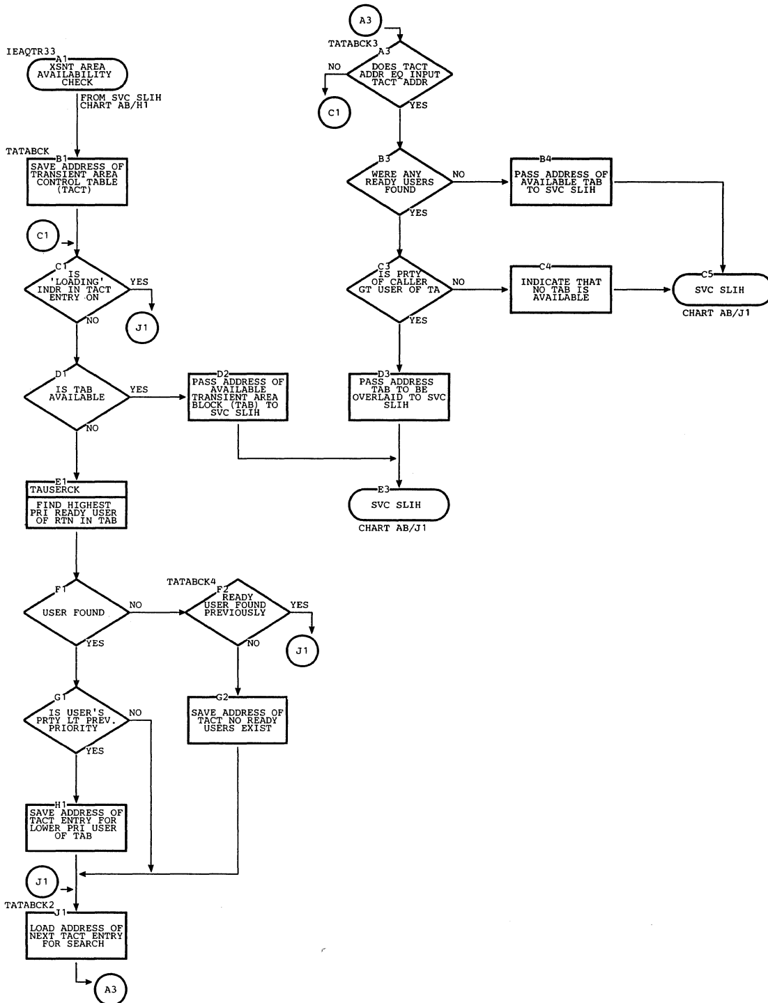
Chart AD. Transient Area Availability Check Routine
