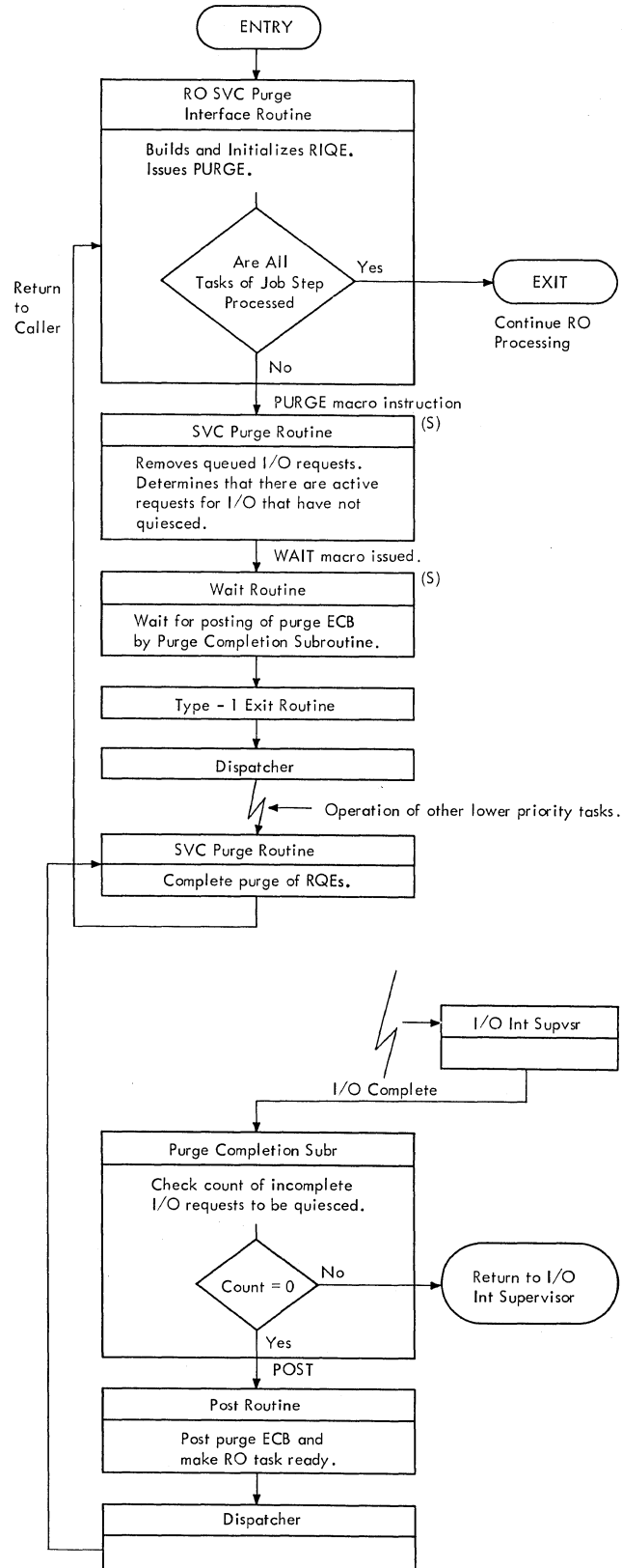
Figure 5-12. Interfaces Between Rollout Module and SVC Purge Routine
