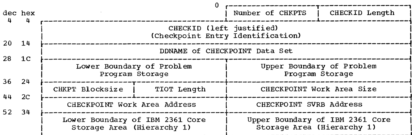
Figure 8-2. CHECKPOINT Header Record (CHR)
