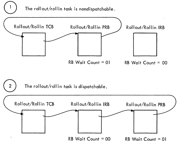
Figure 5-9. Relationship of the Rollout/Rollin TCB, PRB, and IRB During Scheduling of the Rollout/Rollin Task
