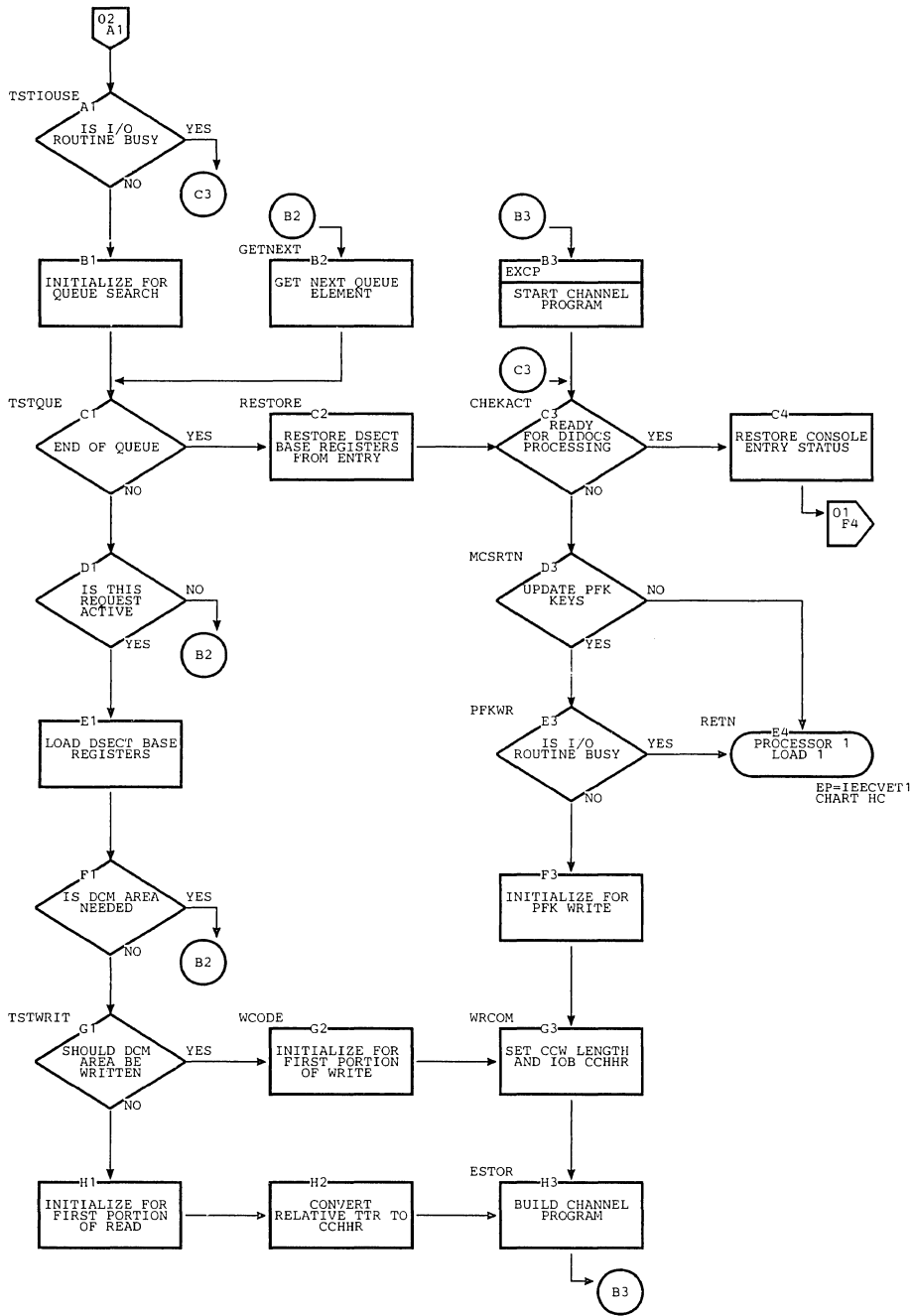
Chart HA. DIDOCs Processor 0, Load 1 (Page 2 of 2)
