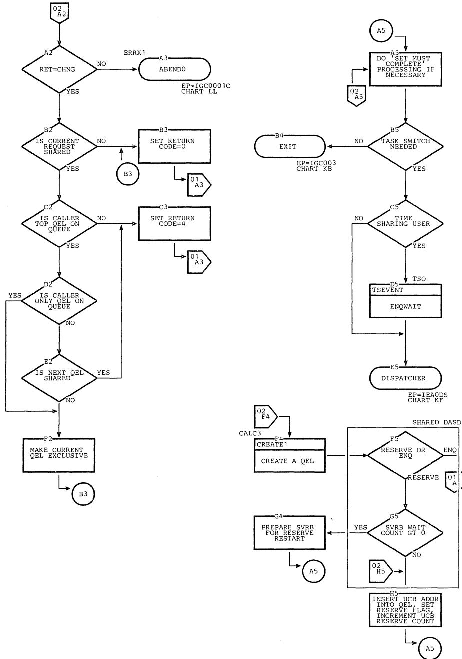
Chart EI. ENQ Routine (Page 2 of 2)
