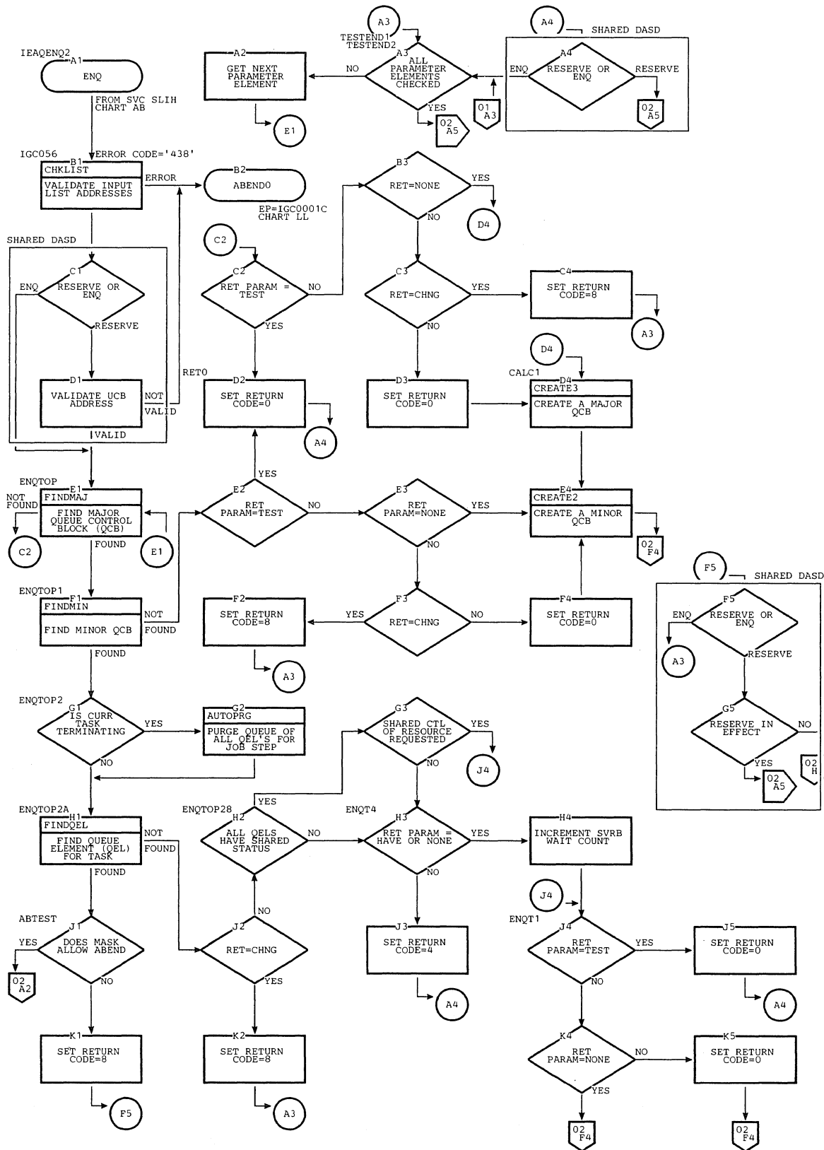
Chart BI. ENQ Routine (Page 1 of 2)
