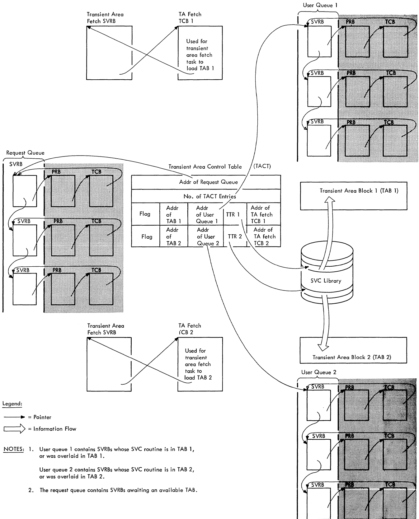
Figure 4-4. The Transient Area Queues
