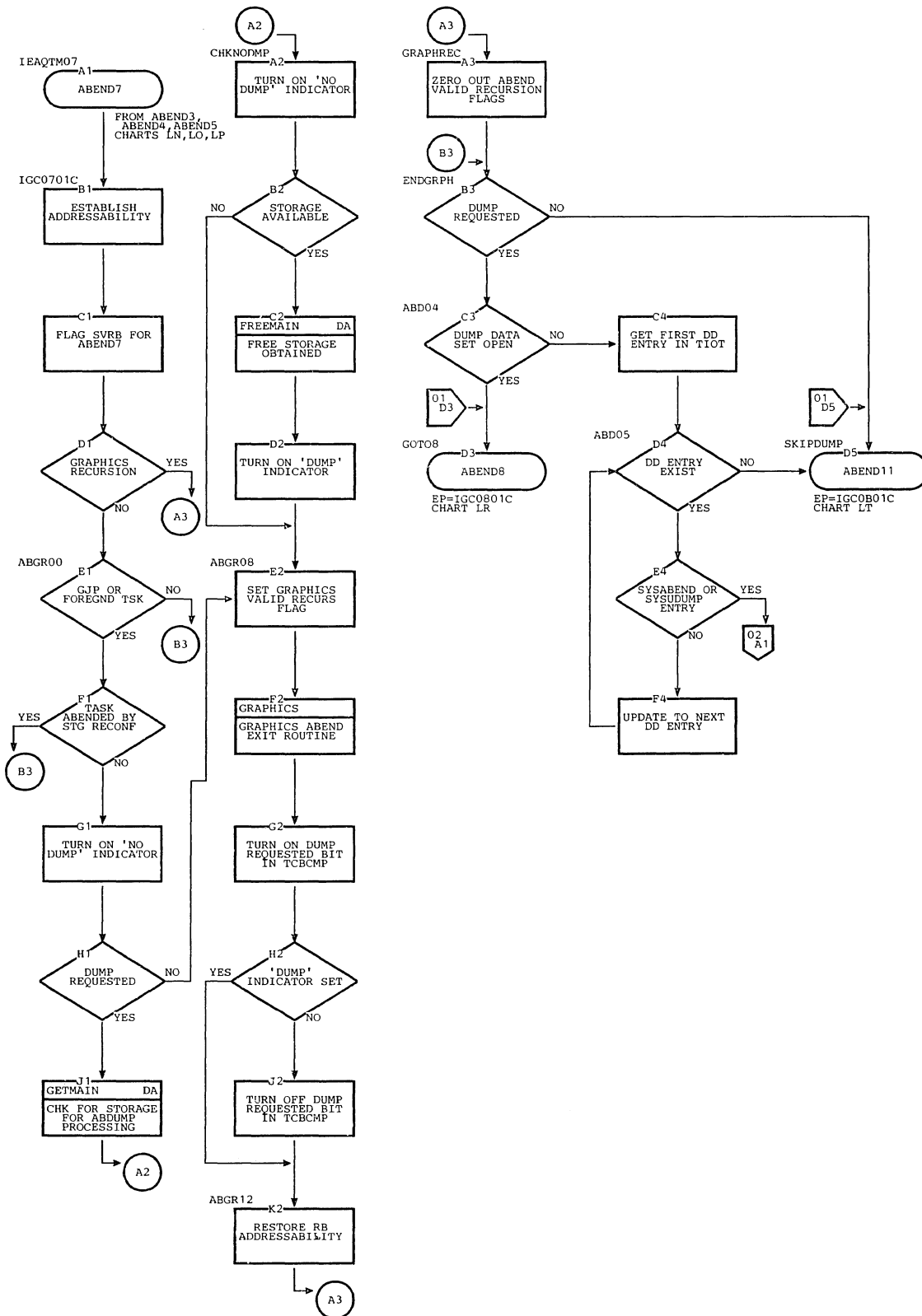
Chart IQ. ABEND7 (Page 1 of 2)
