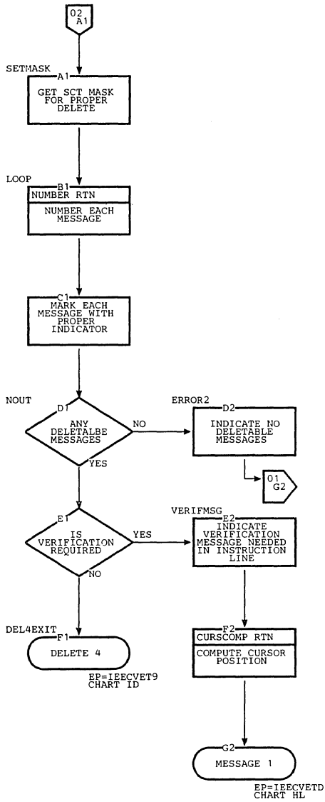
Chart IA. DIDOCS Delete 1 Routine (Page 2 of 2)
