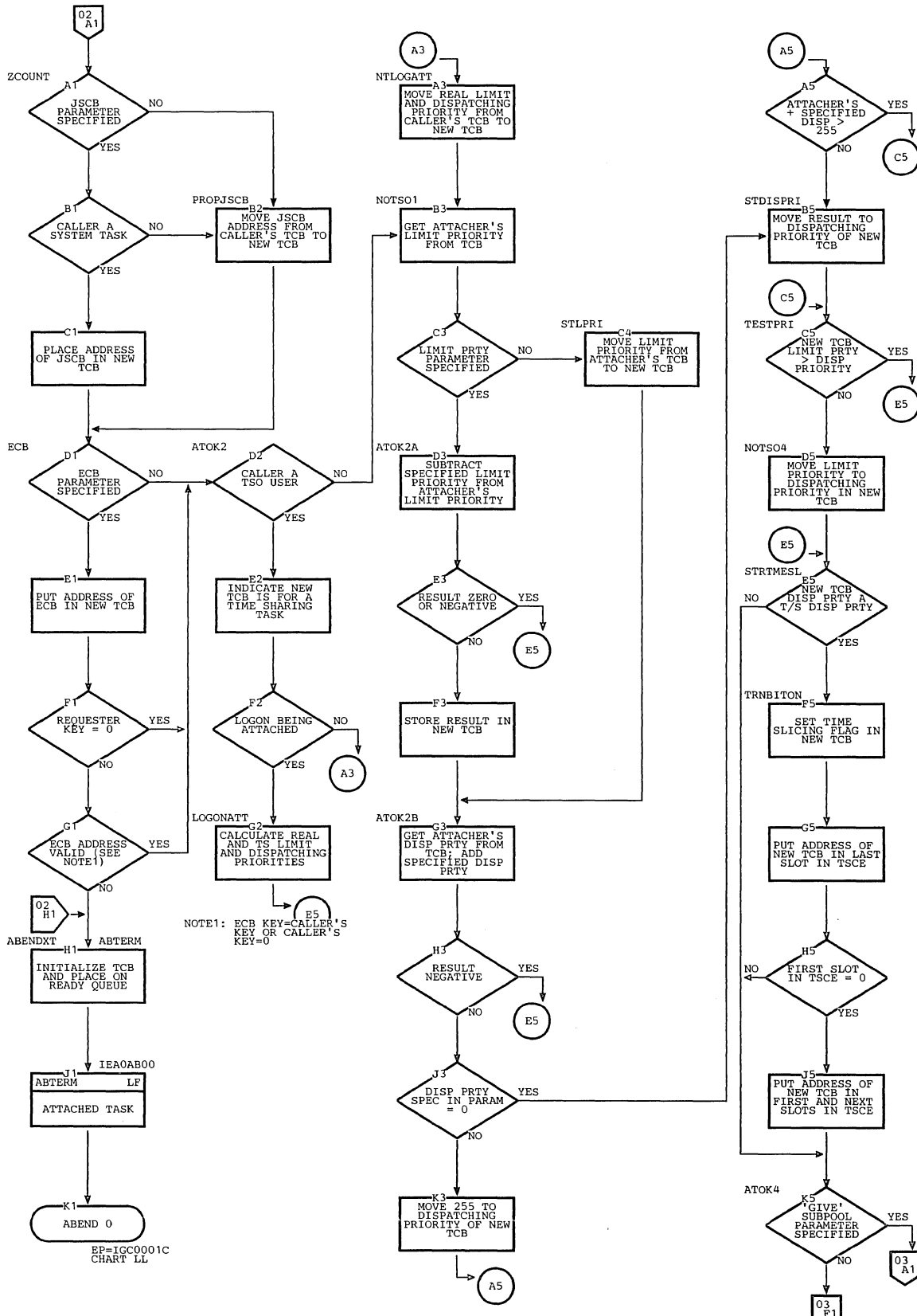
Chart EA. Attach Routine (Page 2 of 4)
