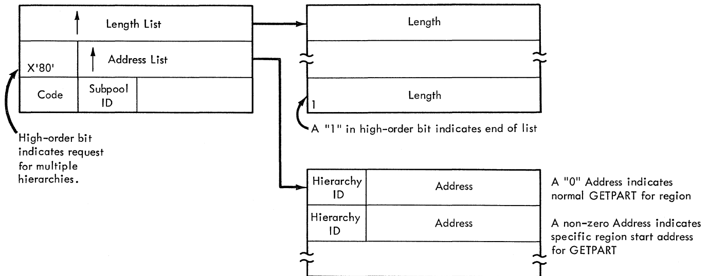
Figure 5-6. List Structure for List Form of GETMAIN (GETPART Module)
