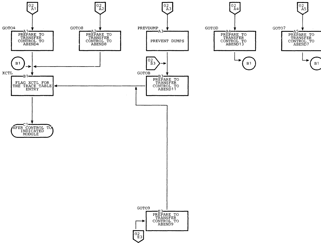
Chart LN. ABEND3 (Page 2 of 2)
