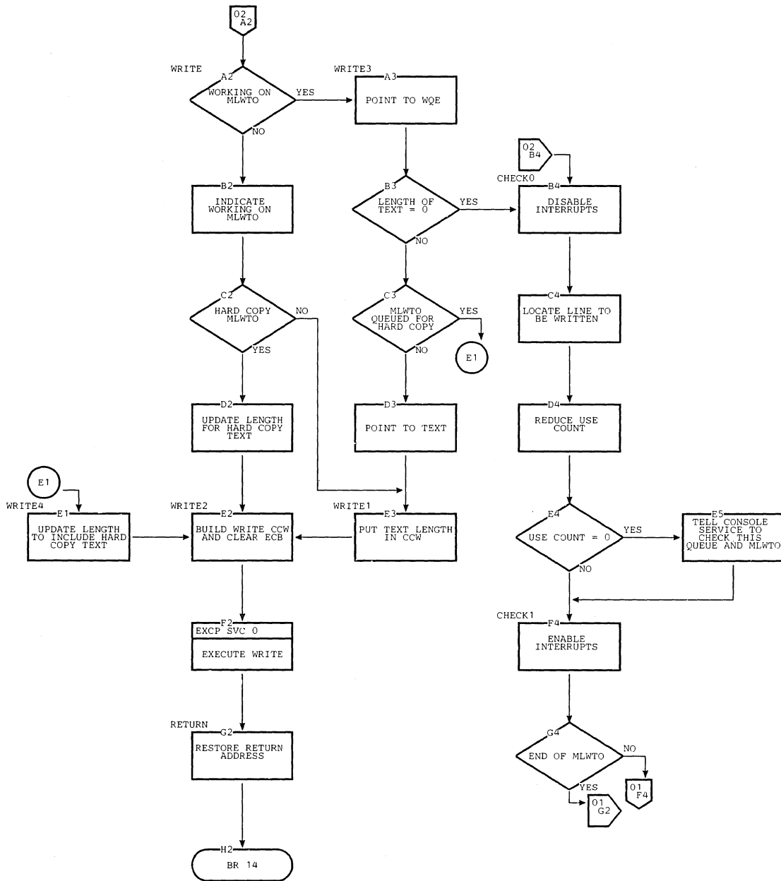
Chart FS. 1052 Processor 2 -- Communications Task with Multiple Console Support (Page 2 of 2)
