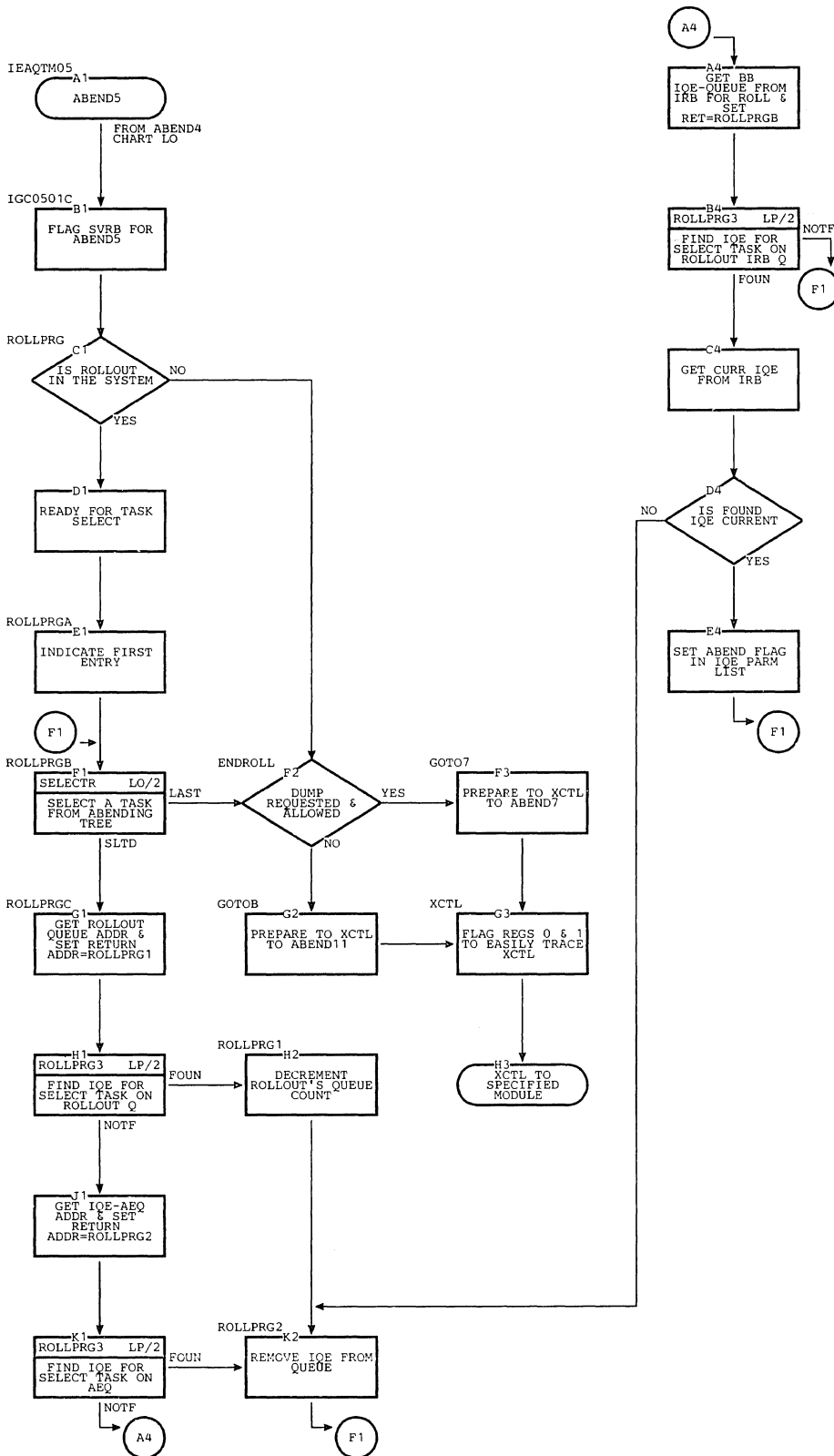
Chart LP. ABEND5 (Page 1 of 2)
