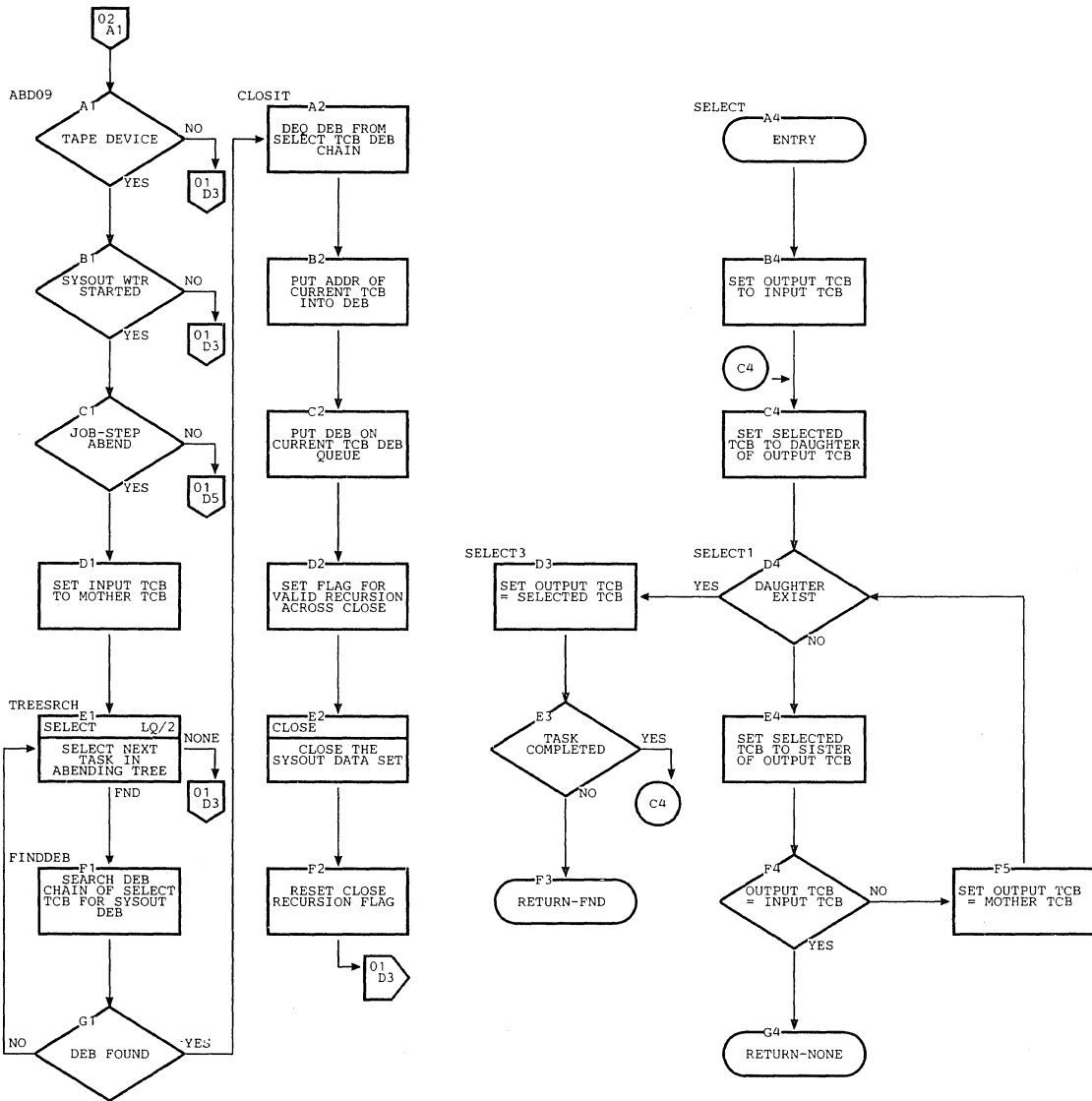
Chart I.Q. ABEND7 (Page 2 of 2)
