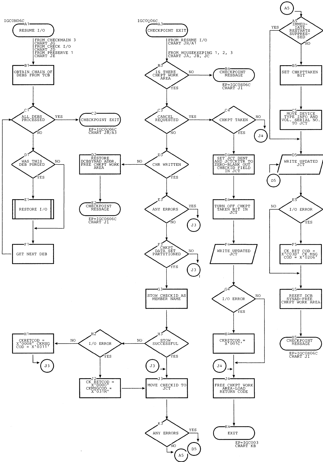
Chart JH. Checkpoint Resume I/O and Exit Routines
