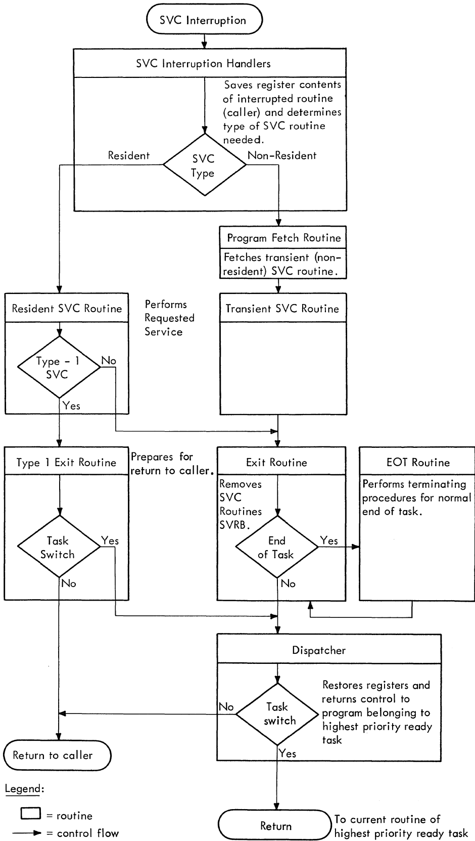
Figure 1-3. Processing After an SVC Interruption
