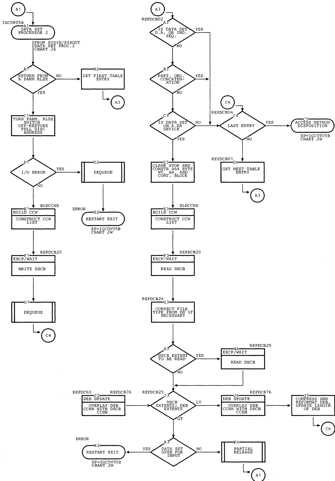
Chart JV. Restart Data Set Processor 2 (Direct Access)
