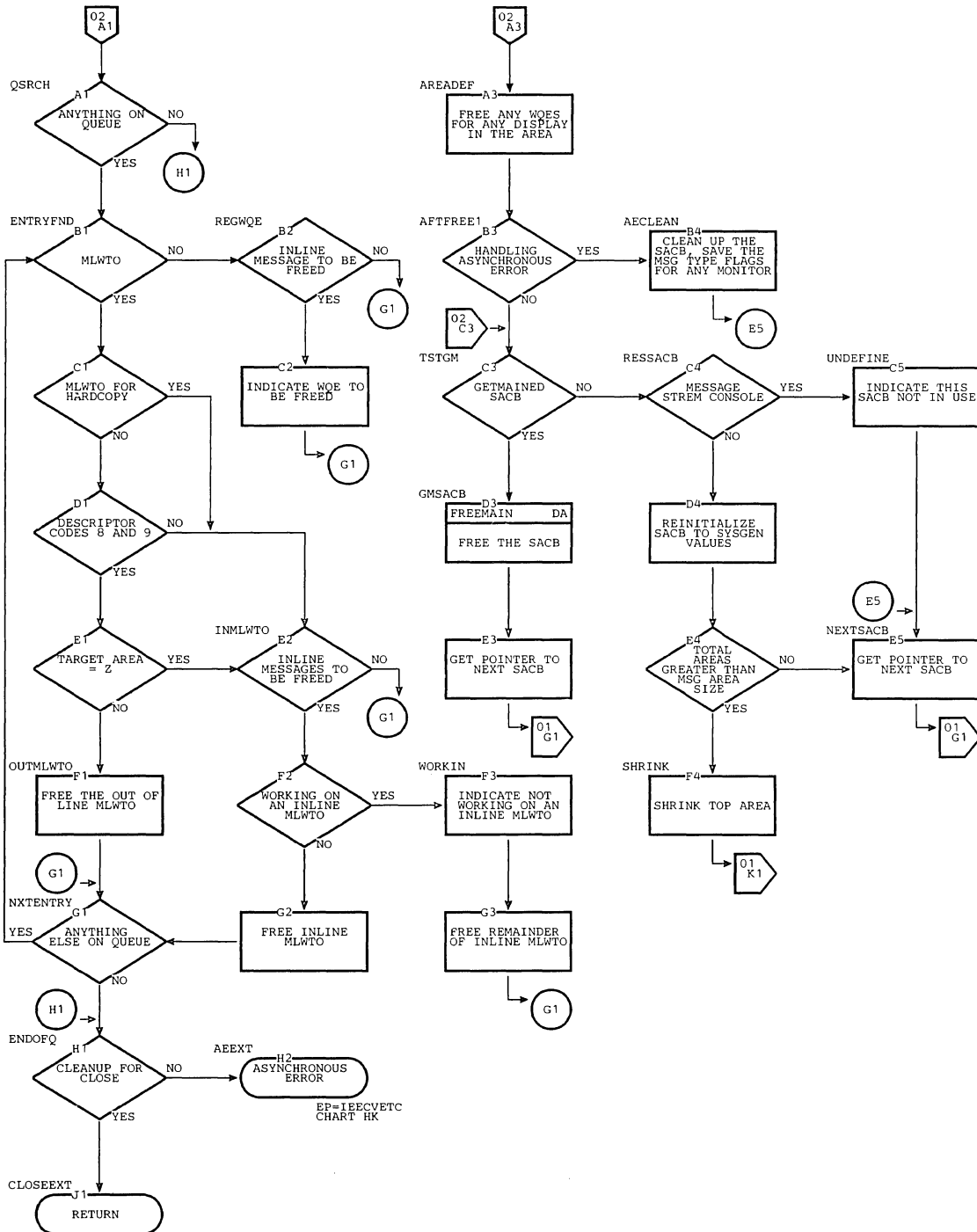
Chart II. DIDOCs Cleanup (Page 2 of 2)
