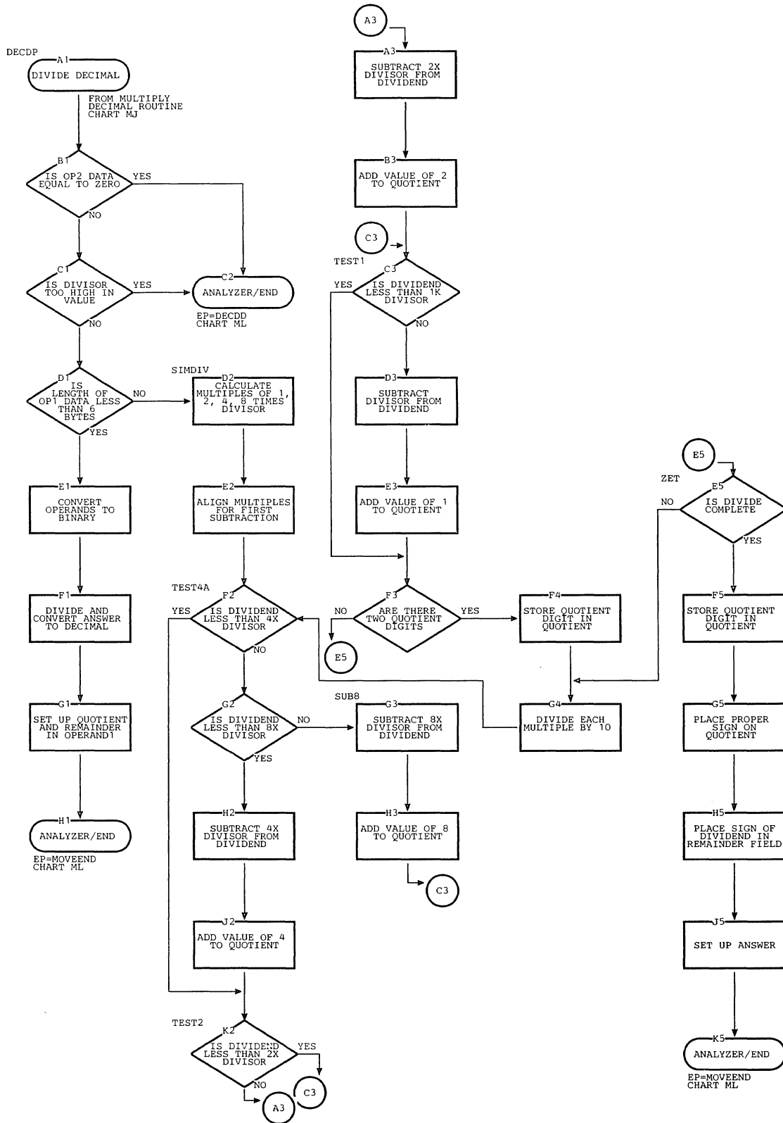
Chart MK. Model 91 Divide Decimal Routine
