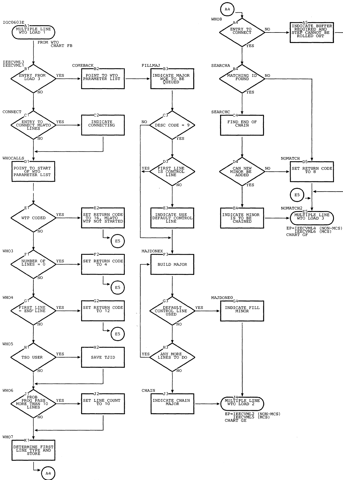
Chart GD. Multiple-Line Write-to-Operator -- Load 1
