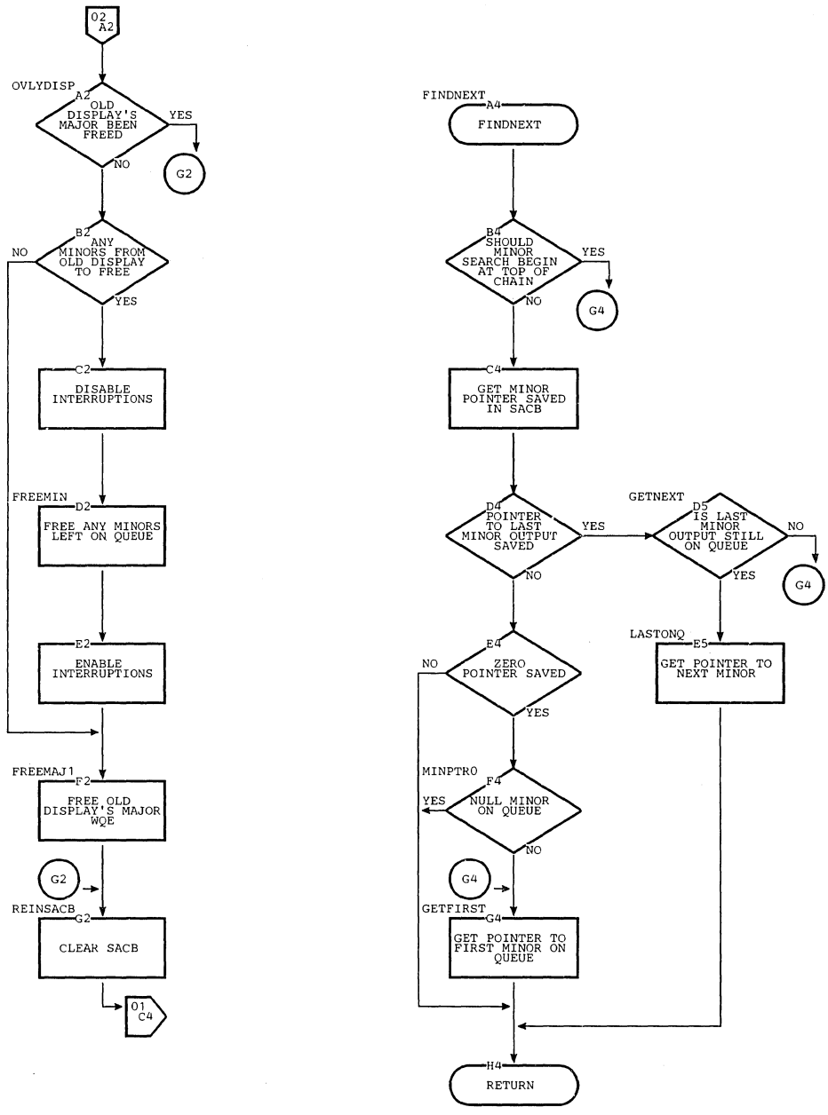
Chart IK. Status Display Interface 2 Routine (Page 2 of 2)
