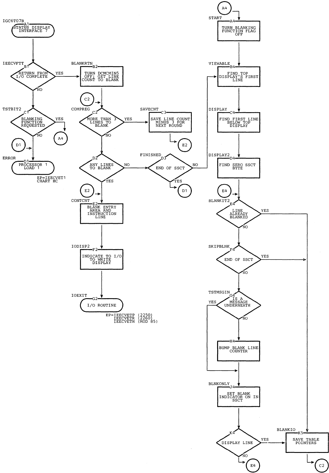
Chart IP. Status Display Interface 7 Routine
