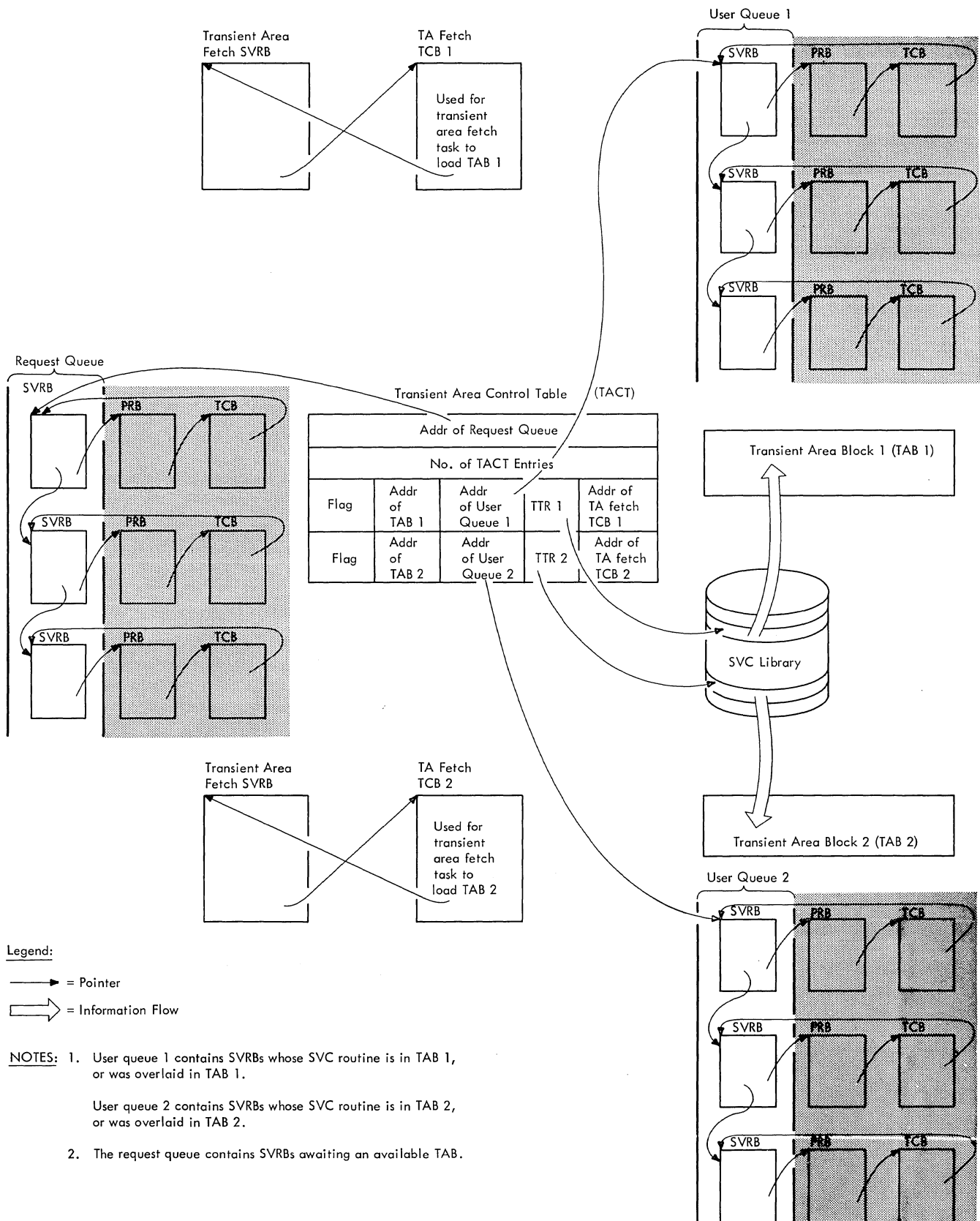
Figure 2-3. The Transient Area Queues
