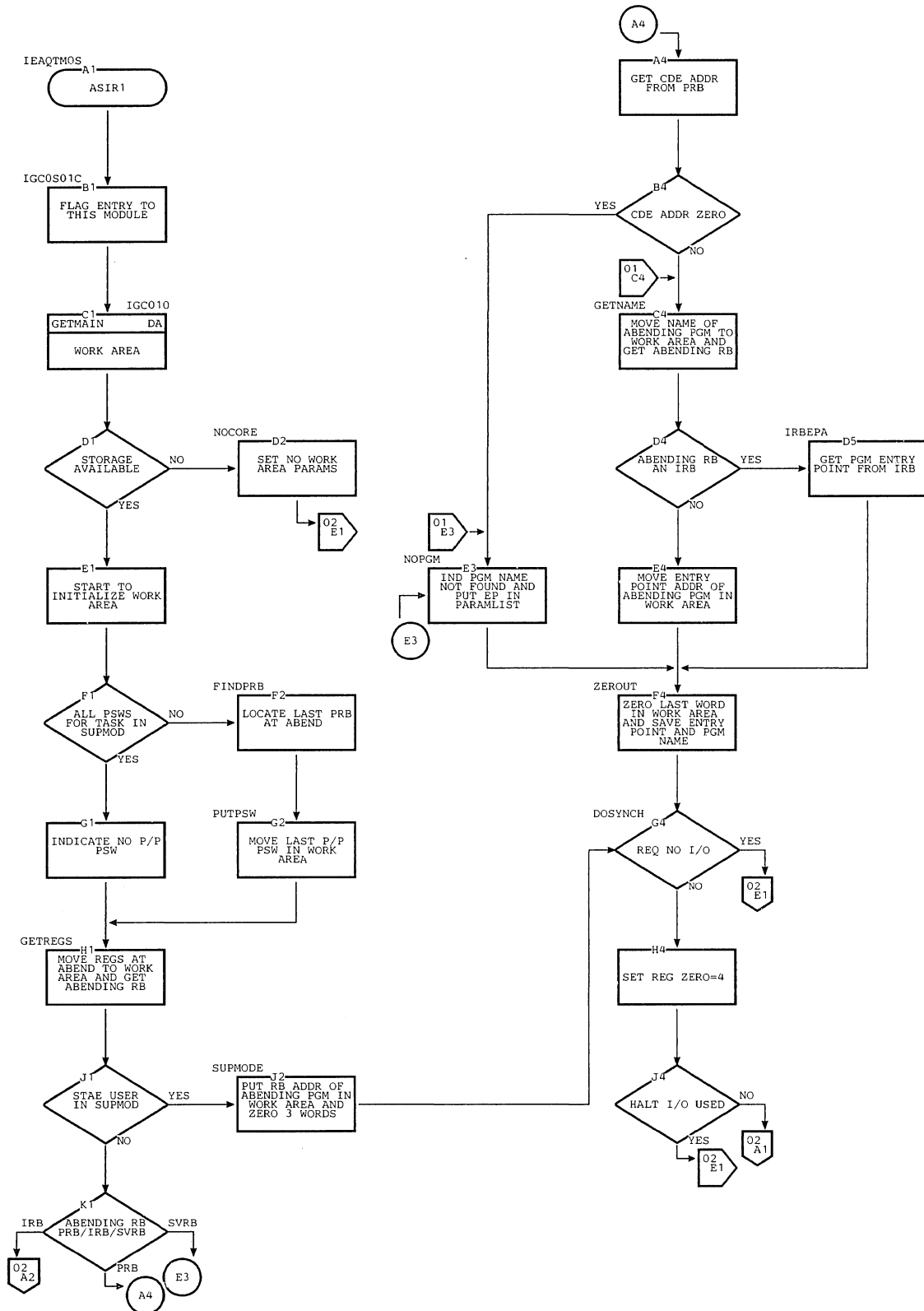
Chart BR. ABEND/STAE Interface 1 Routine (ASIR1) (Page 1 of 2)
