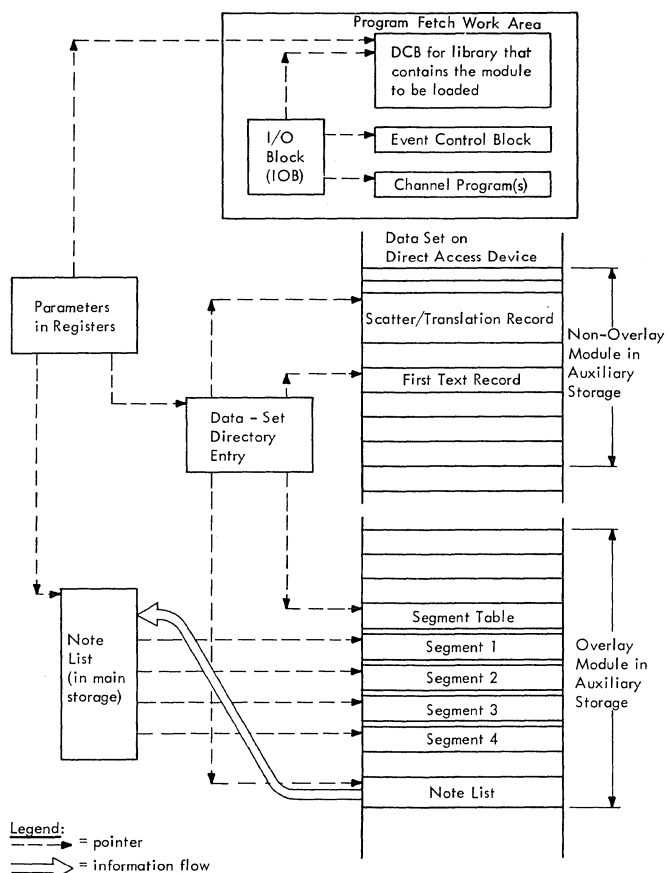
Figure 4-13. Control Blocks and Tables Used by the Program Fetch Routine
