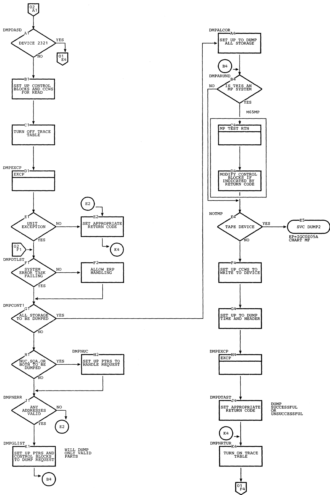
Chart ME. SVC DUMP 1 (Page 2 of 2)
