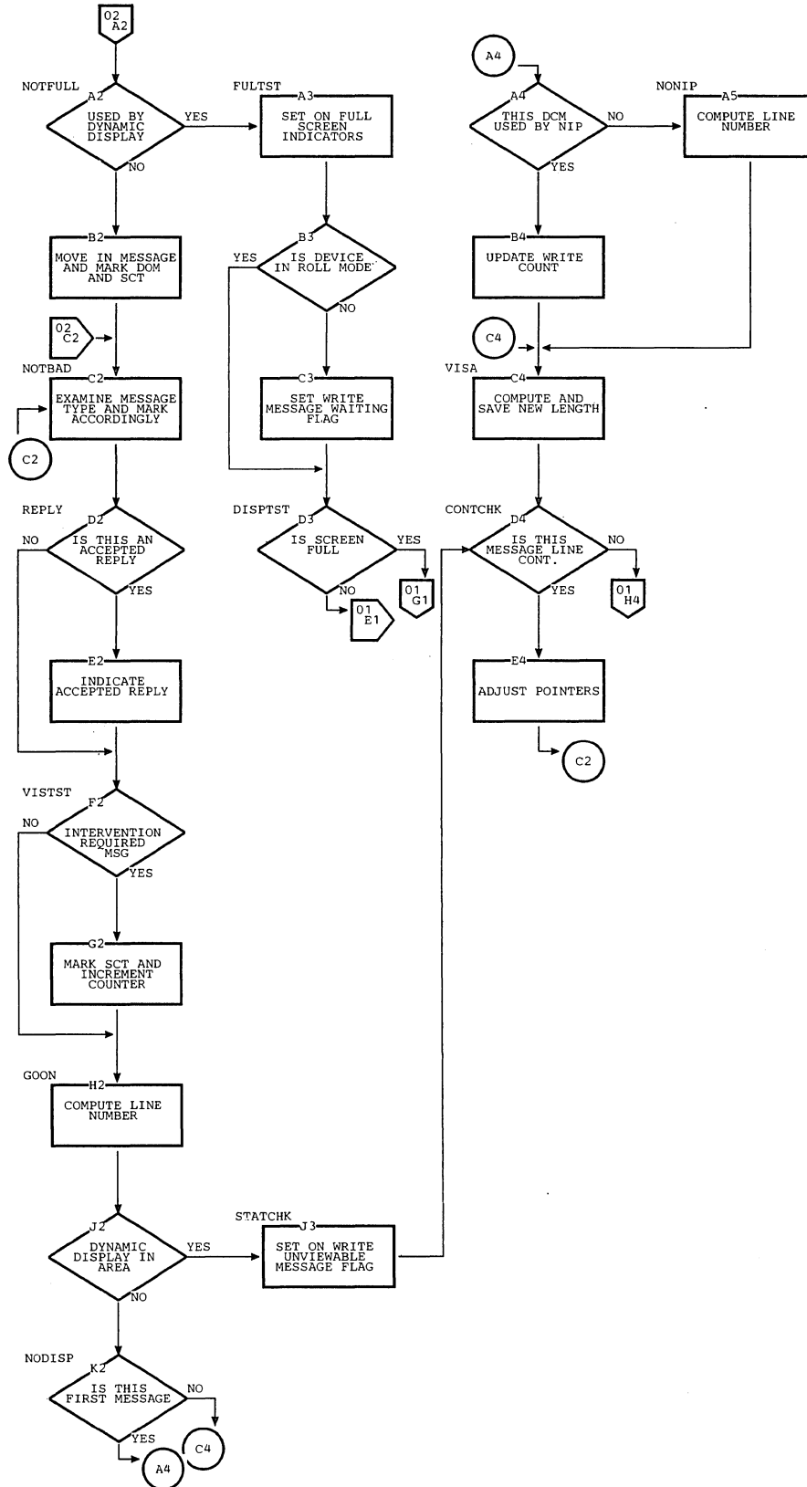
Chart HQ. DIDOCS Display 3 Routine (Page 2 of 2)
