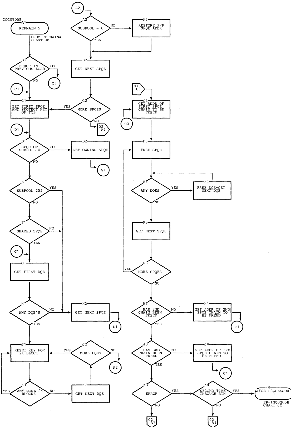
Chart JN. Restart Repmain 5 Routine (Page 1 of 2)
