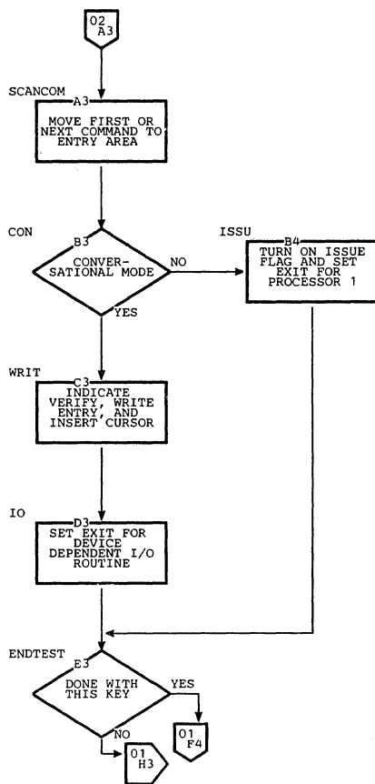
Chart IG. DIDOCS PFK 1 Routine (Page 2 of 2)
