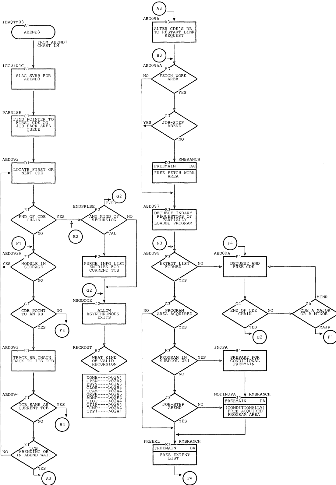
Chart LN. ABEND3 (Page 1 of 2)
