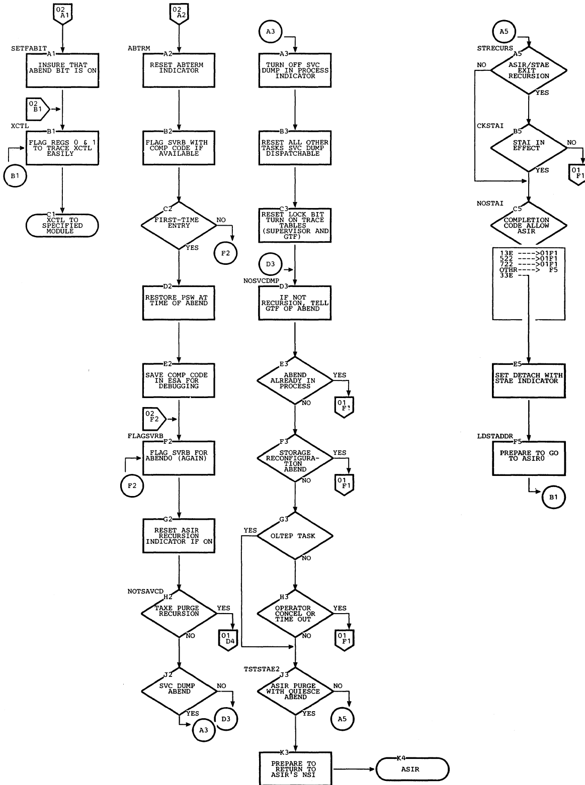
Chart LL. ABEND0 (Page 2 of 3)
