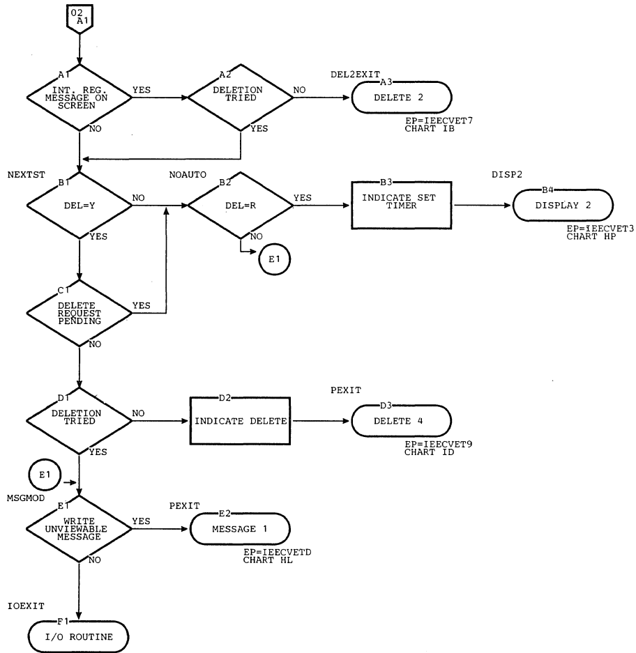
Chart HO. DIDOCS Display 1 Routine (Page 2 of 2)
