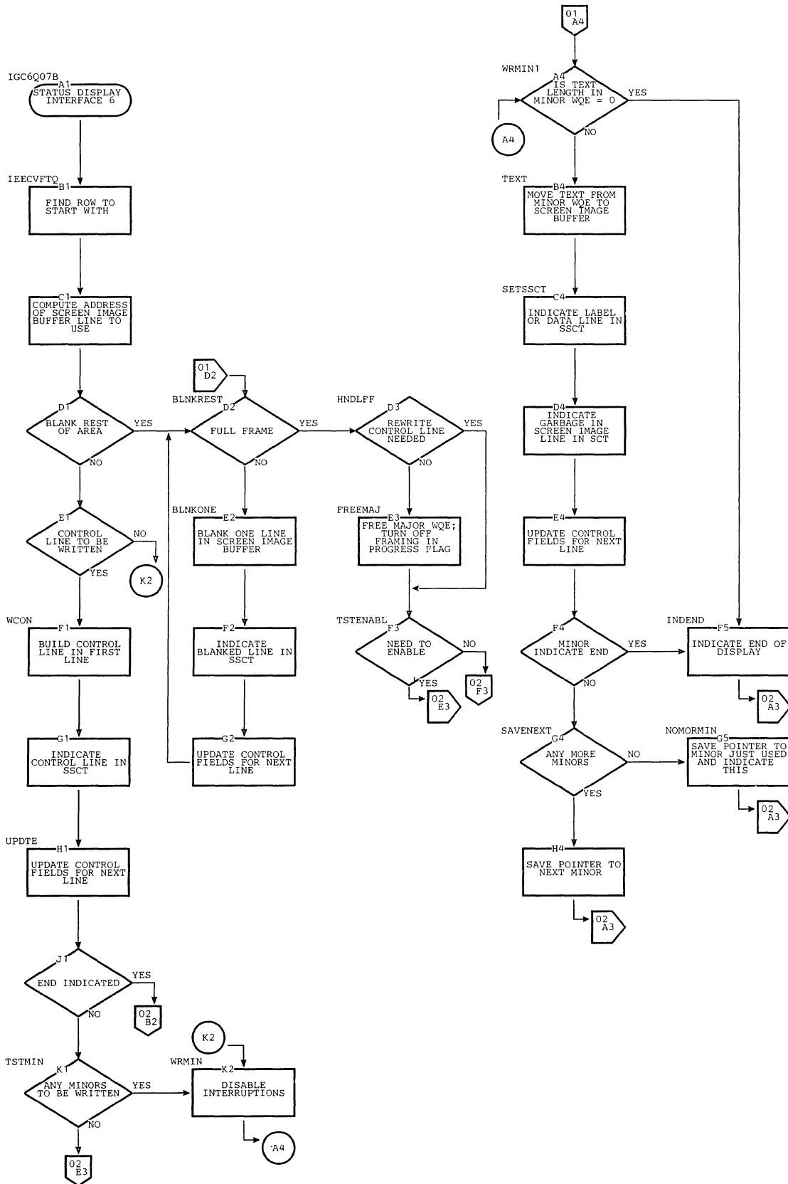
Chart 10. Status Display Interface 6 Routine (Page 1 of 2)
