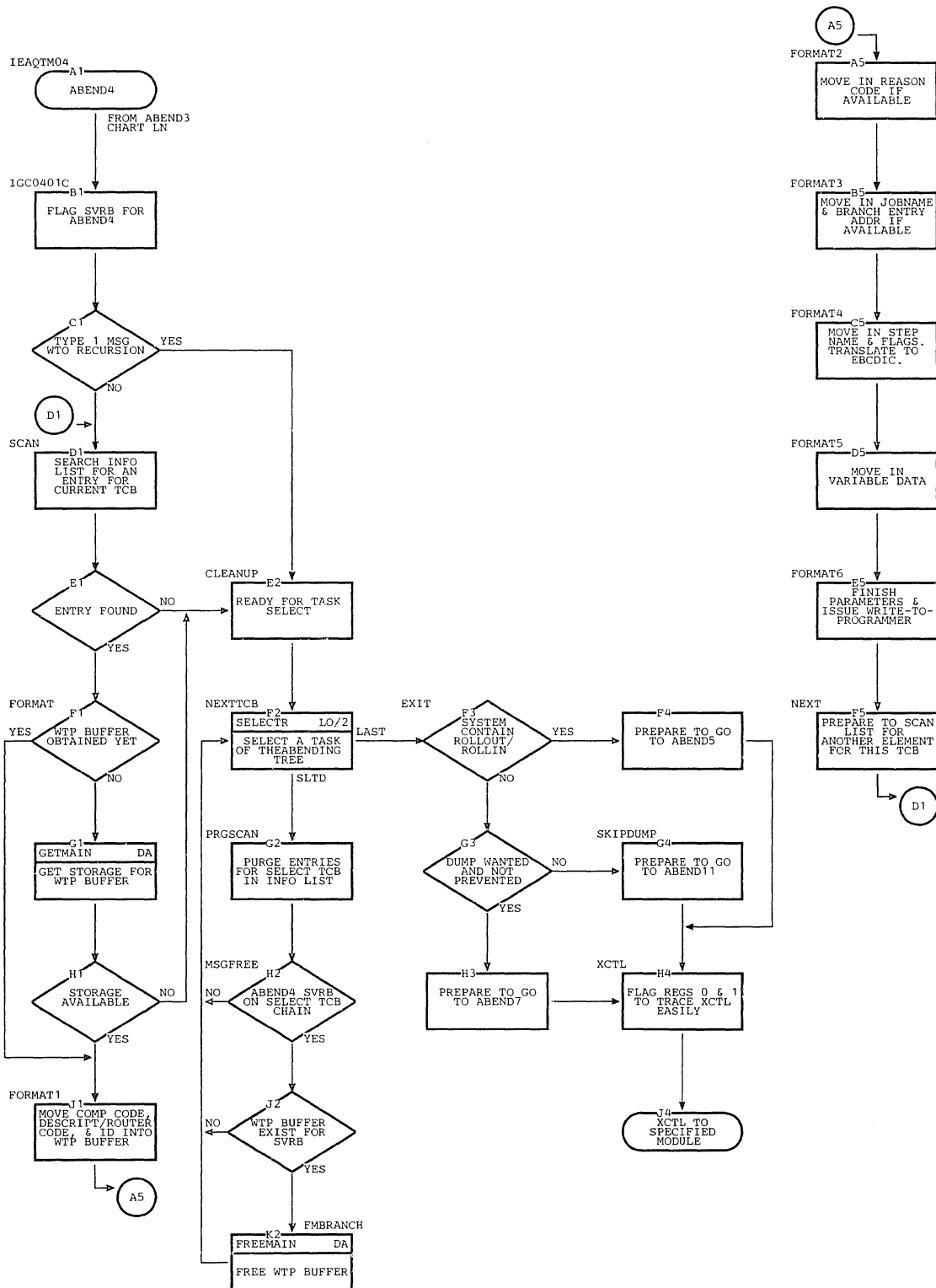
Chart 10. ABEND4 (Page 1 of 2)
