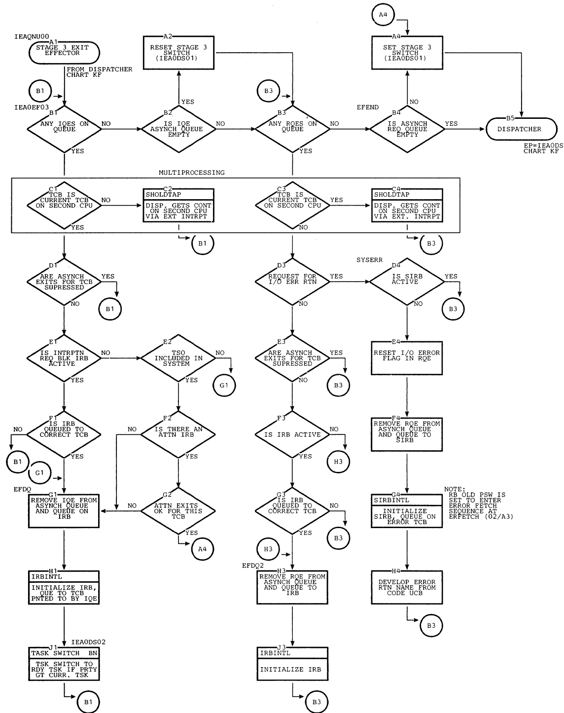
Chart BM. Stage 3 Exit Effector (Page 1 of 2)
