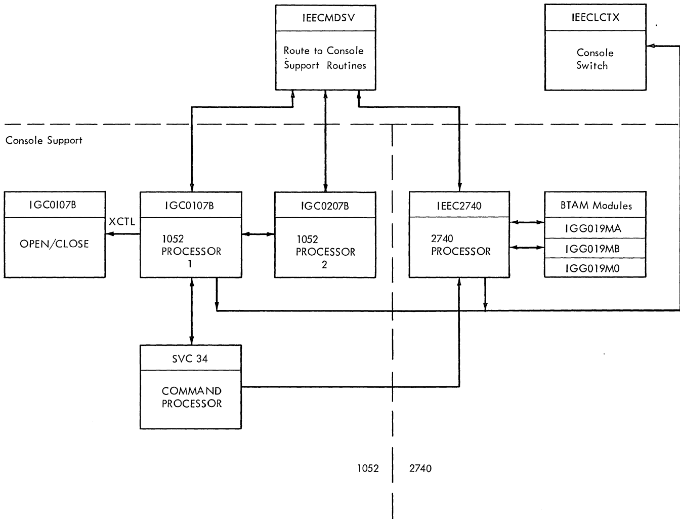
Figure 7-6. 1052 and 2740 Console Support Routines with MCS
