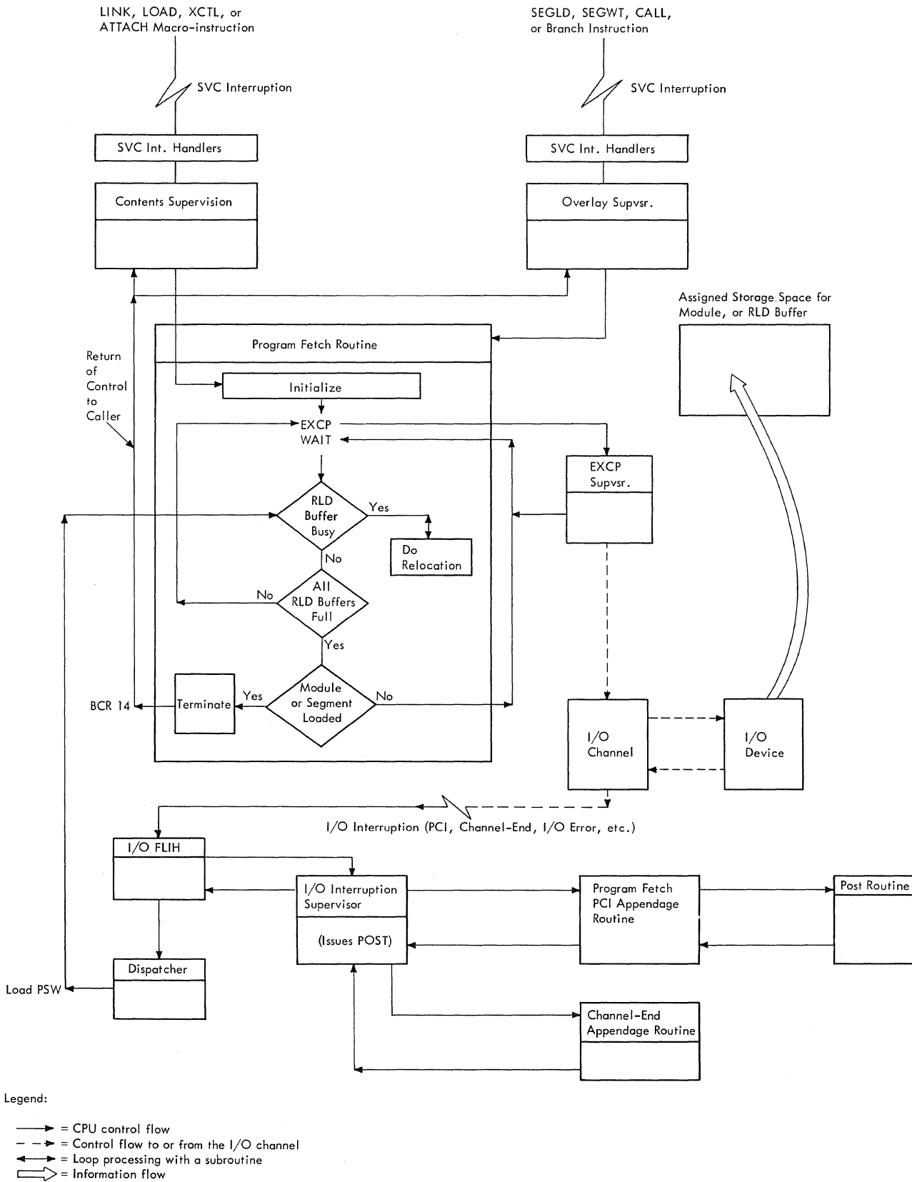
Figure 4-18. Overall Control Flow During the Loading of a Module or Segment
