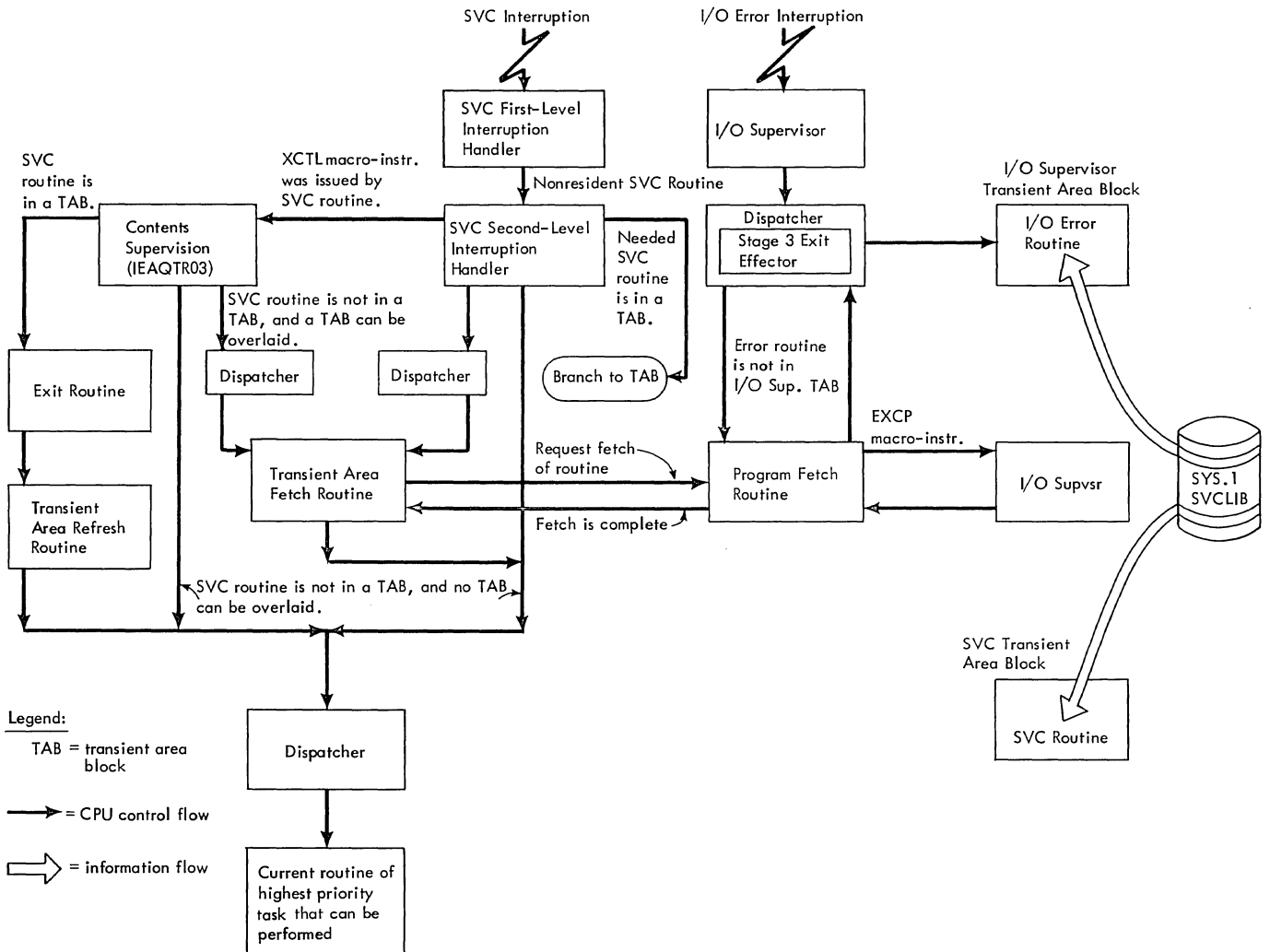
Figure 4-12. Relationships of Program Fetch Routine to Other Routines for the Fetch of an SVC Routine or an I/O Error Routine
