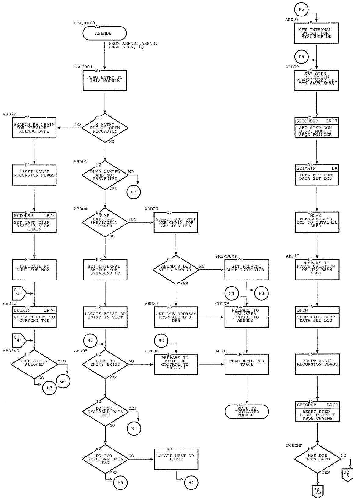
Chart LR. ABEND8 (Page 1 of 4)
