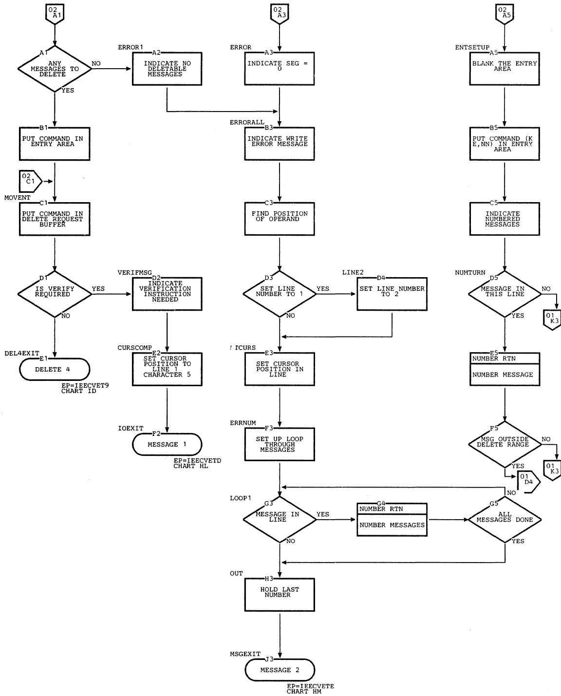
Chart IC. DIDOCs Delete 3 Routine (Page 2 of 2)
