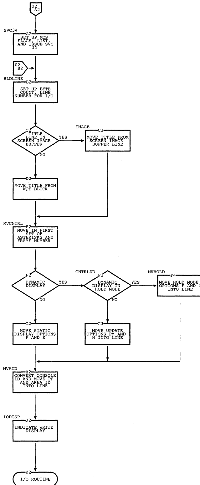
Chart II. Status Display Interface 3 Routine (Page 2 of 2)
