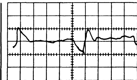
FIGURE 67. DRIVE LINE SHORTED TO GROUND
