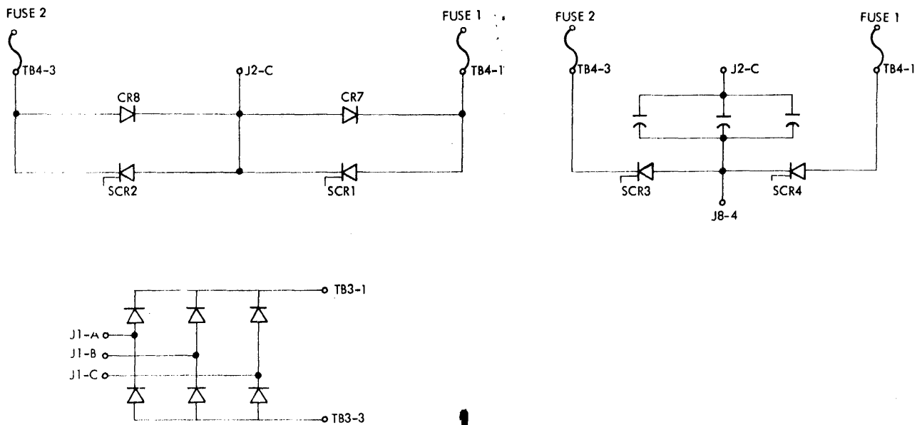
FIGURE 116. CONVERTER-INVERTER TEST POINTS
