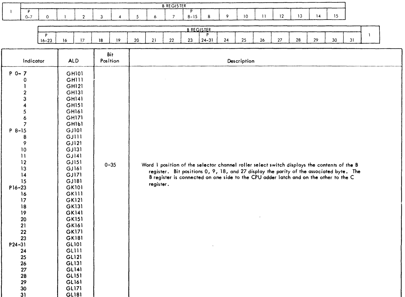
FIGURE 145. SELECTOR CHANNEL ROLLER - POSITION 1
