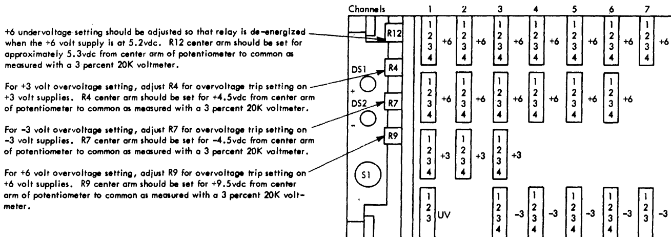
FIGURE 127. OVERVOLTAGE ASSEMBLY
