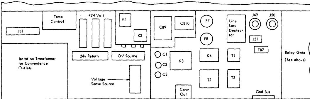
FIGURE 121. POWER DISTRIBUTION FRAMES (PART I OF 2)
