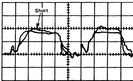
FIGURE 63. SHORTED X DRIVE LINE
