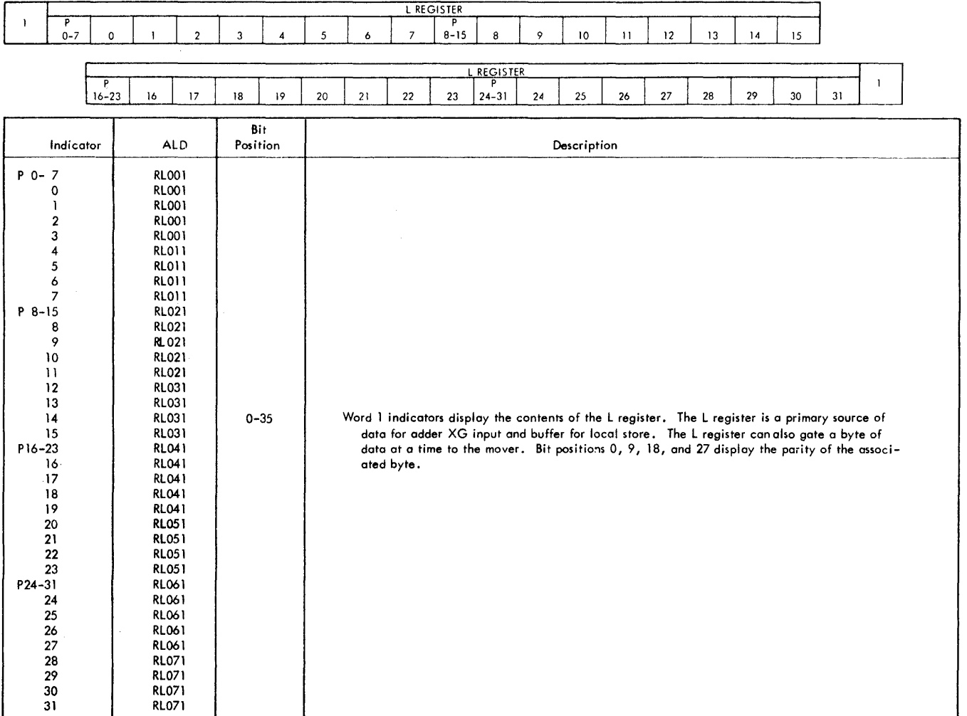
FIGURE 153. CPU 1 ROLLER - POSITION 1
