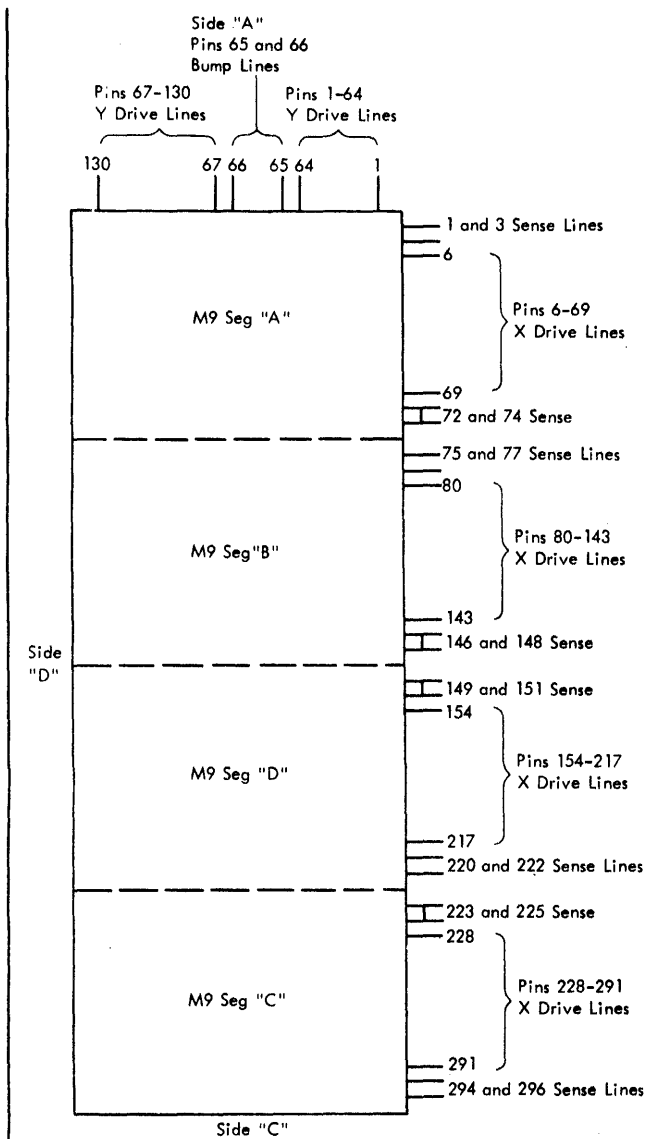
FIGURE 60. PHYSICAL LAYOUT OF M9/M9A PLANES
