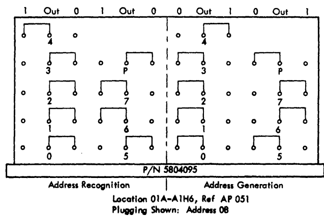
FIGURE 131. 1443 ADDRESS CARD LOCATIONS AND PLUGGING
