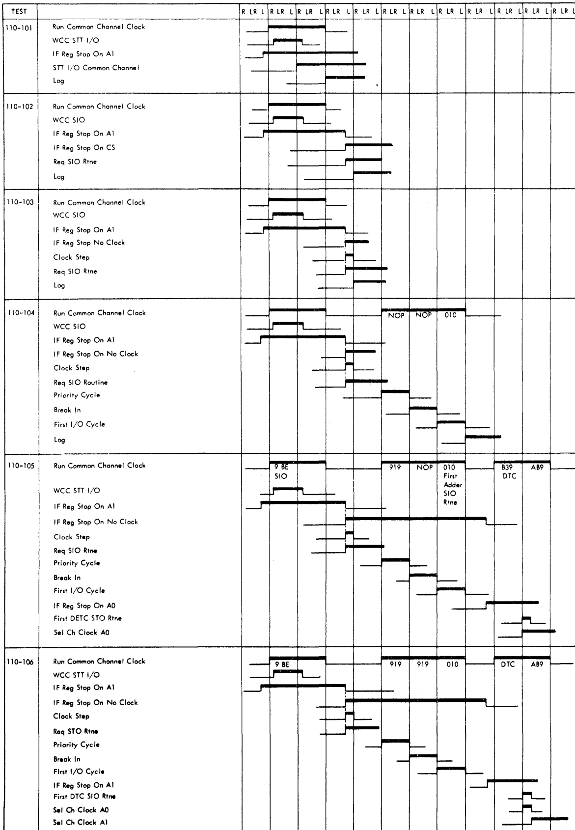
FIGURE 47. START I/O WRITE TIMING
