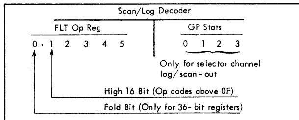
FIGURE 11. SCAN/LOG DECODER
