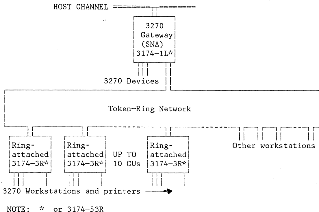
Figure 14. IBM Token-Ring Network
