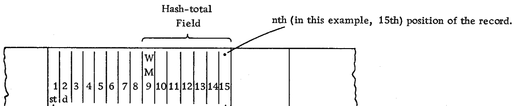
Figure 73. Hash-total Field
