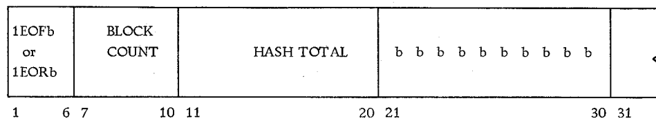
Figure 79. Format 3 of Standard Trailer Label
