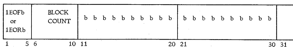
Figure 78. Format 2 of Standard Trailer Label
