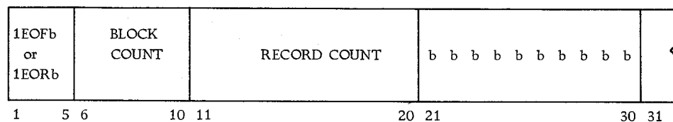
Figure 80. Format 4 of Standard Trailer Label
