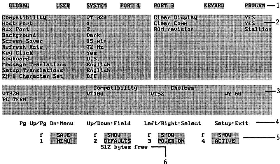
Figure 2-1. Format of Setup Menu
