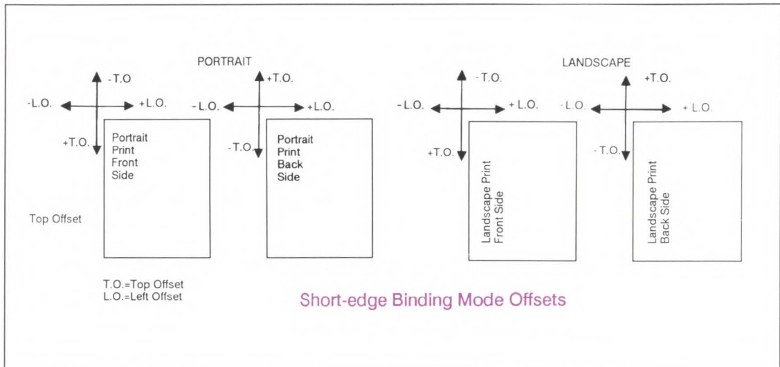
Figure 4-5. Short-Edge Binding Mode Offset
