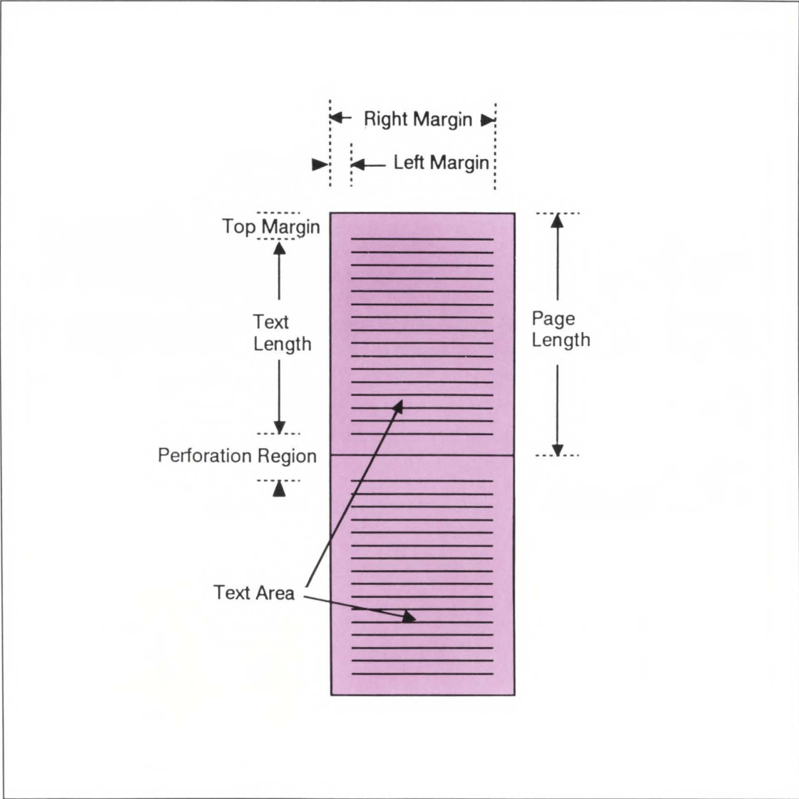
Figure 5-2. Text Area within the Page
