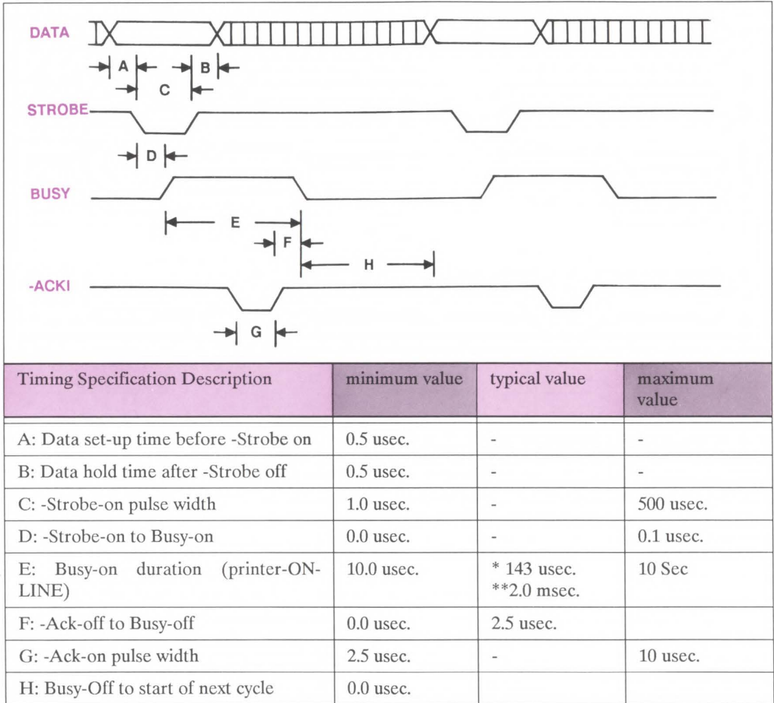
Figure B-1. Parallel Handshake Timing
