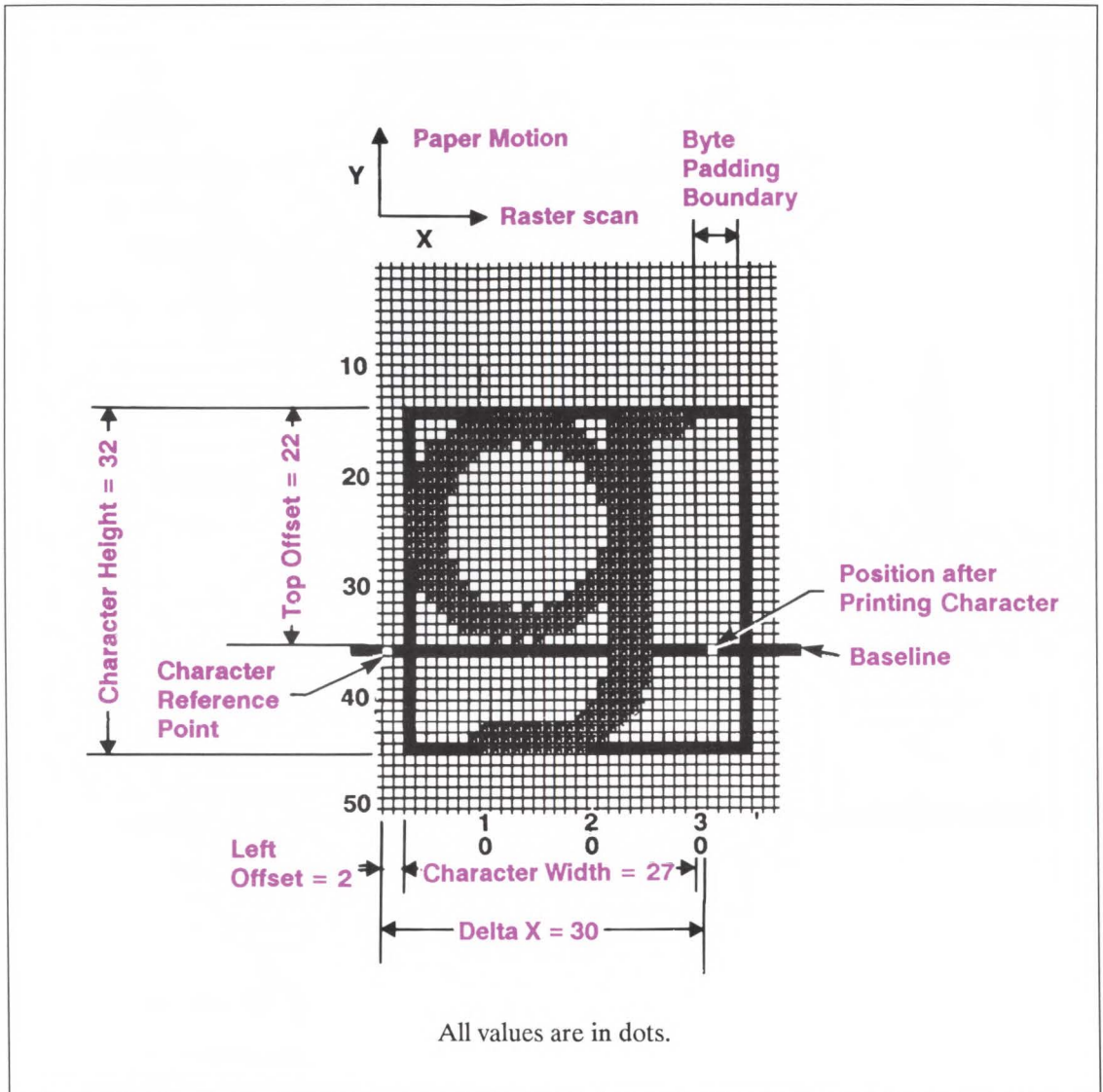
Figure 10-6. Portrait Character Example
