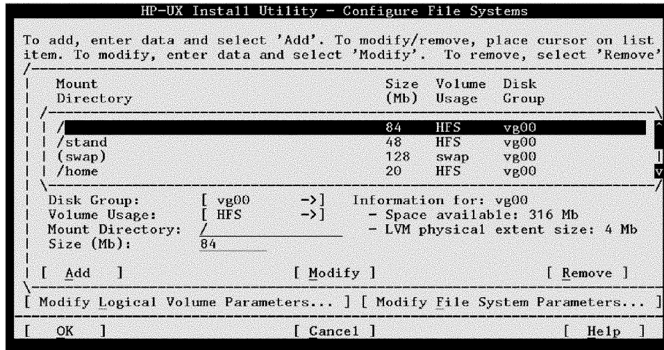
Figure 2-16 Configure File Systems
