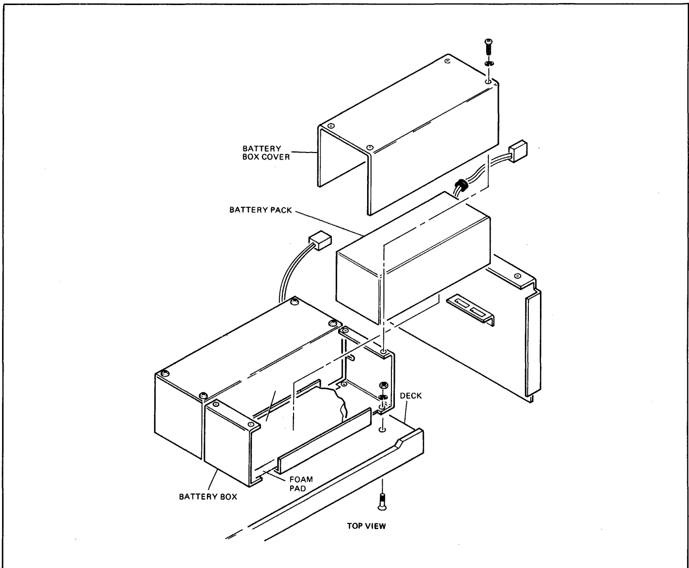
Figure 3. Installation of Batteries in Extender
