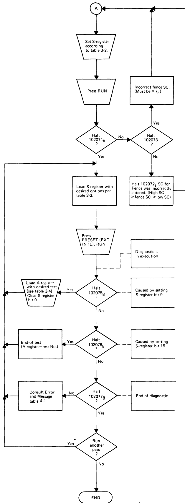
Figure 3-1. Operating Procedure Flowchart (Sheet 2 of 2)
