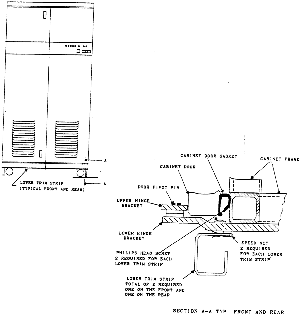
FIGURE 3-4. TRIM STRIP INSTALLATION
