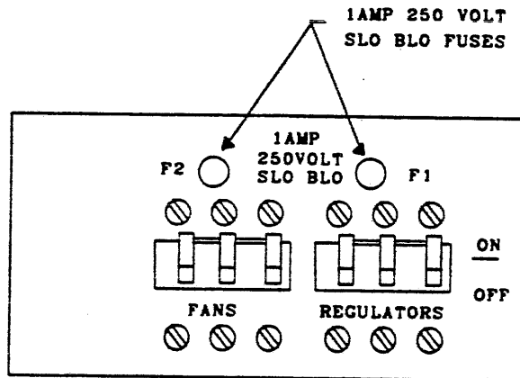
FIGURE 4-19. FANS AND DC REGULATORS CIRCUIT BREAKERS AT S03 (SLO BLO FUSES)
