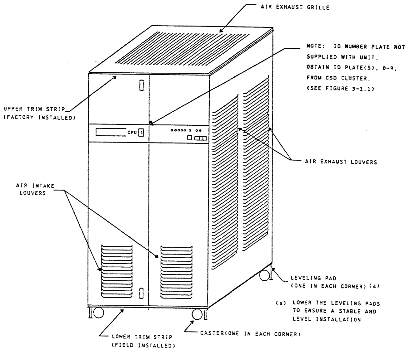
FIGURE 3-1. DPS 8 MULTIC CENTRAL PROCESSOR UNIT (CPU), WCPU68LA
