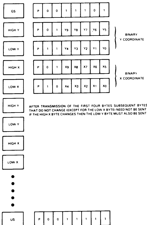
Figure 4-4: Vector Drawing Sequence
