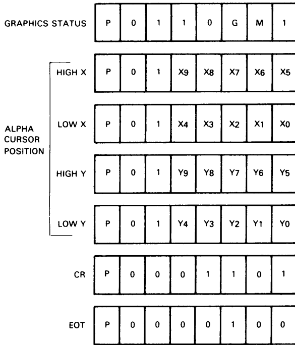
Figure 4-5: Response to ESC, ENQ
