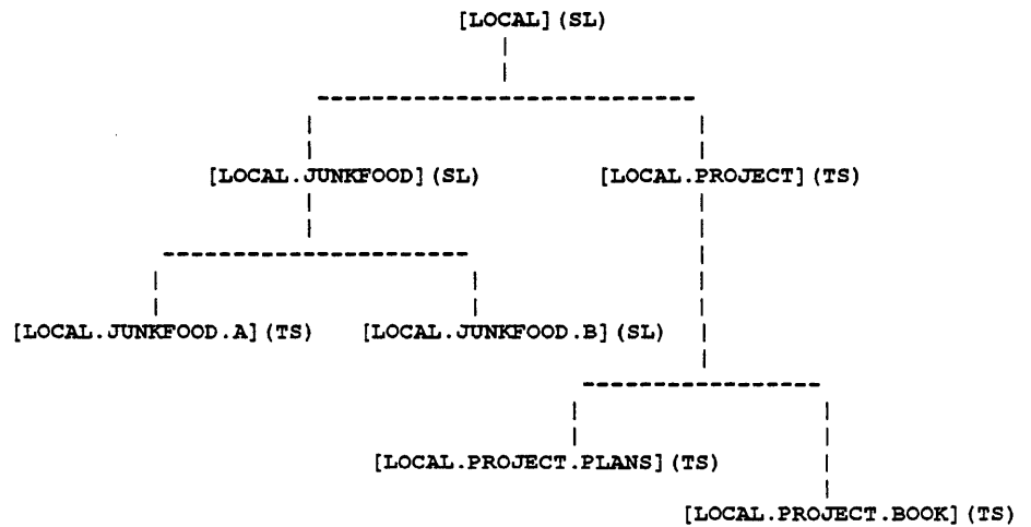
Figure 1-1 Directory Structure Example
