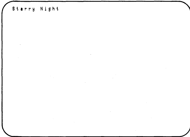
Figure 5-5: Generating Text—VT241
