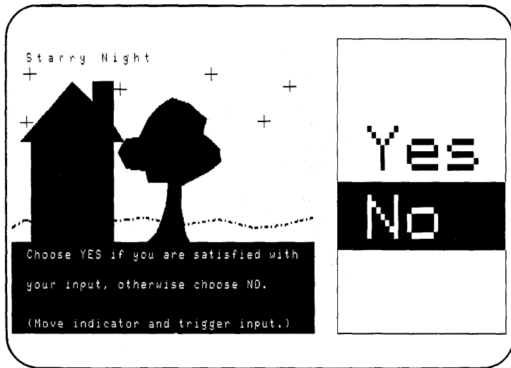
Figure 6–9: Choosing “No”—VT241
