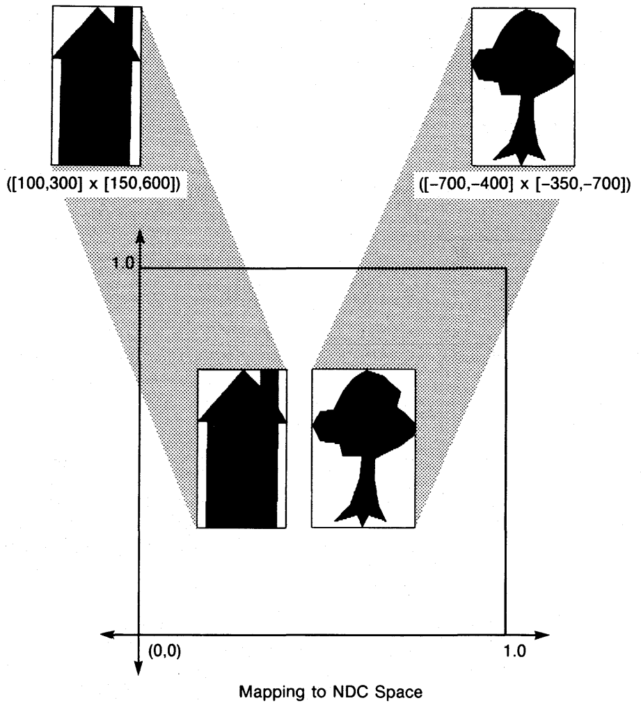
Figure 4–2: Composing a Picture on the NDC Plane
