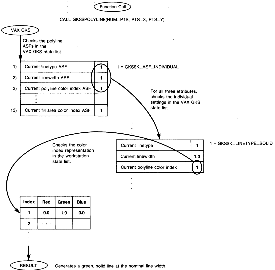
Figure 5-1: Default Aspect Source Flag Settings
