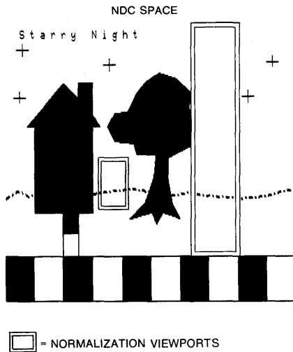
Figure 4-6: Choosing Various Normalization Viewports
