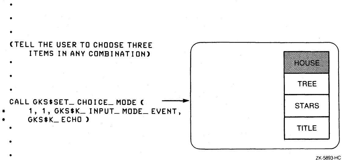
Figure 7-6: Placing a Choice Device in Event Mode
