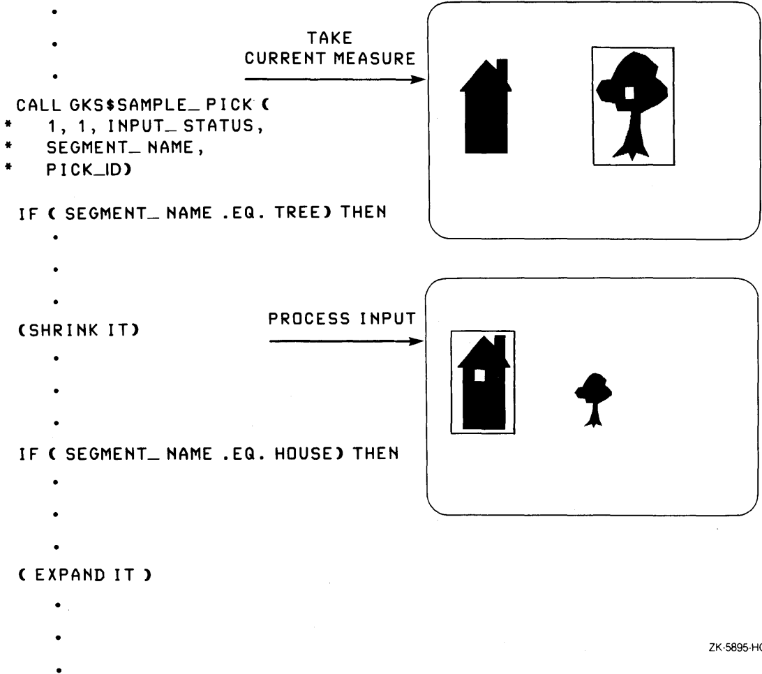
Figure 7-5: Sampling a Pick Device
