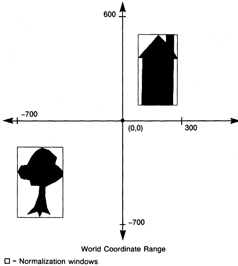
Figure 4-1: Plotting Portions of a Picture in World Coordinates
