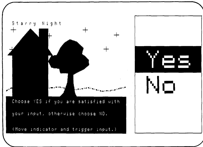
Figure 6–11: Choosing “Yes”—VT241
