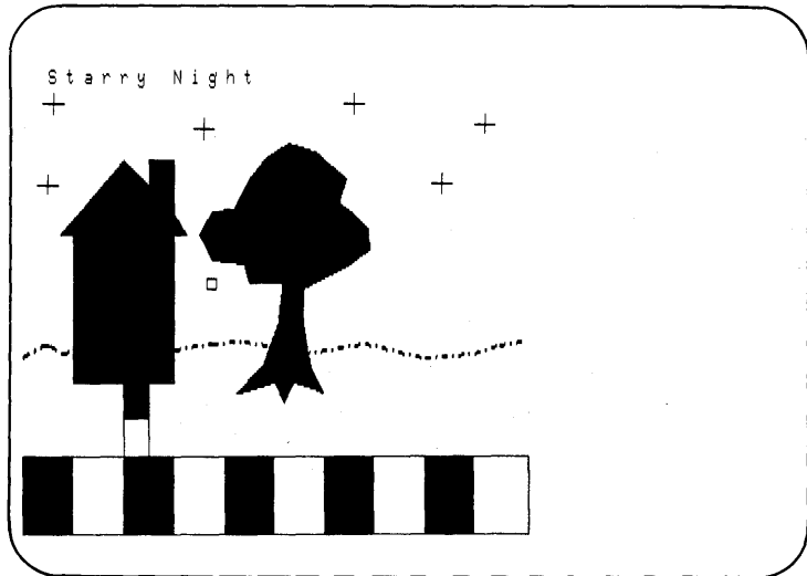
Figure 6-4: Specifying GKS$K_STATUS_NOPICK—VT241
