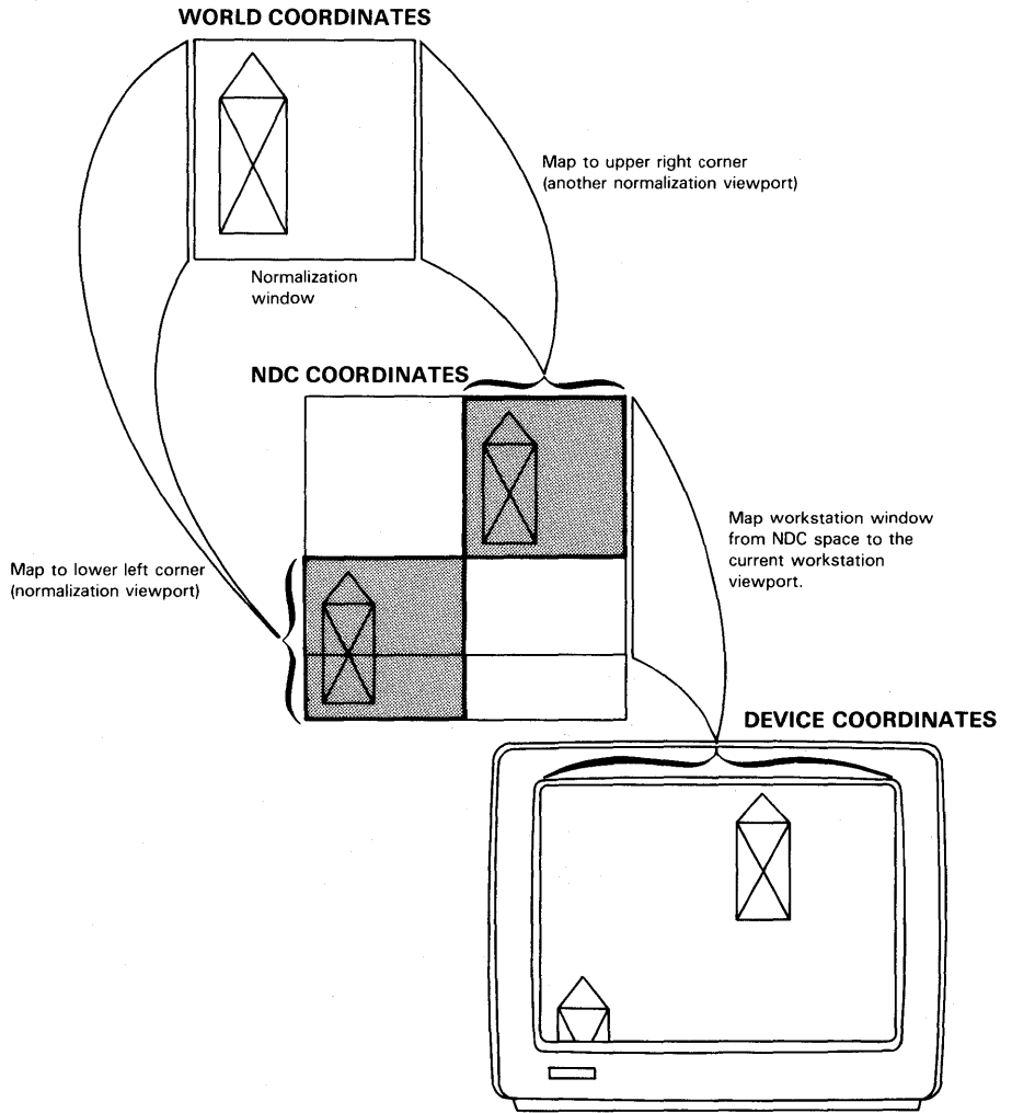
Figure 4-3: The DEC GKS Transformations
