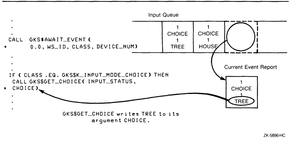
Figure 7–9: Removing Reports from the Queue
