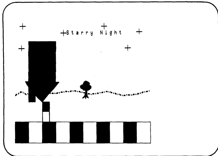
Figure 5-11: Transformed Segments—VT241
