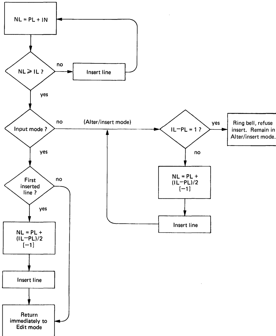
Figure 3-1 How SOS Calculates the Numbers of New, Inserted Lines
