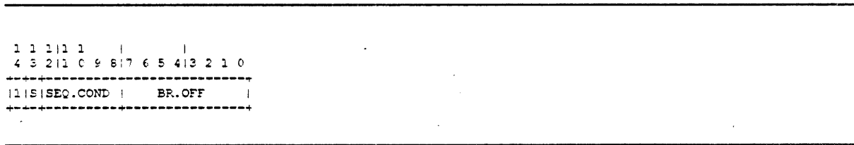
Figure 6-4: Ebox Microsequencer Control, Branch Format
