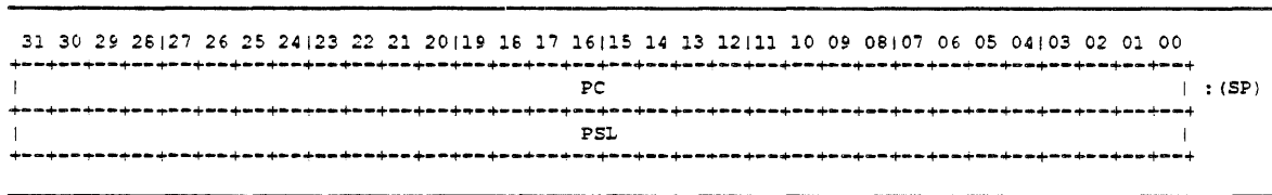
Figure 14-7: Soft Error Interrupt Stack Frame
