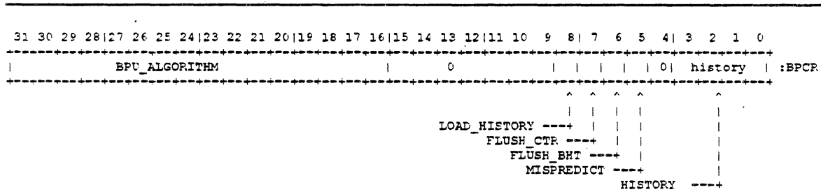
Figure 7-6: BPCR Register
