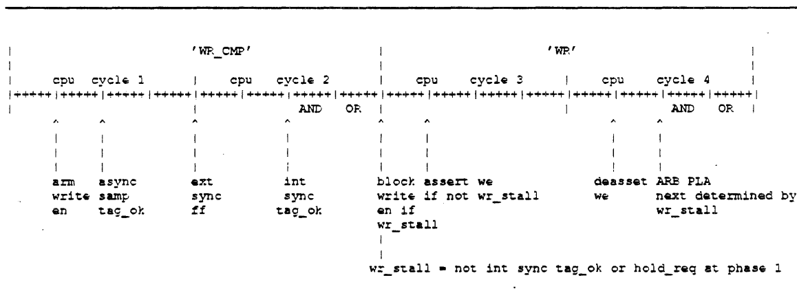
Figure 13-21: wr_stall timing
