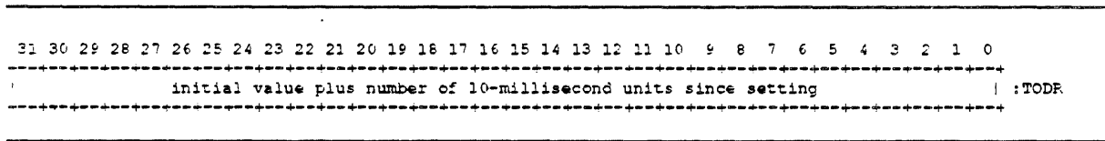
Figure 13-12: Time of Day Register, TODR
