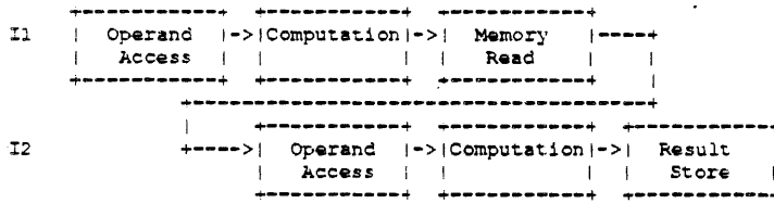
Figure 5-5: Information Flow Against the Pipeline
