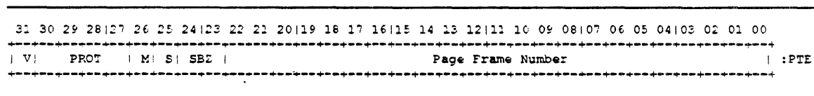
Figure 2-21: PTE Format (25-bit PFN)
