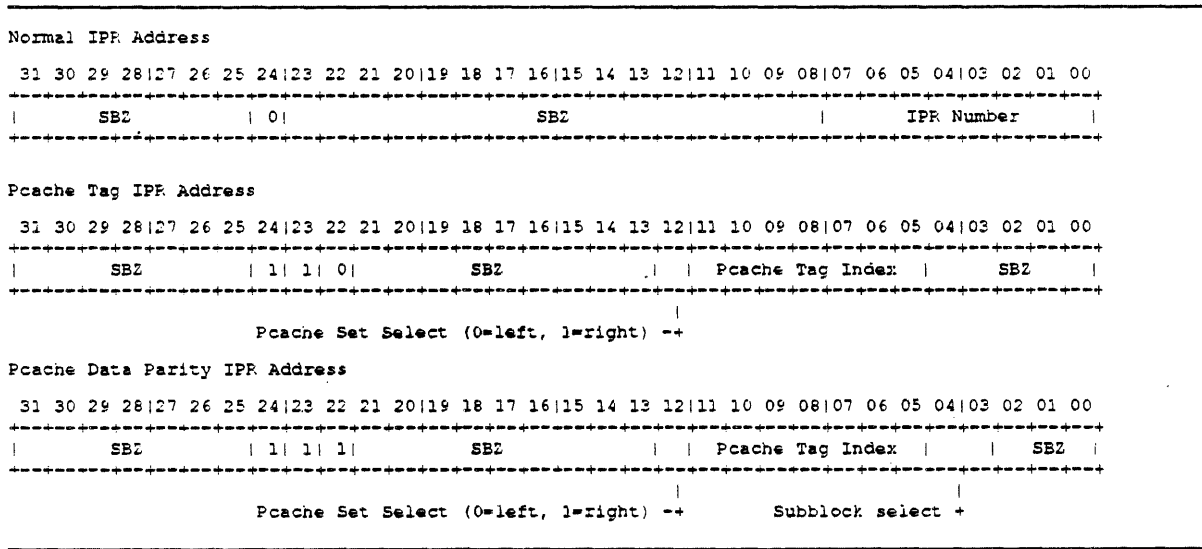
Figure 2-44: IPR Address Space Decoding
