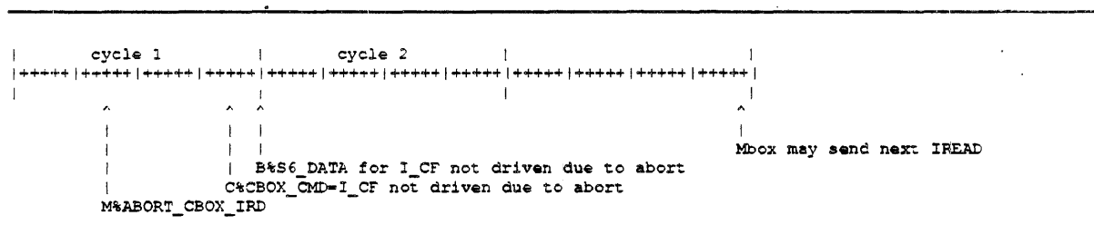
Figure 13-18: M%ABORT_CBOX_IRD Timing
