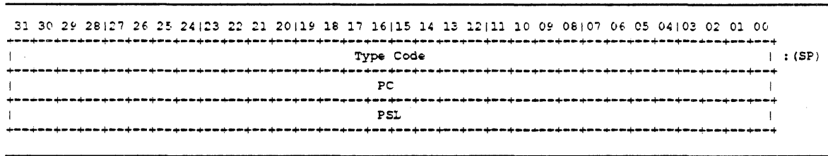
Figure 2-27: Arithmetic Exception Stack Frame
