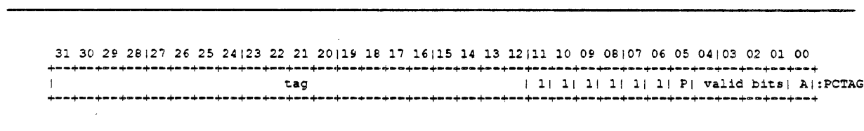
Figure 12-19: PCTAG Register
