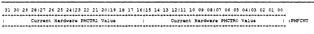
Figure 16-4: PMFCNT Processor Register
