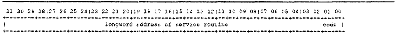
Figure 2-34: System Control Block Vector
