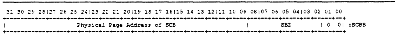
Figure 2-33: System Control Block Base Register
