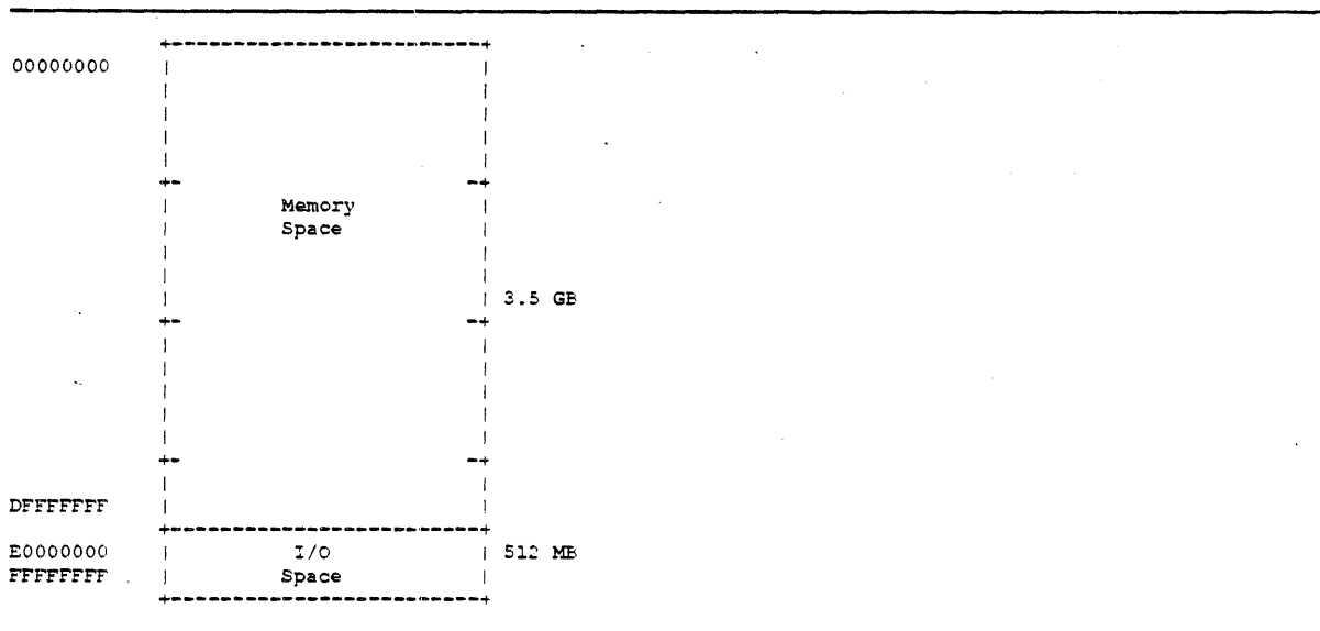
Figure 2-2: 32-bit Physical Address Space Layout
