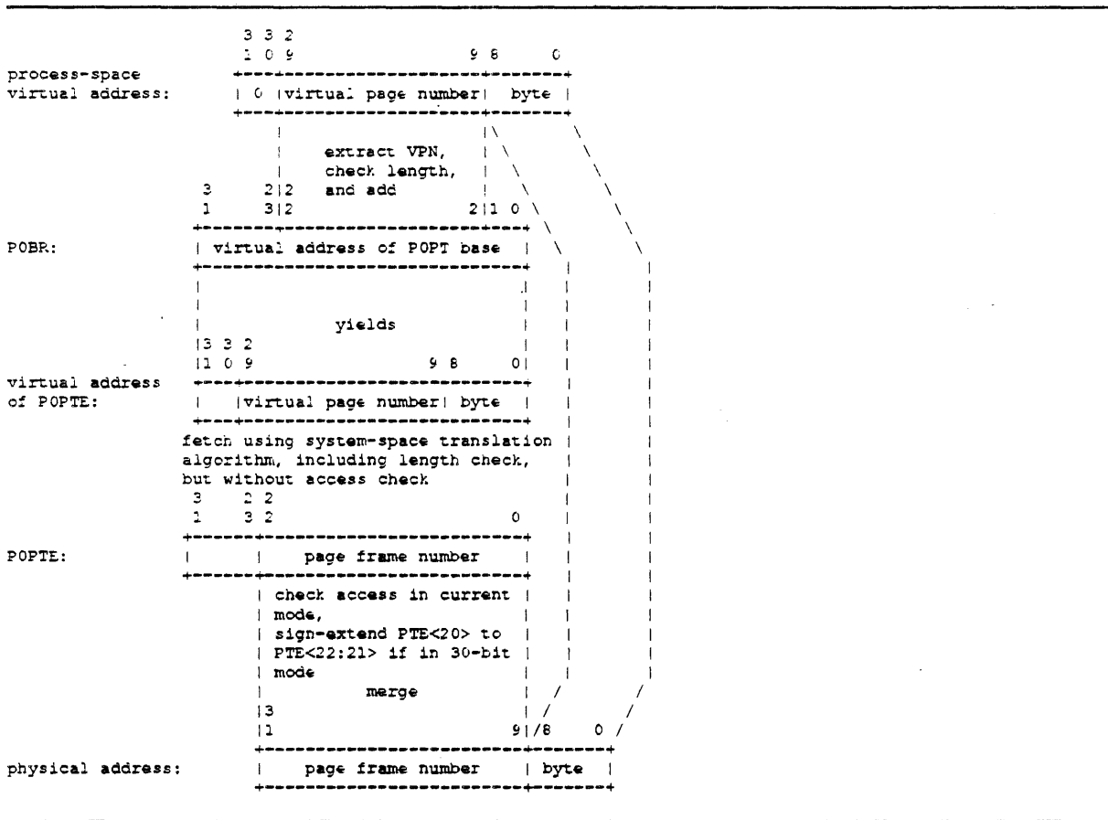
Figure 2-17: P0 Space Translation Algorithm
