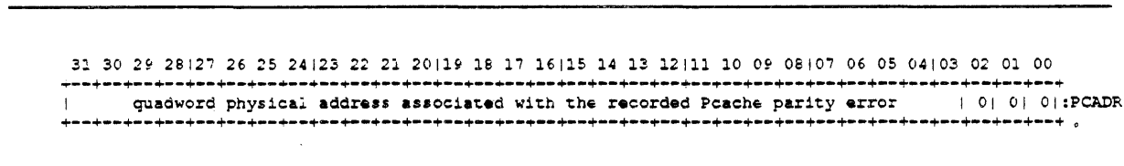
Figure 12-16: PCADR Register
