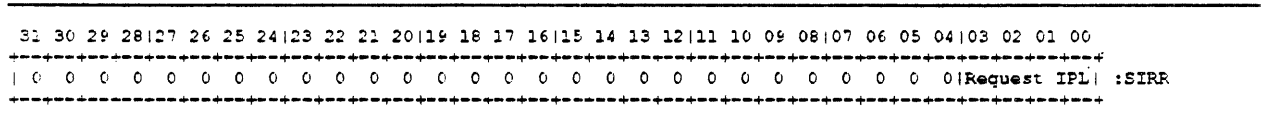
Figure 2-25: Software Interrupt Request Registers
