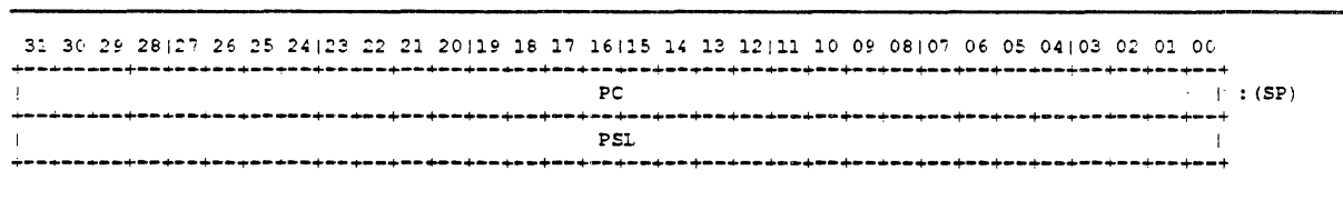
Figure 2-22: Minimum Exception Stack Frame
