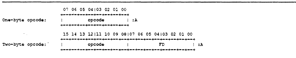
Figure 2-8: Opcode Formats
