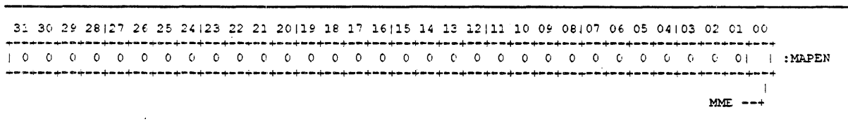
Figure 2-11: MAPEN Register
