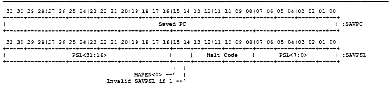
Figure 2-32: Console Saved PC and Saved PSL
