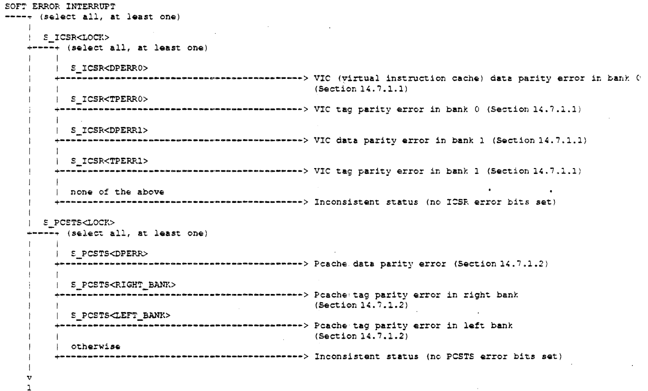
Figure 14-8: Cause Parse Tree for Soft Error Interrupts
