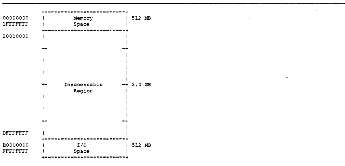
Figure 2-3: 30-bit Physical Address Space Layout
