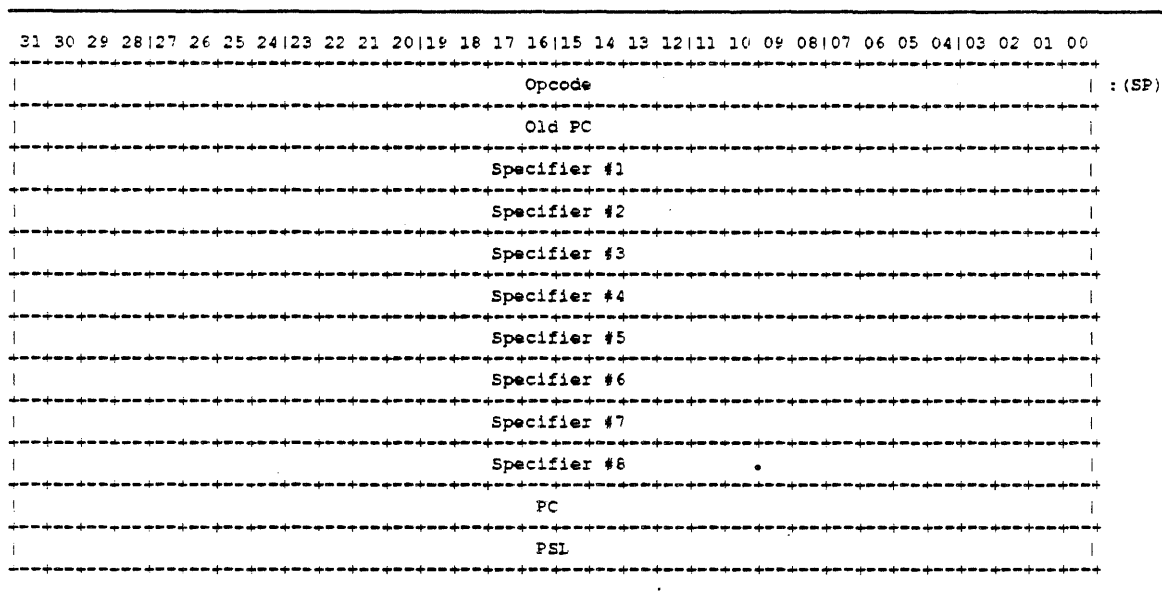
Figure 2-29: Instruction Emulation Trap Stack Frame
