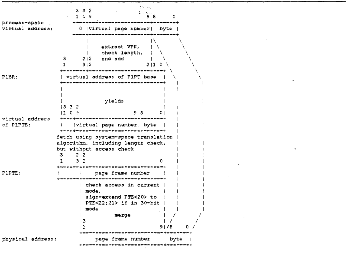
Figure 2-19: P1 Space Translation Algorithm
