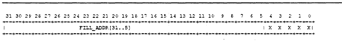
Figure 13-3: FILL_ADDR
