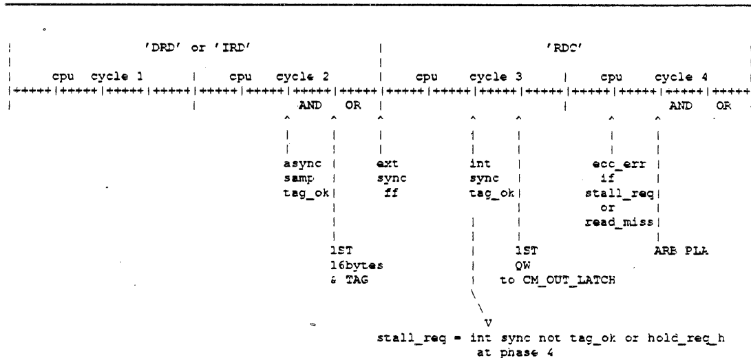
Figure 13-20: stall_req timing
