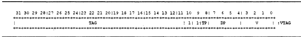
Figure 7-3: VTAG Register
