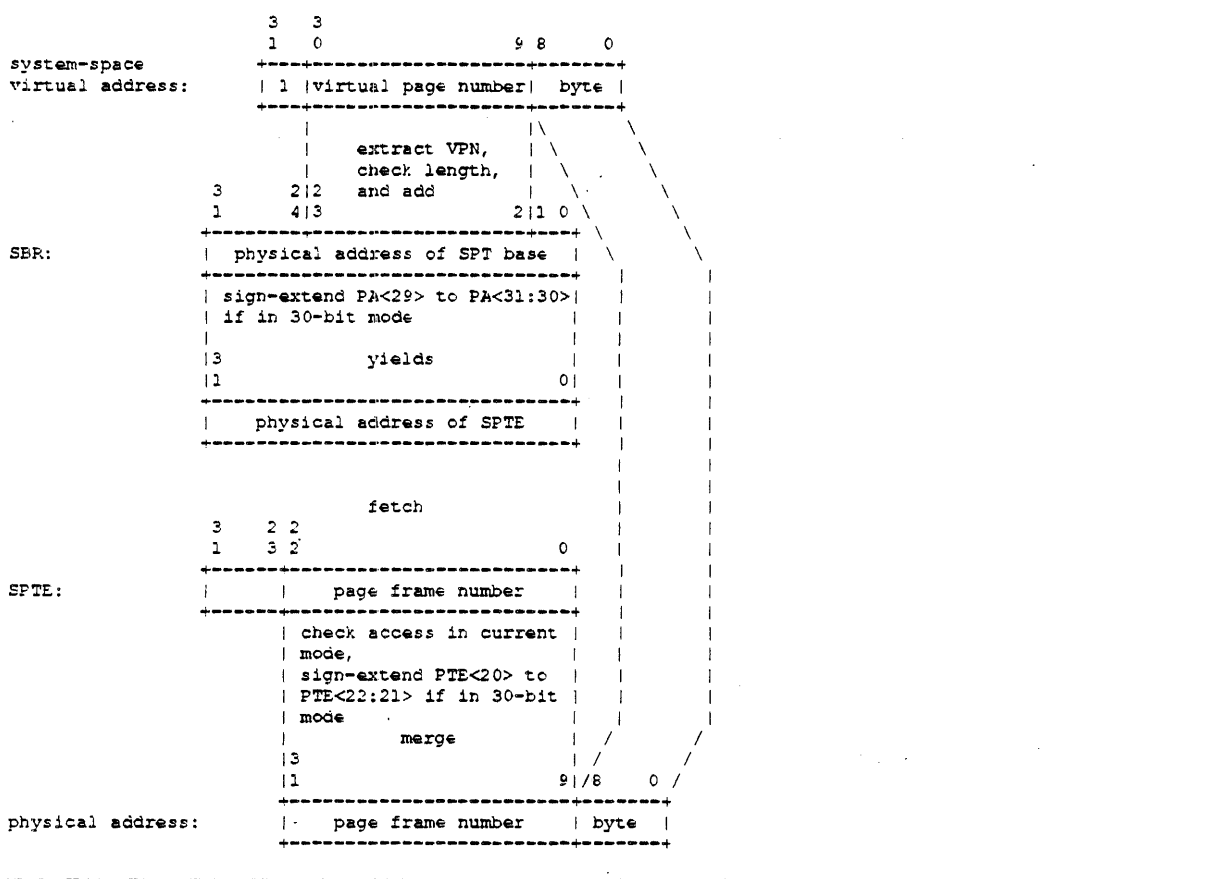
Figure 2-15: System Space Translation Algorithm
