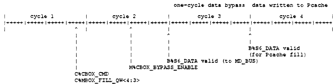
Figure 13-17: B%S6_DATA bypass timing
