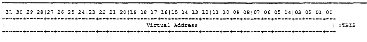
Figure 2-12: TBIS Register
