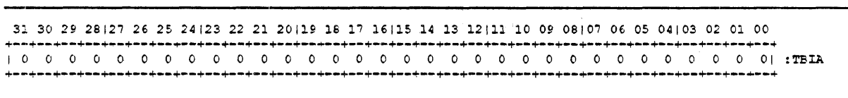
Figure 2-13: TBIA Register
