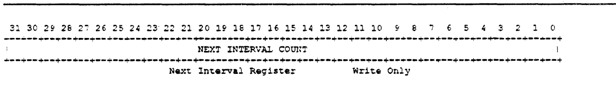
Figure 13-15: NICR
