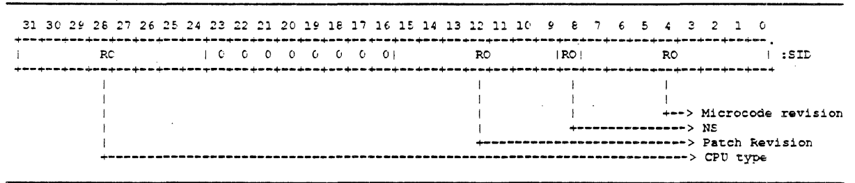
Figure 2-36: System Identification (SID)
