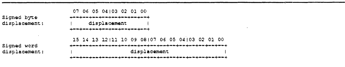
Figure 2-10: Branch Displacements
