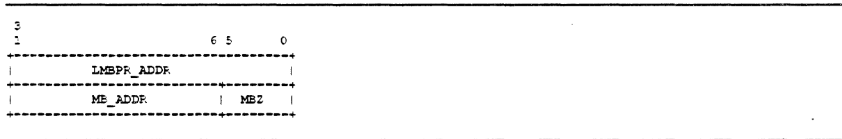
Figure 2-42: Mailbox Pointer
