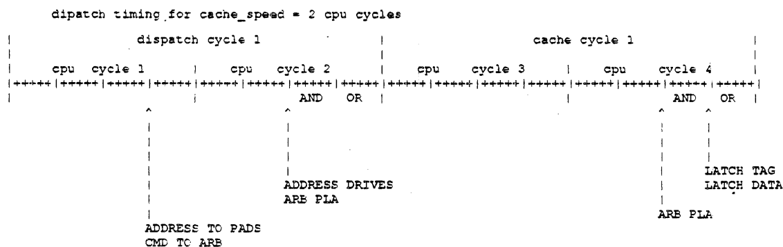
Figure 13-19: DISPATCH timing
