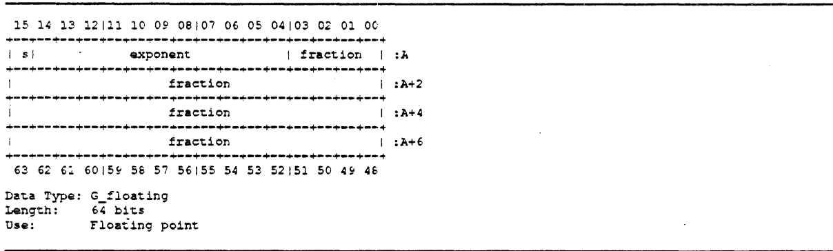
Figure 2-7 (Cont.): Data Types
