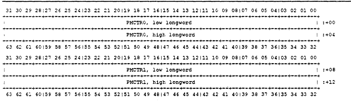
Figure 16-2: Per-CPU Performance Monitoring Data Structure
