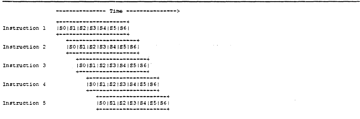
Figure 5-3: Fully-Pipelined Instruction Execution
