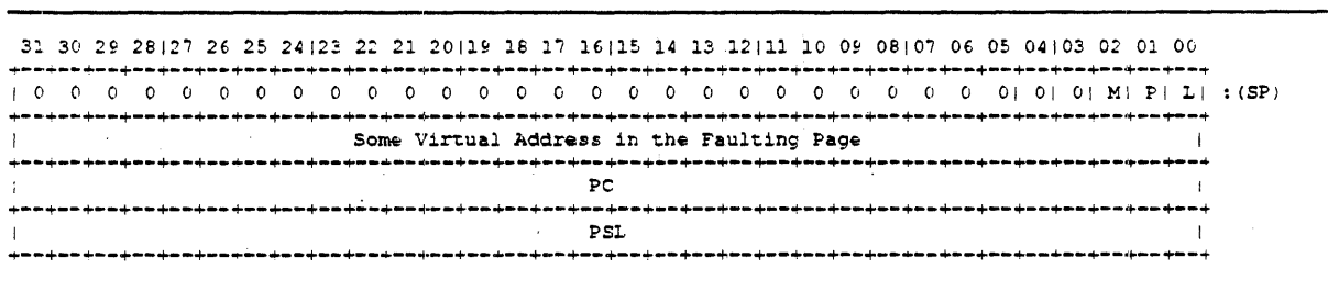
Figure 2-28: Memory Management Exception Stack Frame
