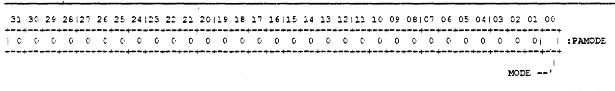
Figure 2-4: PAMODE Register
