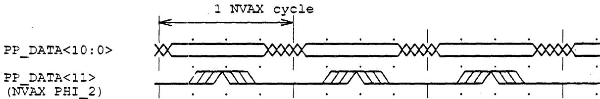
Figure 17-2: Internal Scan Register Operation Timing
