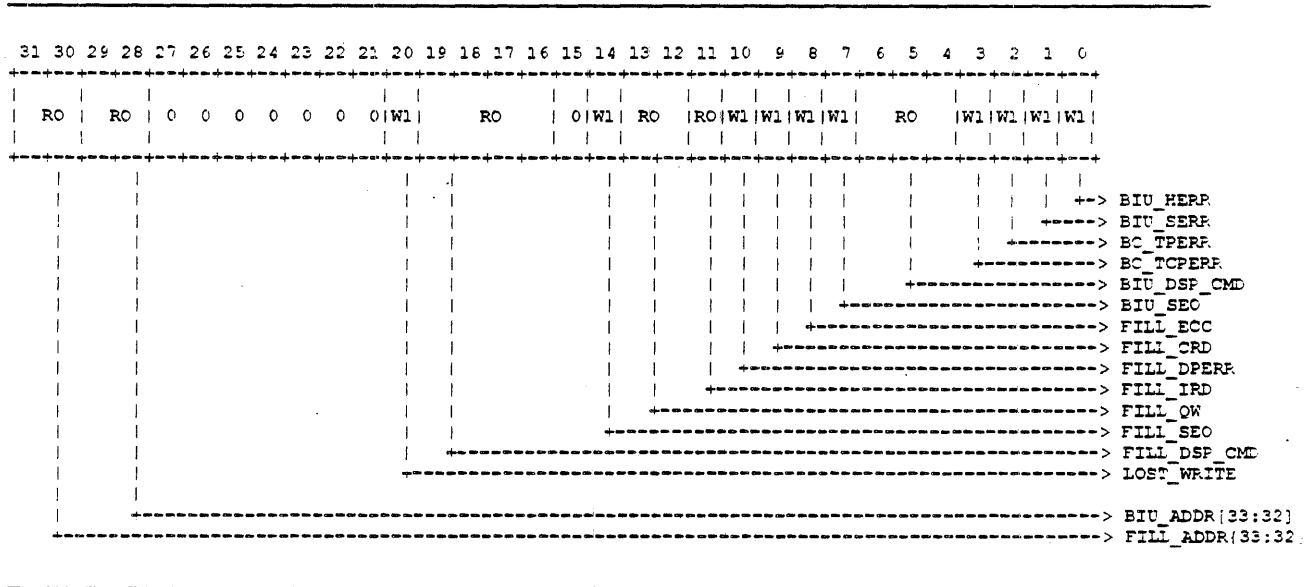
Figure 13-2 (Cont.): BIU_STAT
