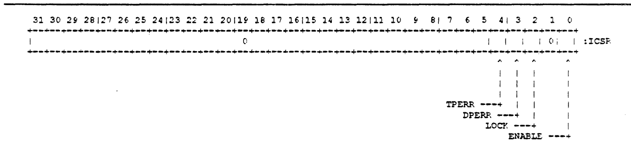
Figure 7-5: ICSR Register
