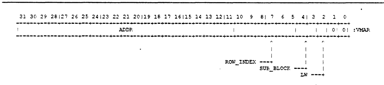
Figure 7-2: VMAR Register
