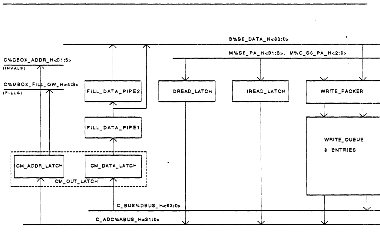
Figure 13-16: Mbox Interface
