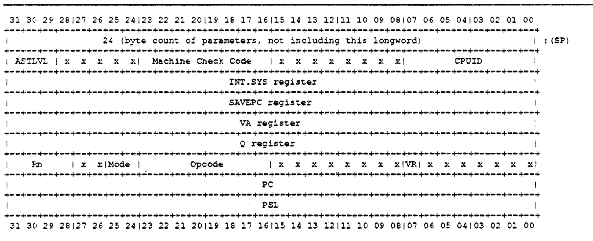
Figure 14-3: Machine Check Stack Frame
