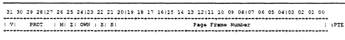
Figure 2-20: PTE Format (21-bit PFN)
