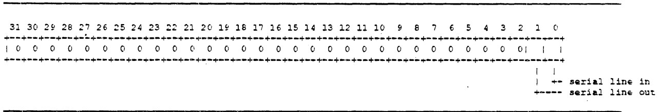
Figure 13-10 (Cont.): SIO
