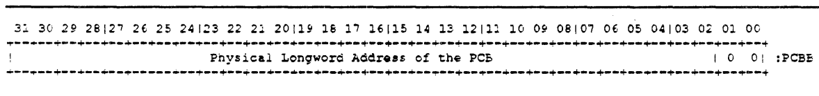
Figure 2-38: Process Control Block Base Register
