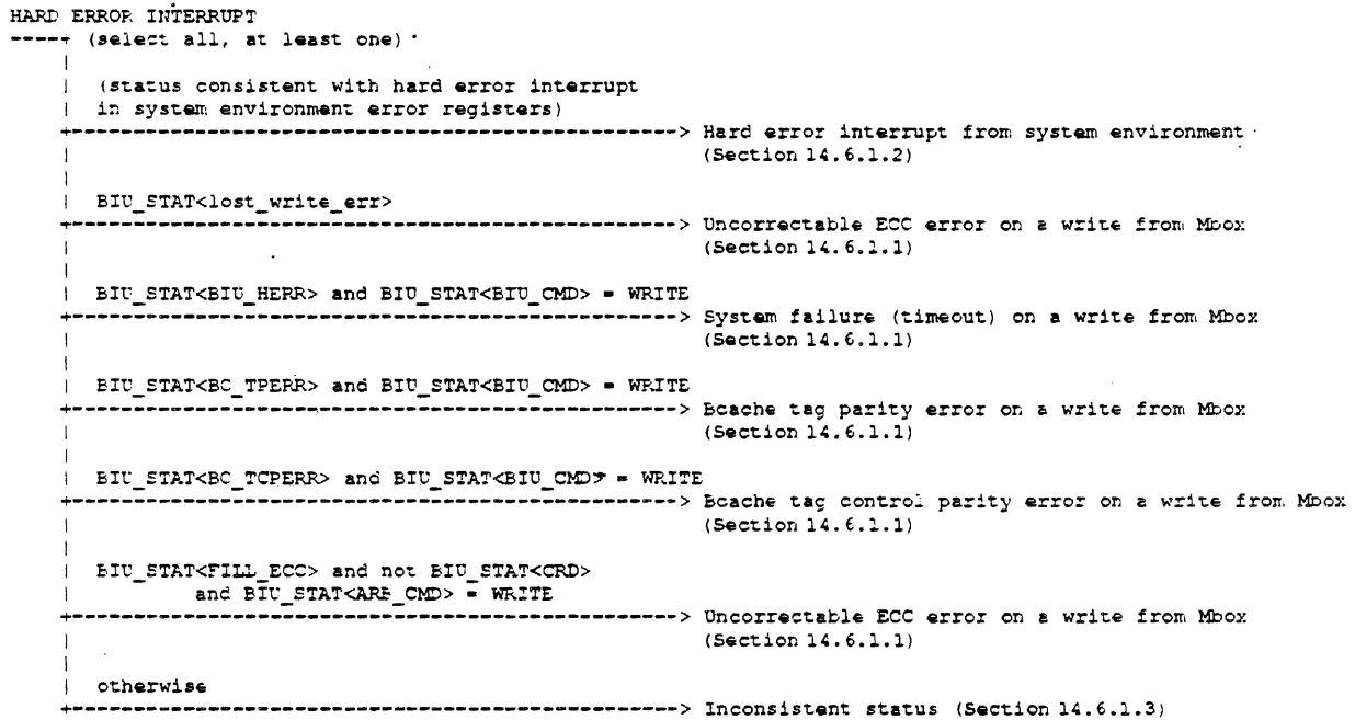
Figure 14-6: Cause Parse Tree for Hard Error Interrupts
