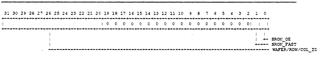
Figure 13-11: SOE-IE
