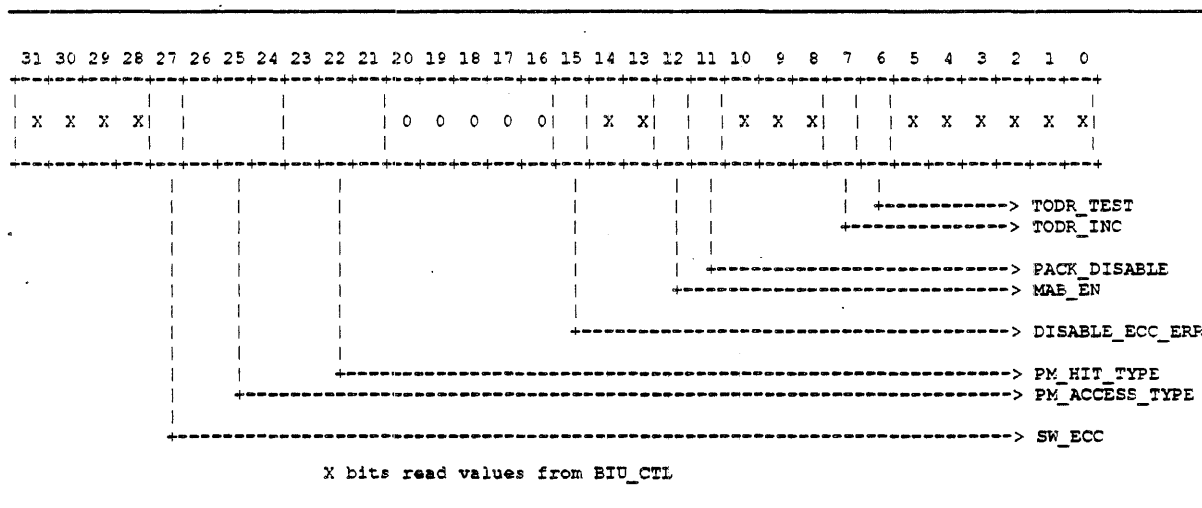
Figure 13-5: DIAG_CTL
