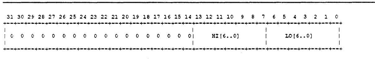
Figure 13-6: FILL_SYNDROME
