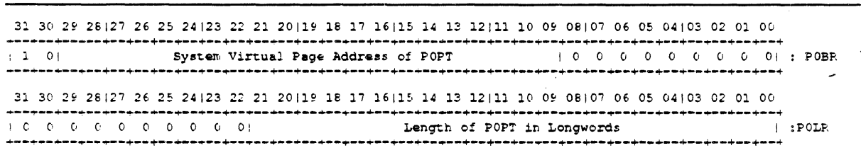
Figure 2-16: P0 Base and Length Registers
