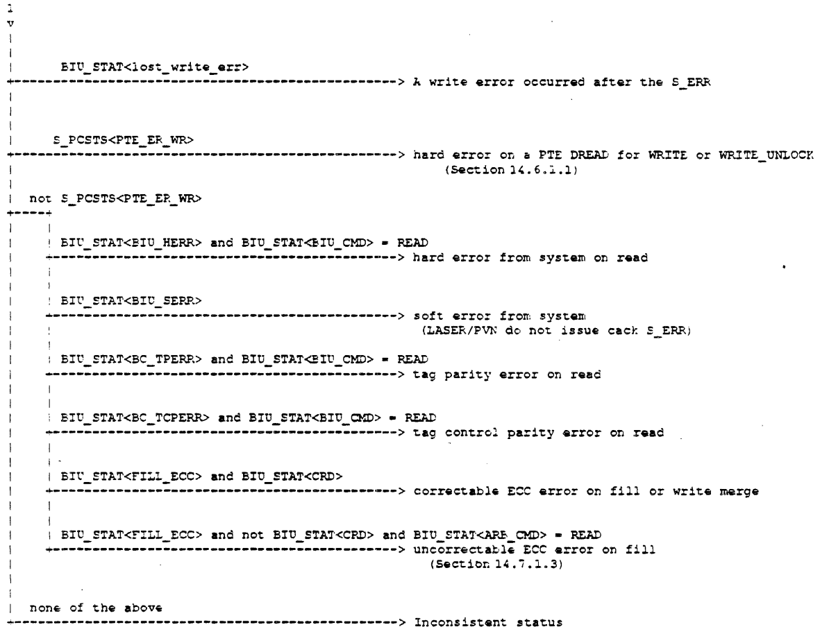
Figure 14-8 (Cont.): Cause Parse Tree for Soft Error Interrupts
