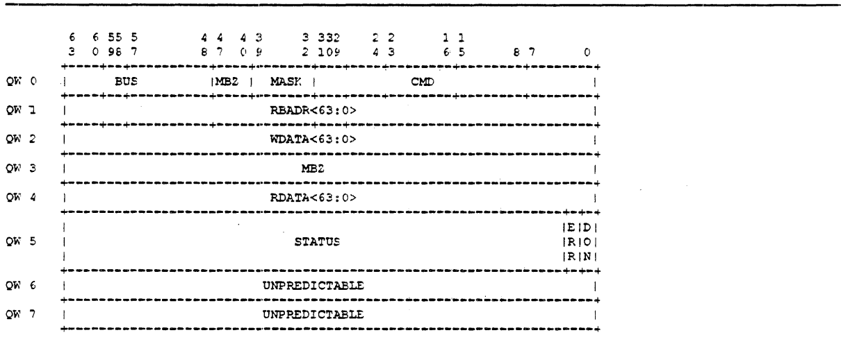
Figure 2-41: Mailbox Data Structure
