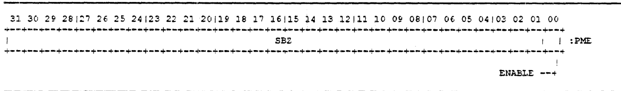
Figure 16-3: PME Processor Register
