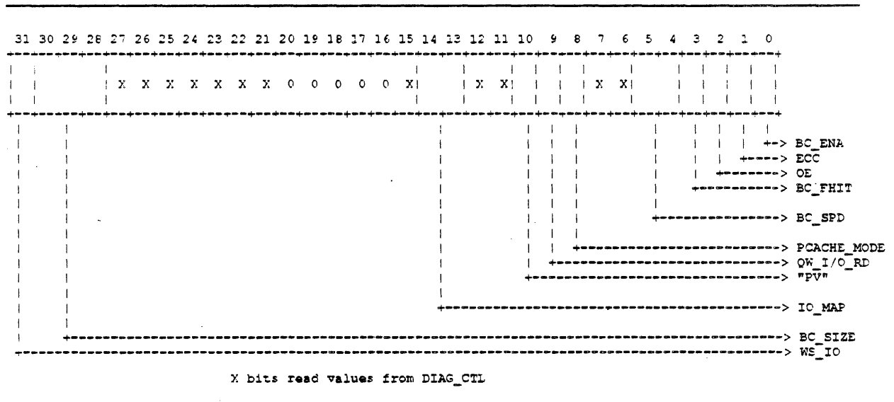
Figure 13-4: BIU_CTL
