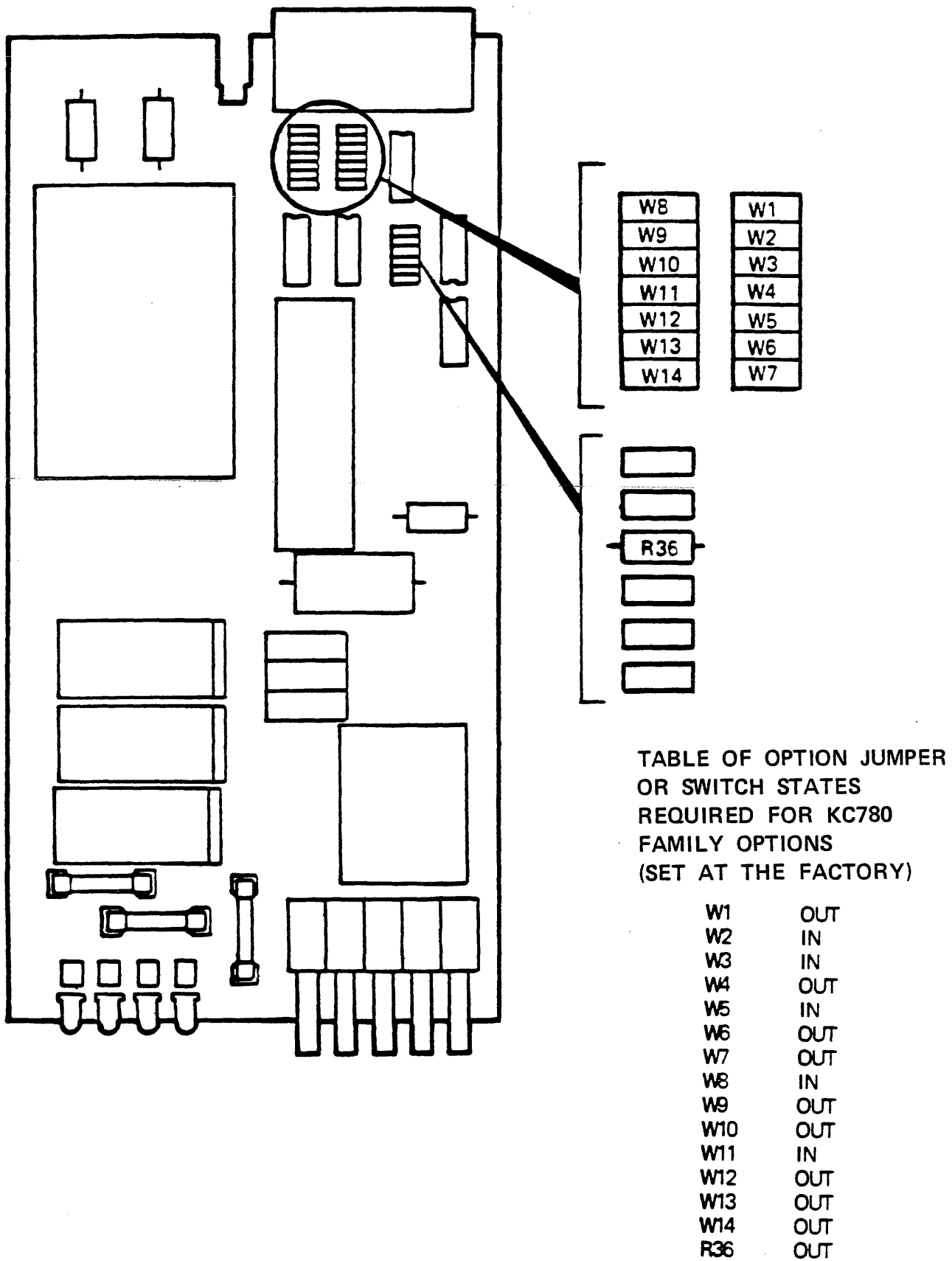
Figure A-5 DF02 Interface Board Jumps for KC780-BA
