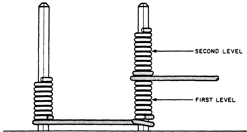
Figure B-4 Two Levels of Wire Wrap
