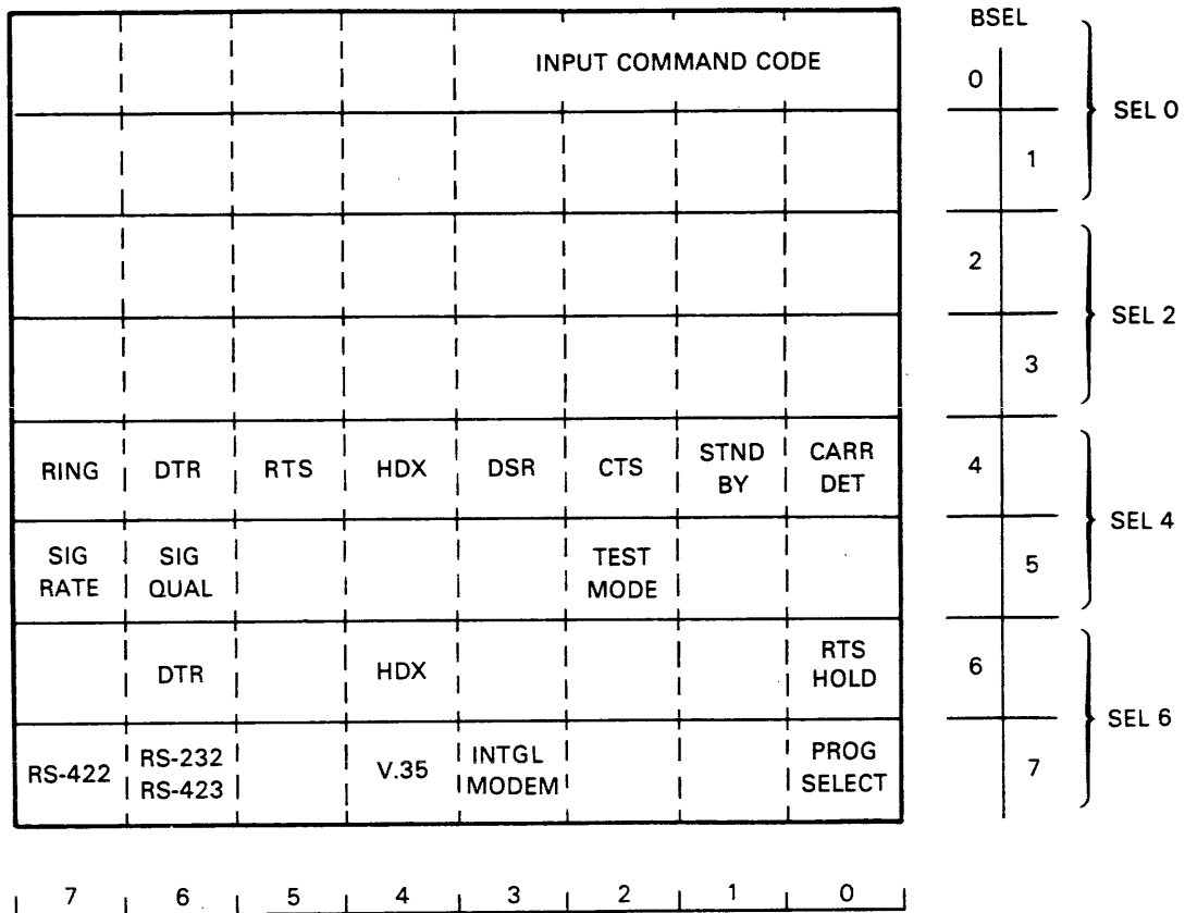
Figure 3-4 Modem Status Read Format
