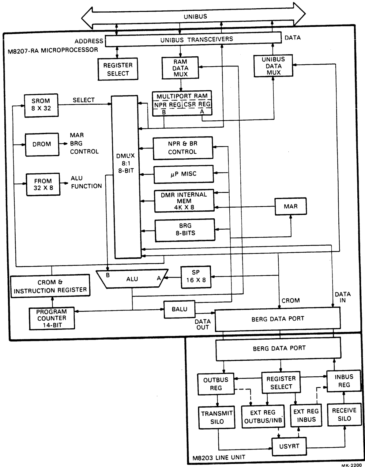
Figure D-1 Data and Control Flow - Basic
