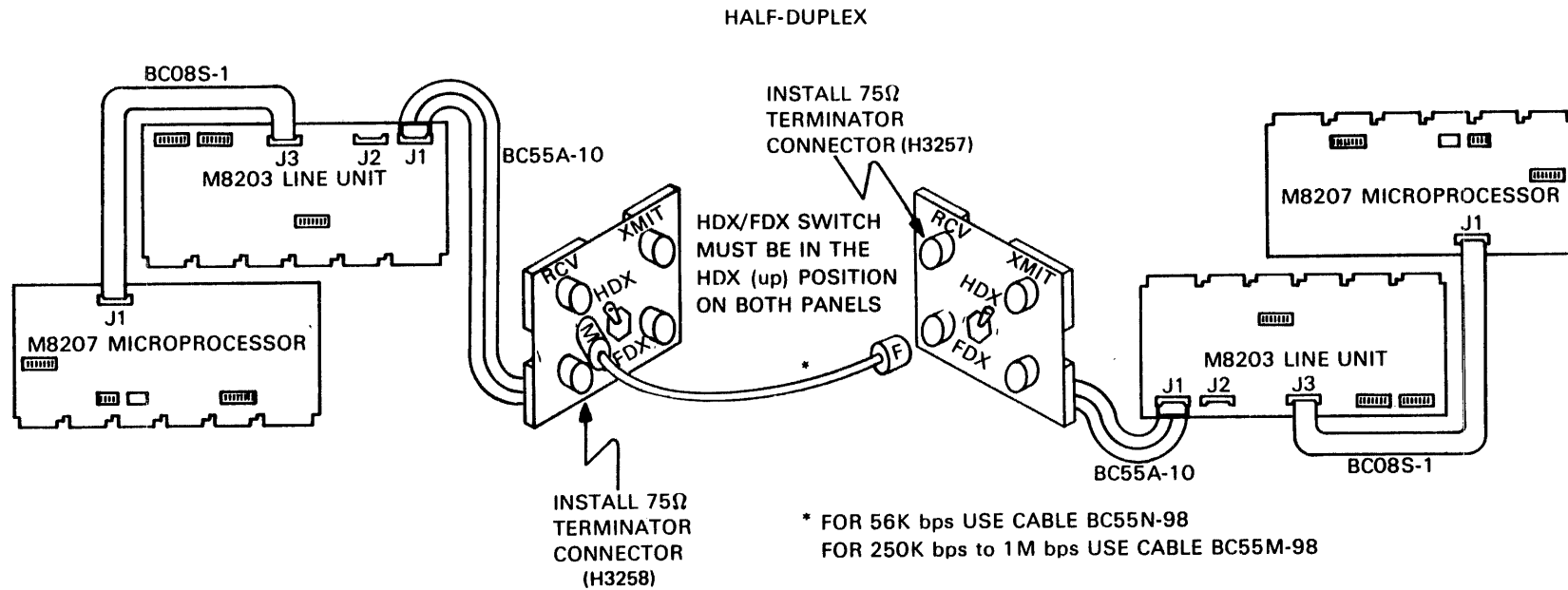
Figure 2-8 DMR11 to DMR11 Integral (Local) Modem Cabling Diagram
