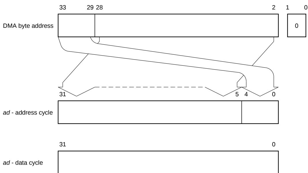
Figure 1-5. Interpretation of the ad signal during a DMA transaction
