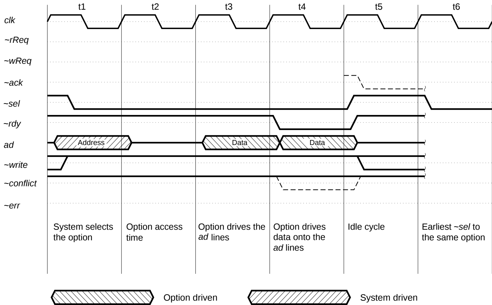
Figure 1-1. I/O read of an option by the system
