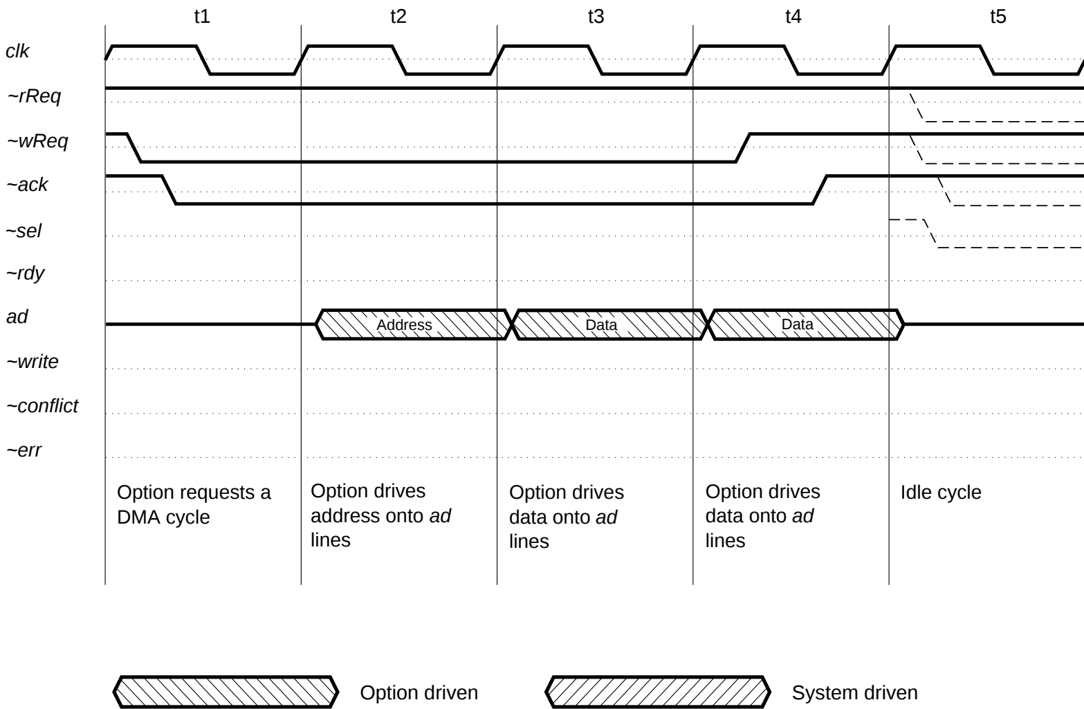
Figure 1-9. Two-word DMA write to the system by an option
