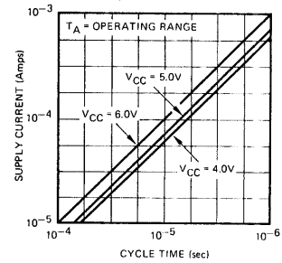
FIGURE 7. DYNAMIC SUPPLY CURRENT ( I_{CC3} ) VERSUS CYCLE TIME
