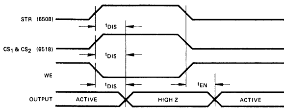
FIGURE 3. OUTPUT ENABLE
