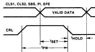
FIGURE 2. CONTROL REGISTER LOAD CYCLE
