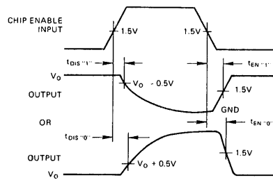
FIGURE 2. OUTPUT ENABLE AND DISABLE TIMES
