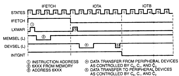
DEVICE INTERRUPT GRANT RESET TIMING
