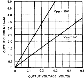
OUTPUT SINK CURRENT I_{OL} DECREASES 0.3%/°C
