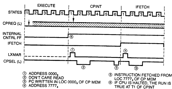
CONTROL PANEL INTERRUPT GRANT TIMING
