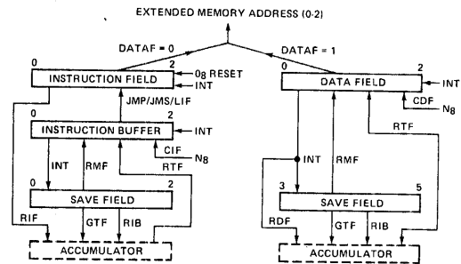
FIGURE 4: EMA REGISTERS
