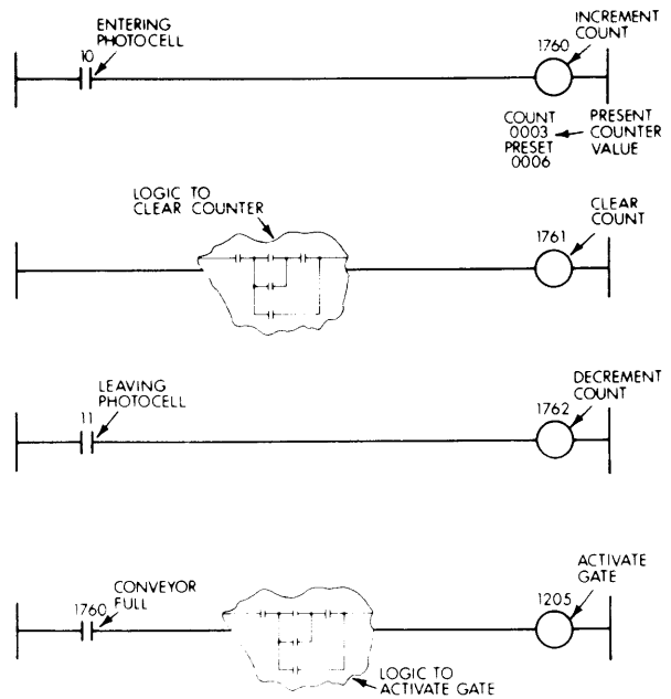
Figure 1-25 Limiting Parts on a Conveyor Using an Up-Down Counter
