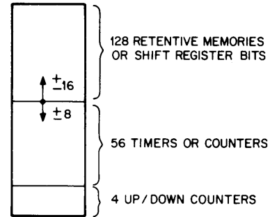
Figure 1-20 Internal Function Partitioning
