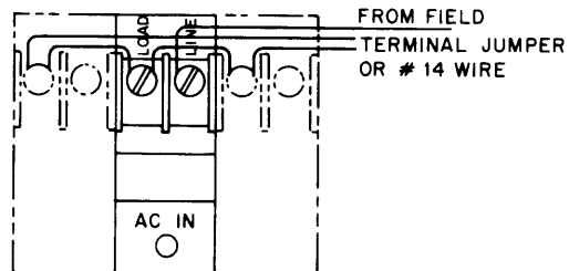
Figure 2-7 Field Wiring Connections to Converters
