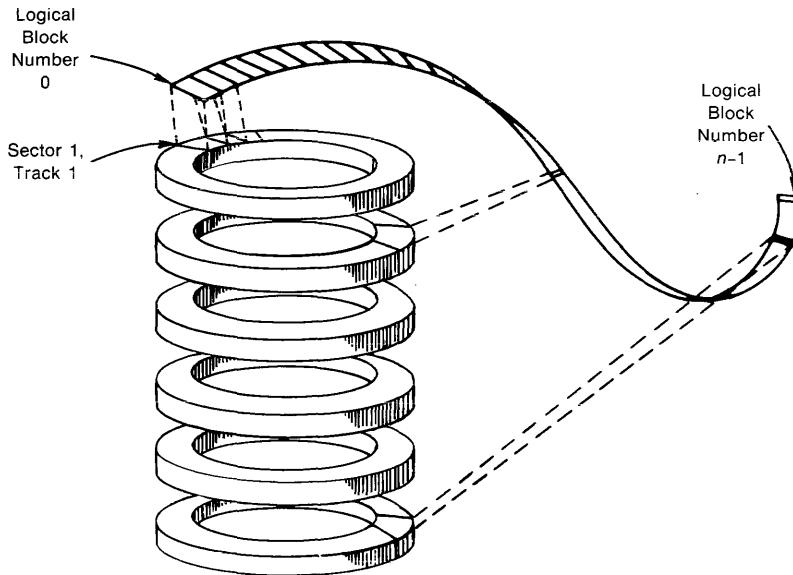
Figure 2: Logical Disk Structure
