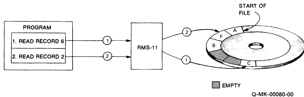
Figure 1-21: Program Randomly Reading a Relative File
