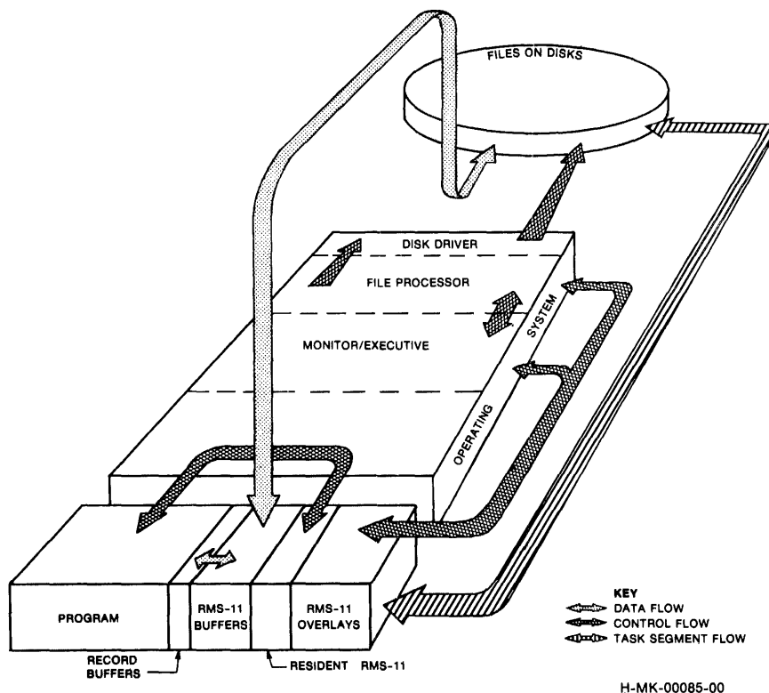
Figure 1-27: RMS-11's Environment
