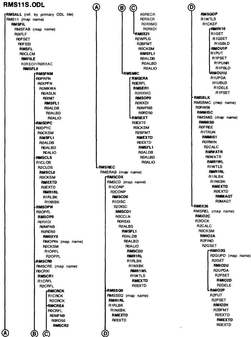
Figure C-1: RMS11S.ODL and RMS11X.ODL Overlay Structures (Cont).
