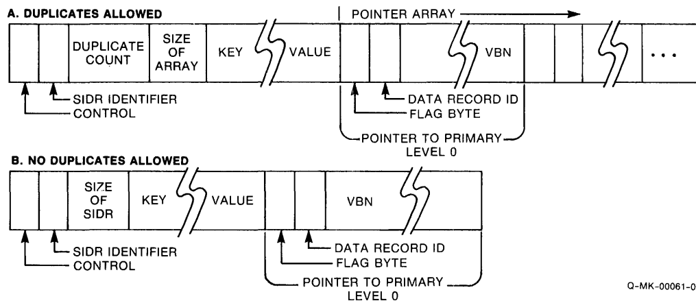
Figure 5-4: Format for Secondary Index Data Record
