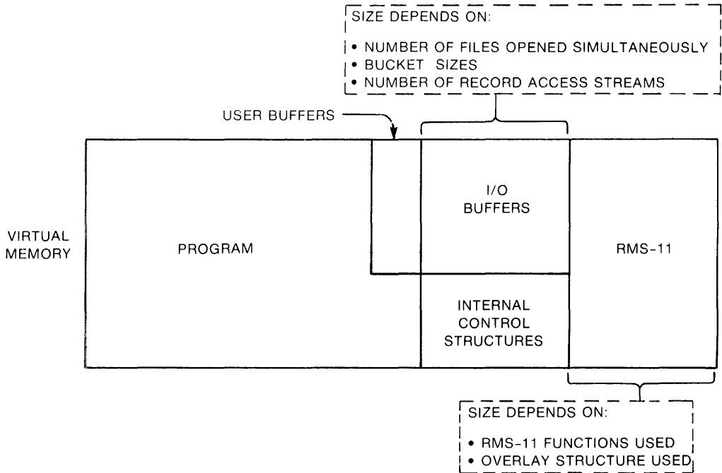
Figure 1-25: RMS-11 Task Structure
