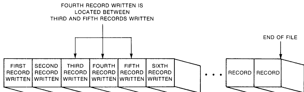
Figure 1-14: Sequential File Organization
