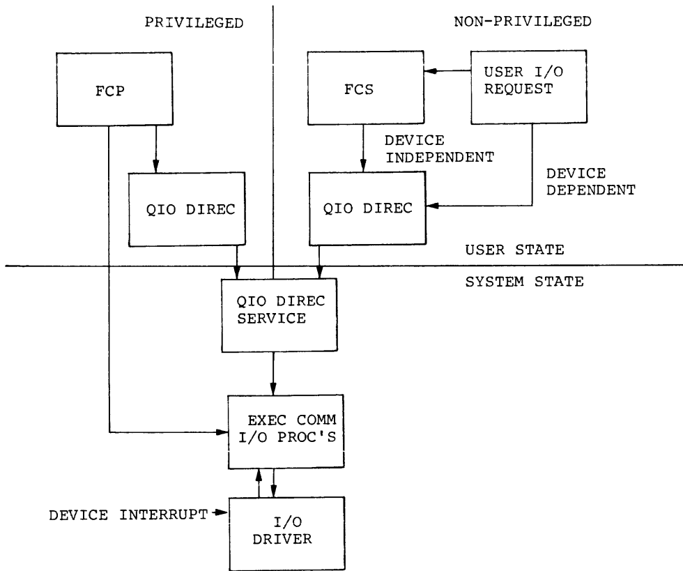
Figure 1-1 I/O Control Flow
