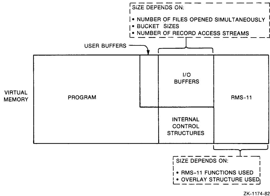
Figure 3-1: RMS-11 Task Structure
