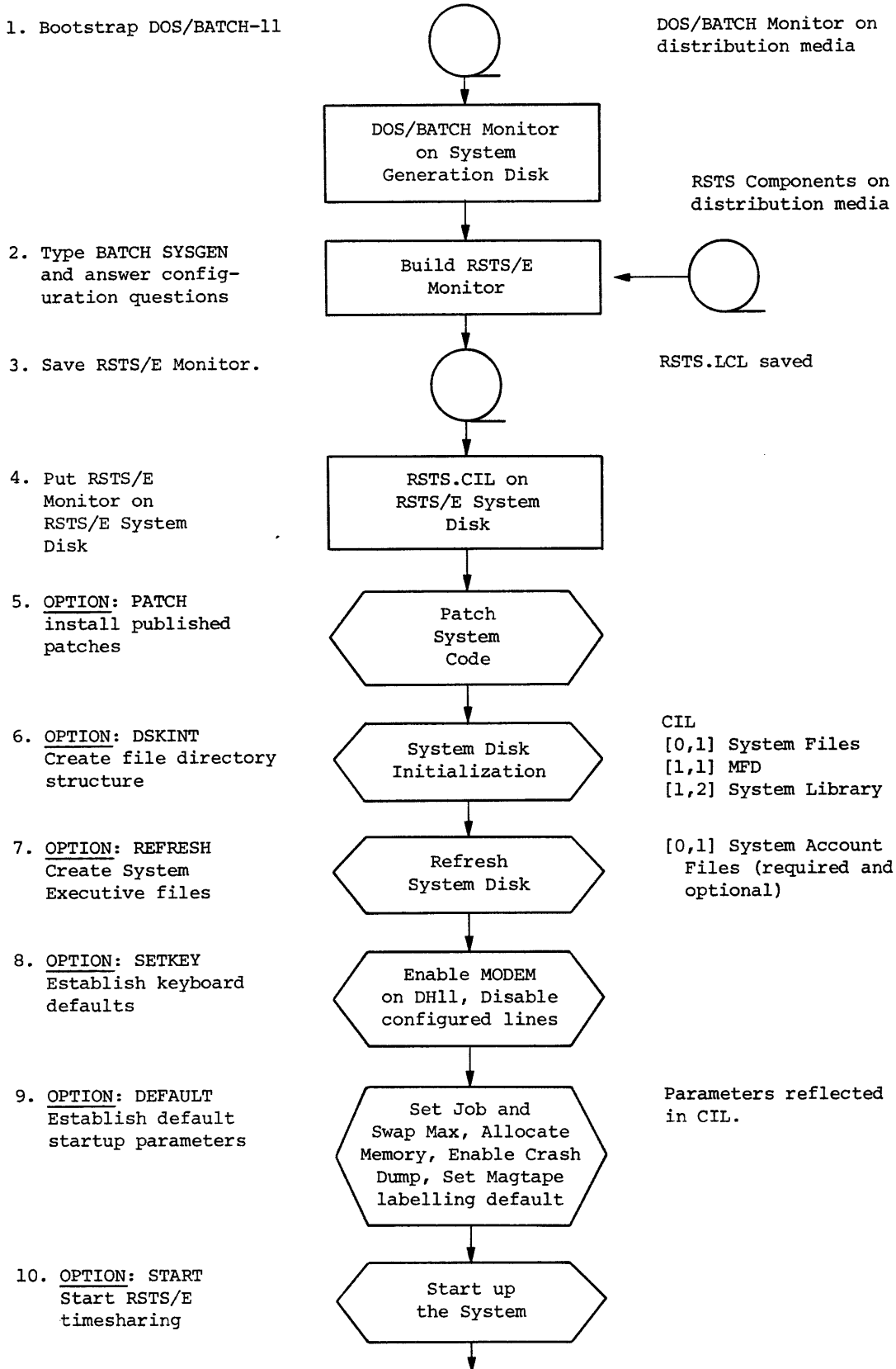
Figure 1-1 System Generation Flow Chart
