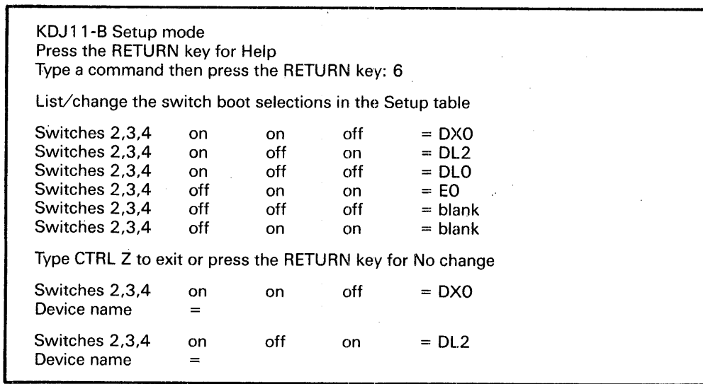
Figure 4-7 Switchpack Boot Selection
