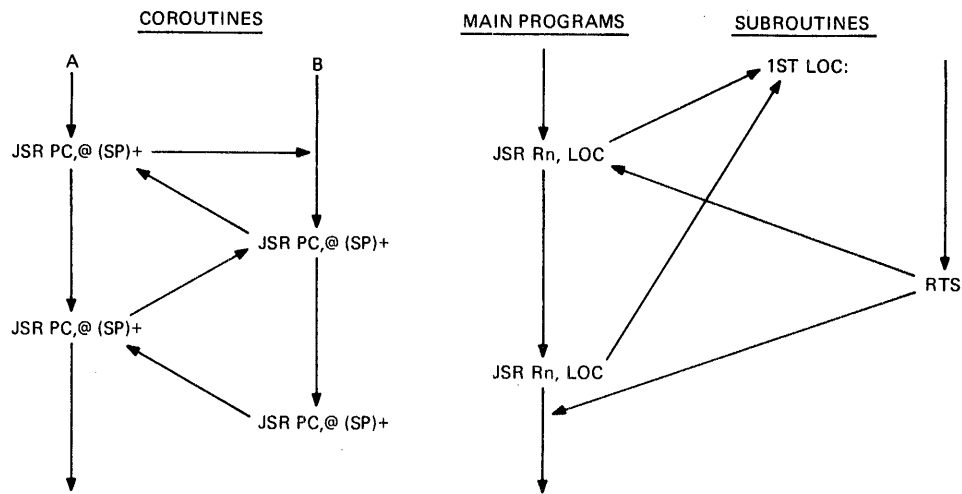
Figure 11-9 Coroutines Versus Subroutines
