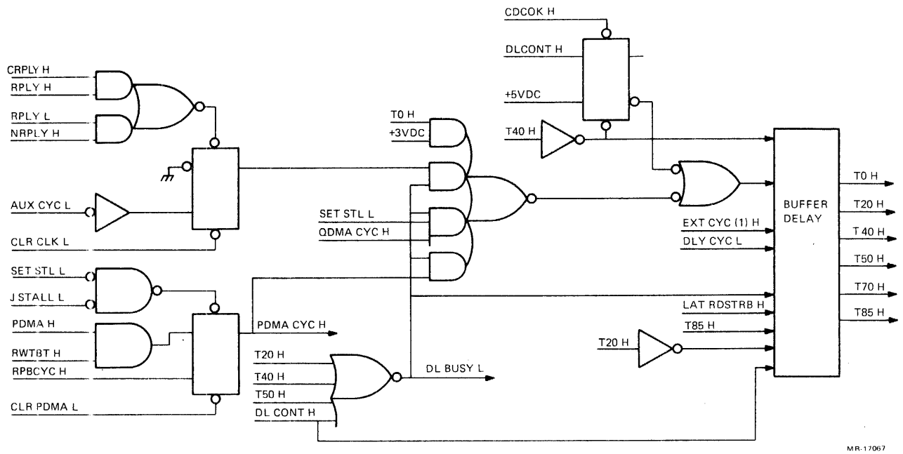
Figure 5- 6 Oscillator Control
