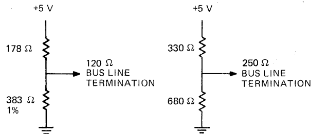
Figure 6-14 Bus Line Termination
