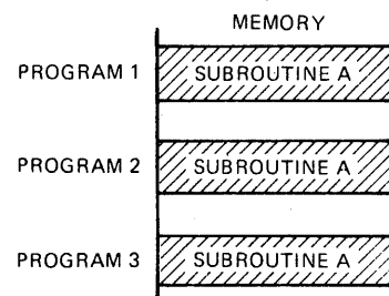
CONVENTIONAL APPROACH A SEPARATE COPY OF SUBROUTINE A MUST BE PROVIDED FOR EACH PROGRAM.
