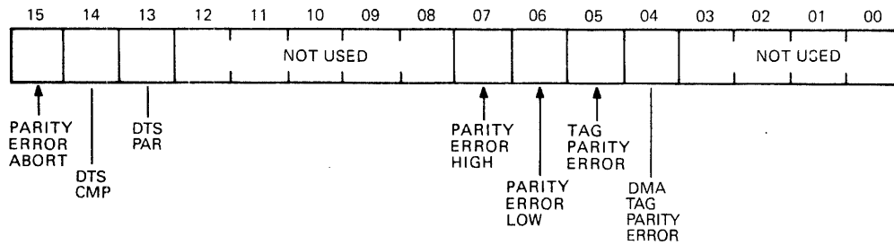
Figure 1-25 Memory System Error Register (MSER)
