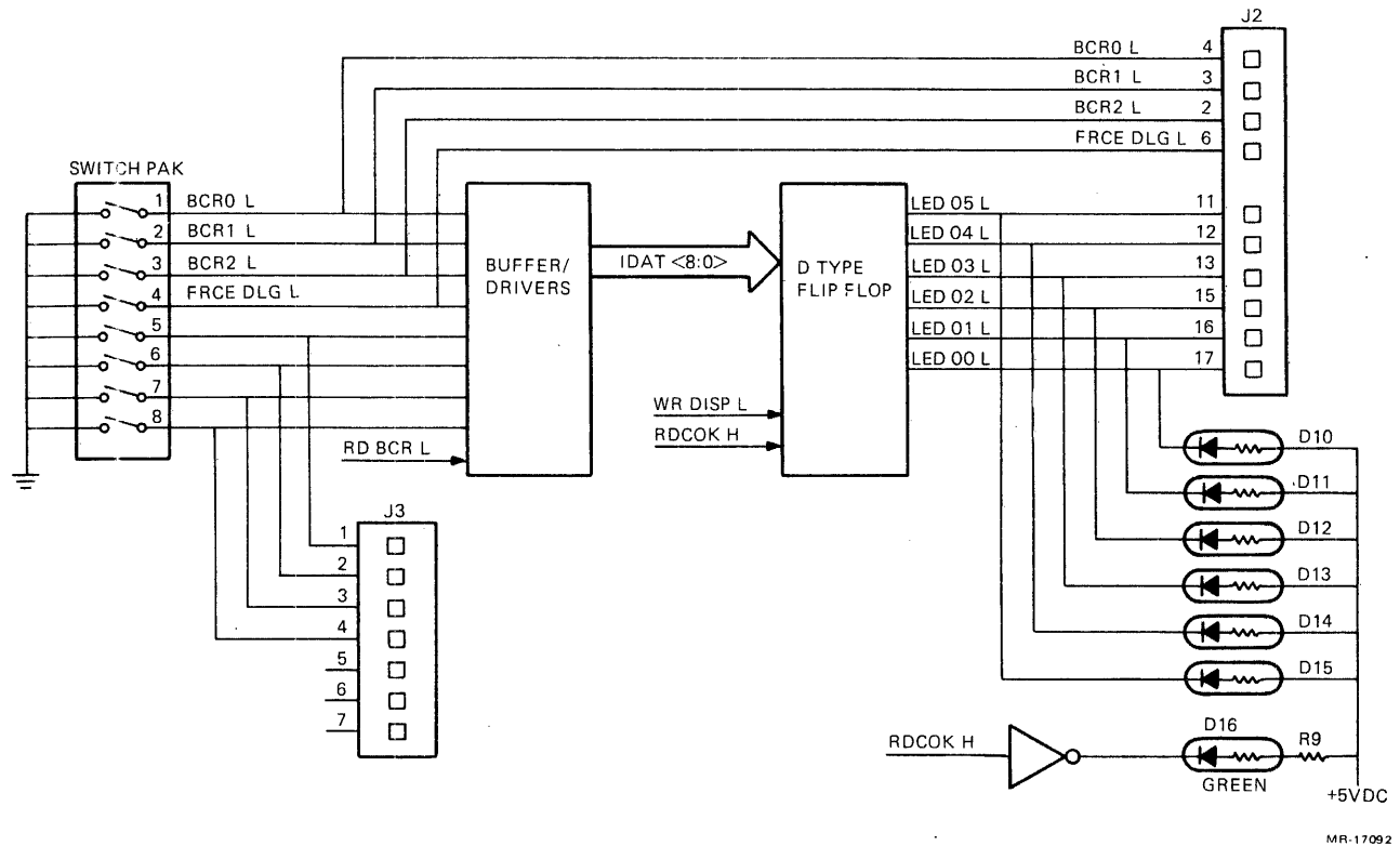
Figure 5-37 Configuration and Display Circuits
