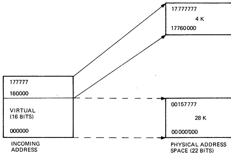
Figure 1-5 16-Bit Mapping
