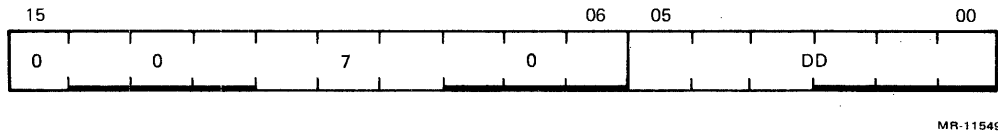
Figure 9-11 Call to Supervisor Mode
