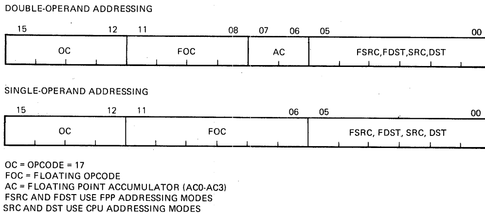
Figure 10-5 Floating-Point Addressing Modes
