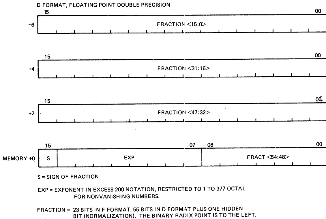
Figure 10-2 Double-Precision Format
