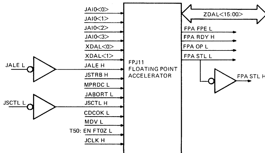
Figure 5-40 Floating-Point Accelerator
