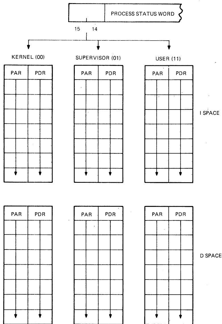
Figure 1-12 Active Page Register
