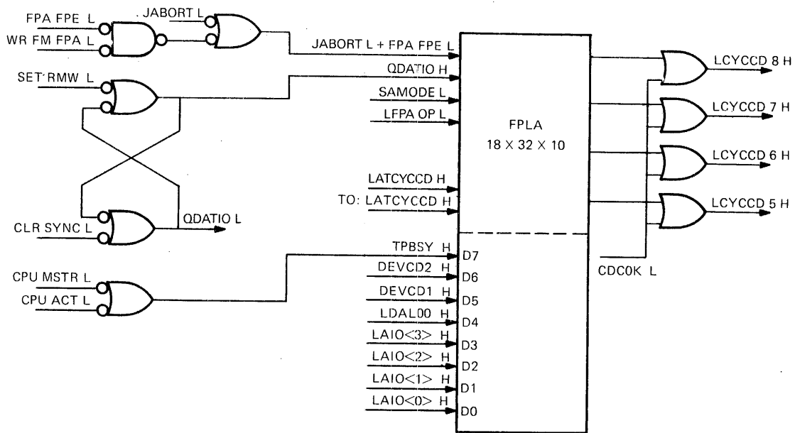
Figure 5-14 Cycle Encoder
