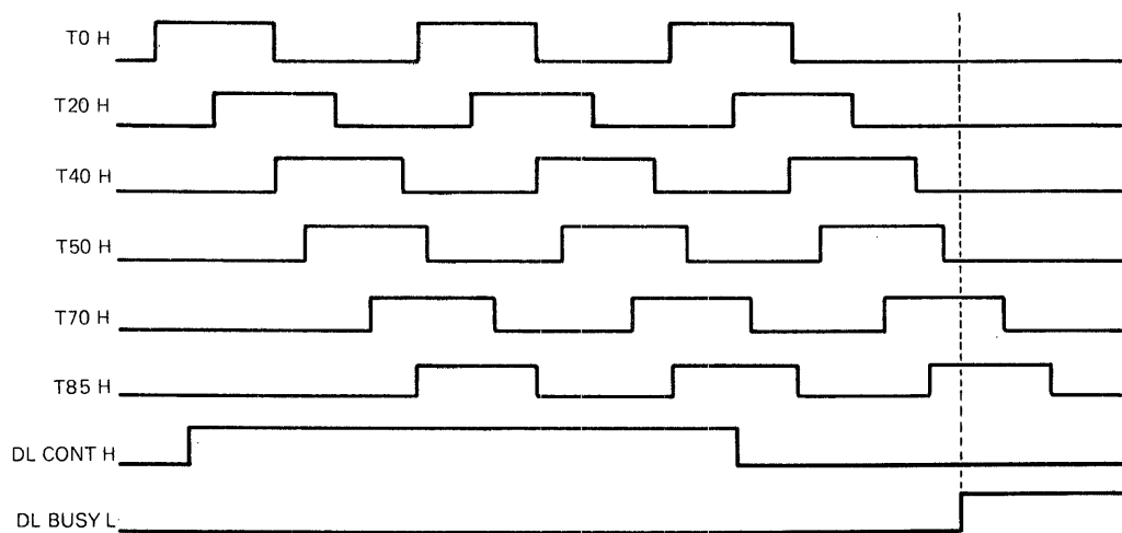
Figure 5-15 Oscillator Outputs
