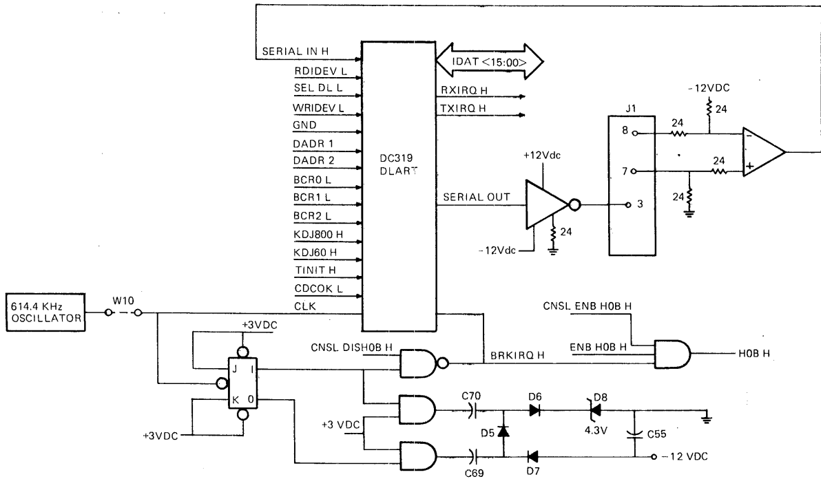
Figure 5-35 Console Serial Line Logic
