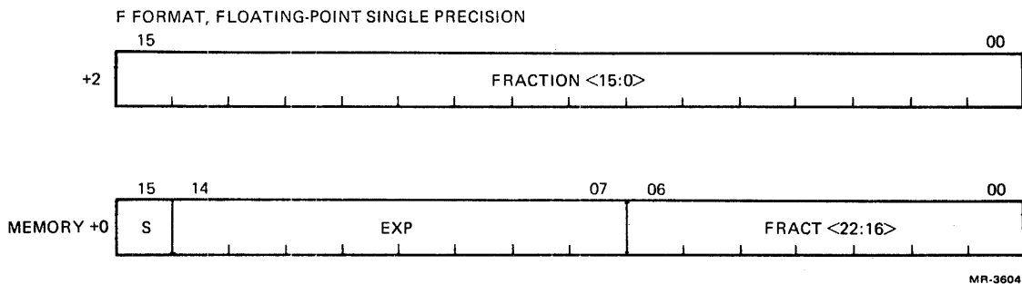
Figure 10-1 Single-Precision Format
