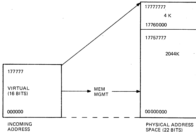
Figure 1-7 22-Bit Mapping
