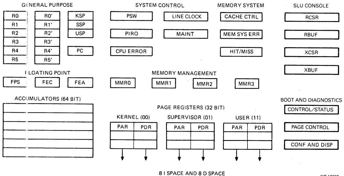
Figure 1-1 Programming Model
