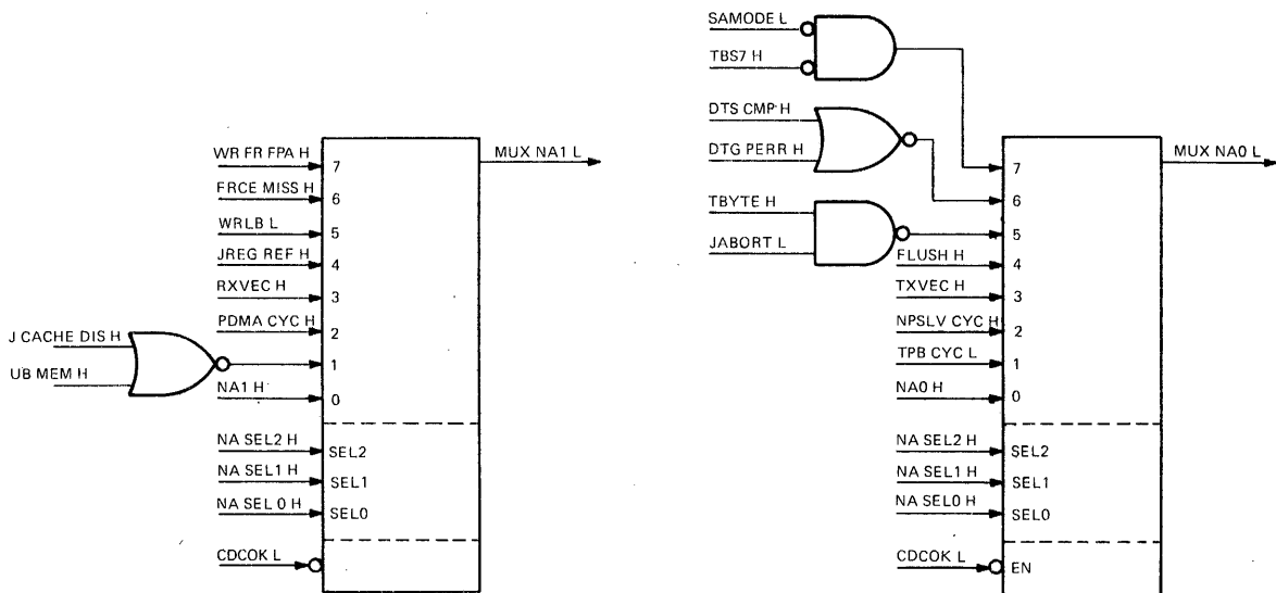
Figure 5-17 Next Address Multiplexer
