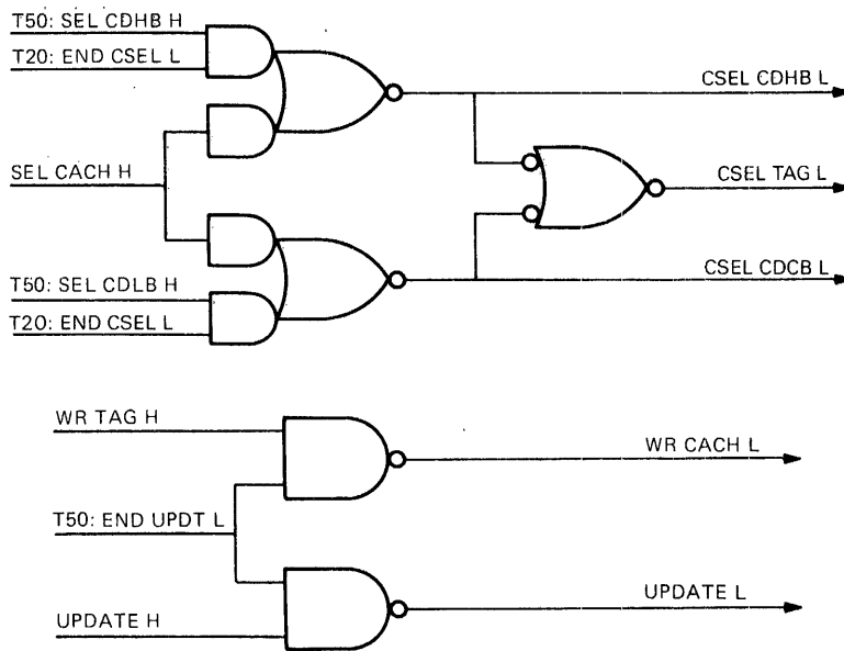
Figure 5-28 Cache Control Signals
