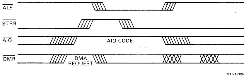
Figure 5-3 NOP Transaction
