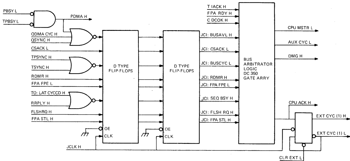
Figure 5-11 Bus Arbitrator
