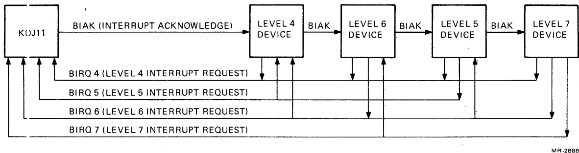
Figure 6-11 Position-Independent Configuration
