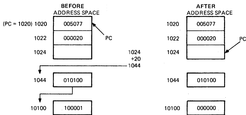
Figure 8-31 CLR @A Clear
