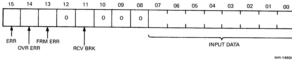
Figure 1-27 Receiver Buffer Register
