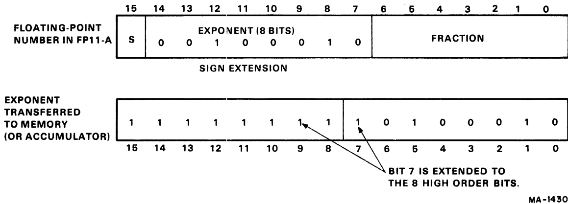
Figure 5-8 Store Exponent Example No. 2
