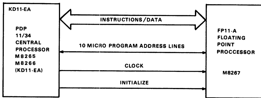
Figure 1-1 KD11-EA/FP11-A Signal Interface
