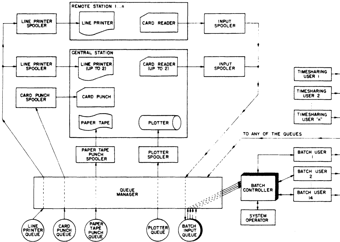
Figure 1-2 Programs in the Batch System
