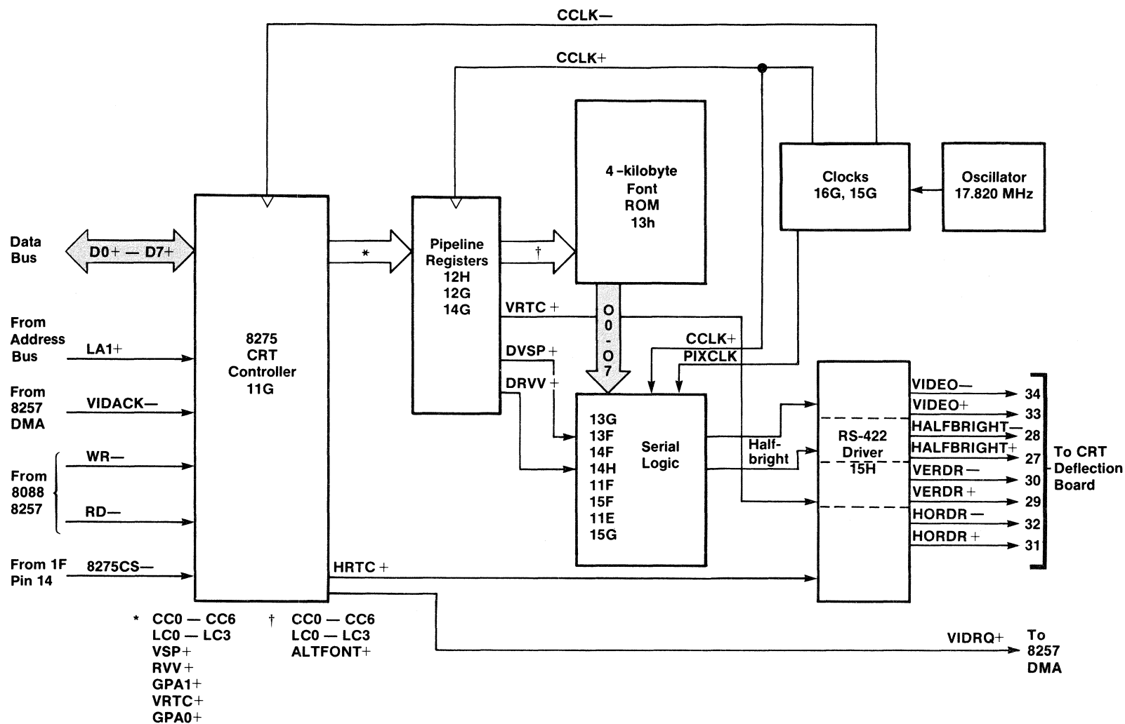
Figure 3-10. Video Display Control Logic.
