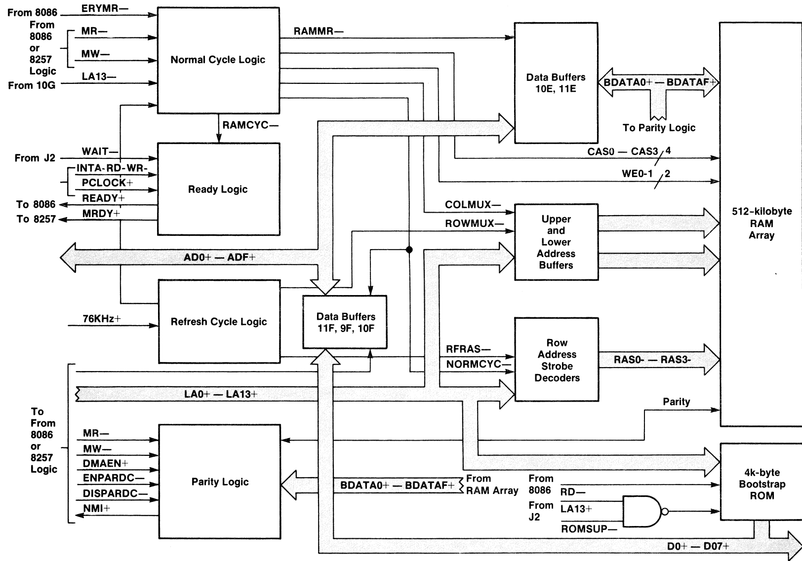
Figure 3-15. Memory Logic.
