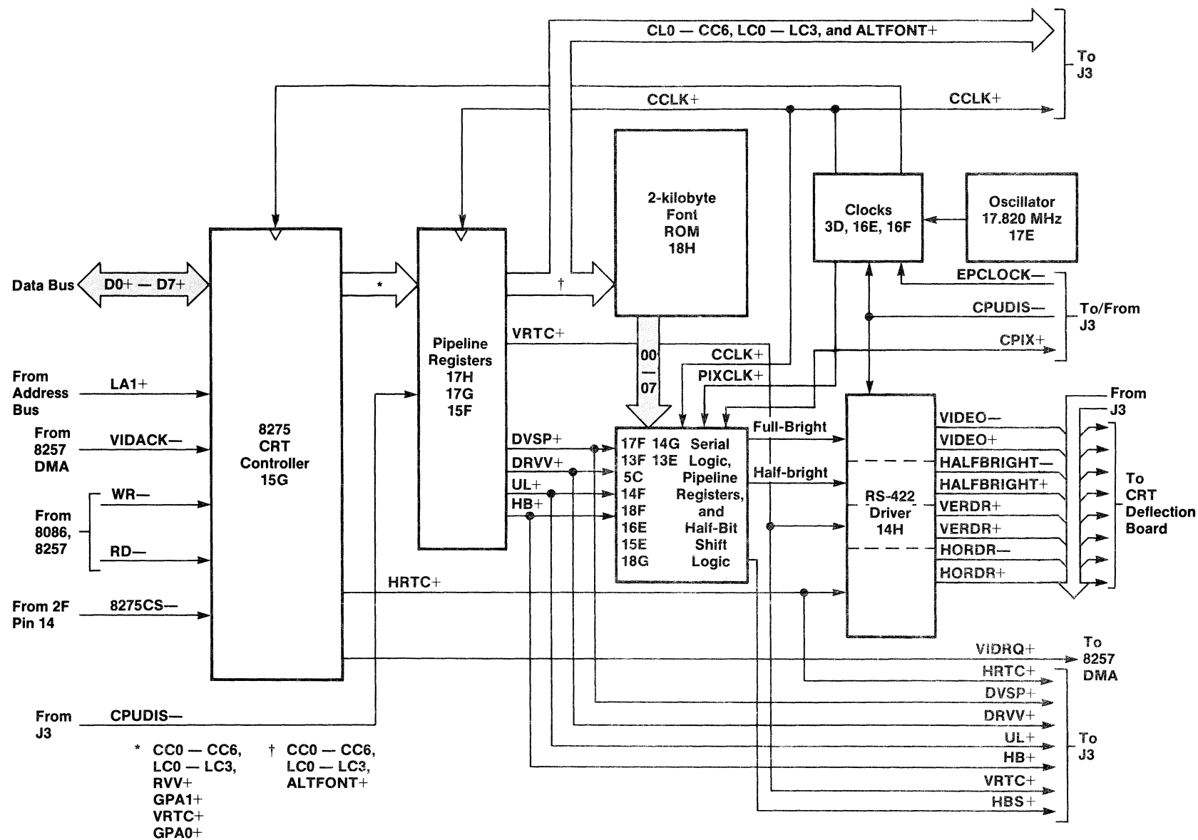
Figure 3-21. Video Display Control Logic.
