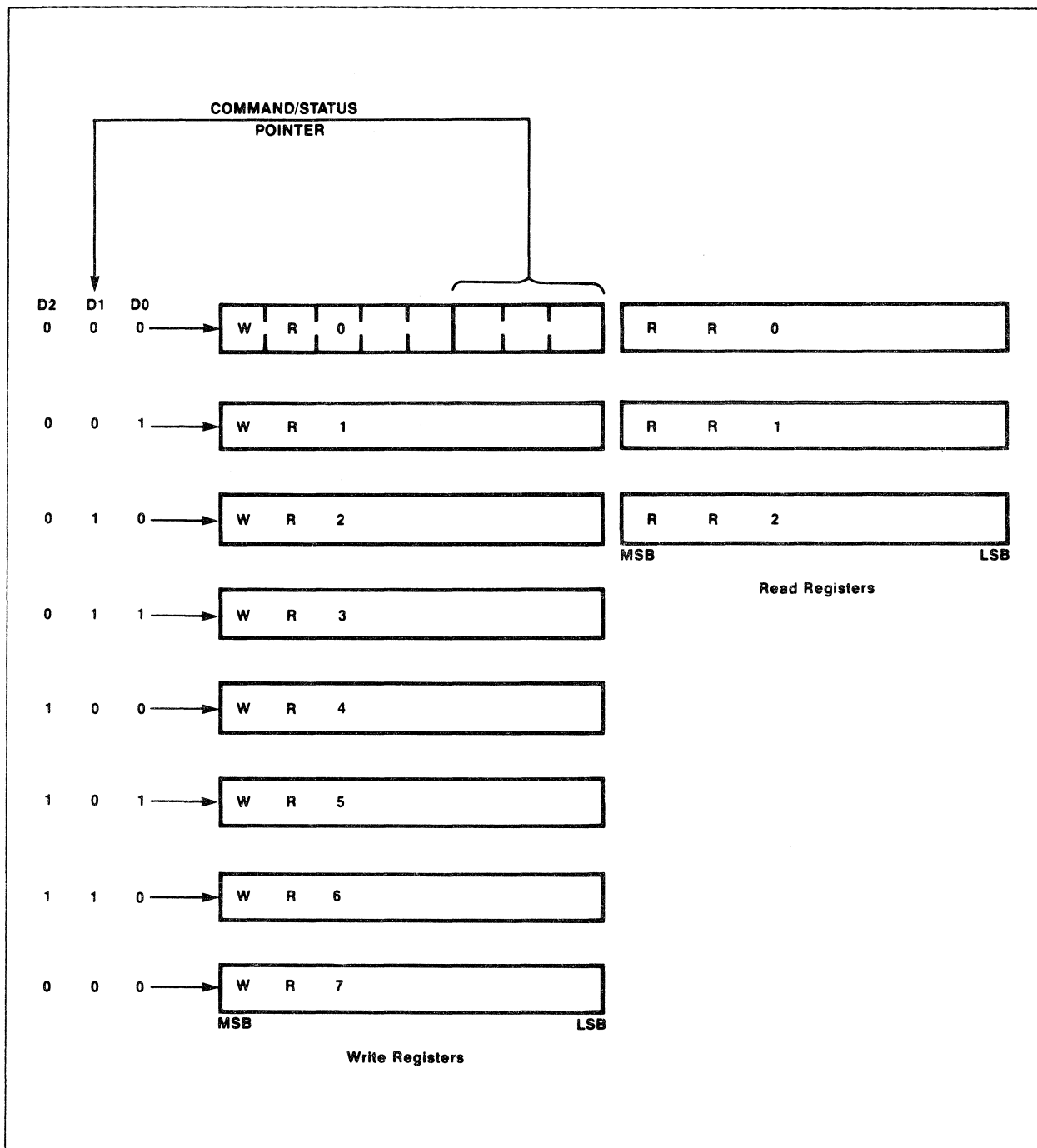
Figure 2-4. 7201 Register Hierarchy.
