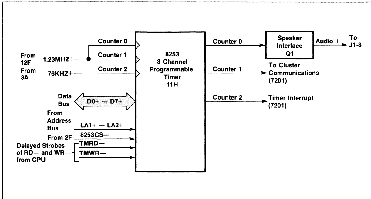
Figure 3-19. Timer Logic and Speaker Interface.
