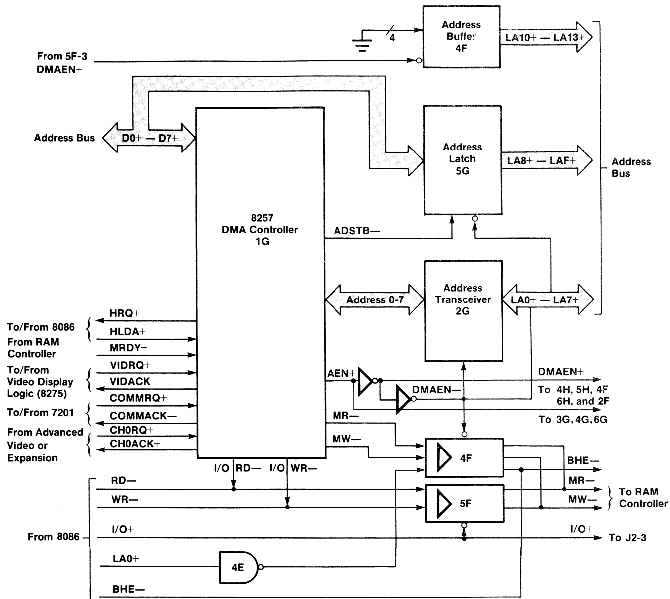
Figure 3-16. DMA Logic.
