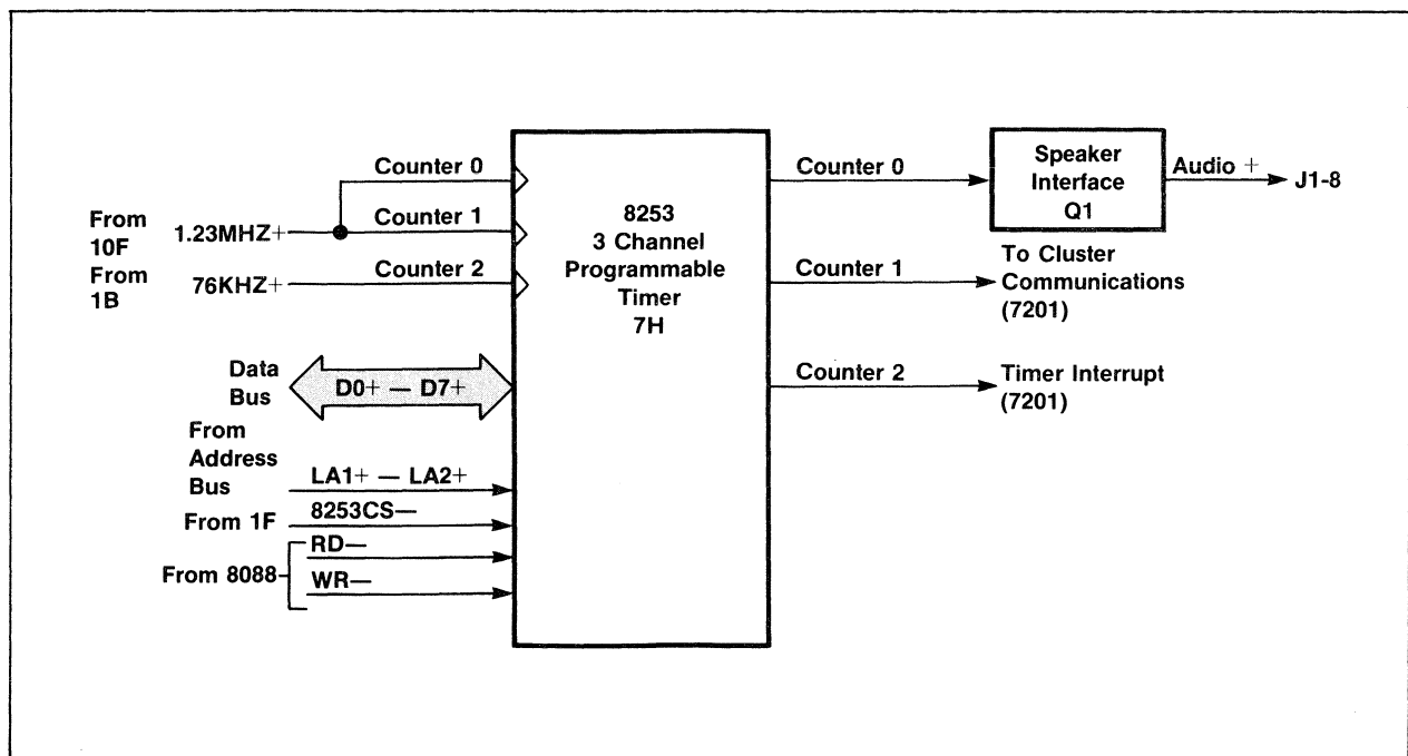
Figure 3-8. Timer Logic and Speaker Interface.
