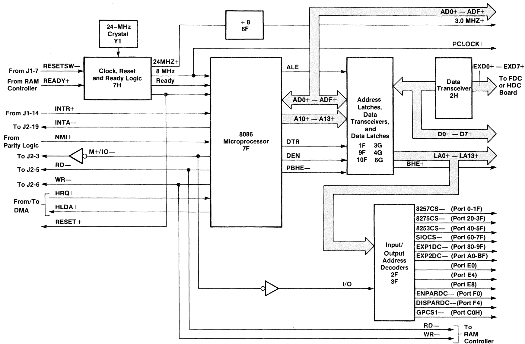
Figure 3-13. 8086 Microprocessor Logic.
