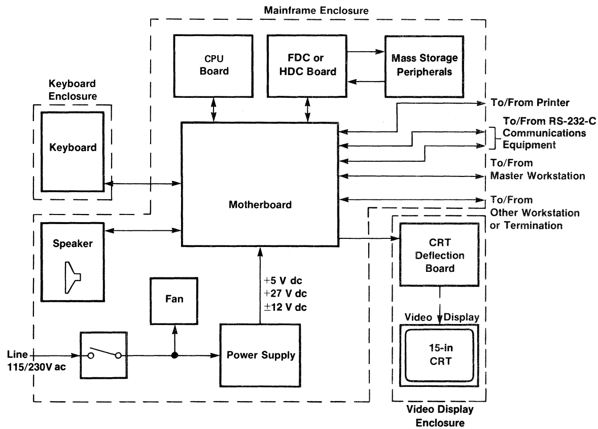
Figure 1-1. AWS-220, -230, and -240 Workstations.
