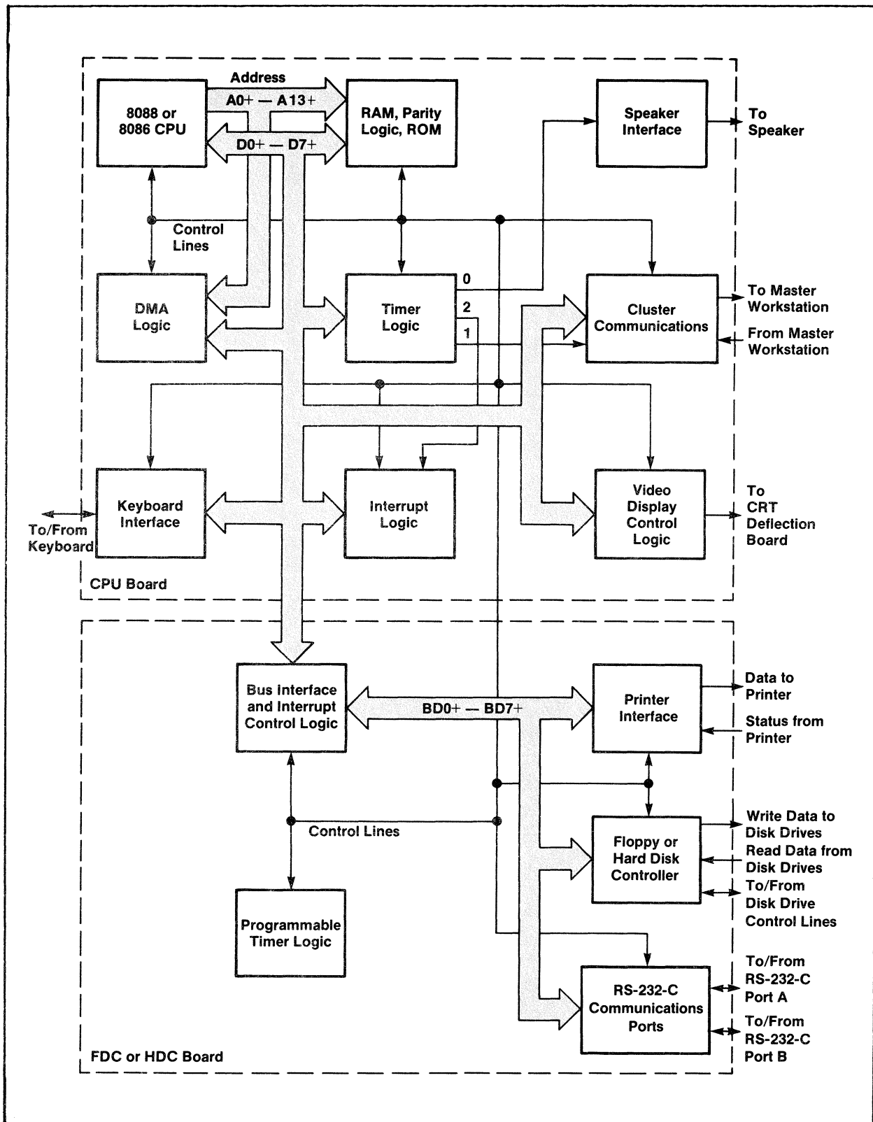
Figure 2-1. Workstation Logic.
