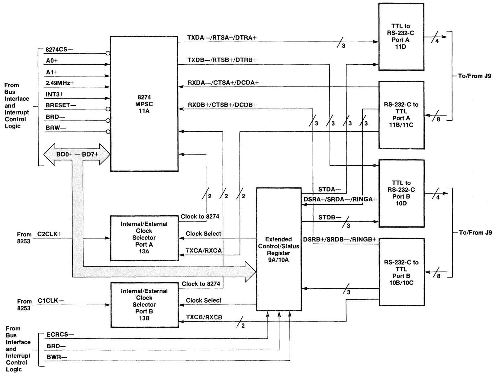
Figure 3-27. RS-232-C Communications Logic.
