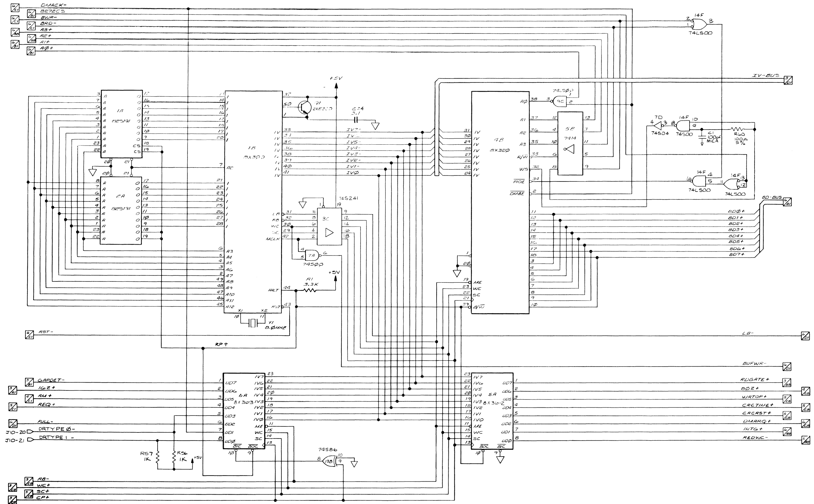
Figure 3-31. HDC Board Schematic. (Page 2 of 8)
