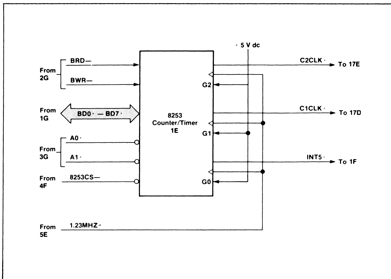
Figure 3-32. 8253 Counter/Timer Logic.
