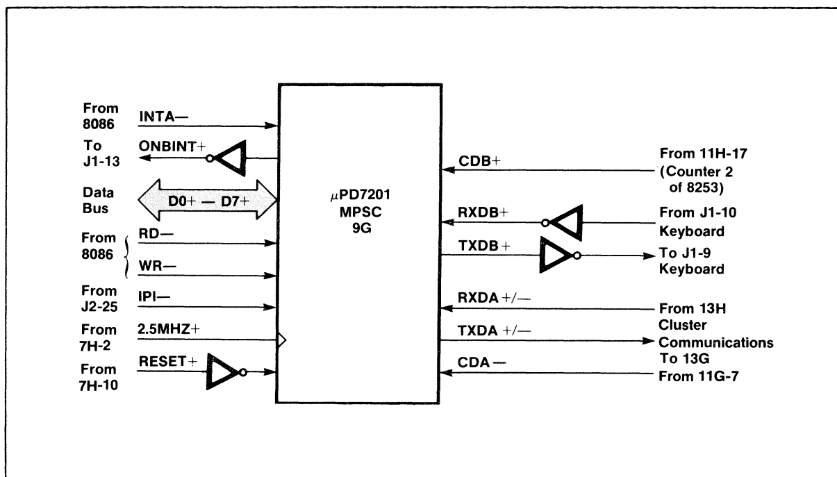
Figure 3-20. Interrupt Logic.
