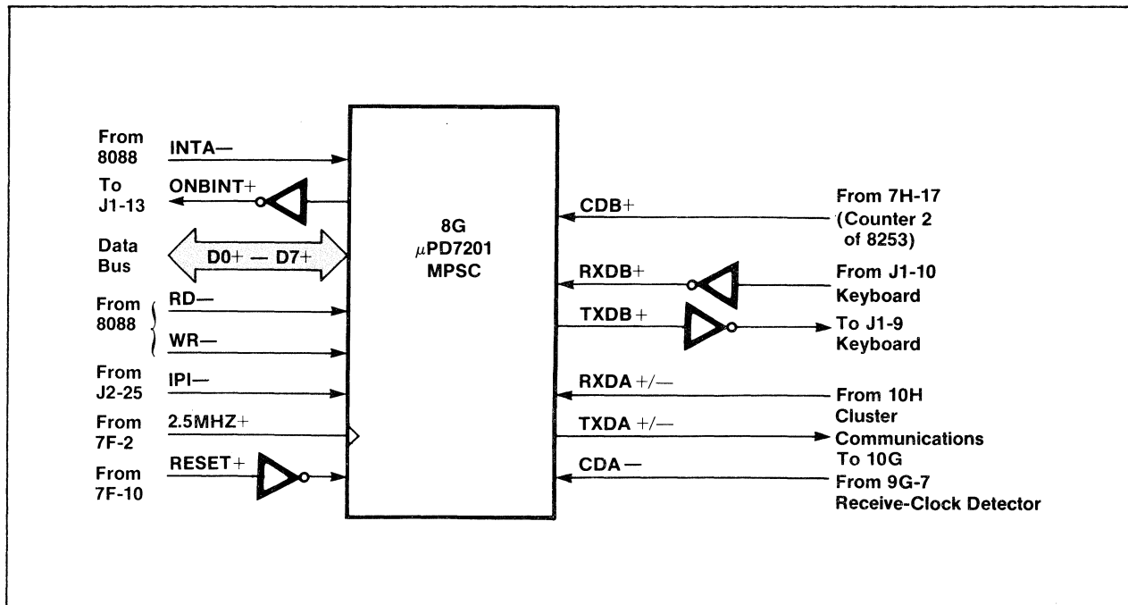
Figure 3-9. Interrupt Logic.
