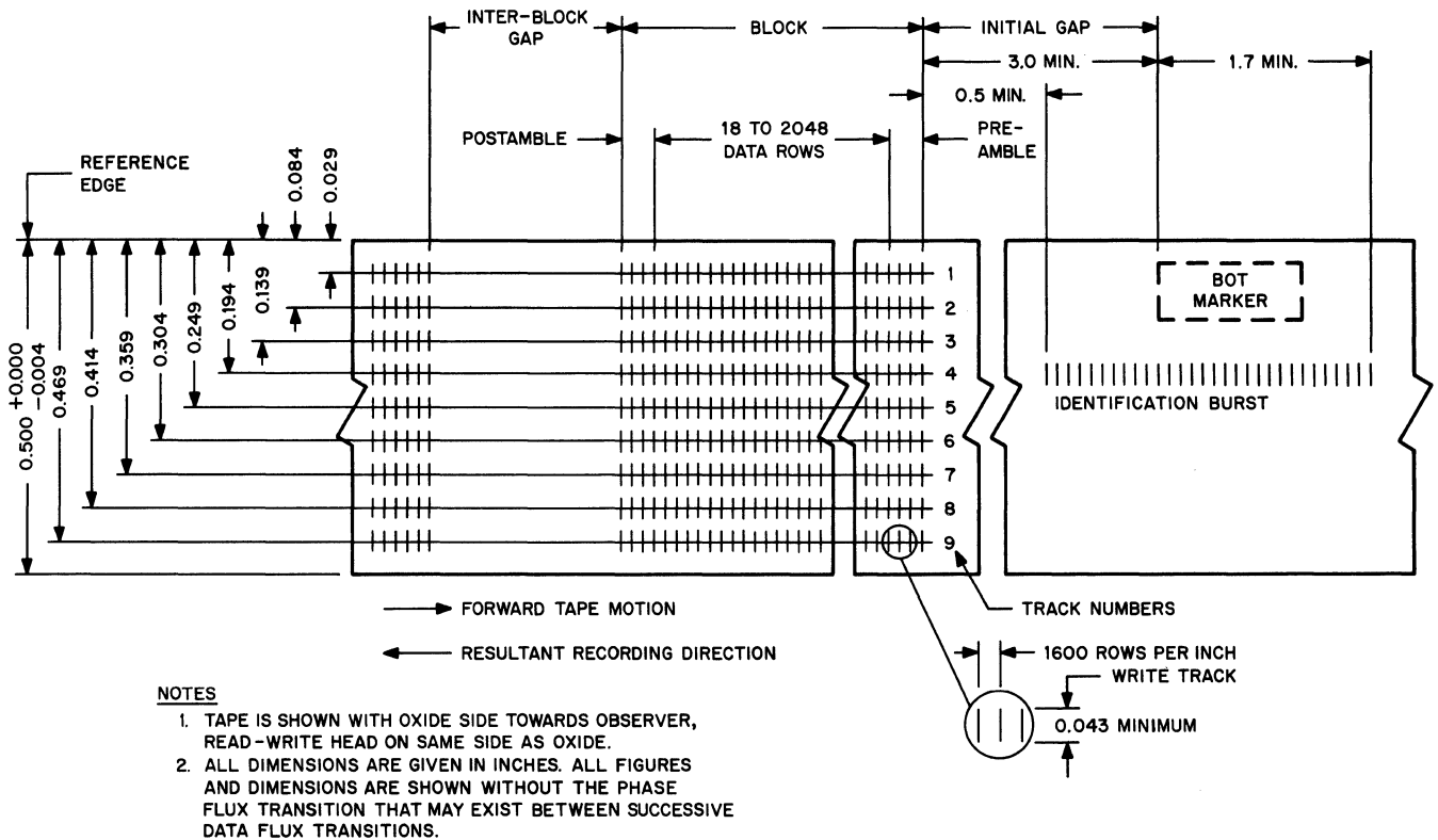
Figure 3. 9-Track 1600 cpi PE Format (Source USASI)
