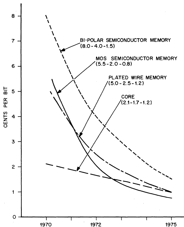
Figure 2. Mainframe Memory Cost per Bit Projection (1 Million Bytes)
