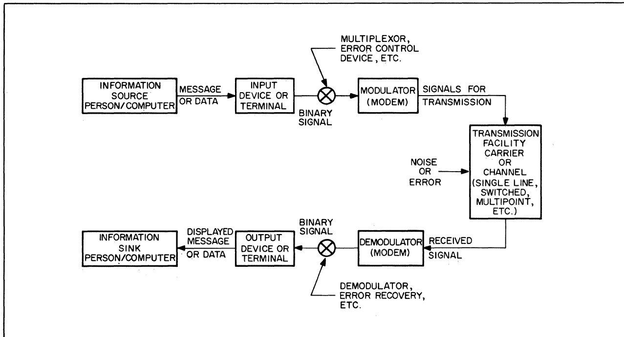
Figure 3. Basic Components of Data Communications Systems
