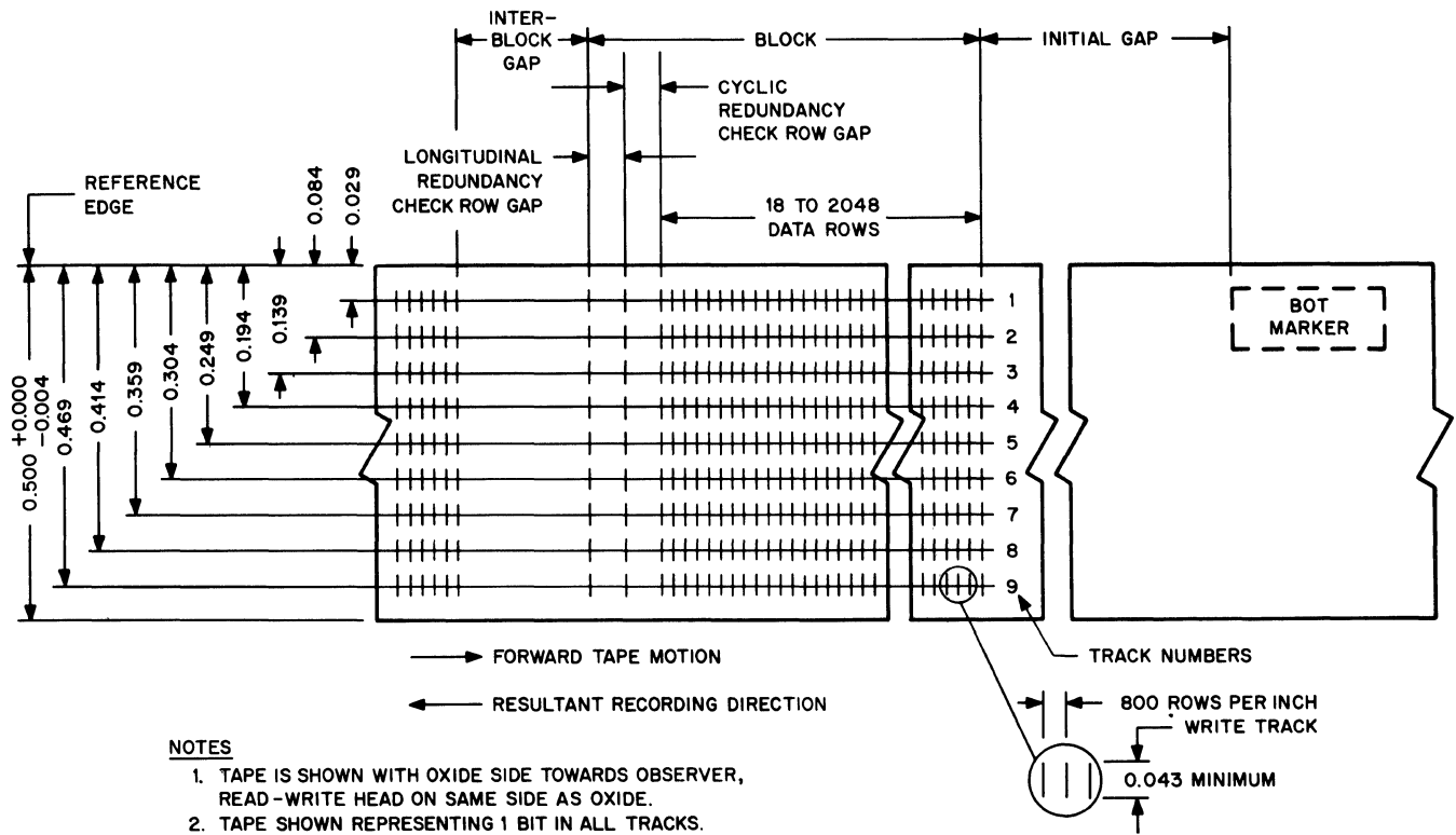
Figure 2. 9-Track Tape Format (Source USASI) 800 cpi
