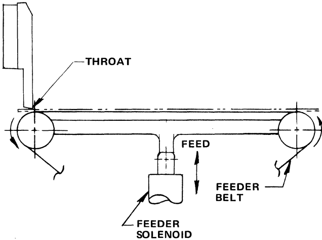
Figure 2. Friction Feed
