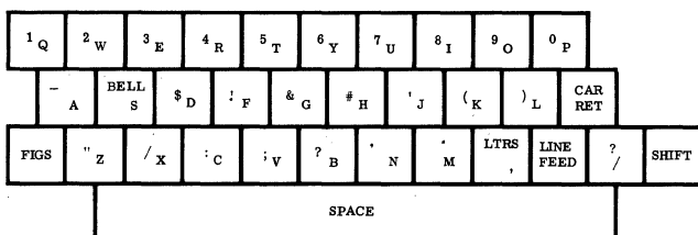
Figure 2. Typical 3-Row Teleprinter Keyboard
