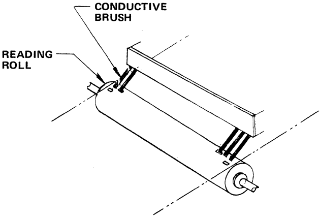
Figure 3. Conductive Brush
