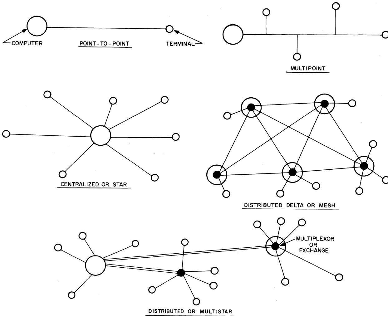
Figure 8. System Configurations
