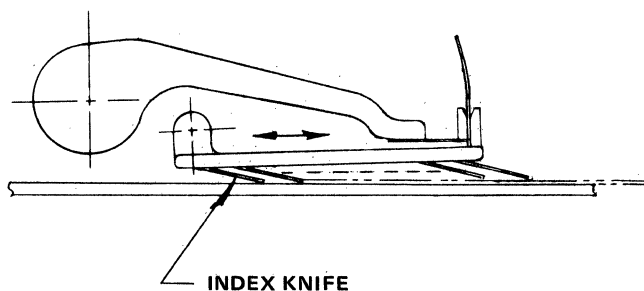
Figure 7. Indexing Knives
