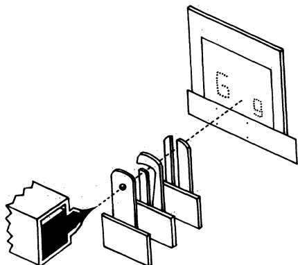
Figure 1. One Method of Inkjet Printing (Courtesy of Teletype Corp.)
