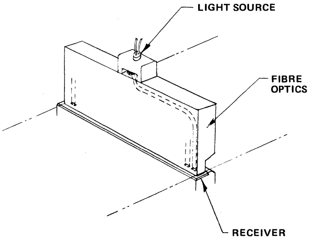
Figure 4. Fibre Optics Read
