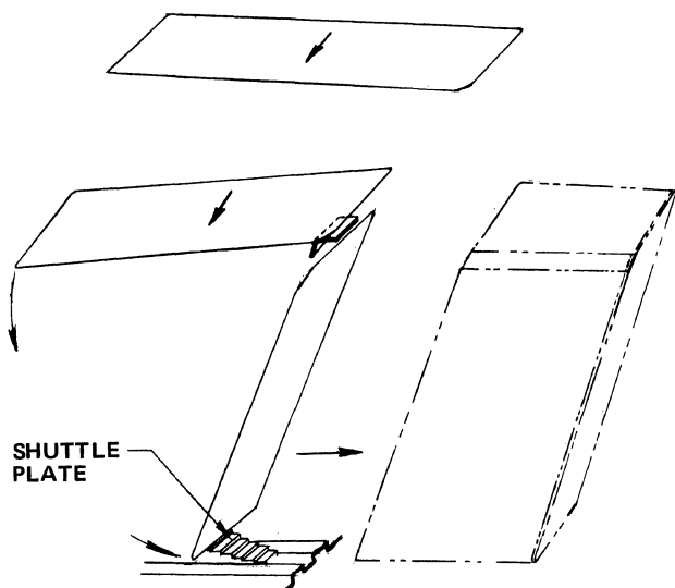
Figure 5. Radial Stacker
