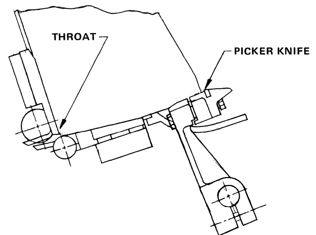
Figure 1. Picker Knife
