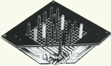
SINGLE-LEVEL MATRIX BOARD (Cutaway view)
