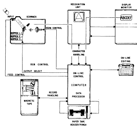
Figure 1. Data Flow
