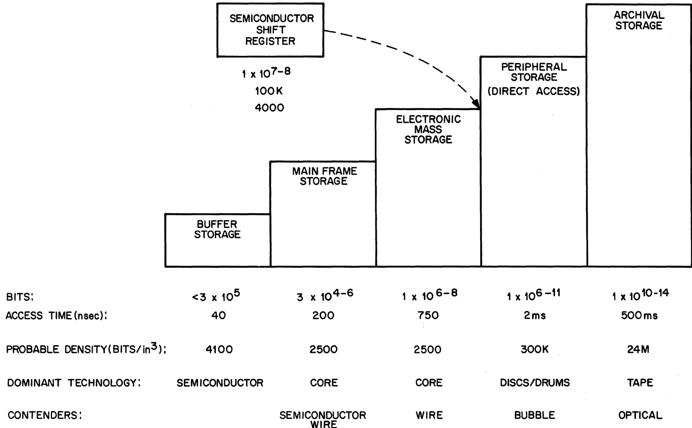
Figure 1. Memory Hierarchy
