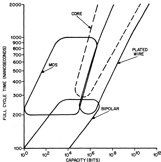
Figure 3. Optimum Cost/Performance/Capacity of Various Memory Technologies
