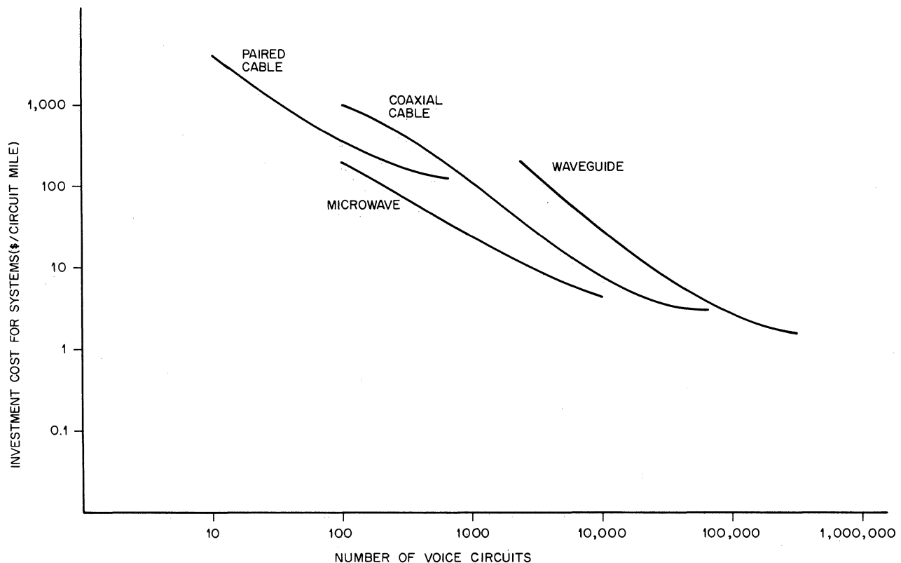
Figure 2. Economics of Scale for Different Communication Technologies
